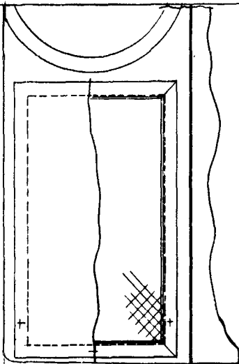
PARTIAL PLAN VIEW SHOWING COLD AIR EXIT OPENING WITH COVER OR SCREEN
