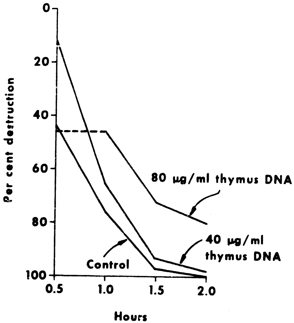
Figure 1. Destruction of E. licheniformis DNA in presence of Calf Thymus DNA by Sonic Extract of E. coli W-1485.
