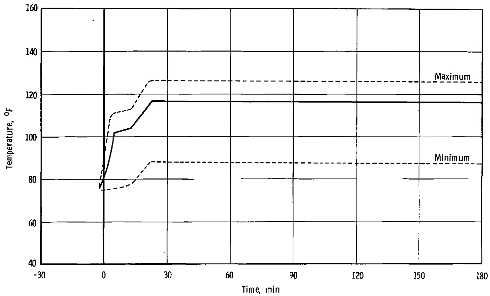
Fig. 25 Model 4 Temperature
