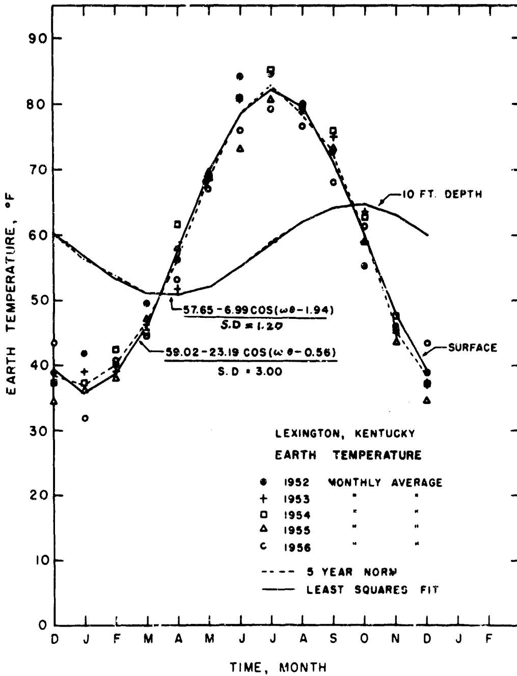
Figure 2 Comparison of least-squares curve, 5-year norm, and observed temperatures at Lexington, Kentucky
