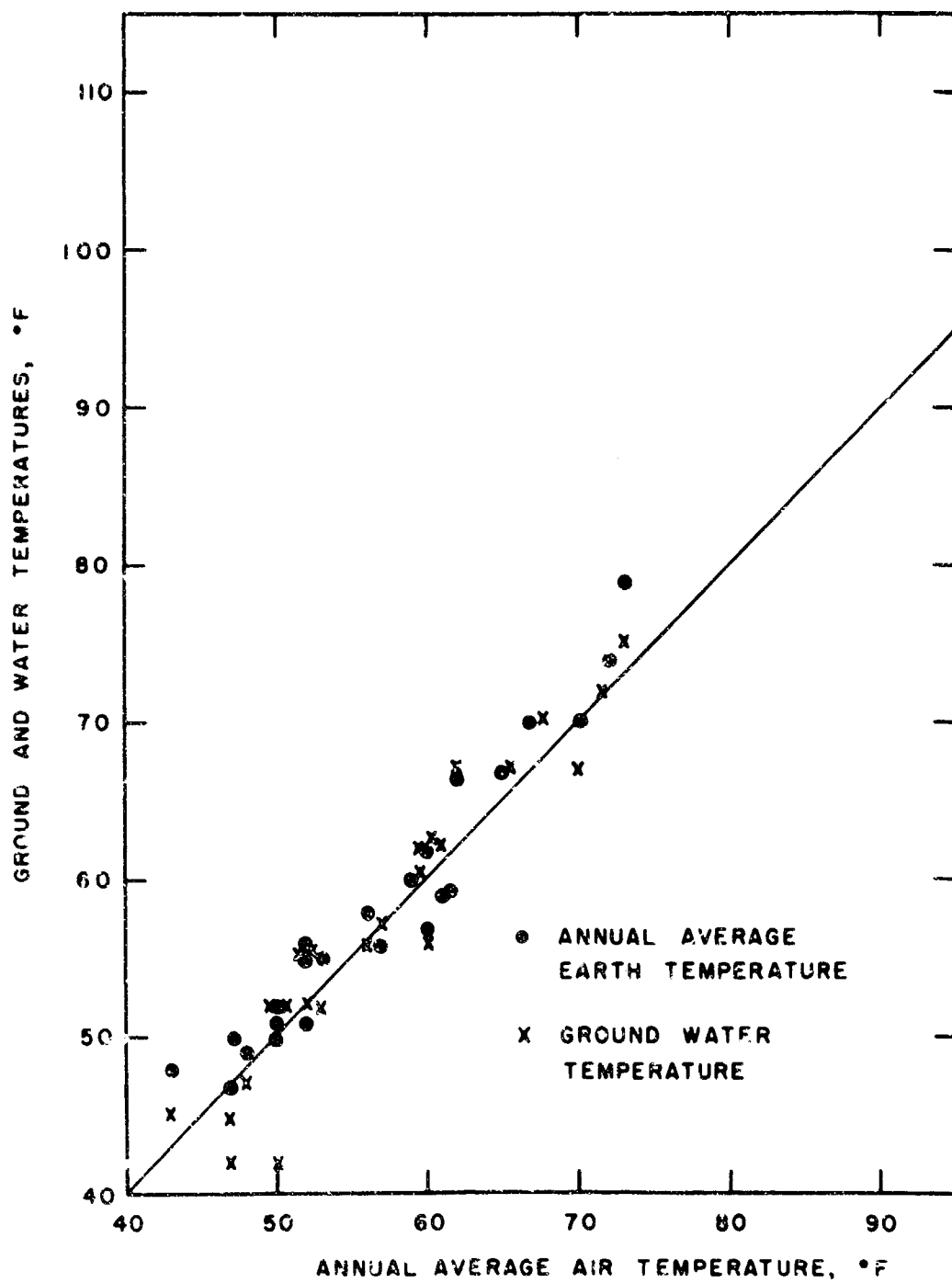
Figure 4 Annual average earth and water temperature vs. annual average air temperature
