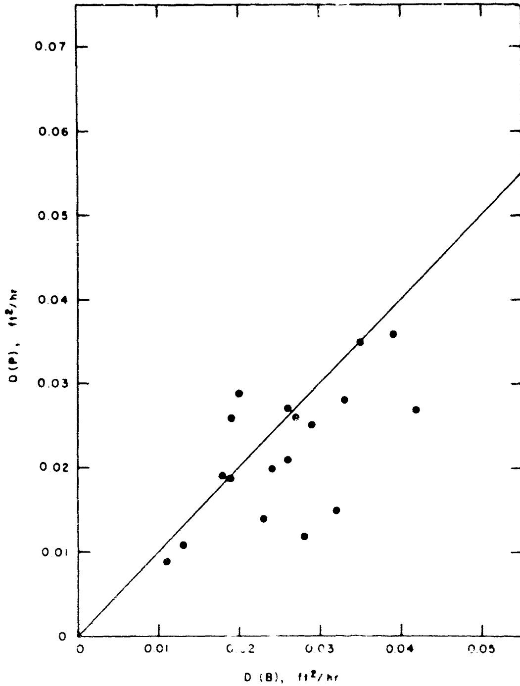
Figure 3 Thermal diffusivities computed by amplitude method and phase angle method
