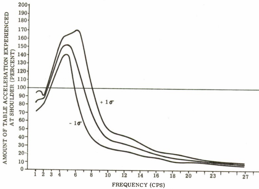
SHOULDER ACCELERATION EXPRESSED AS MEAN PERCENTAGE OF TABLE ACCELERATION
