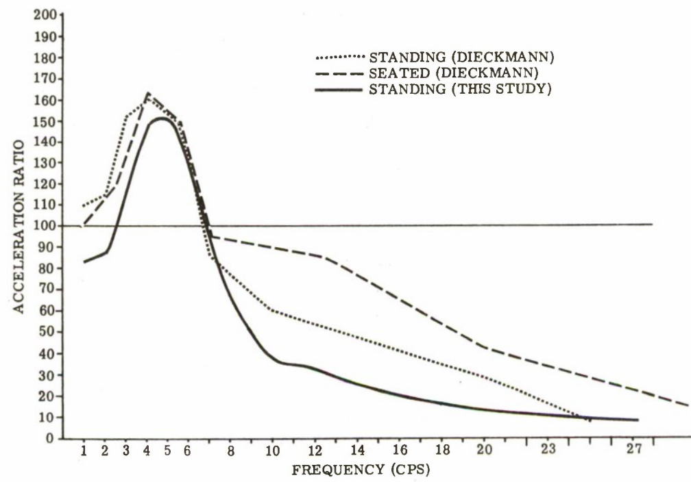
SHOULDER ACCELERATION EXPRESSED AS A PERCENTAGE OF TABLE ACCELERATION
