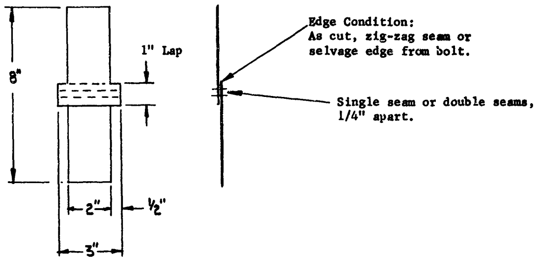
Lap Seams
