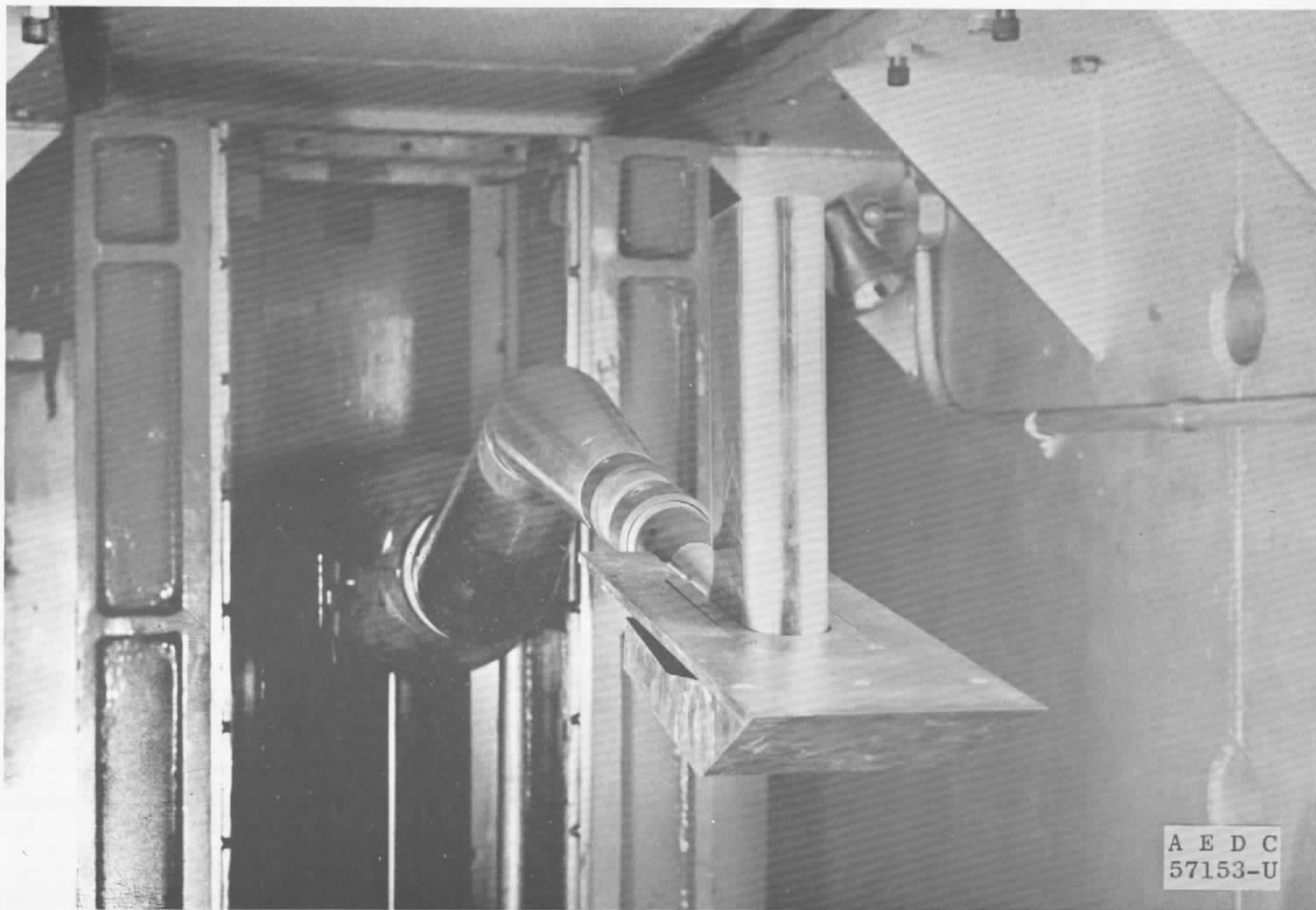
b. Shock Generator Model in Tunnel C, Retracted
