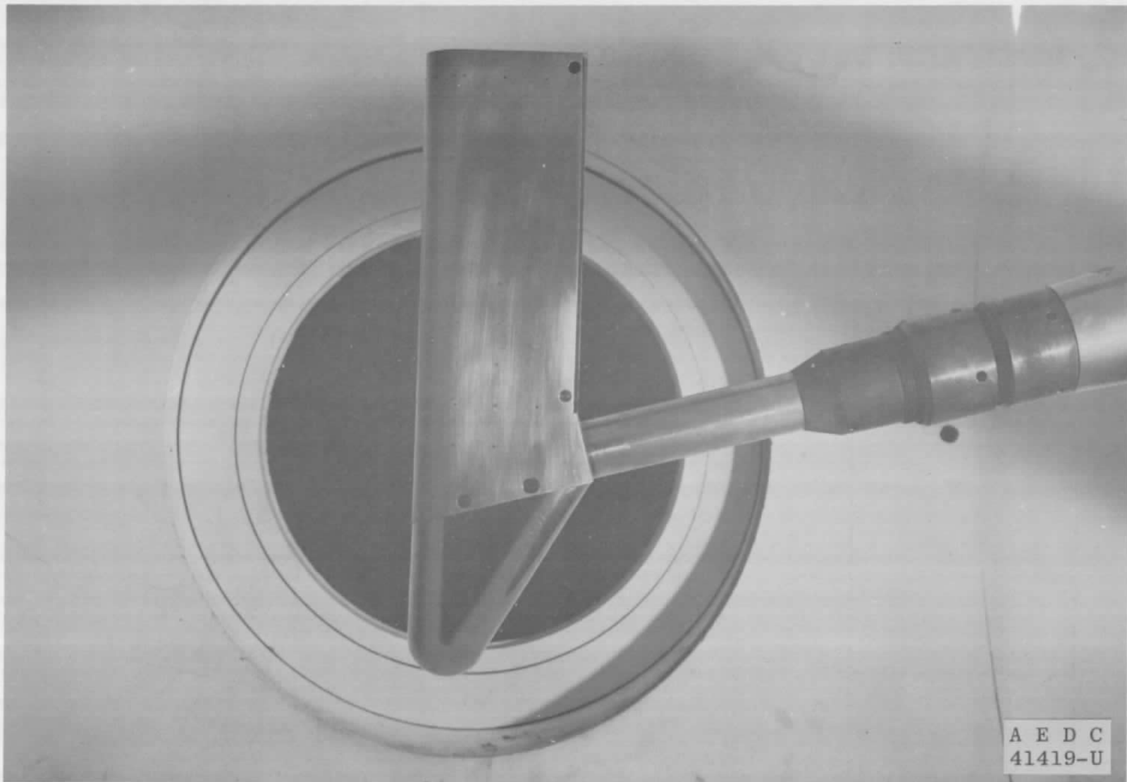
a. Blunt Nose Model in Tunnel B Fig. 3 Model Installation Photographs
