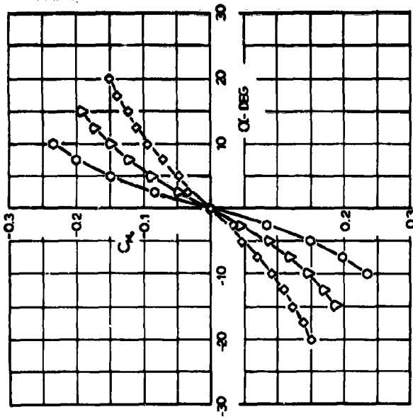
MOMENT COEFFICIENT
