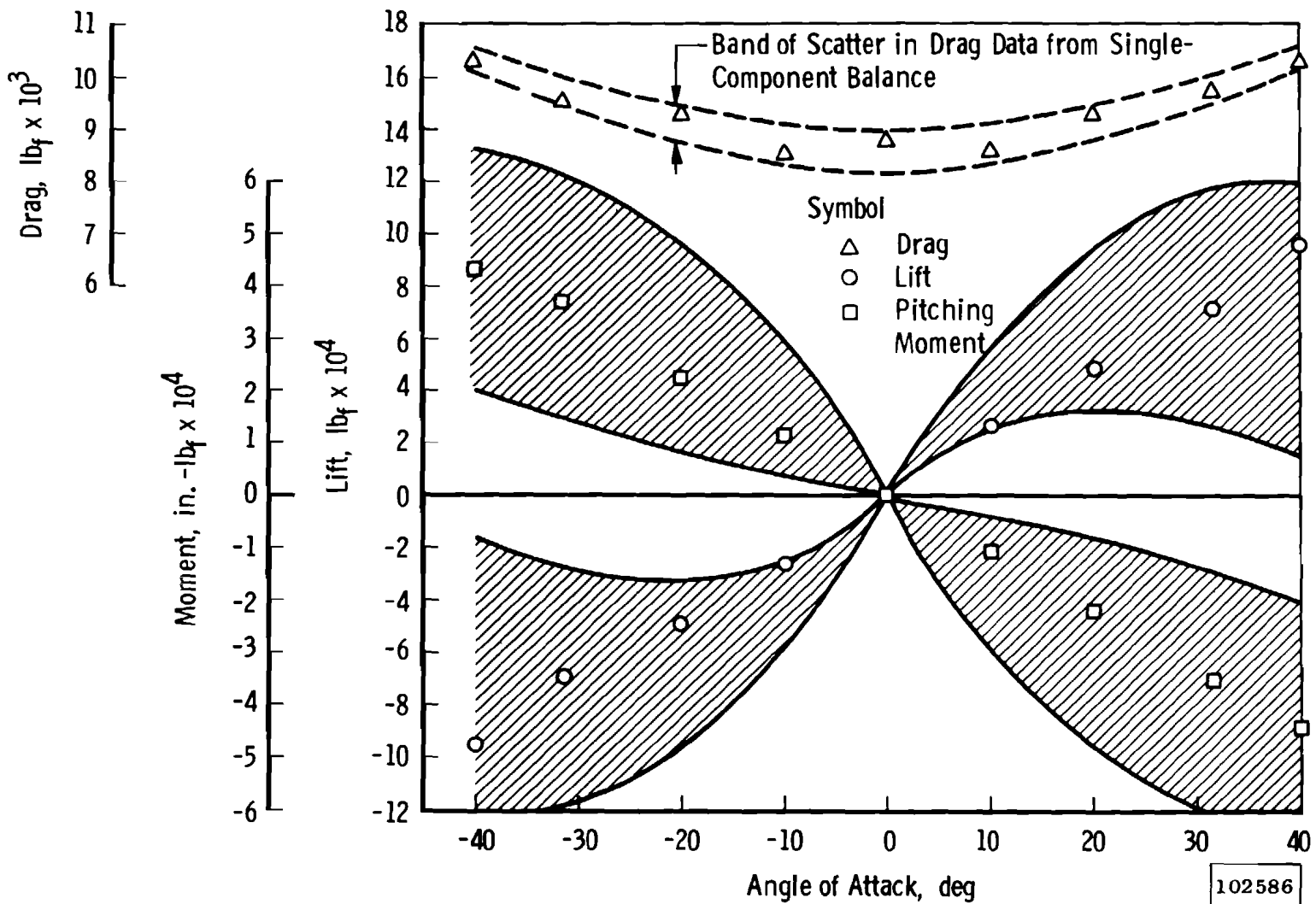
Fig. 11 Example Wind Tunnel Lift, Drag, and Pitching-Moment Measurements on Blunted Cone (Shaded Regions Lie between Extremes of Free-Molecular and Newtonian Theories for Lift and Moment)
