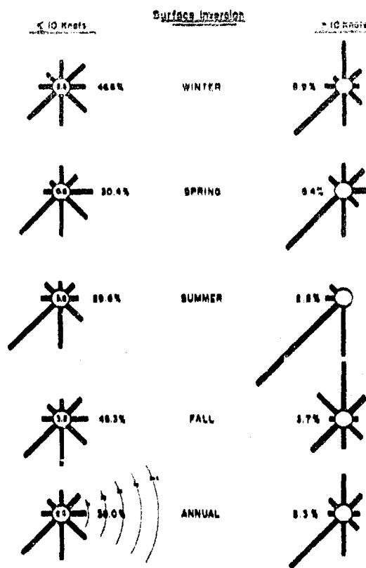
Figure 3.20. Annual and Seasonal Wind Directions During Surface-based Inversions at Norfolk (ORF). Wind Speeds: \leq 10 knots, and > 10 knots.
