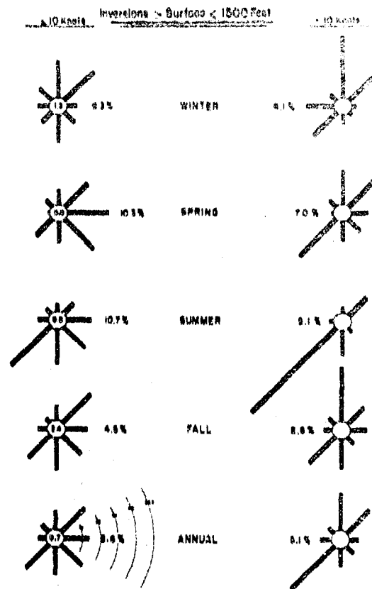
Figure 3.21. Annual and Seasonal Wind Directions During Inversions between the Surface and 1,500 feet at Norfolk (ORF). Wind Speeds: \leq 10 knots and > 10 knots.
