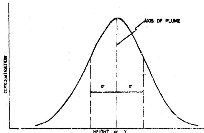
Figure 1.5. Normal Distribution of Air Pollution.
