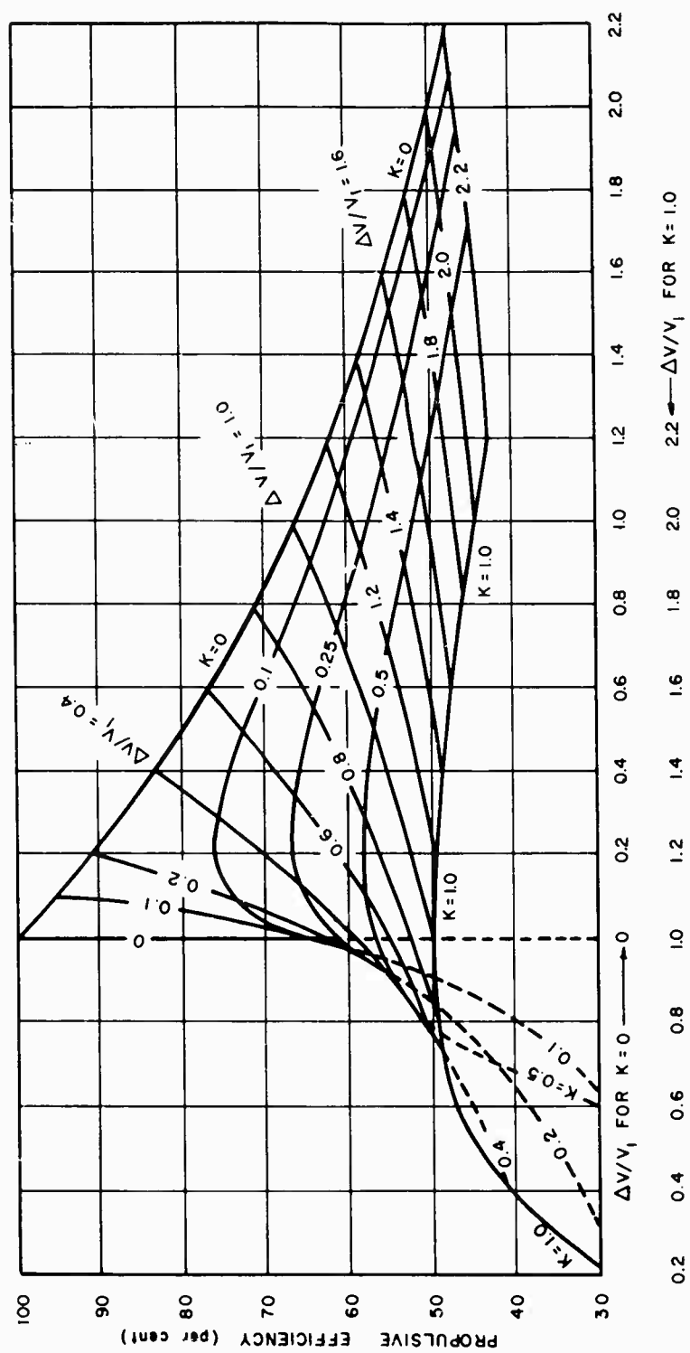
Fig. 5 - Propulsive Efficiency of a Pumpjet for Several Values of Duct-Loss Coefficient
