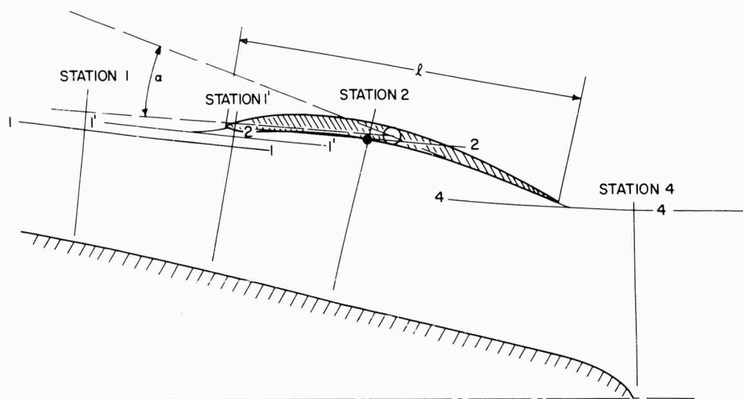
Fig. 16 - Pumpjet Shroud on Tapered Afterbody
