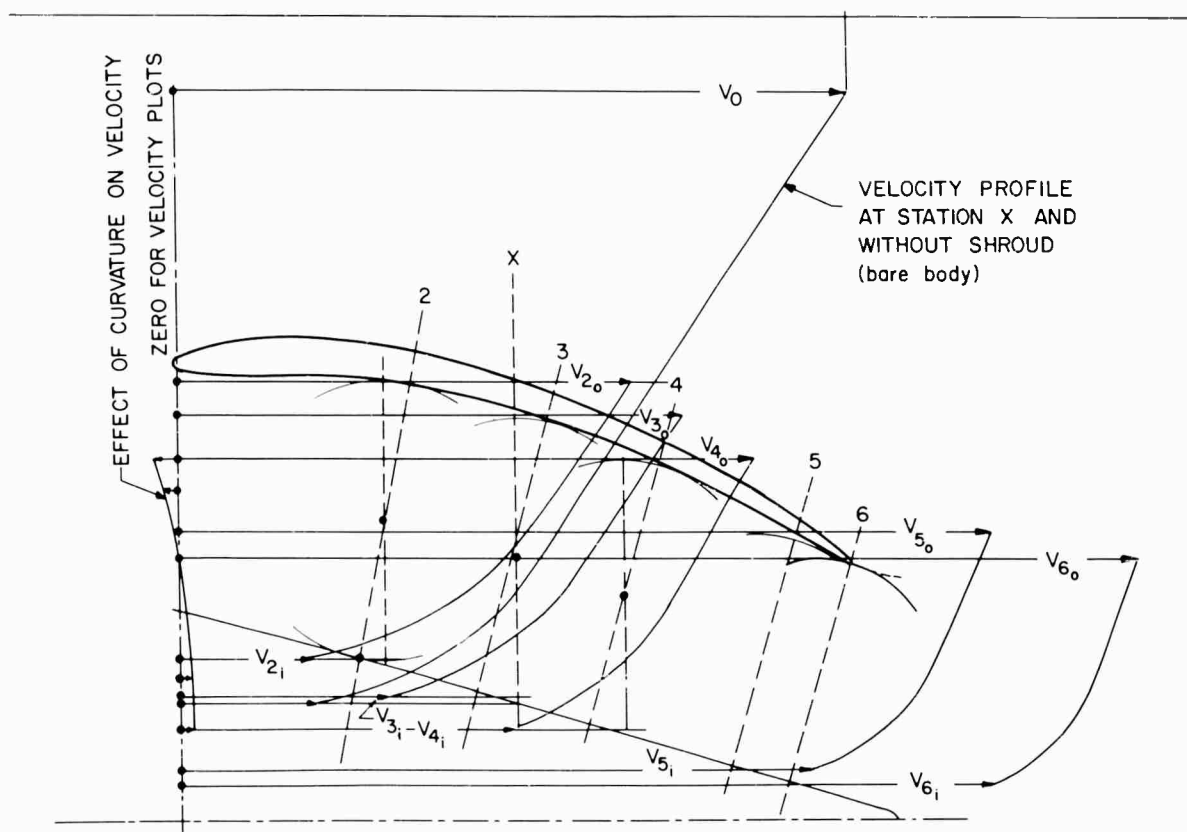
Fig. 17 - Velocity Distribution within a Shroud on a Tapered Afterbody
