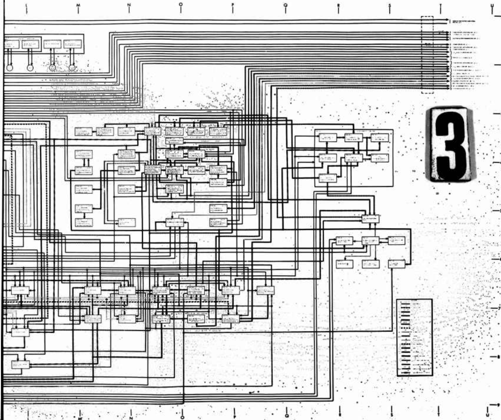
Figure A-1. Functional Flow Diagram of Atlas F Weapon System Operational Ground Equipment
