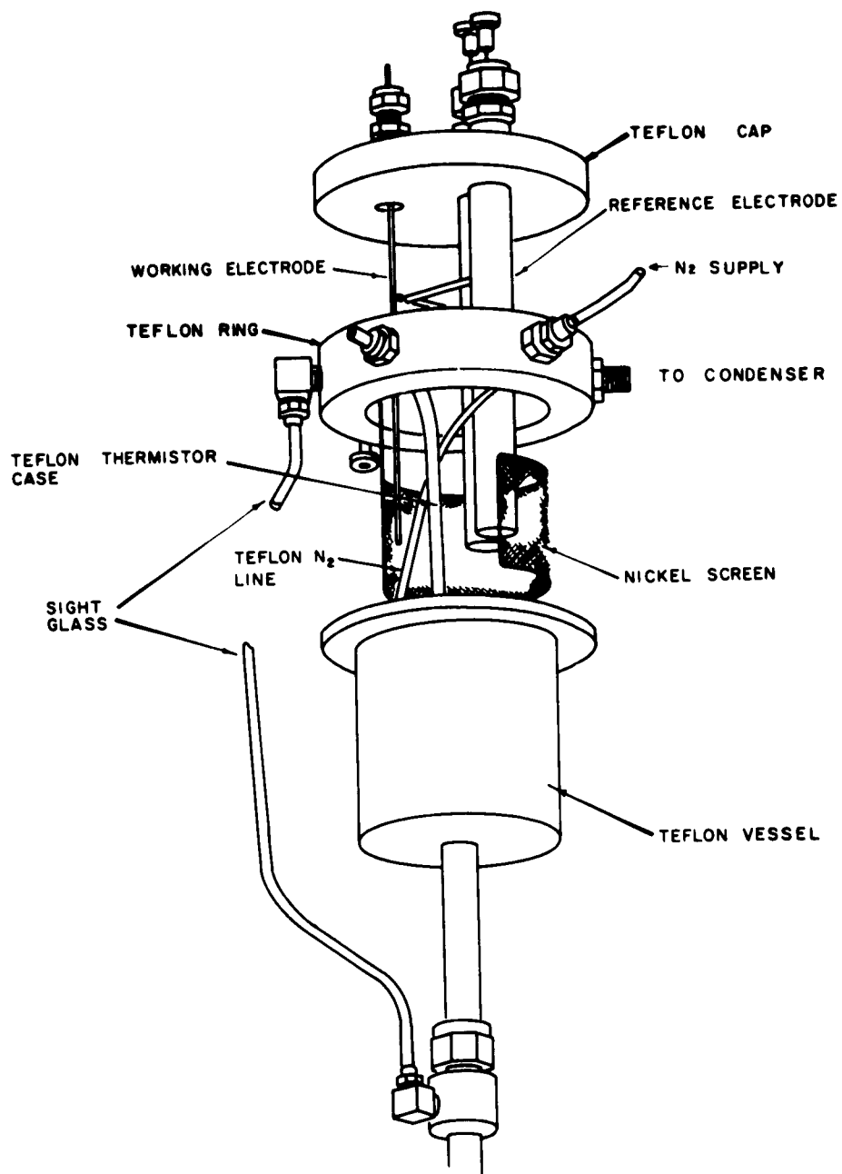
Fig. 3 -ELECTROLYTIC CELL
