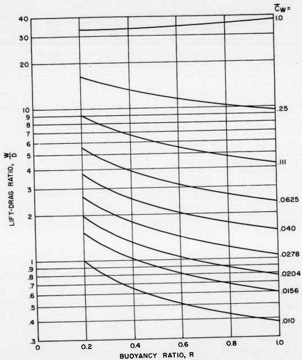
FIGURE 6-LIFT-DRAGE RATIO Vs BUOYANCY RATIO Rev = 6 \times 10^6 , s^2 Z = 33
