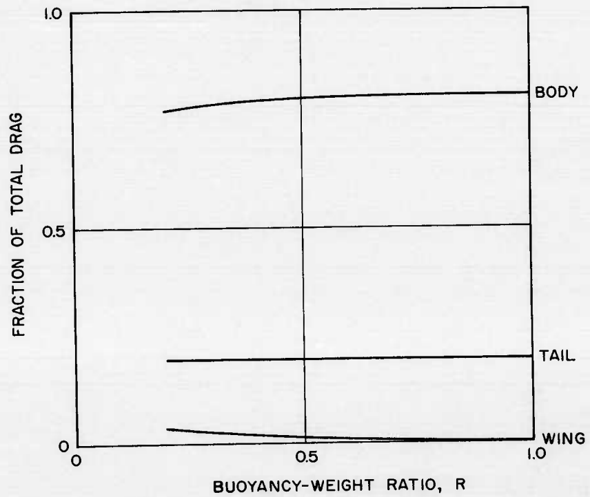
FIGURE 4-DRAG BREAK-DOWN FOR \bar{C}_w = 0.010 Re_v = 12 \times 10^7 , s'z = 0.7 (OPTIMUM BODY)
