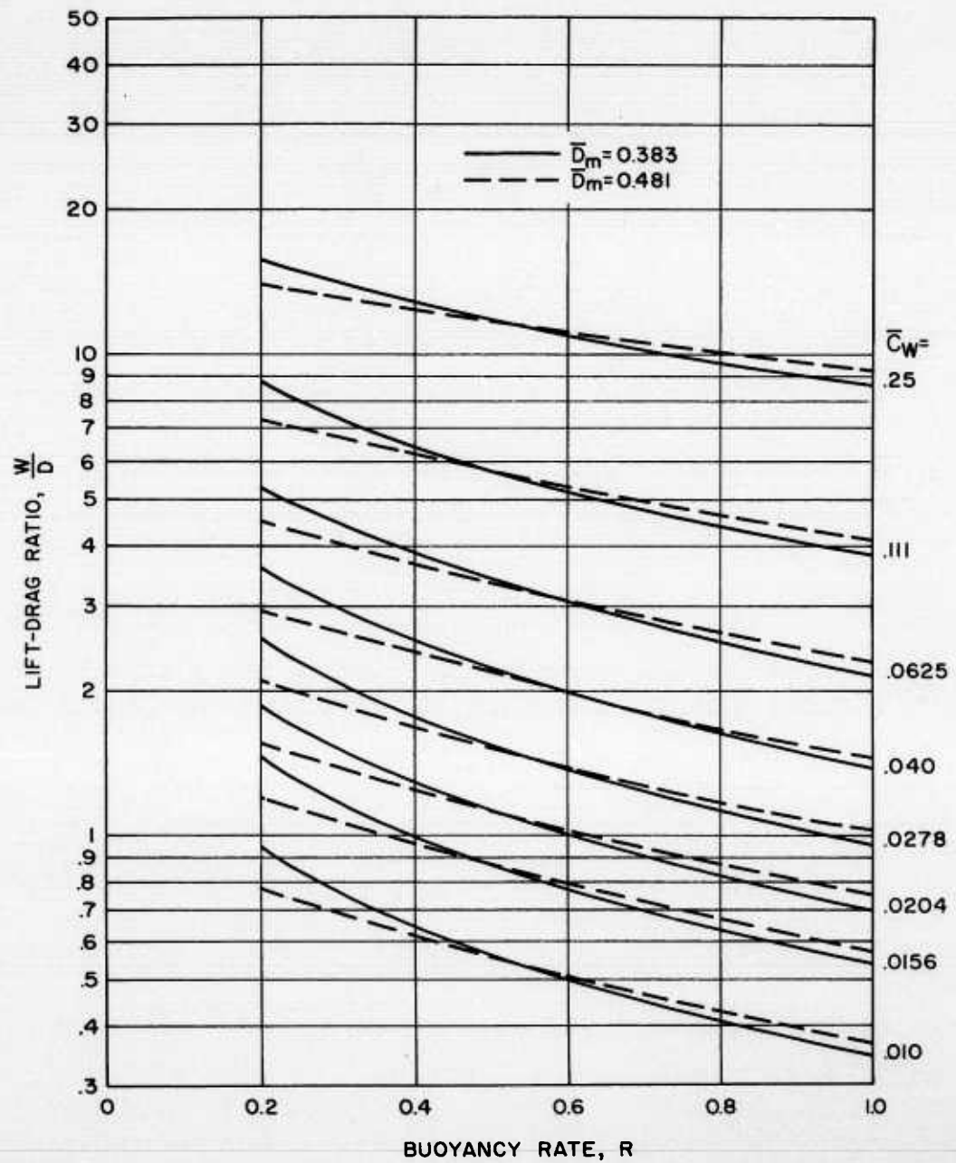
FIGURE 7-EFFECT OF \bar{D}_m ON LIFT-DRAGE RATIO Rev = 6 \times 10^6 , s^*Z = 33
