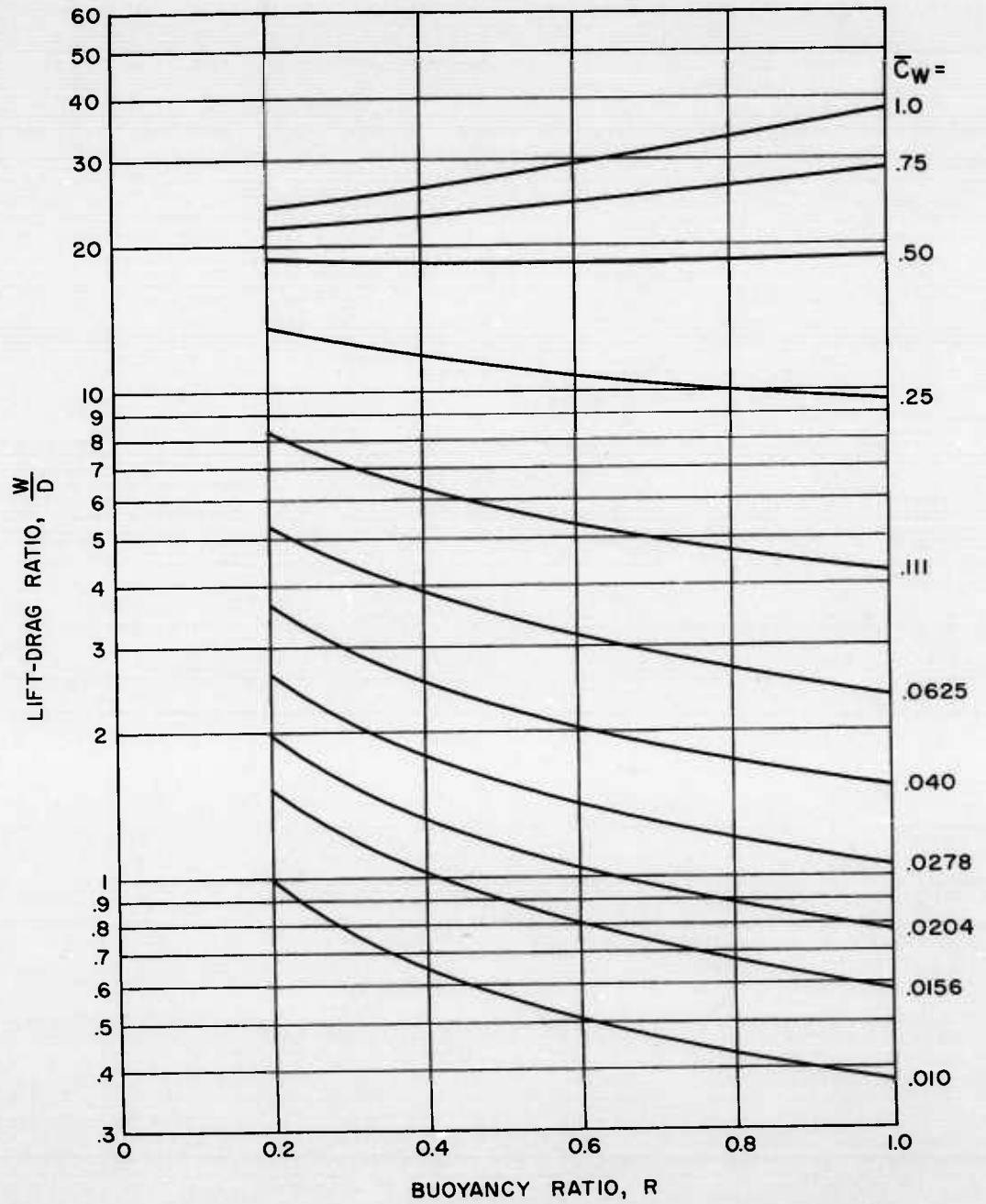
FIGURE 5-LIFT-DRAGE RATIO Vs BUOYANCY RATIO. (OPTIMUM BODY ONLY) Re_v = 6 \times 10^6 , s^*z = 0.7
