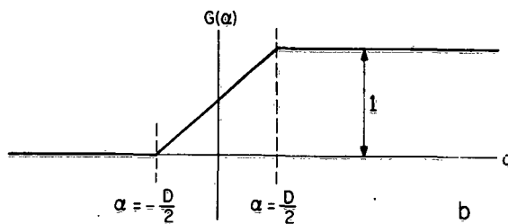
FIGURE 1b, c. The linear surface impedance variation.
