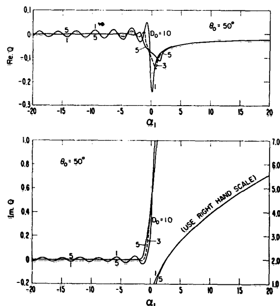
FIGURE 5. The real and the imaginary parts of Q as a function of \alpha_1 or KC_1 d_1 where d_1 is the distance from the coastline.
