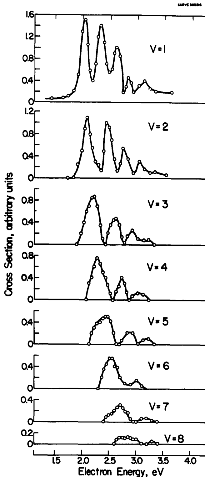
Figure 4 Energy dependence of the vibrational cross section of nitrogen by electron impact. The curves are obtained from sets of curves similar to Fig. 3 taken at different energies of the incident electrons. When the ordinate numbers are multiplied by 10^{-16} a cross section scale (in \text{cm}^2 ) is obtained such as to give a total vibrational cross section in agreement with Haas. See text for a discussion of errors in cross section scale.
