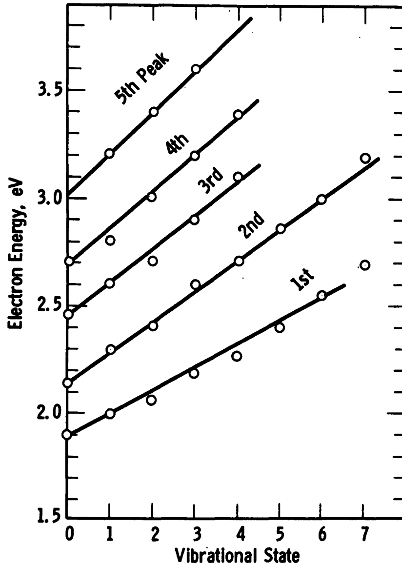
Fig. 7. Position of the cross section peaks on the energy scale vs quantum number of the final state. On a simply long-life model of the compound state, all solid lines should be horizontal, e.g., the first peak should occur at the same energy, regardless of the final vibrational state.
