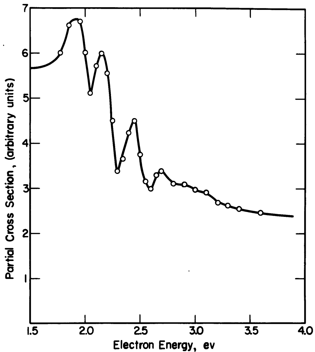
Figure 5 Elastic scattering of electrons in N_2 at 72 degrees vs electron energy in the energy range of the compound state.
