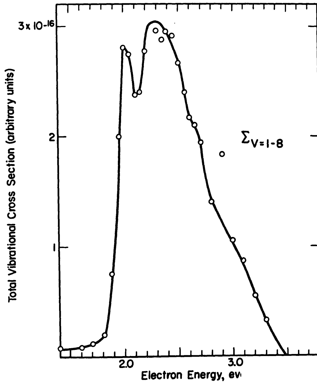
Fig. 6. Sum of the vibrational cross sections to individual states vs electron energy in N_2 .
