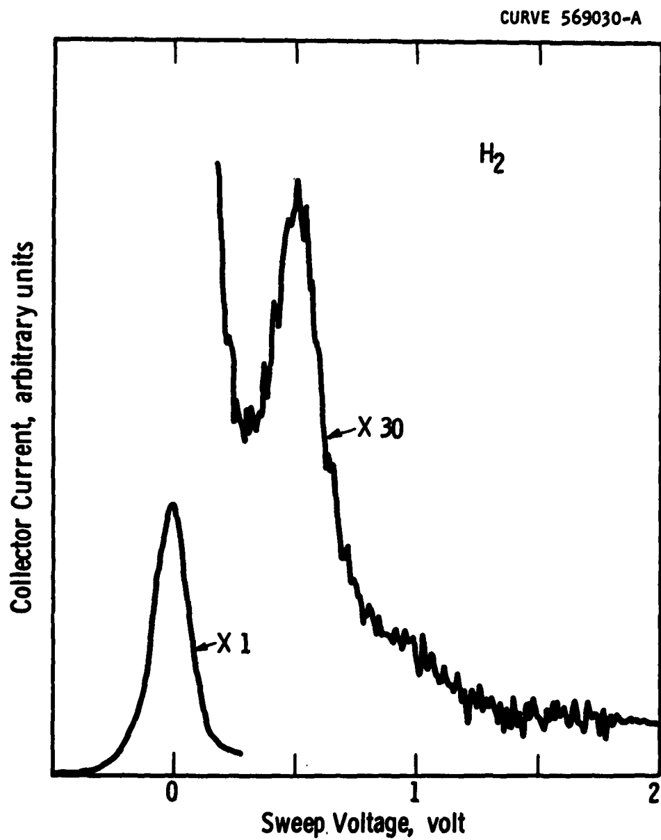
Fig. 10. Energy spectrum of scattered electrons in H 2 . The curve is obtained in the same manner as Fig. 3.
