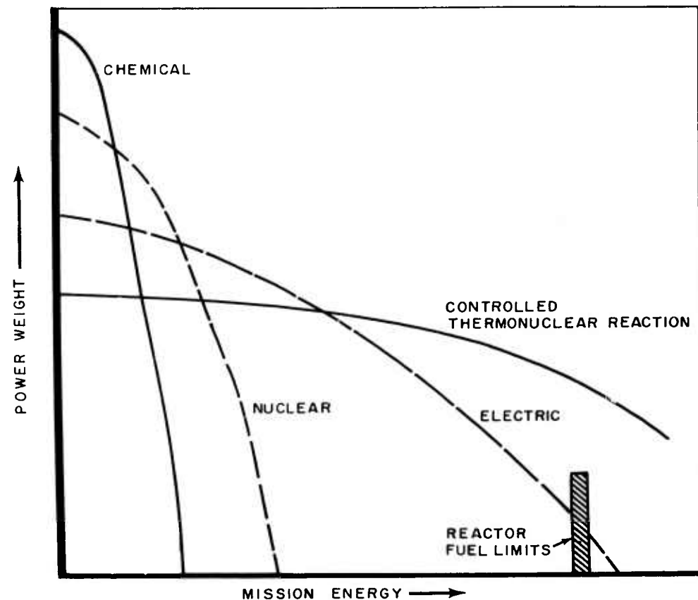
Figure 8. Space Propulsion Mission Capabilities
