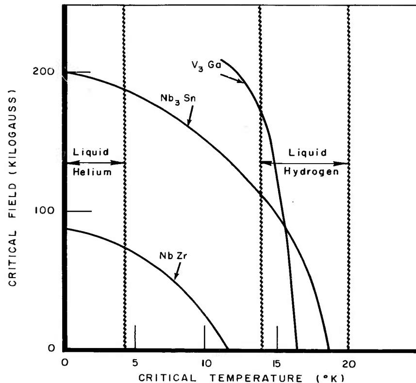
Figure 5. Superconductive Properties
