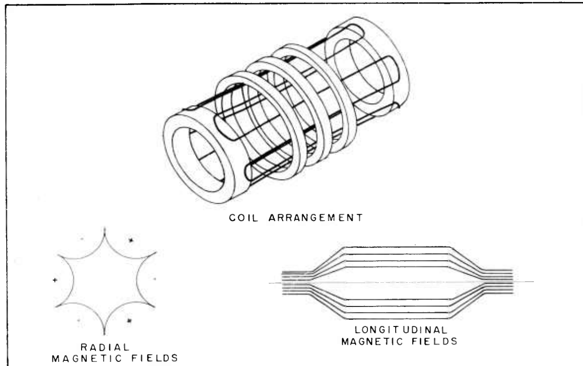
Figure 4. Multipolar Magnetic Confinement Geometry
