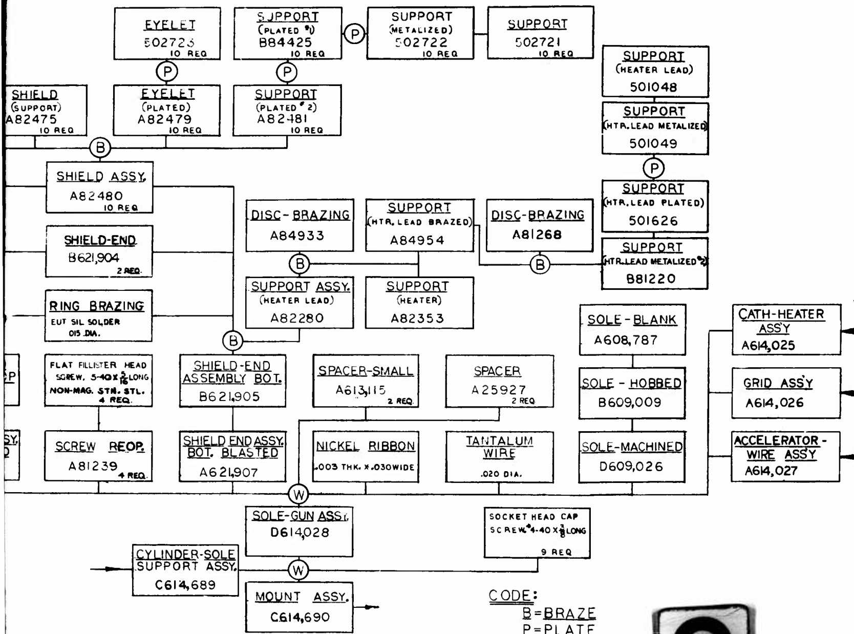
FLOW CHART MOUNT ASSEMBLY QKA 851
