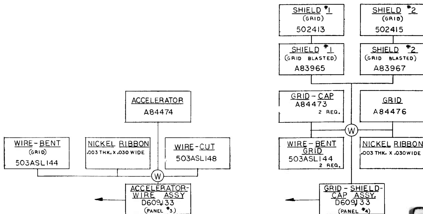
FLOW CHART GUN ASSEMBLY QKA 852
