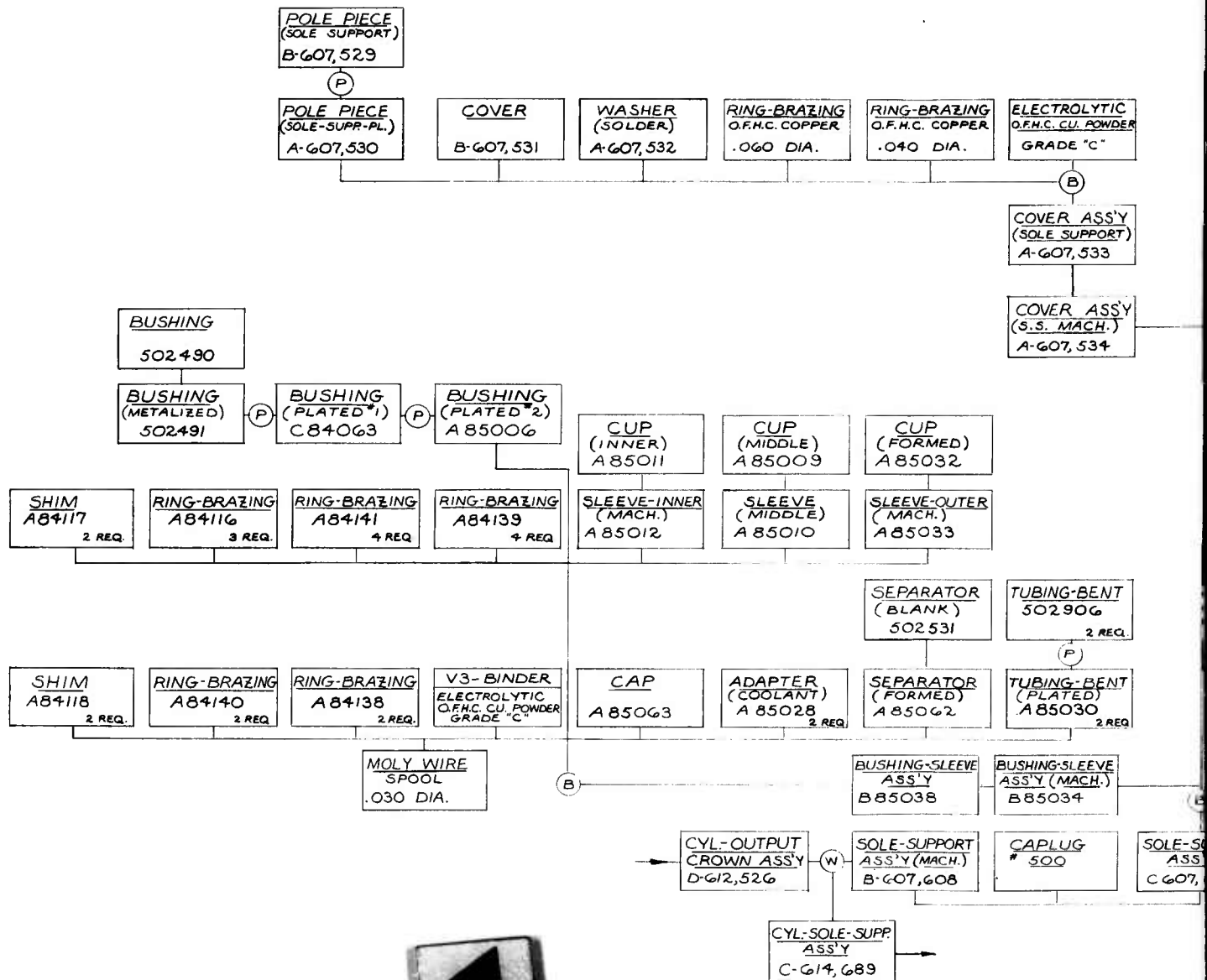
FLOW CHART (CYL. SOLE SUPPORT ASS'Y) QK851
