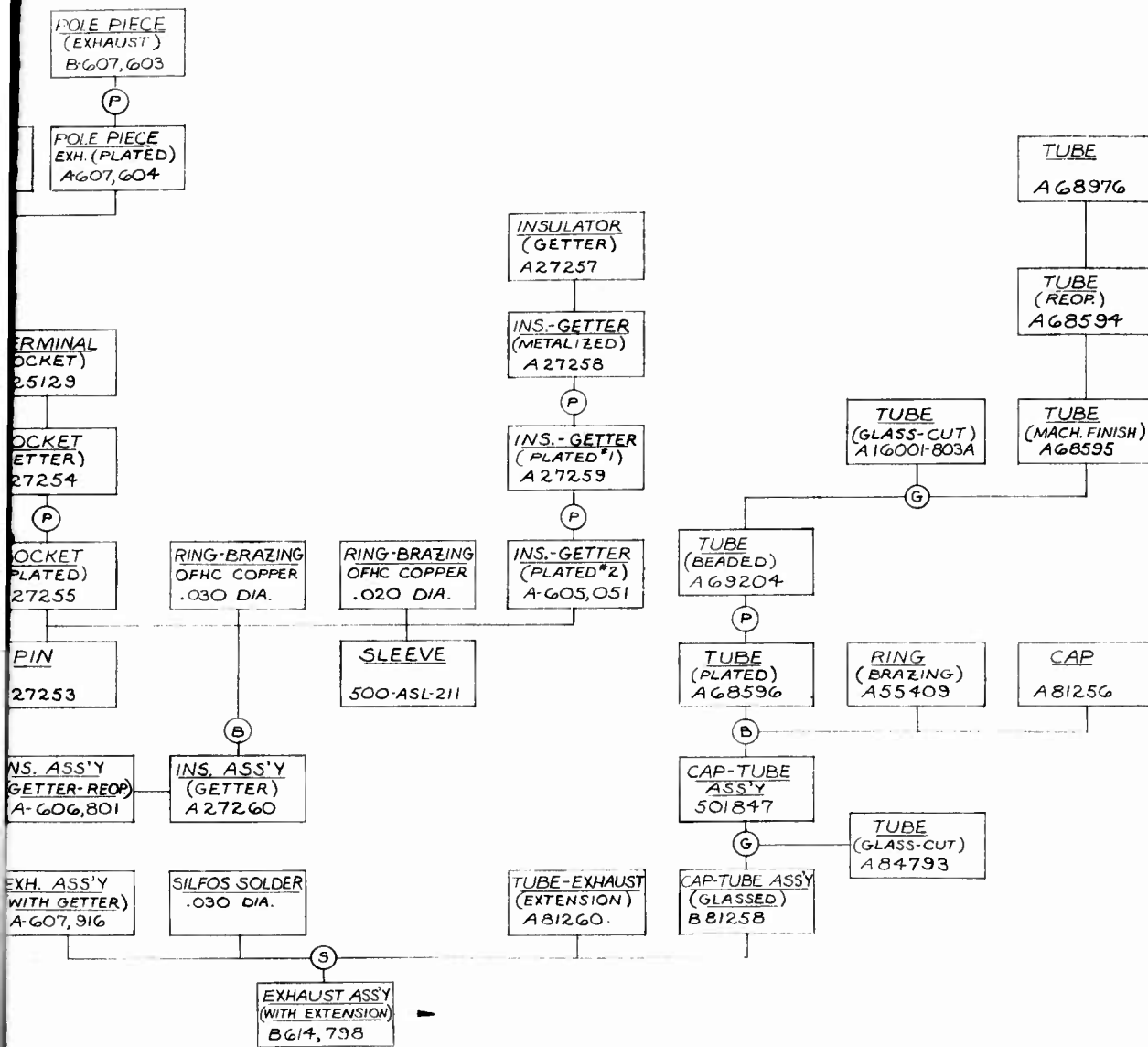
FLOW CHART (EXHAUST ASSY (WITH EXTENSION)) QKA 851
