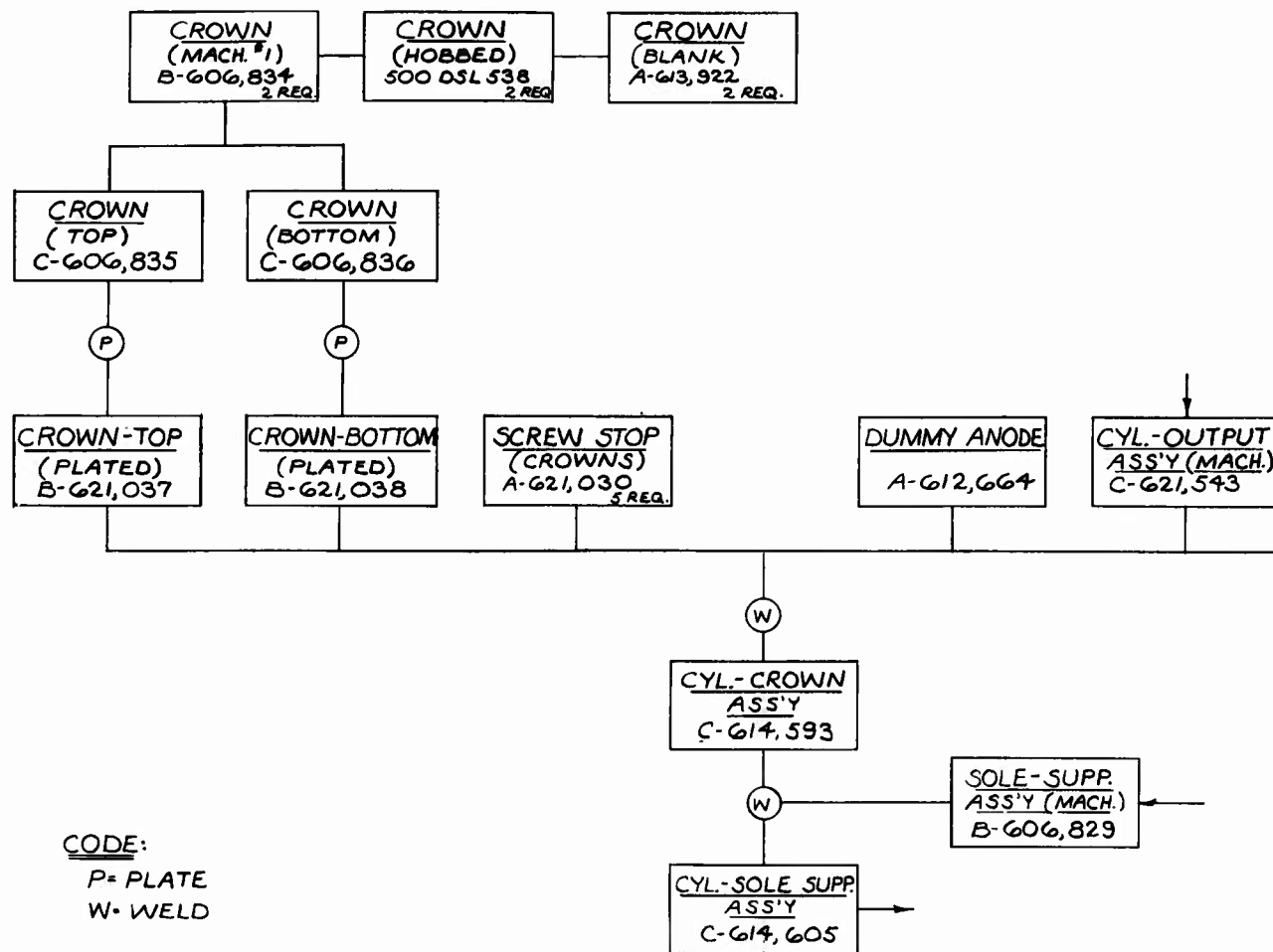
FLOW CHART CYL. SOLE SUPPORT ASS'Y QKAB55
