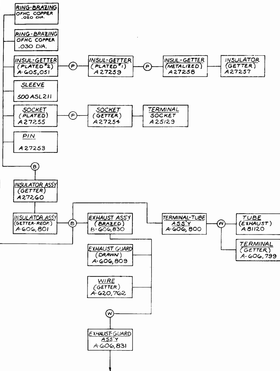
FLOW CHART EXHAUST-GUARD ASS'Y QKA855
