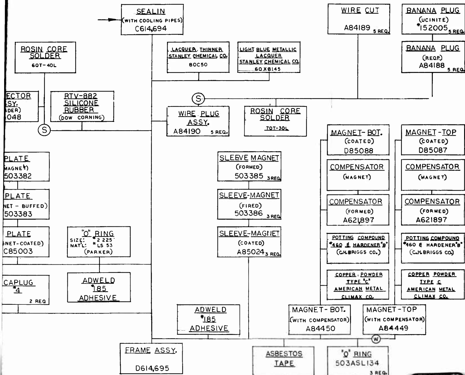
FLOW CHART FRAME ASSEMBLY QKA 851
