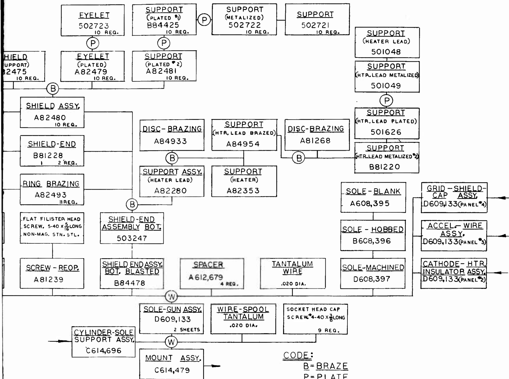
FLOW CHART MOUNT ASSEMBLY QKA 852
