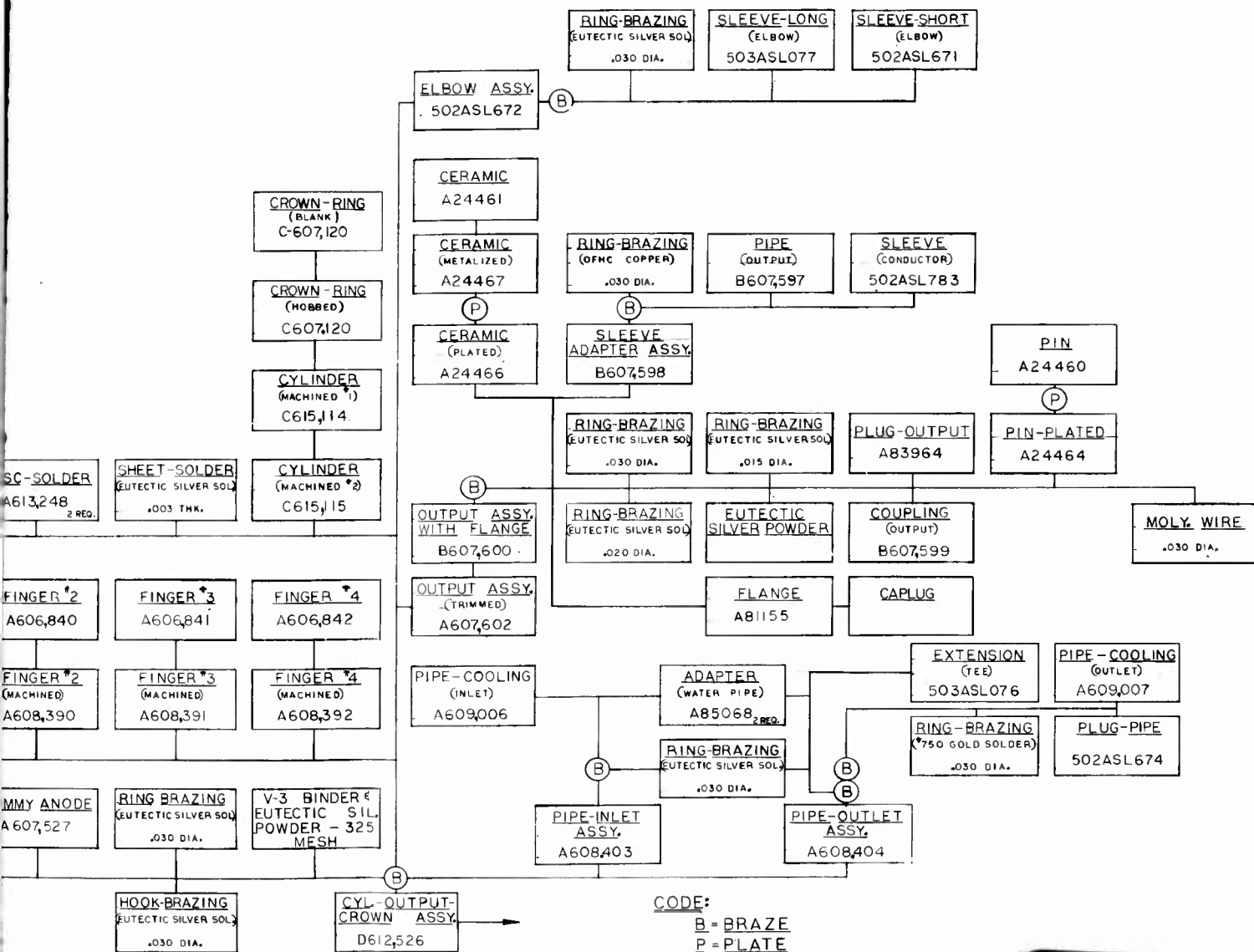
FLOW CHART CYLINDER OUTPUT CROWN ASSY.
