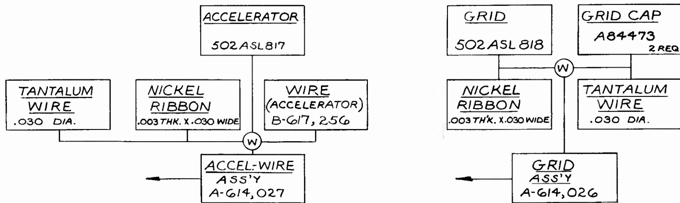
FLOW CHART GUN ASS'Y QKA851
