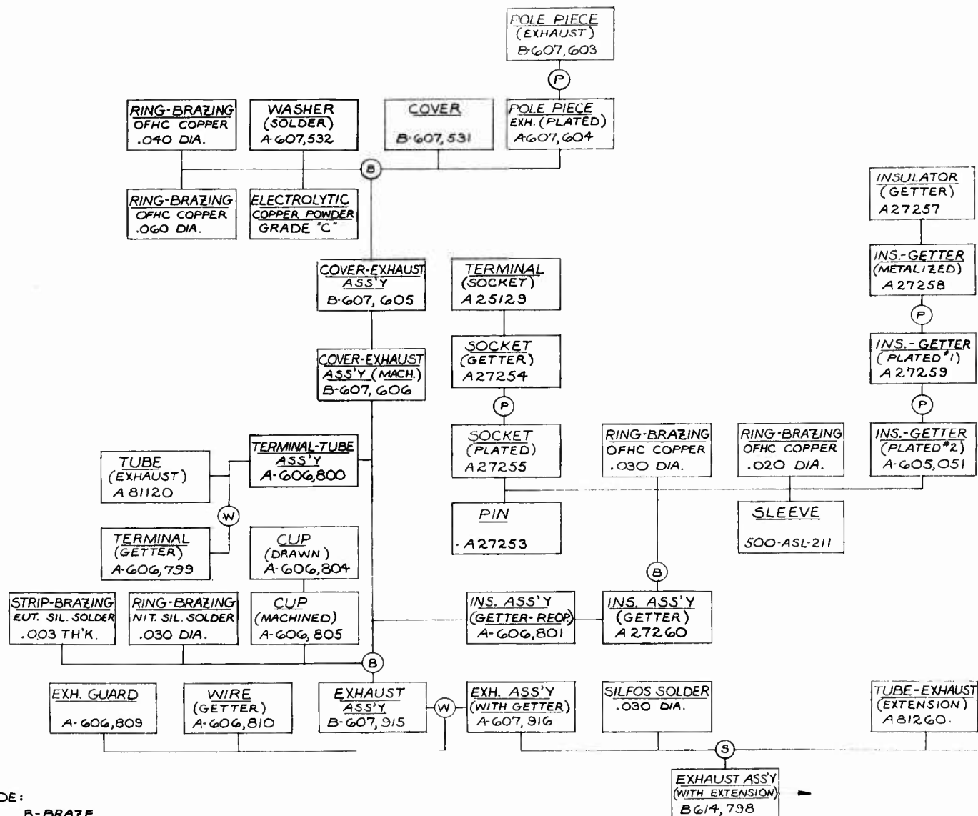
FLOW CHART (EXHAUST ASS'Y (WITH EXTENSION)) QKA 851
