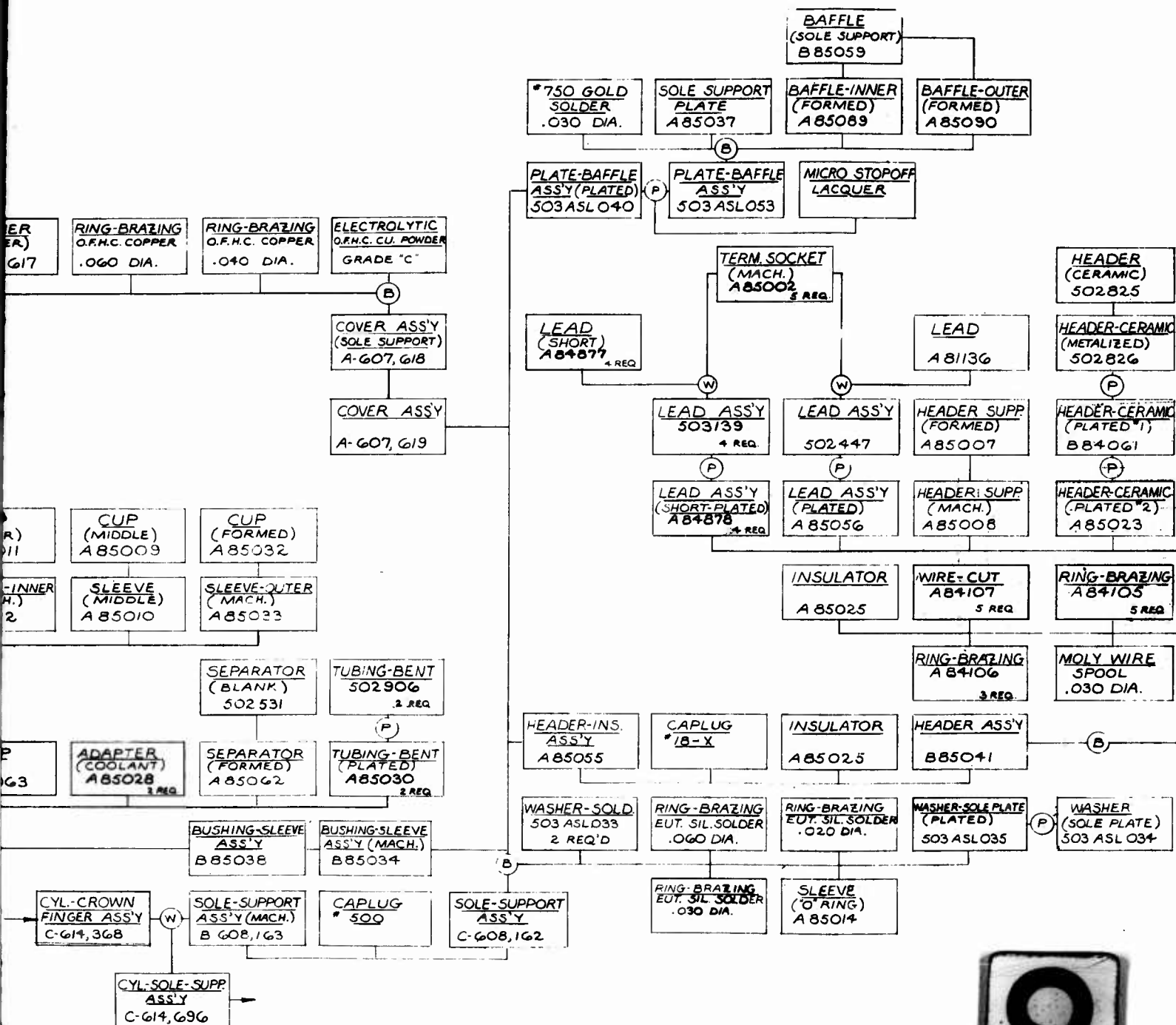
FLOW CHART CYL-SOLE SUPPORT ASS'Y QK852
