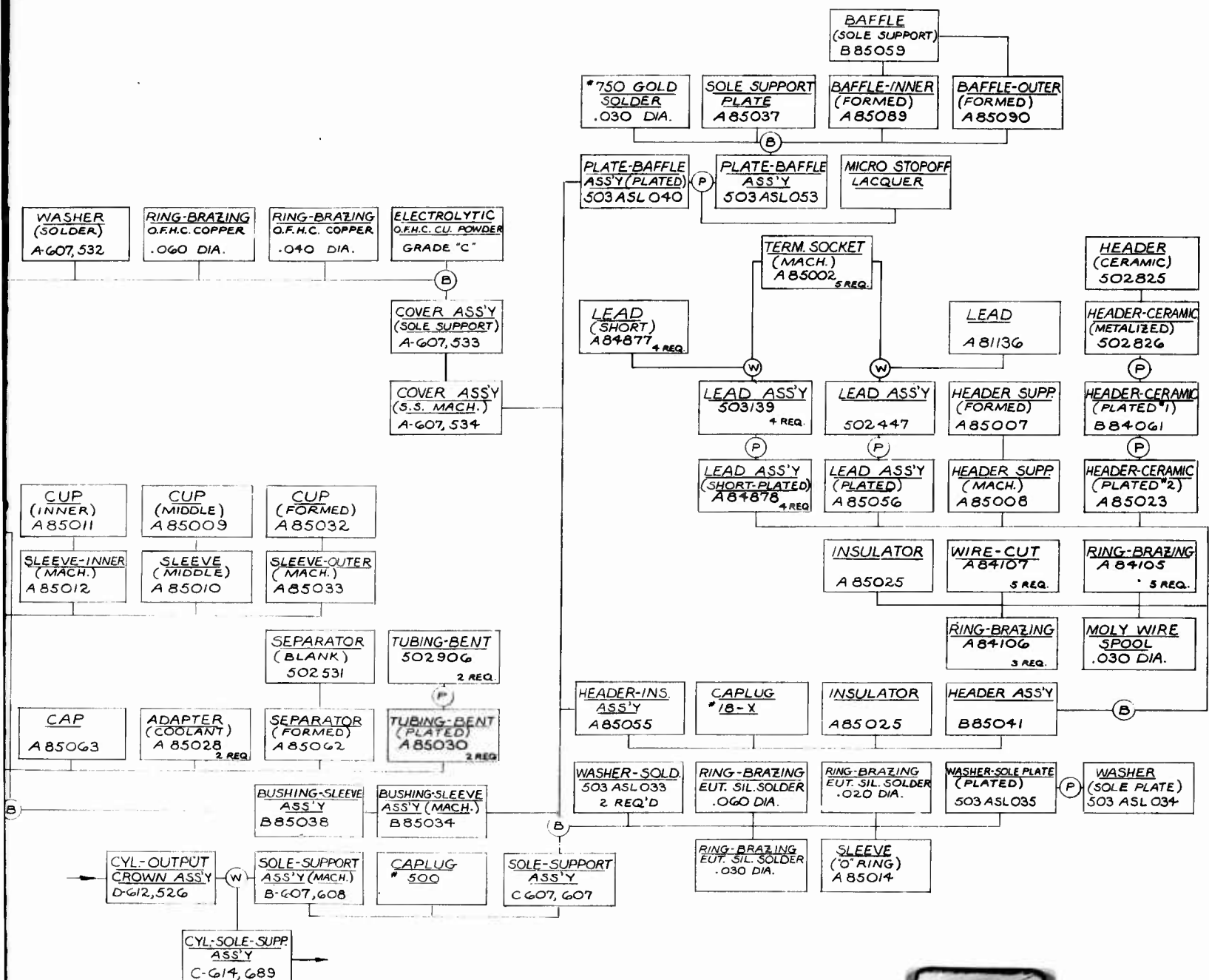
FLOW CHART (CYL. SOLE SUPPORT ASS'Y) QK851
