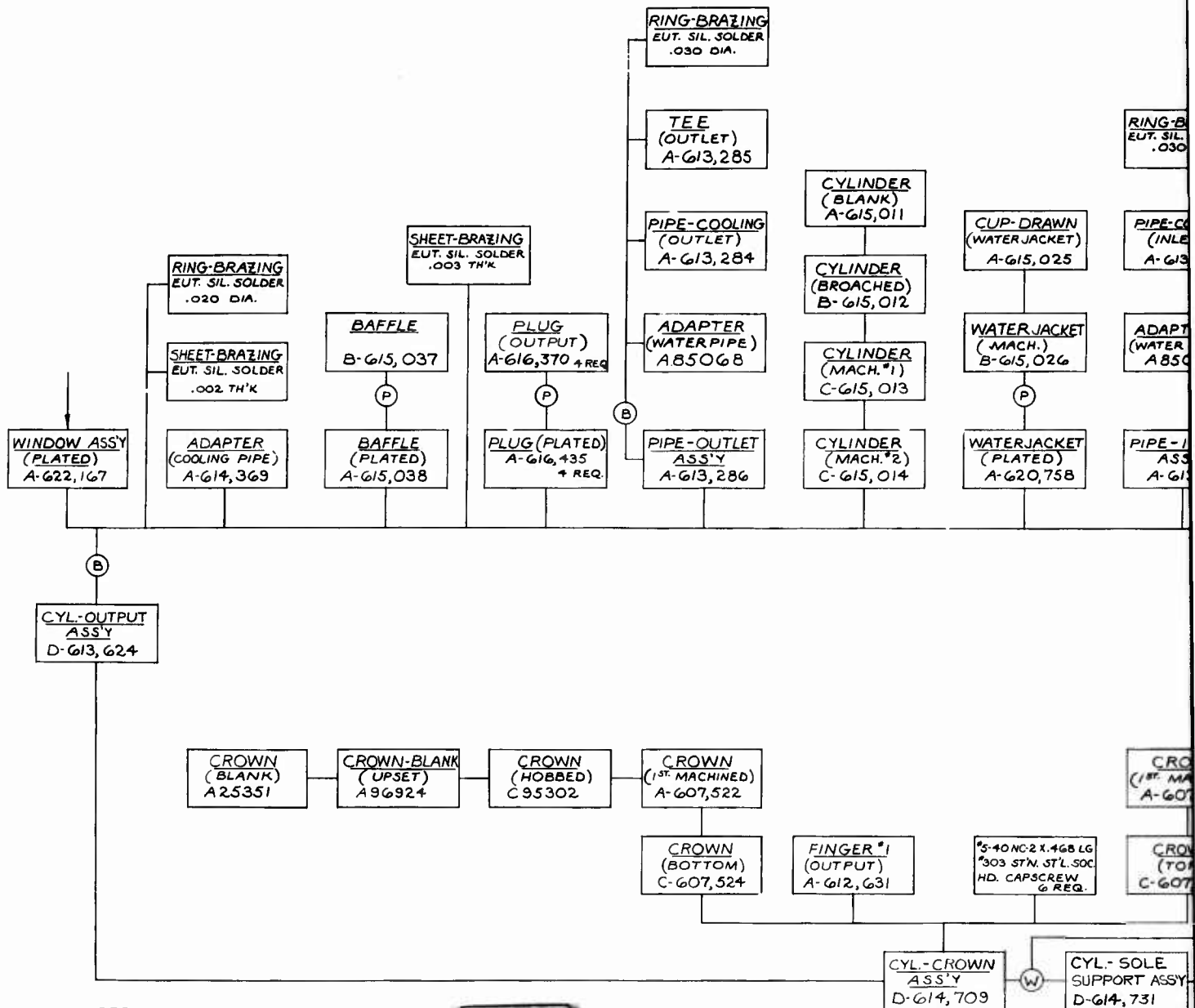
FLOW CHART CYL.-SOLE SUPPORT ASS'Y QKA 857
