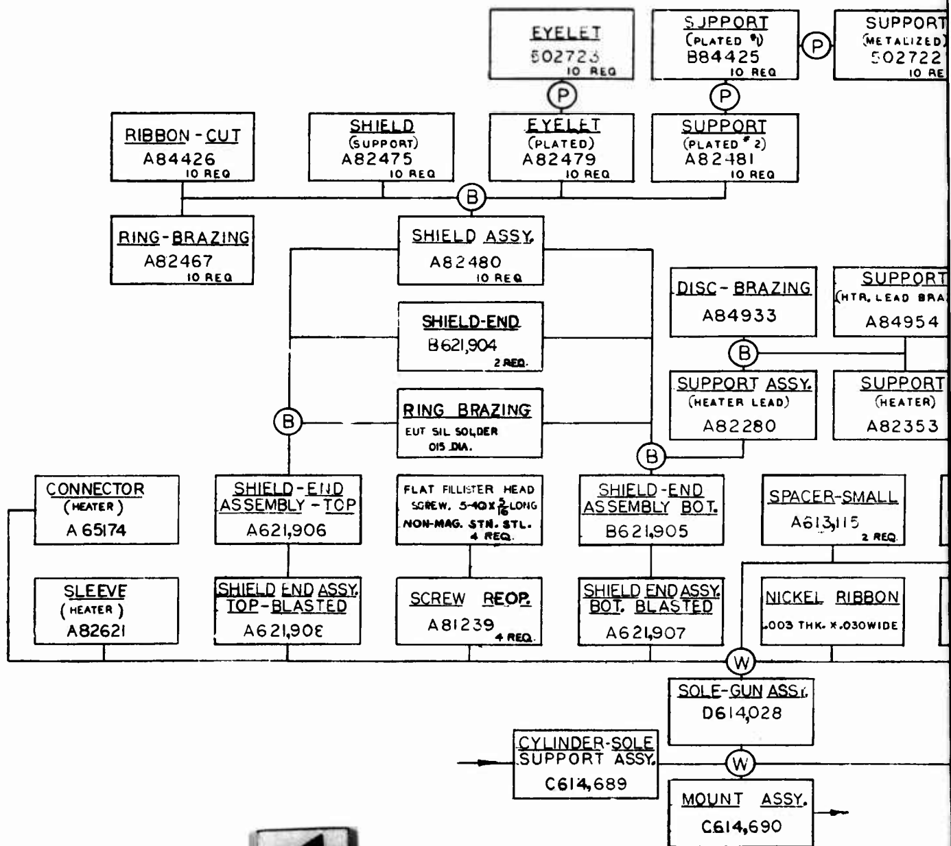
FLOW CHART MOUNT ASSEMBLY QKA 851
