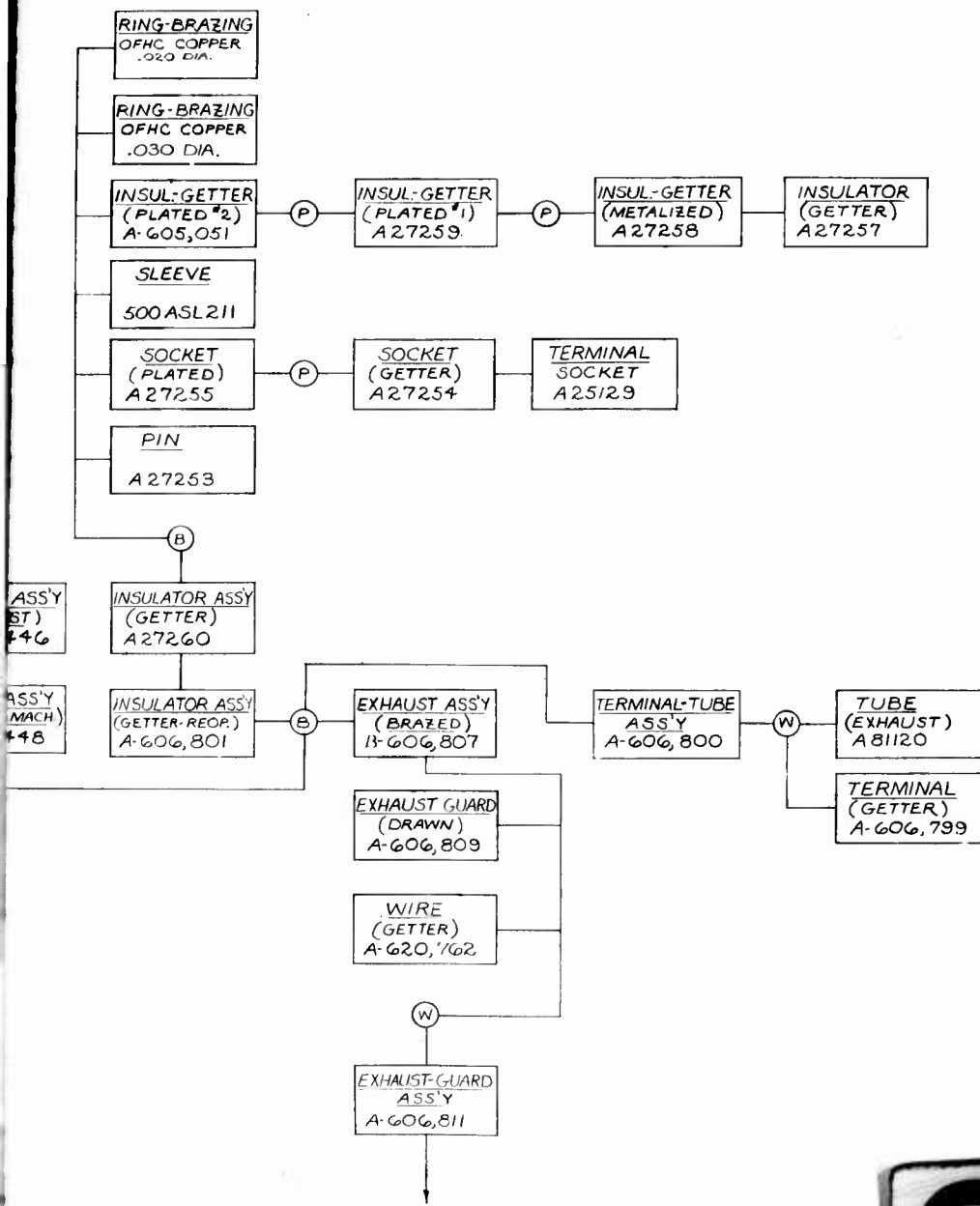
FLOW CHART EXHAUST-GUARD ASS'Y QKA857
