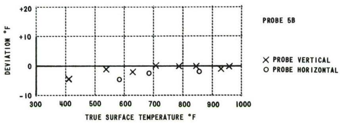
Figure 27 ORIENTATION TESTS ON ALUMINUM
