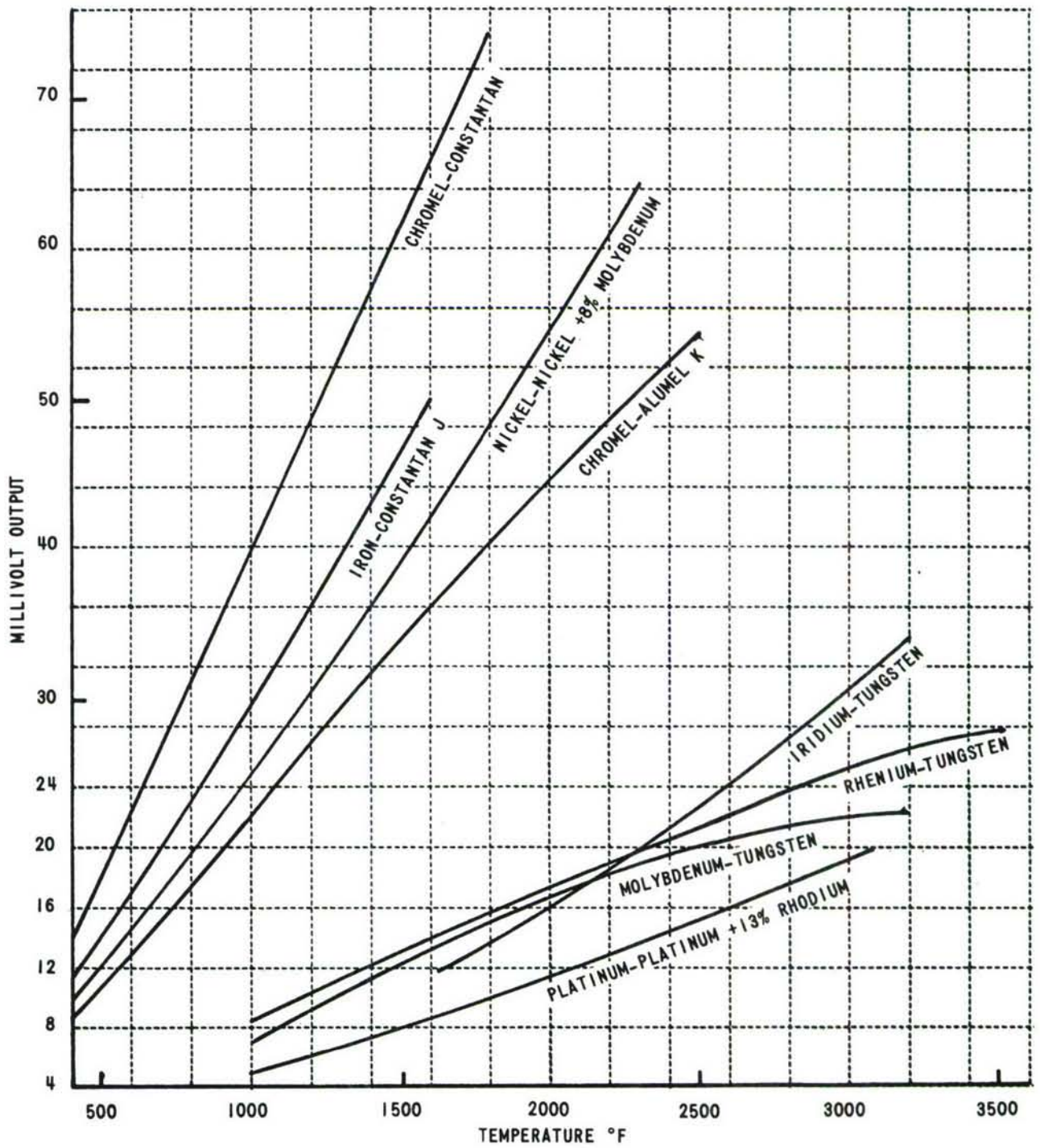
Figure 44 OUTPUT OF VARIOUS THERMOCOUPLES
