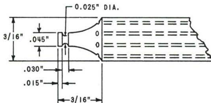
Figure 57 SENSOR SUPPORT
