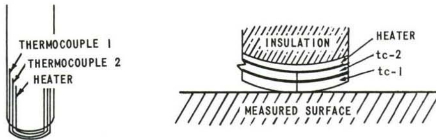
Figure 1 TEMPERATURE SENSOR
