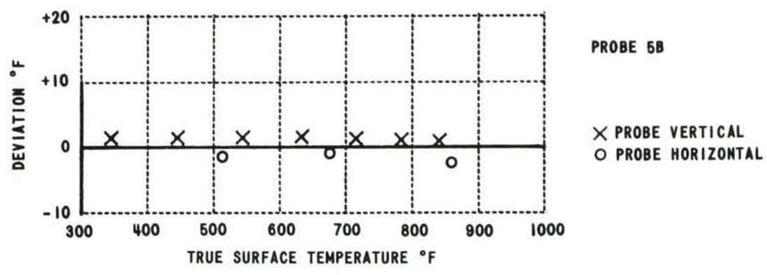
Figure 28 ORIENTATION TESTS ON HOT ROLLED STEEL
