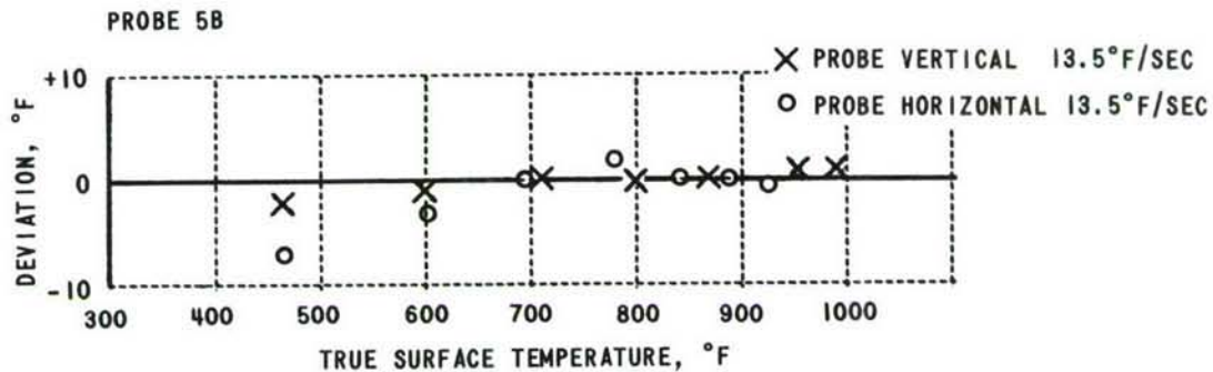
Figure 29 ORIENTATION TESTS ON STAINLESS STEEL
