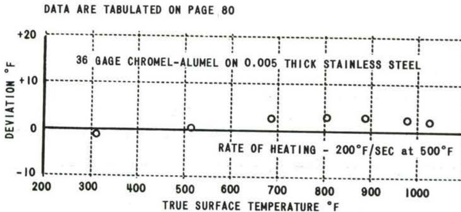
Figure 38 TRANSIENT TEST ON STAINLESS STEEL
