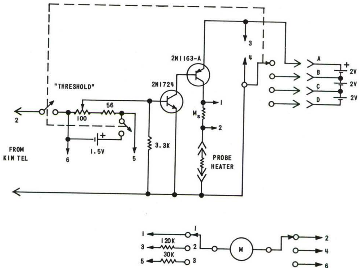
Figure 6 POWER AMPLIFIER
