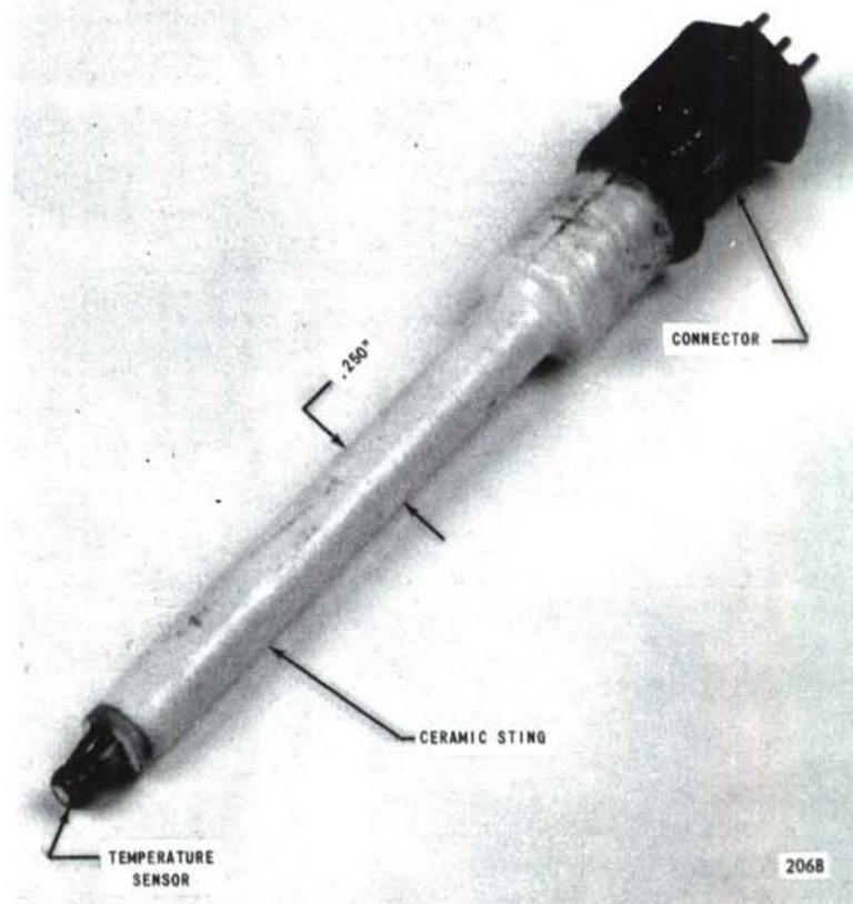
Figure 50 SURFACE TEMPERATURE PROBE MODEL I
