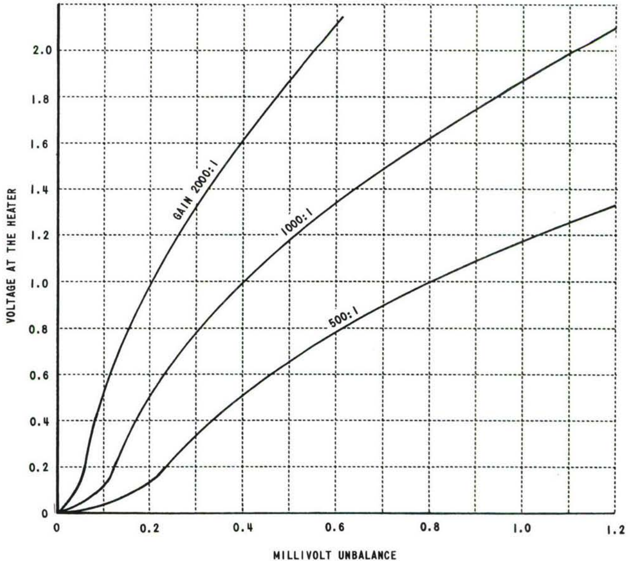
Figure 47 VOLTAGE CHARACTERISTICS OF THE CONTROLLER
