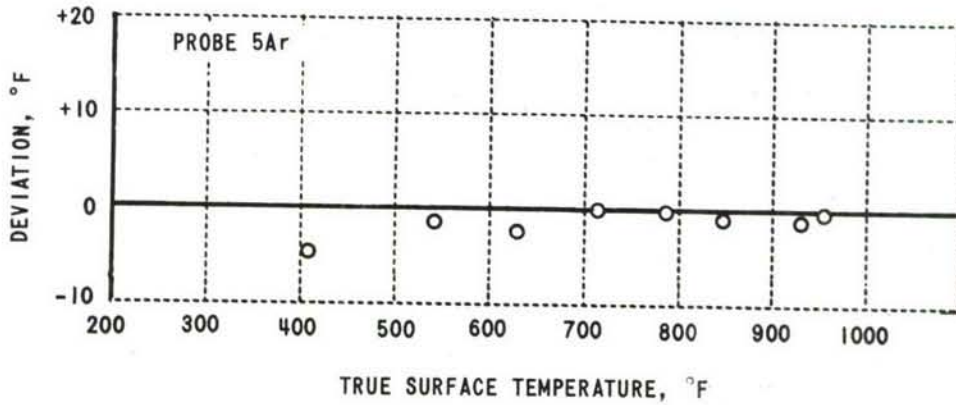
Figure 9 TRANSIENT TESTS ON ALUMINUM
