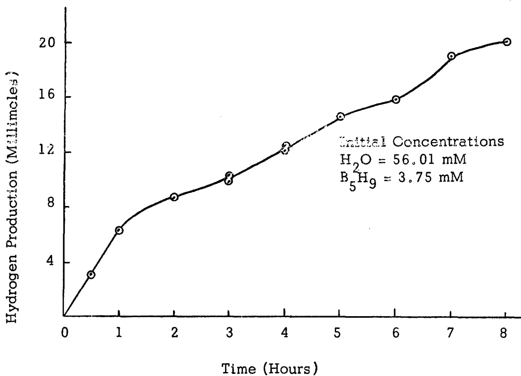
Figure 6. Plot of Hydrogen Production of Stoichiometric Pentaborane Hydrolysis Reaction at 150^\circ\text{C} .
