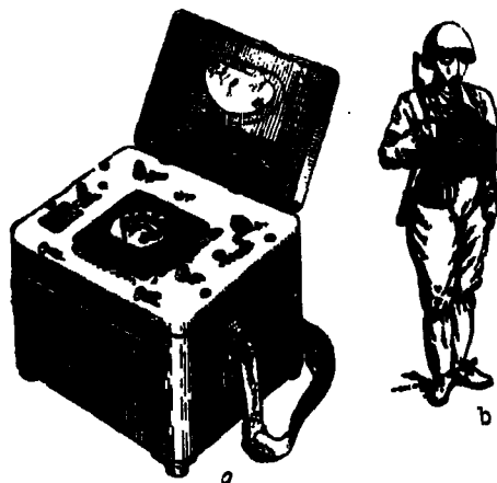
Fig. 14. General view of radiometer (a) and its use for measuring the contamination of an object (b).
