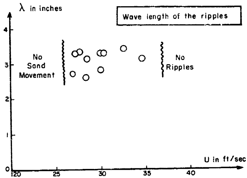
FIGURE 22 - WAVE LENGTH OF THE RIPPLES
