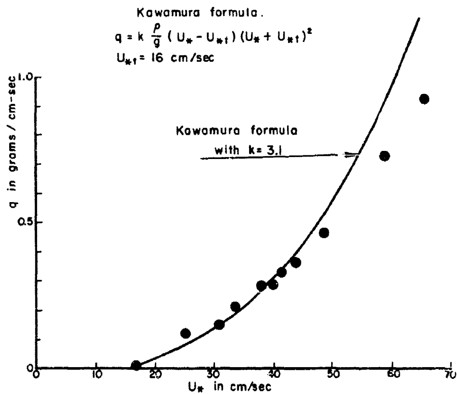
FIGURE 5-COMPARISON BETWEEN EXPERIMENTAL RESULTS AND KAWAMURA FORMULA
