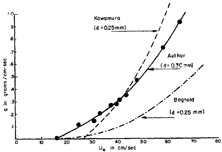
FIGURE 3 - RATE OF SAND TRANSPORT
