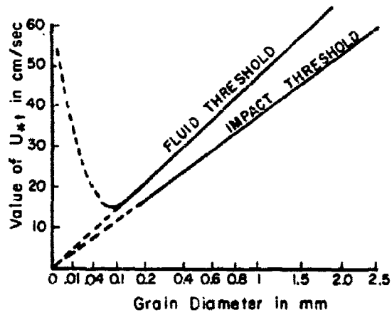
FIGURE 1 - VARIATION OF THE THRESHOLD WITH GRAIN SIZE
