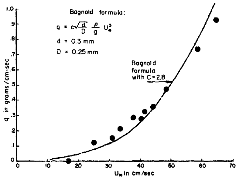
FIGURE 4 - COMPARISON BETWEEN EXPERIMENTAL RESULTS AND BAGNOLD FORMULA
