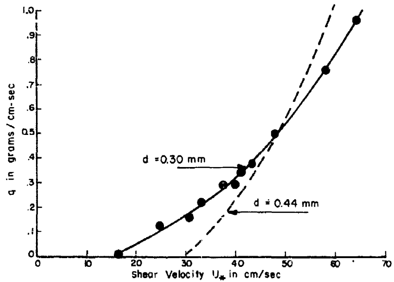
FIGURE 2 - RATE OF SAND TRANSPORT
