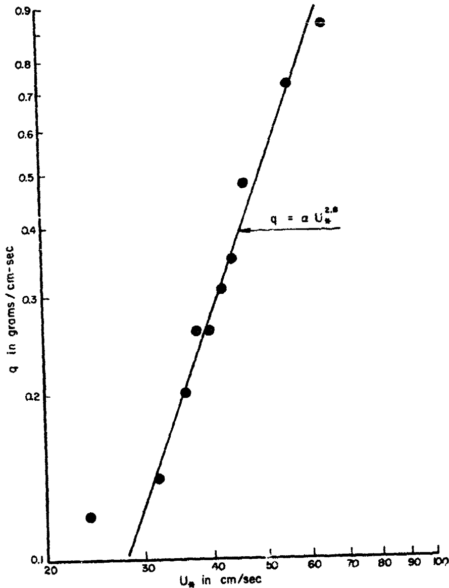
FIGURE 6- RATE OF SAND TRANSPORT
