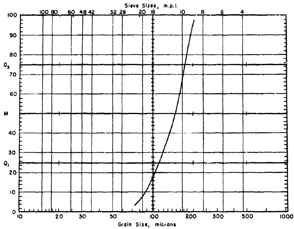
FIGURE 1. MECHANICAL ANALYSIS OF SAND
