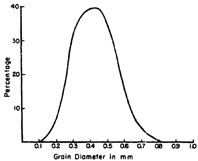
FIGURE 4 - GRAIN SIZE DISTRIBUTION
