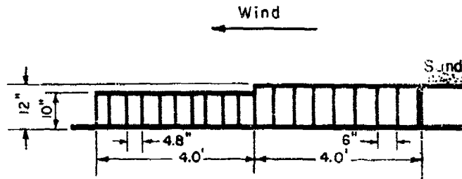
FIGURE 7 - HORIZONTAL SAND TRAP
