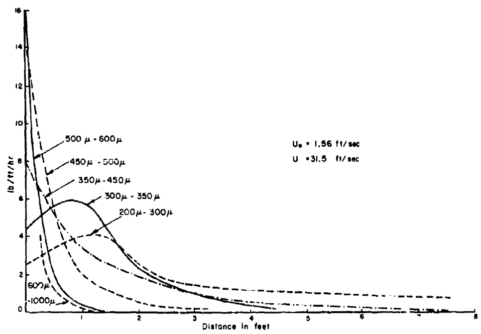
FIGURE 32 - SAND DISTRIBUTION IN THE HORIZONTAL TRAP FOR DIFFERENT GRAIN SIZES
