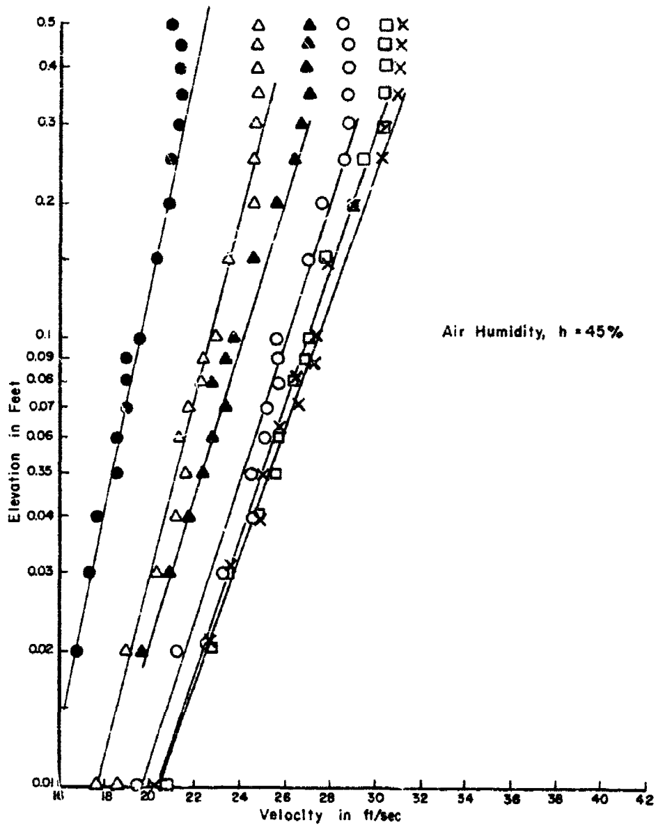
FIGURE 5 - TYPICAL VELOCITY DISTRIBUTION ABOVE SAND SURFACE
