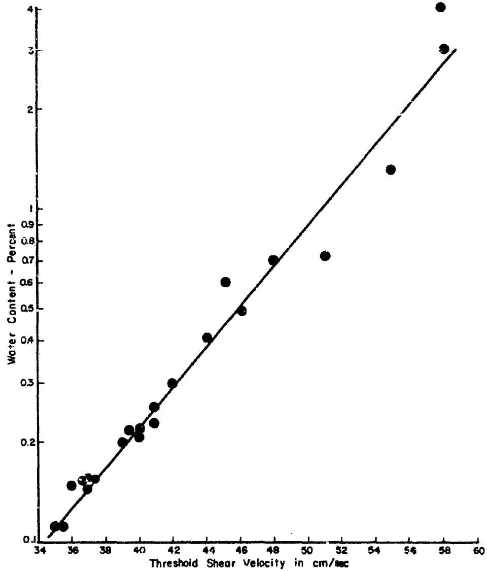
FIGURE 13 - VARIATION OF THE THRESHOLD WITH MOISTURE
