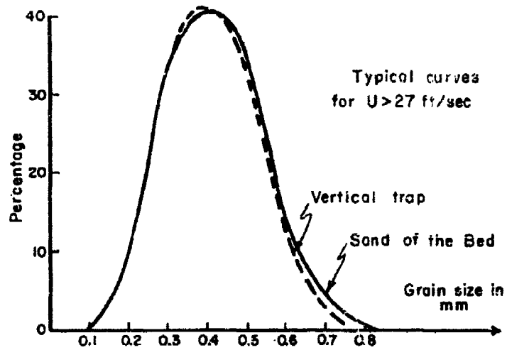
FIGURE 20 - GRAIN SIZE DISTRIBUTION FOR U > 27 ft/sec
