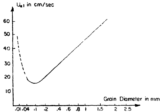
FIGURE 1- INITIATION OF SAND MOVEMENT
