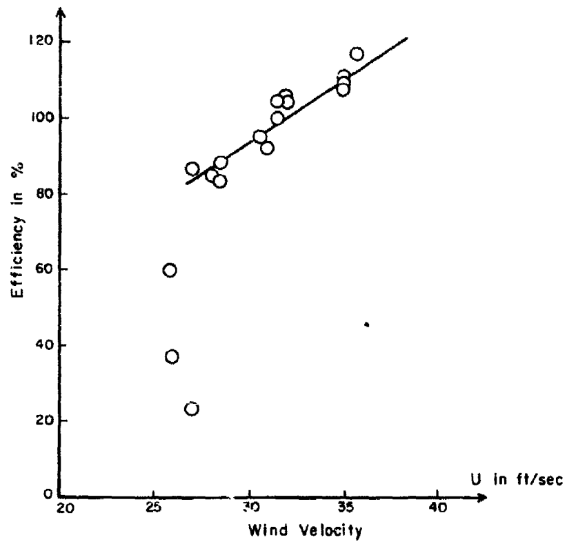
FIGURE 19 - EFFICIENCY OF THE VERTICAL TRAP
