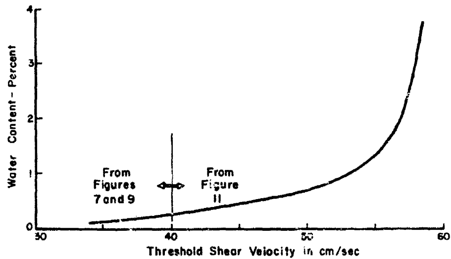
FIGURE 12 - VARIATION OF THE THRESHOLD WITH MOISTURE (COMPLETE RESULTS)
