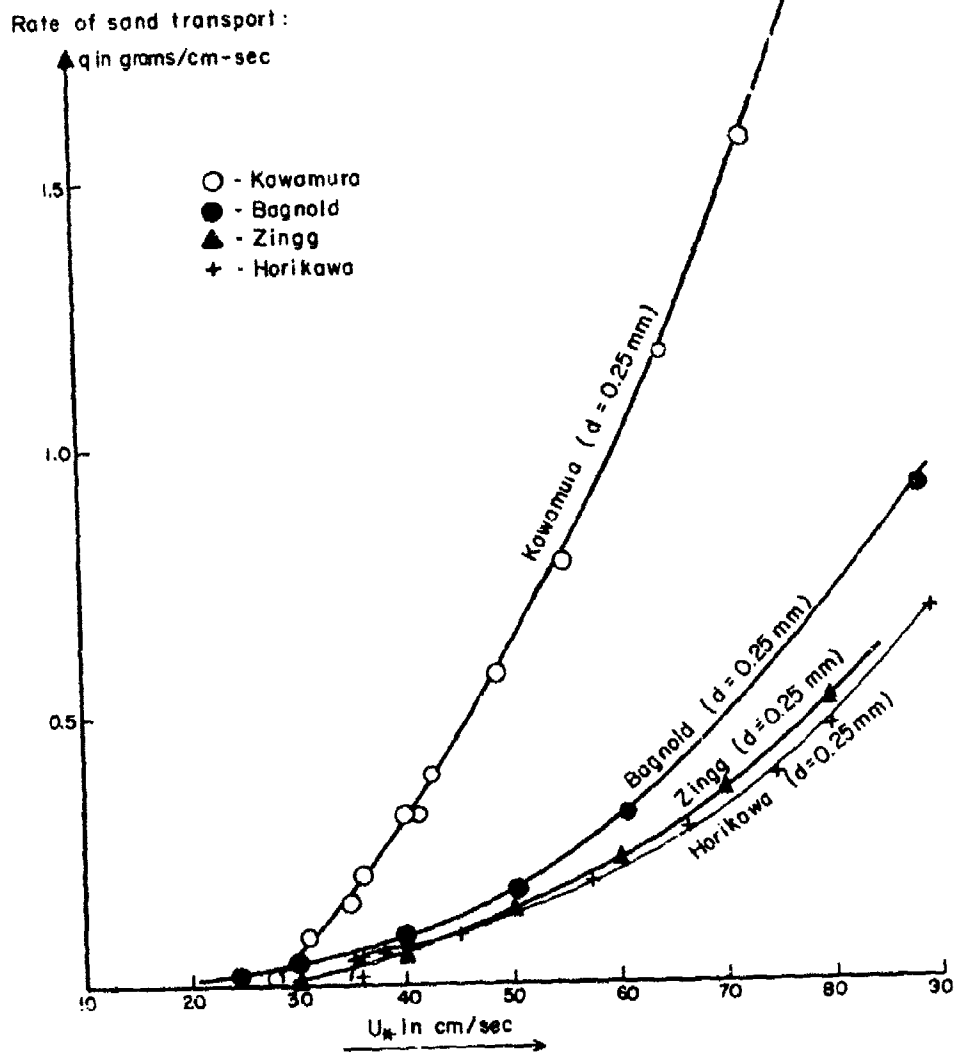
FIGURE 2 - EXPERIMENTAL RESULTS ON SAND TRANSPORT
