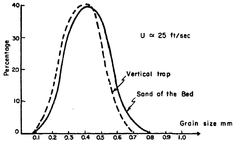
FIGURE 21 - GRAIN SIZE DISTRIBUTION FOR U \approx 25 ft/sec
