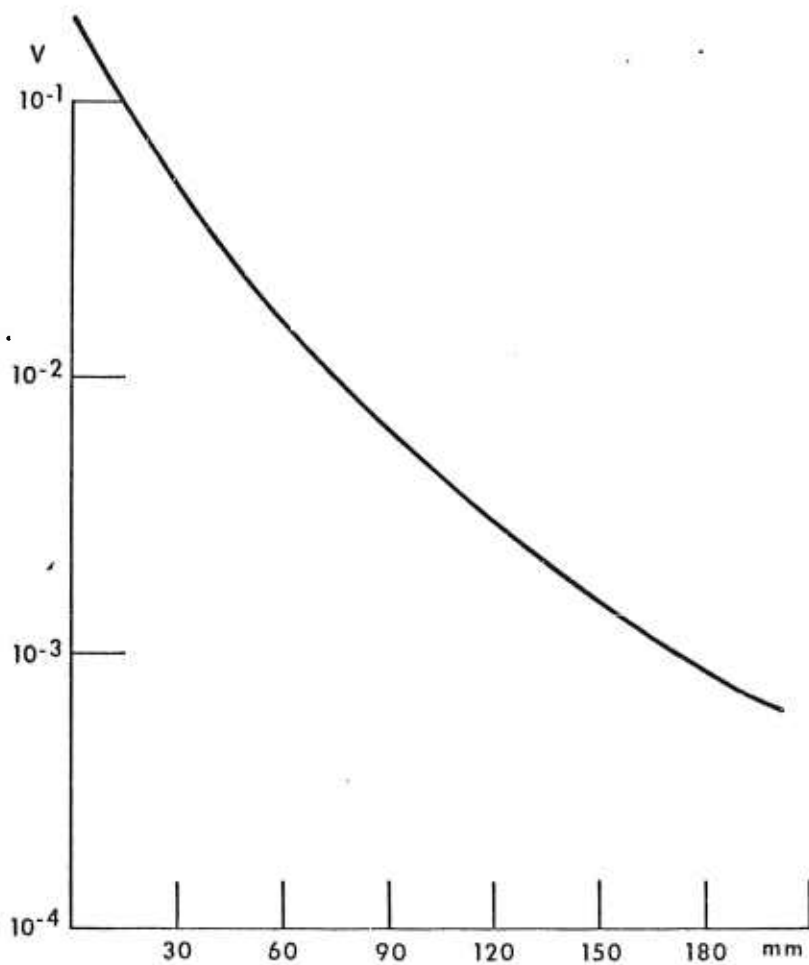
Fig. 5 Voltage Across the Resistor R=5k\Omega as the Function of the Distance of the Projectile From the Impact Probe (See Fig. 3). Ambient Pressure 30 mm Hg, Velocity of the Model 5334 m/sec.
