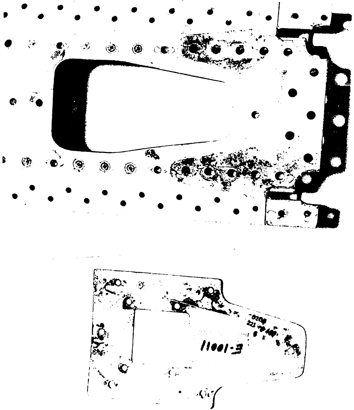
FIGURE 16 - Innercoastal Doubler and Electrical Door From RJ43-MA-11 Engine Serial MA-E10011-1 Showing Corrosion Which Occurred During the Accelerated Storage Phase of the RJ43-MA-11 Phase II Long-Term Storage Test.
