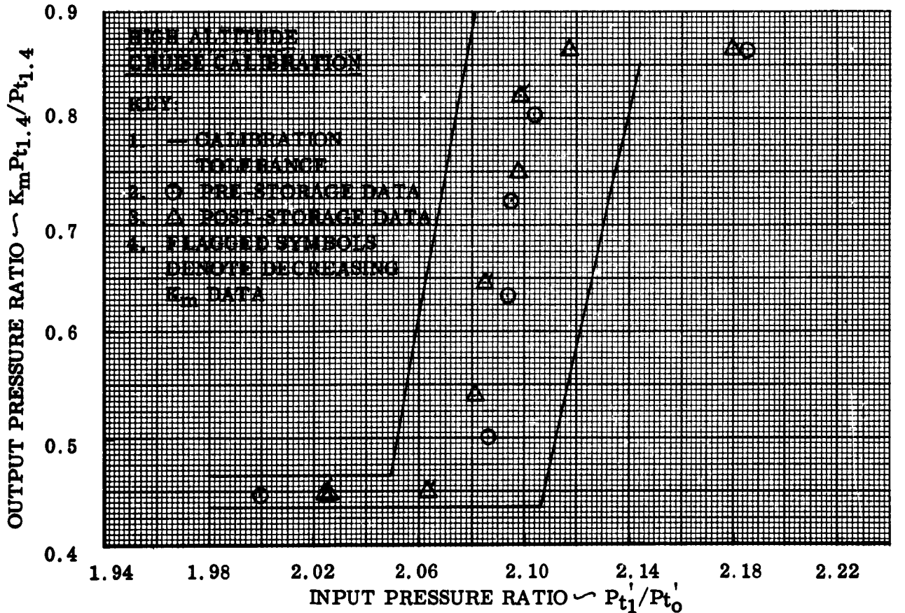
FIGURE 6 - RJ43-MA-11 Ramjet Engine Serial MA-E14901-1 Mach Sensor Control Calibration Data Before and After the RJ43-MA-11 Phase II Accelerated Storage Test.
