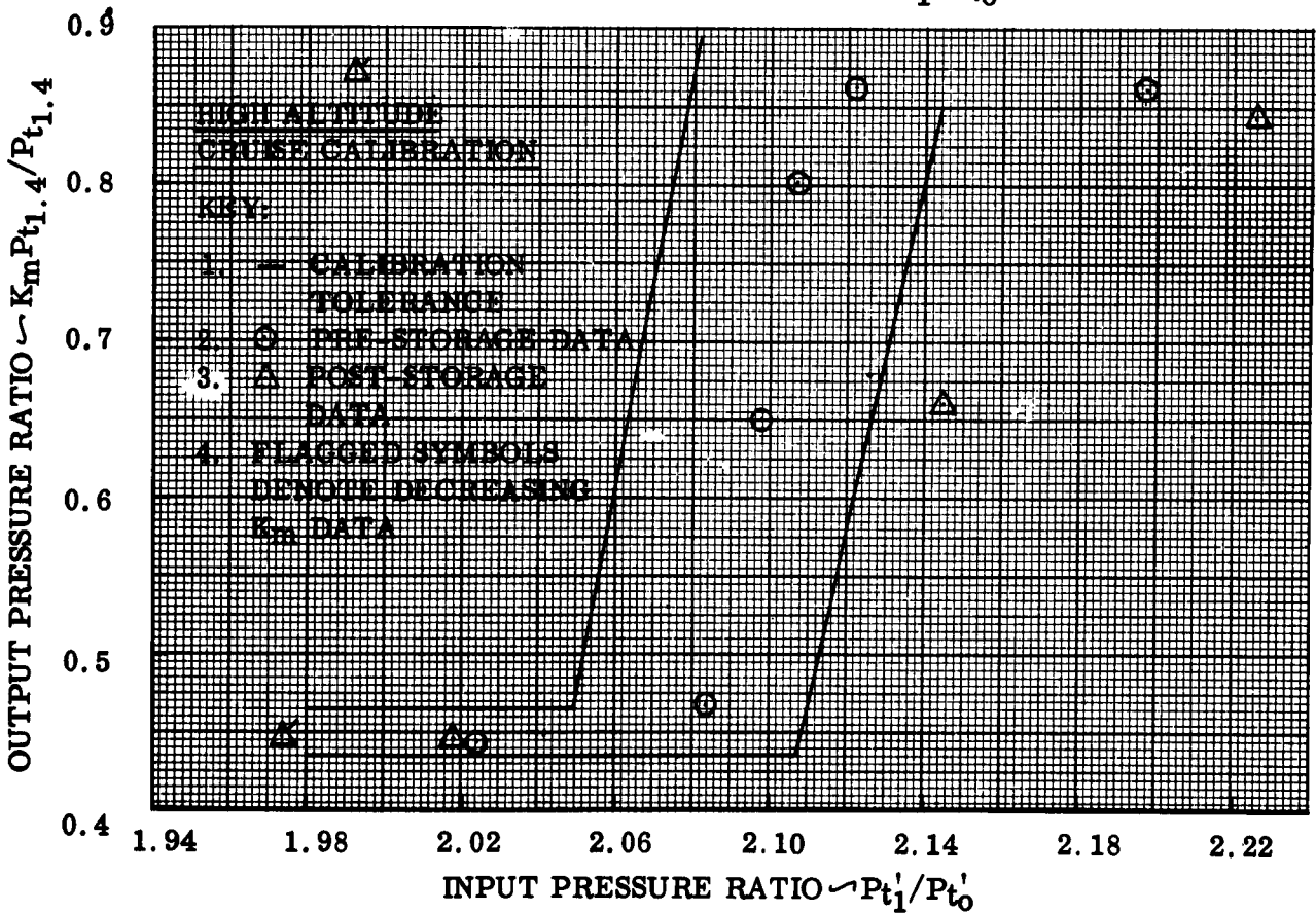
FIGURE 3 - RJ43-MA-11 Ramjet Engine Serial MA-E10011-1 Mach Sensor Control Calibration Data Before and After the RJ43-MA-11 Phase II Accelerated Storage Test.
