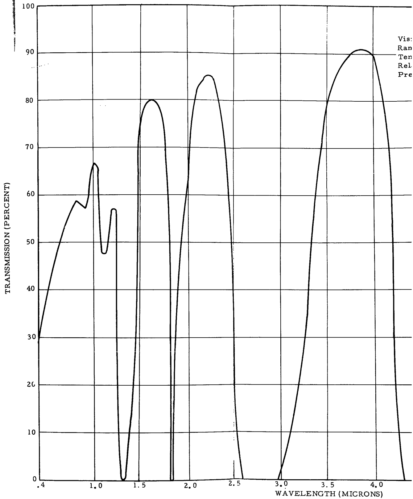
Figure 3. ATMOSPHERIC TRANSMISSION CURVE
