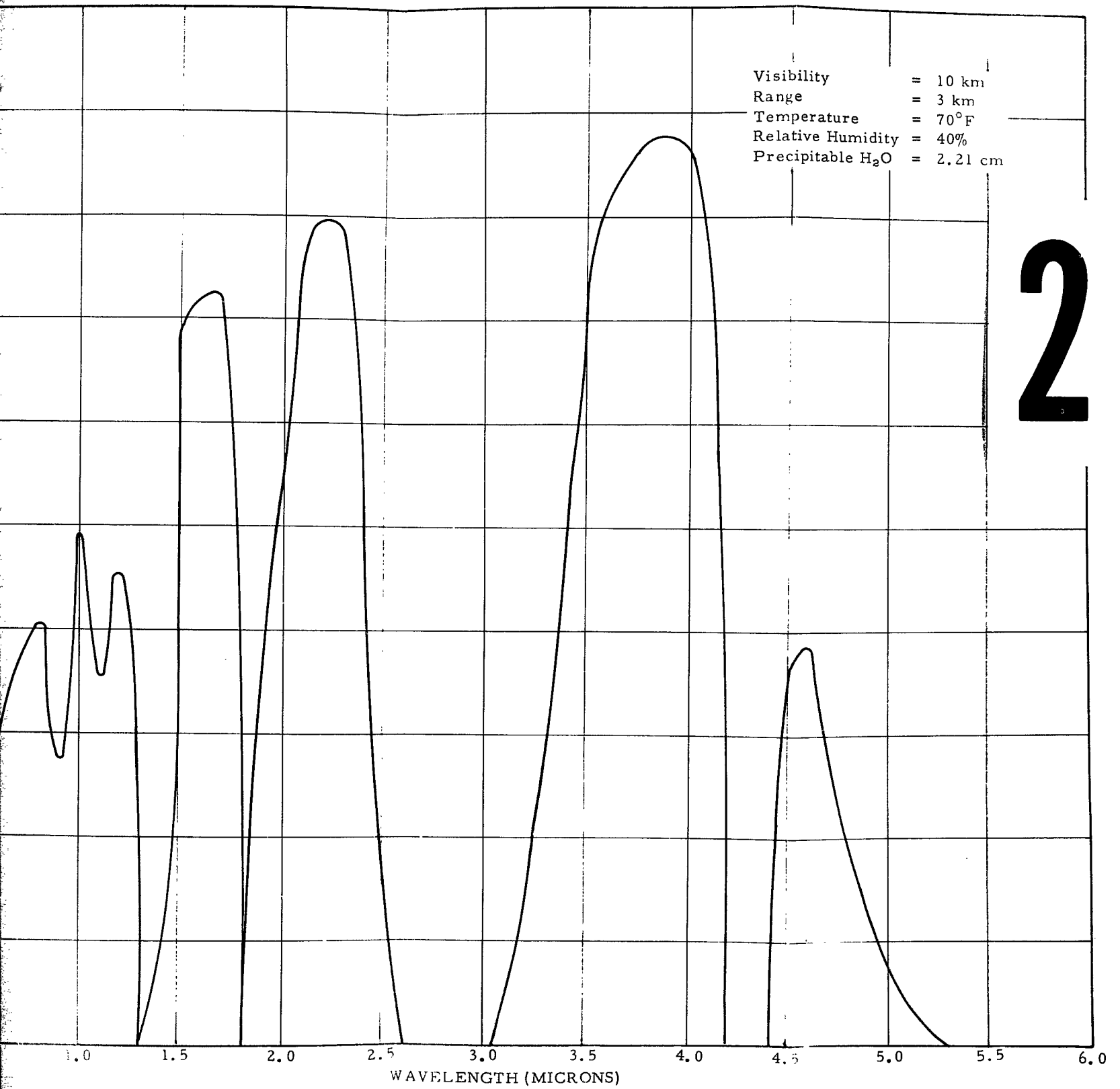
Figure 4. ATMOSPHERIC TRANSMISSION CURVE
