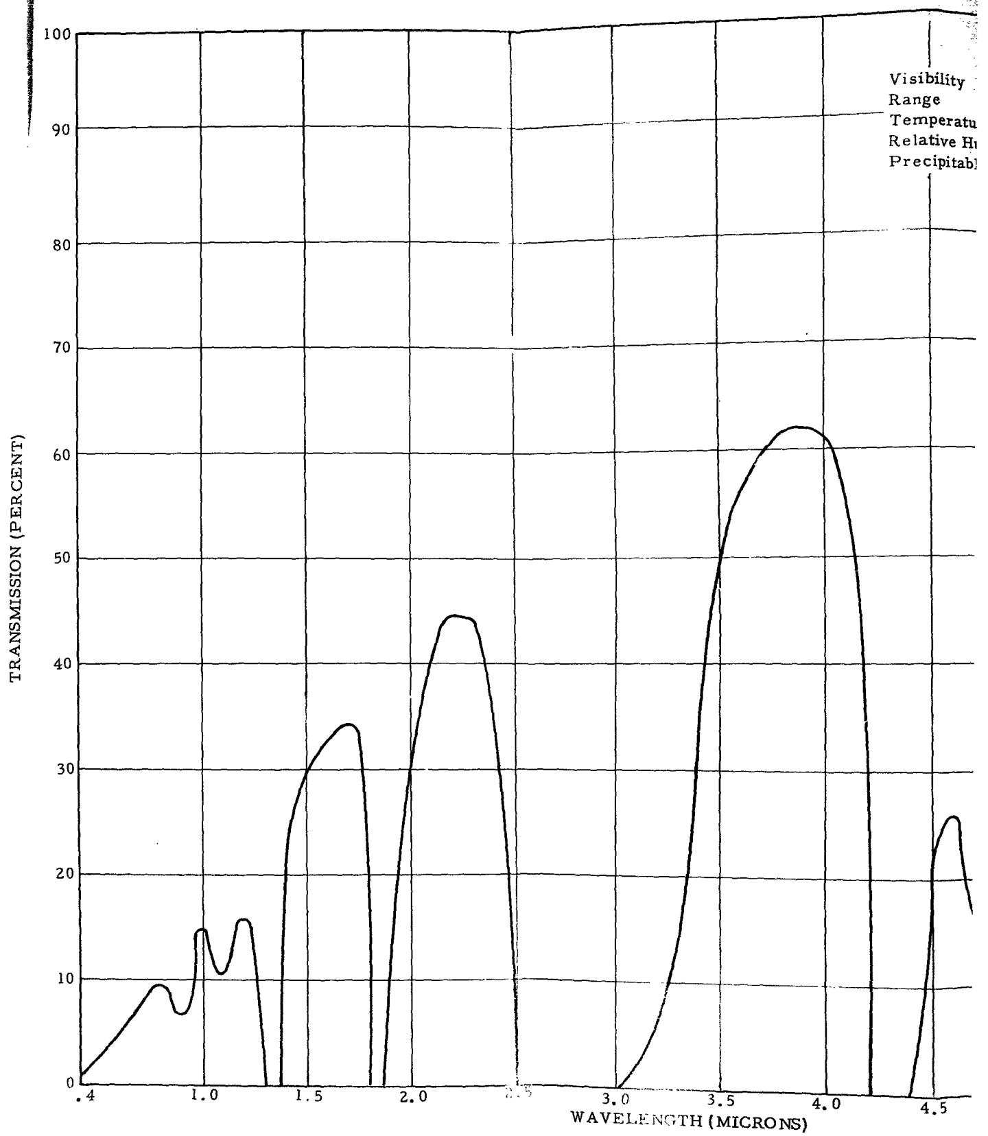
Figure 15. ATMOSPHERIC TRANSMISSION CURVE
