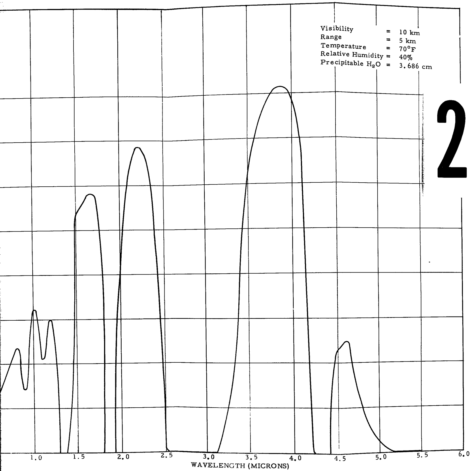
Figure 6. ATMOSPHERIC TRANSMISSION CURVE
