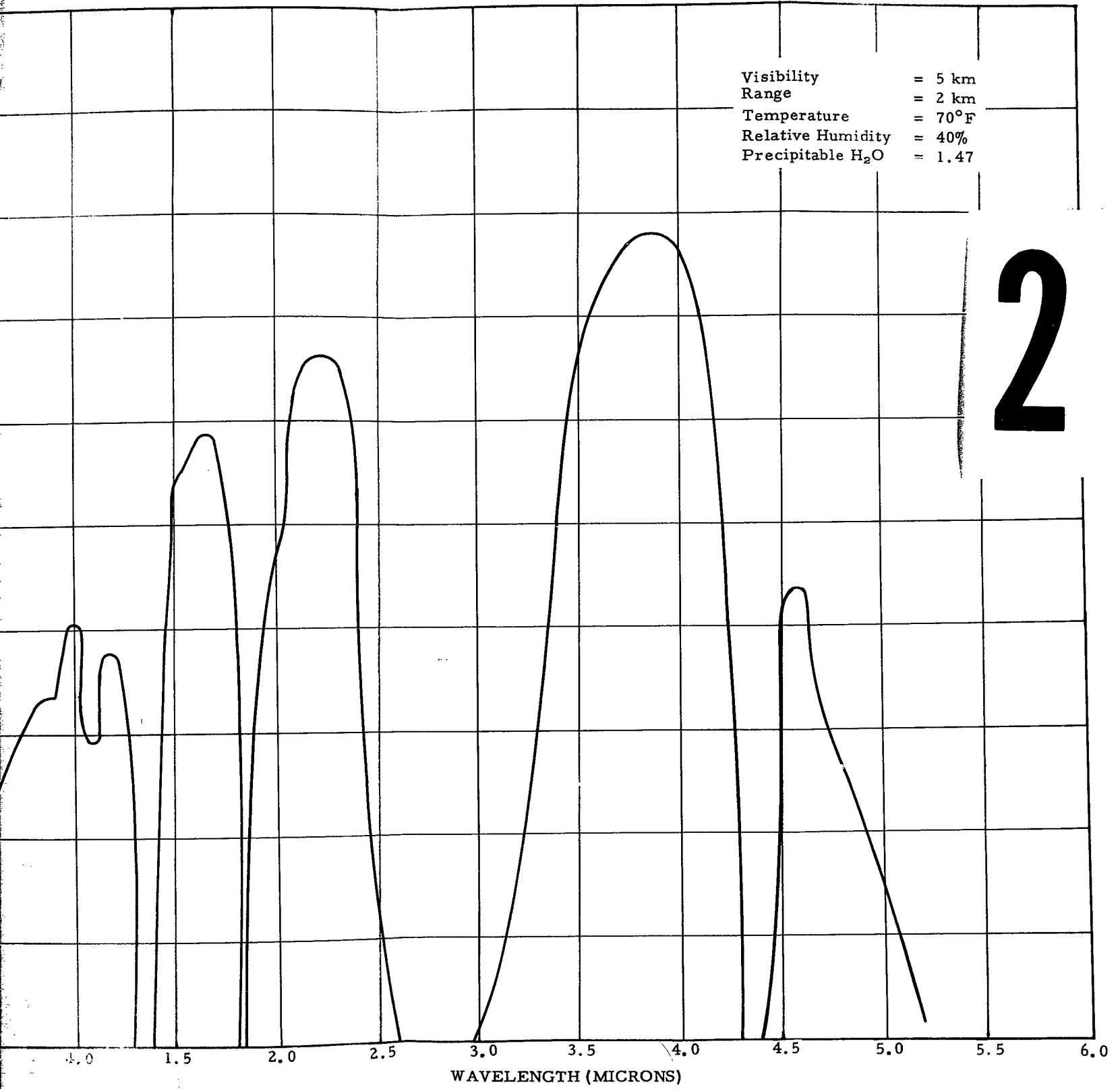
Figure 13. ATMOSPHERIC TRANSMISSION CURVE
