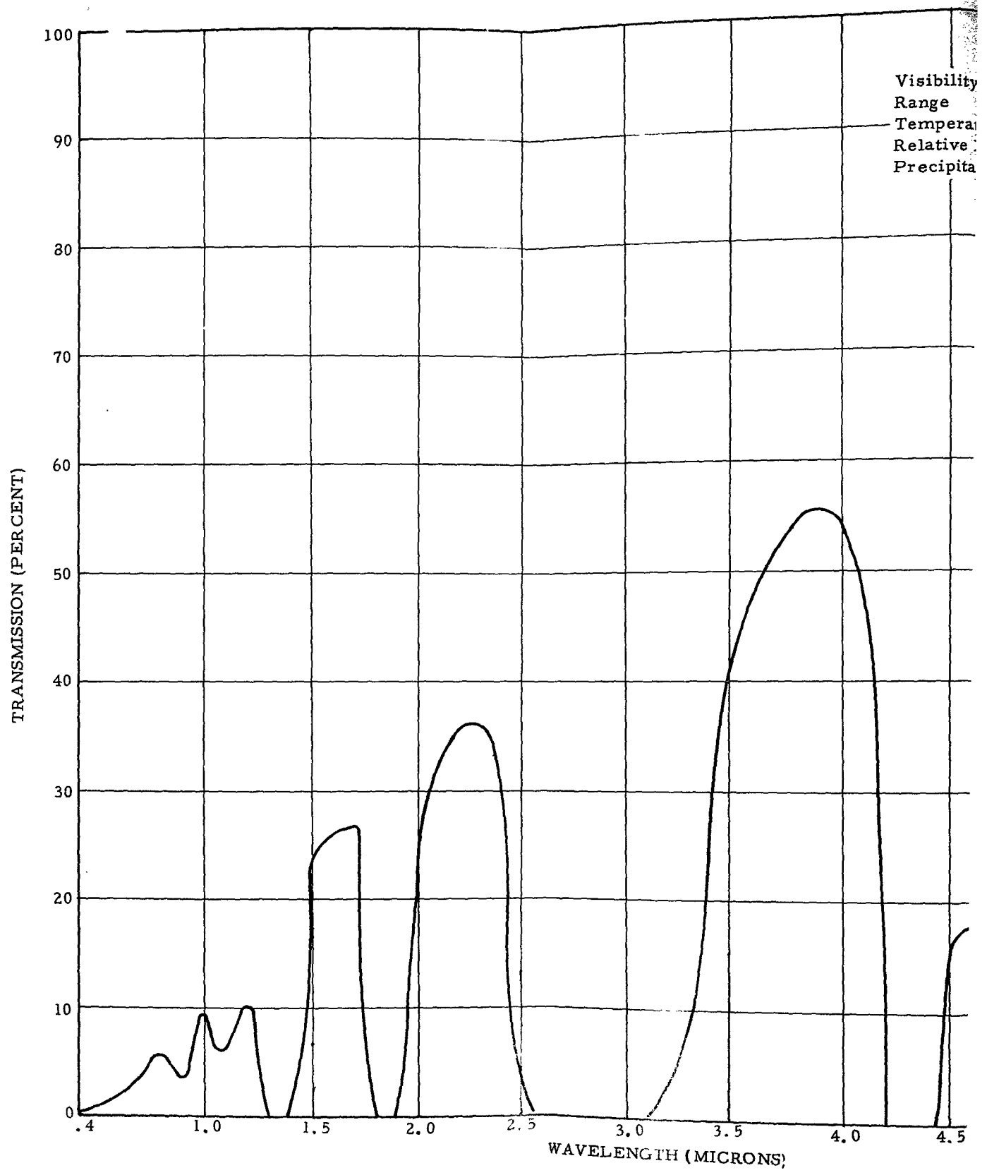
Figure 16. ATMOSPHERIC TRANSMISSION CURV
