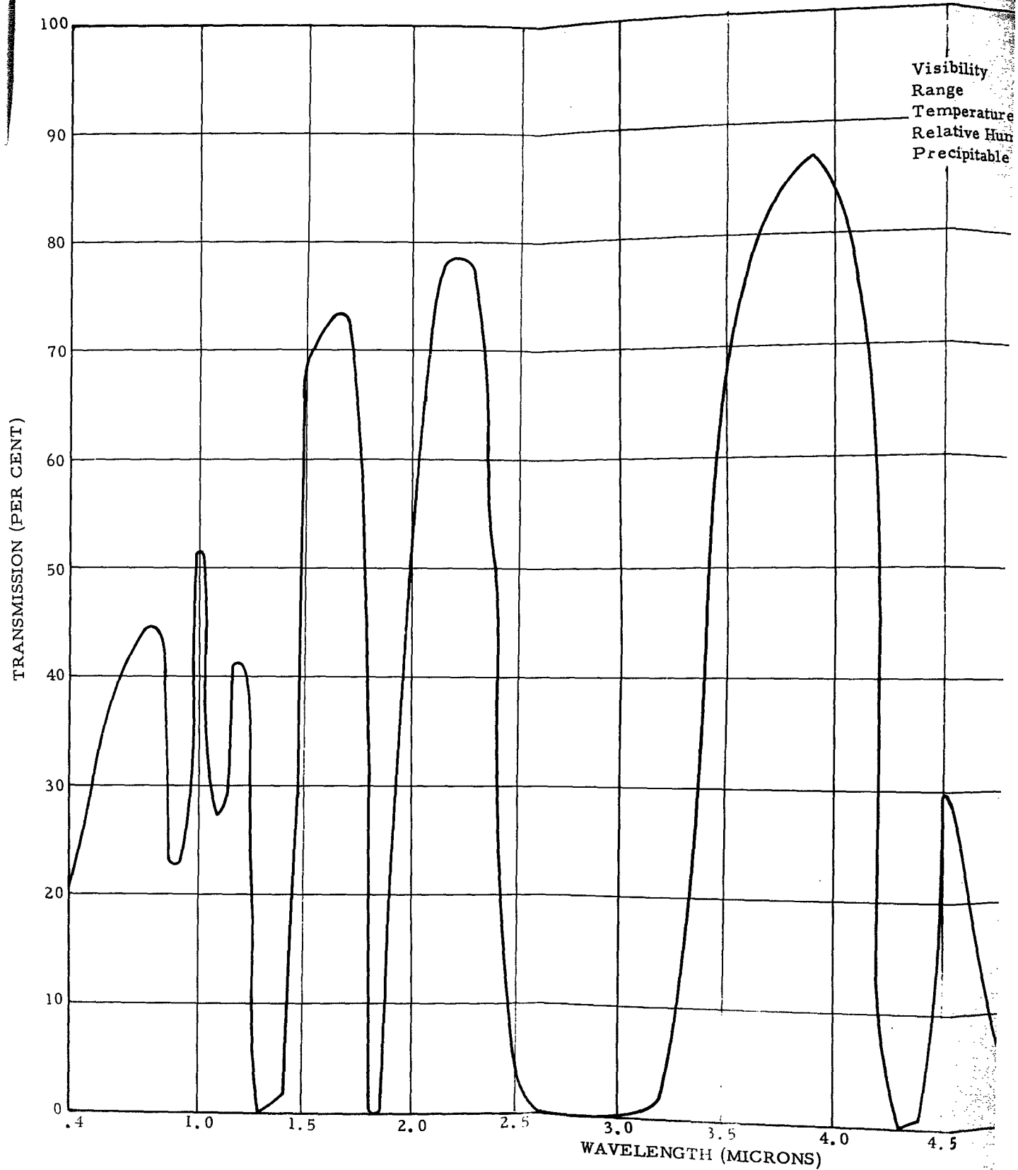
Figure 7. ATMOSPHERIC TRANSMISSION CURVE
