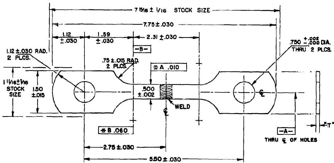
Figure B-3 Specification for Unnotched Tensile Specimen Tested at Cryogenic Temperatures
