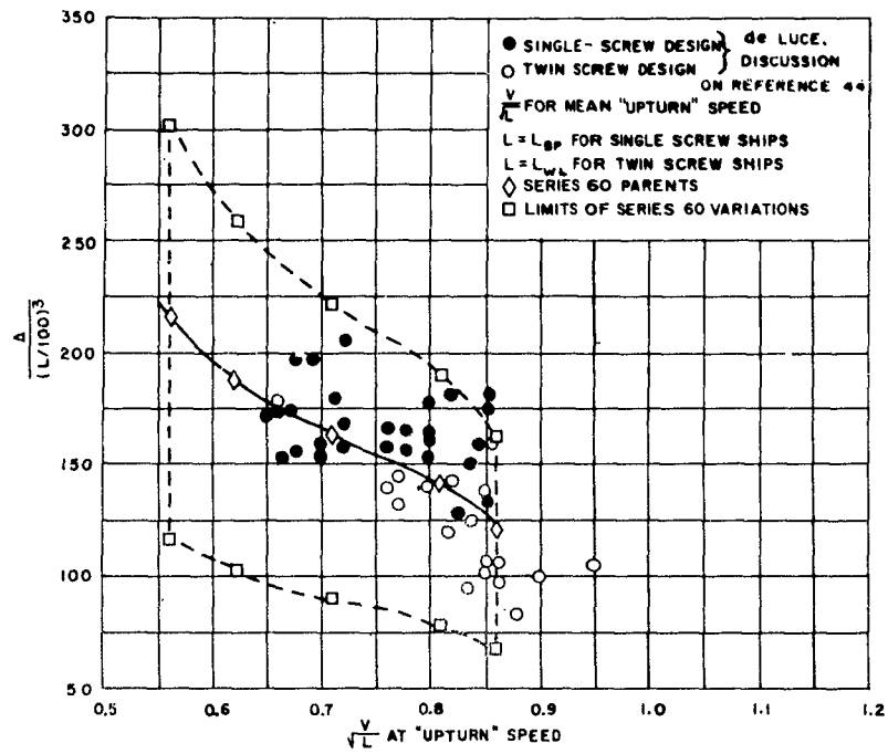
Figure 23 - Comparison of Series 60 with U. S. Data, \frac{V}{\sqrt{L}} and \frac{d}{(L/100)^3}
