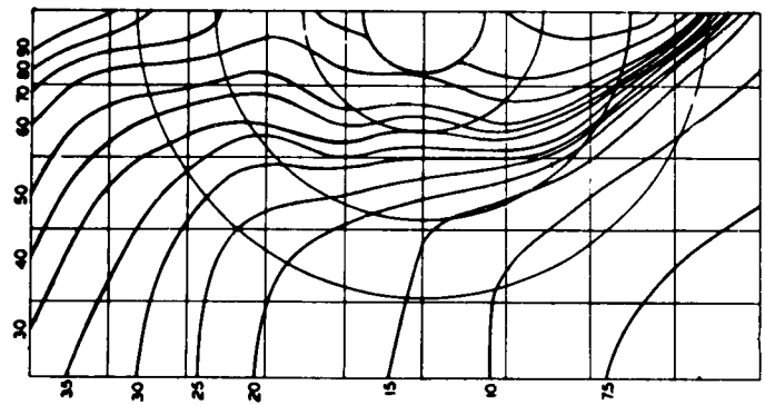
Figure 75c - Model 4213 C_B = 0.75
