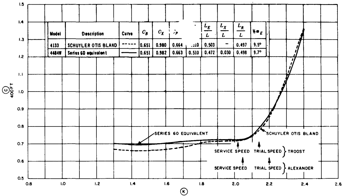
Figure 25b – Comparison, Series 60 and SCHUYLER OTIS BLAND
