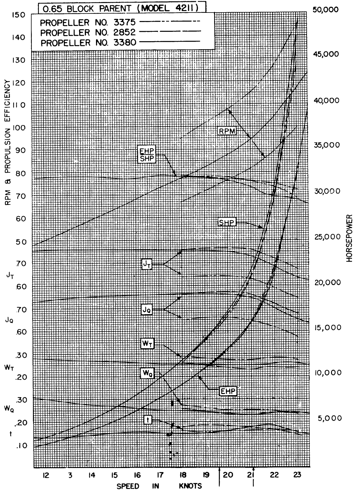
Figure 47 – Power, RPM, and Coefficient Curves for 0.65 Block Parent, at Even Keel and Designed Displacement—Model 4211
