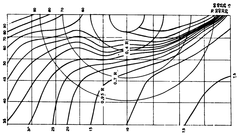
Figure 72a - Parent Form, Model 4280
