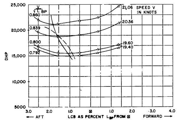
Figure 38b – C_B = 0.65
