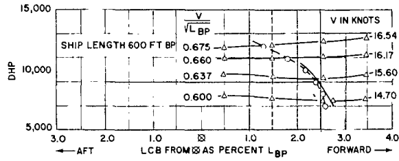
Figure 38d - C_B = 0.75
