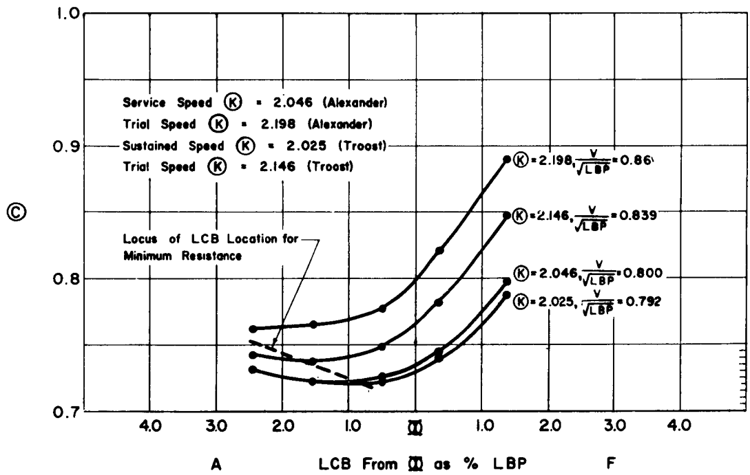
Figure 27 - Cross Curves of (C) on LCB. C_B = 0.65
