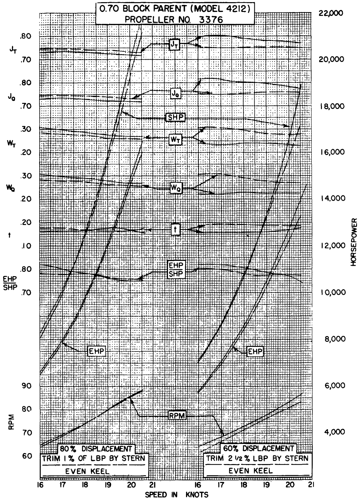
Figure 52 – Power, RPM, and Coefficient Curves for 0.70 Block Parent at Light Displacement Conditions
