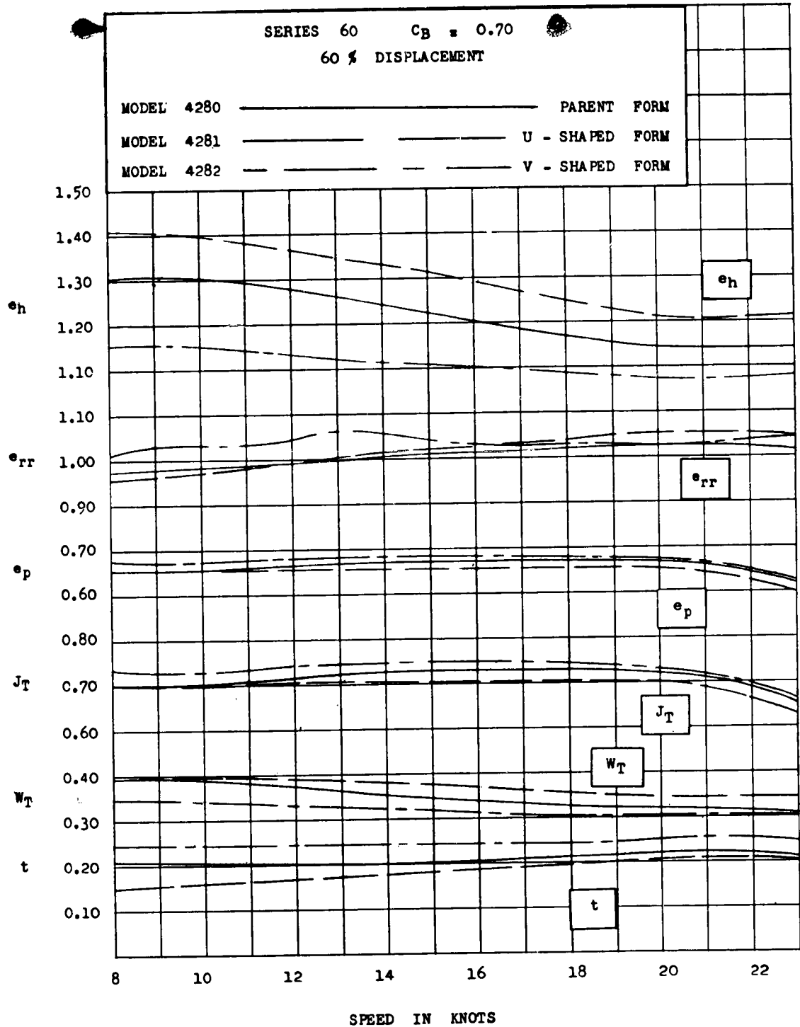
Figure 69 - Comparison of Coefficient Curves
