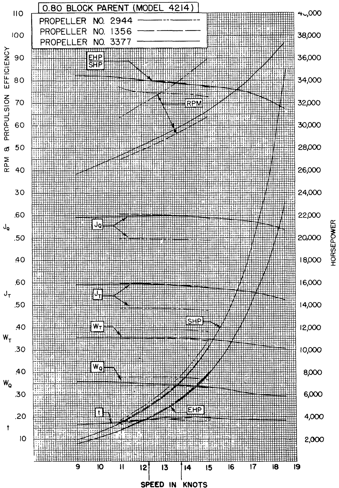
Figure 50 - Power, RPM, and Coefficient Curves for 0.80 Block Parent, at Even Keel and Designed Displacement—Model 4214
