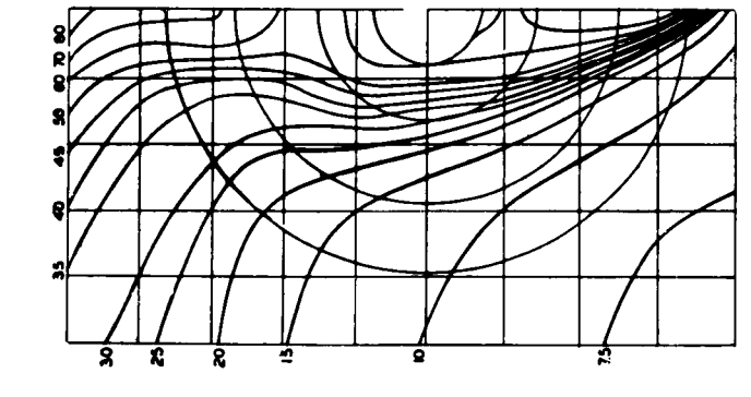
Figure 75b - Model 4218 C_B = 0.65
