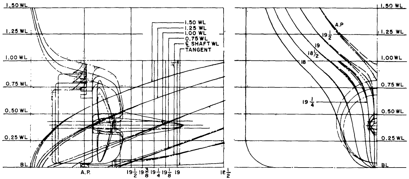
Figure 43 – Stern Lines for Propeller Diameter Variations, 0.70 Block Parent (Model 4212)
