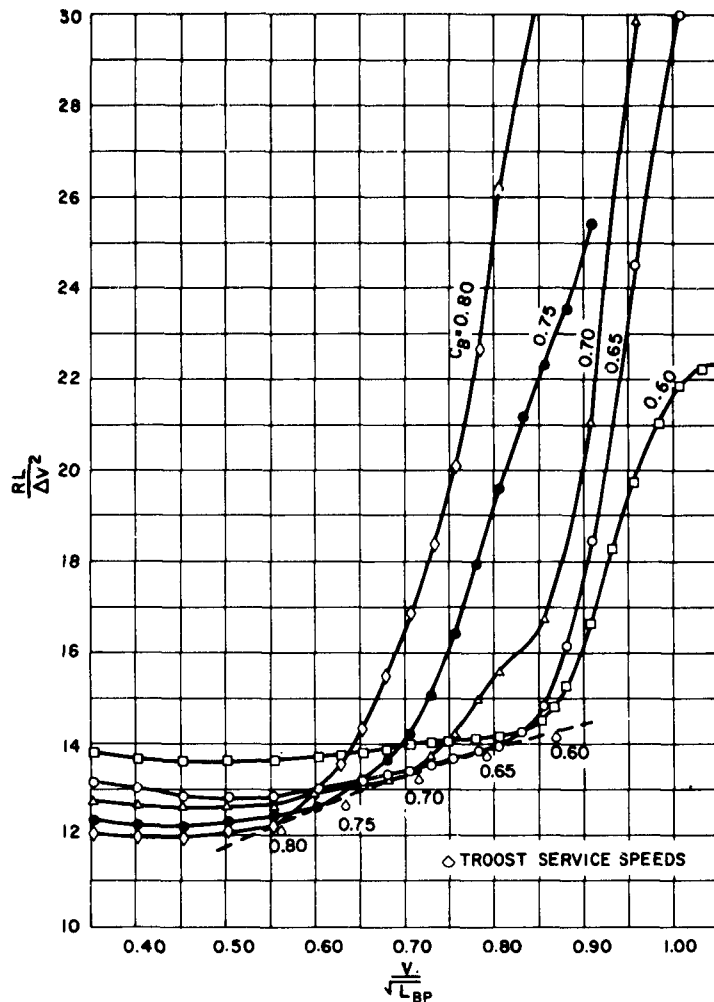
Figure 93 - \frac{RL}{\Delta V^2} on \frac{V}{\sqrt{L}} for Series 60 Parents
