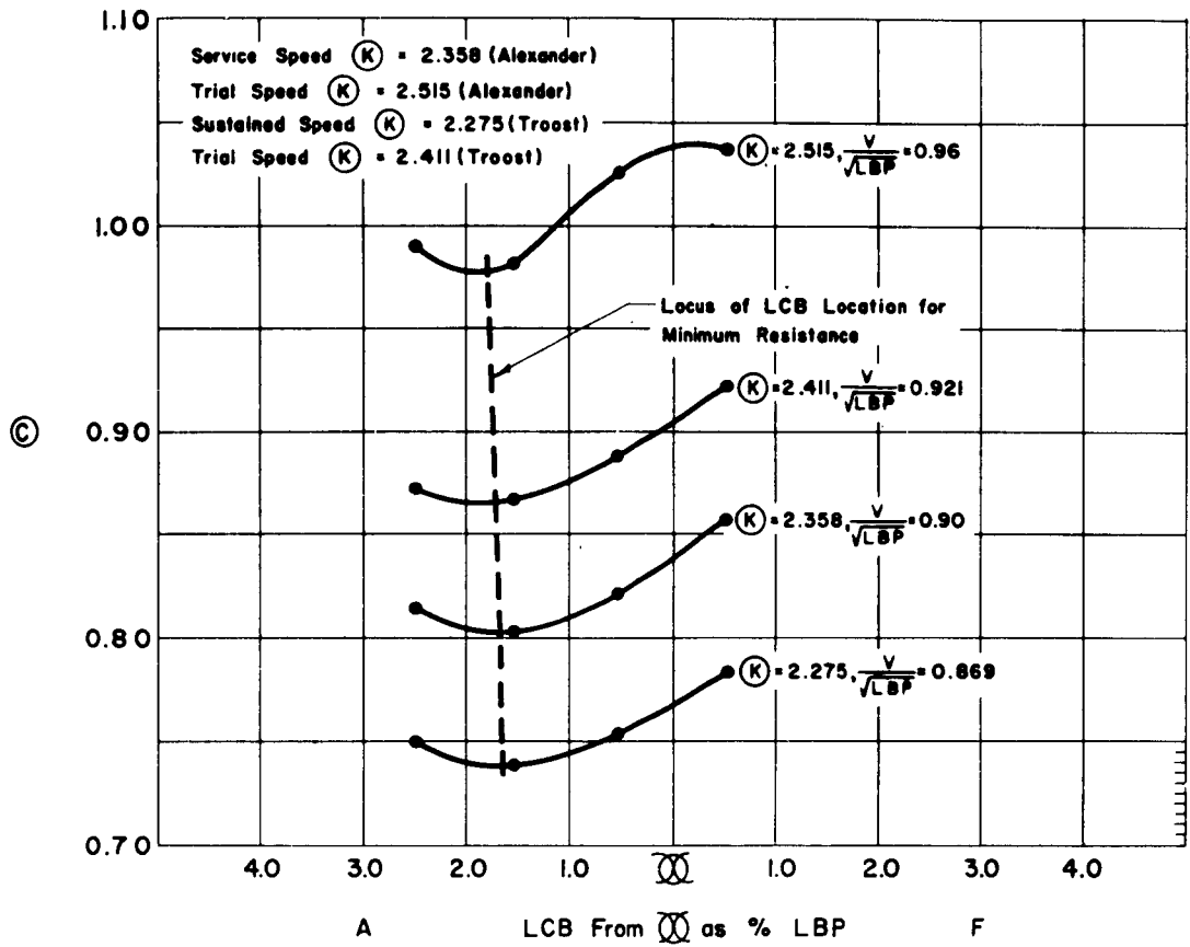
Figure 26 - Cross Curves of (C) on LCB. C_B = 0.60
