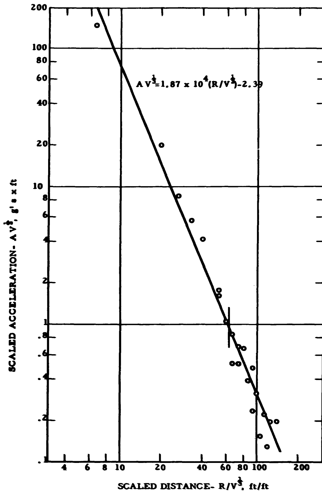
Fig.26 - Scaled Acceleration vs. Scaled Distance for Explosive AD 20A
