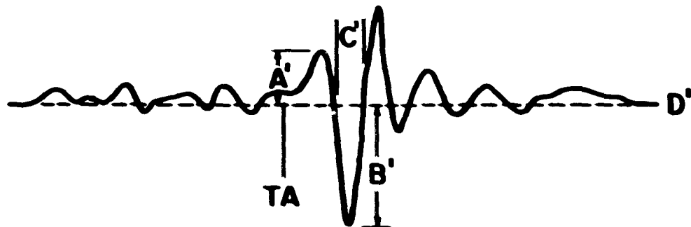
Tracing of record from transverse gage
