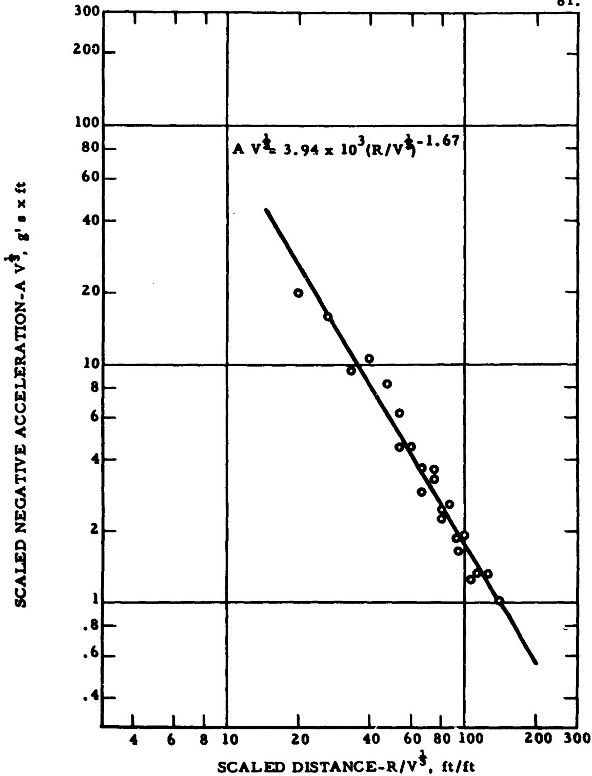
Fig. 32 - Scaled Negative Acceleration vs. Scaled Distance for Explosive SG 45
