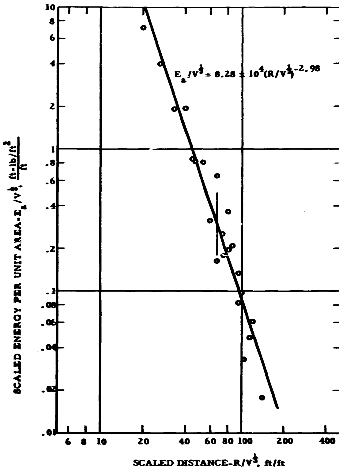
Figure 21-Scaled Energy vs. Scaled Distance for Explosive AD 10
