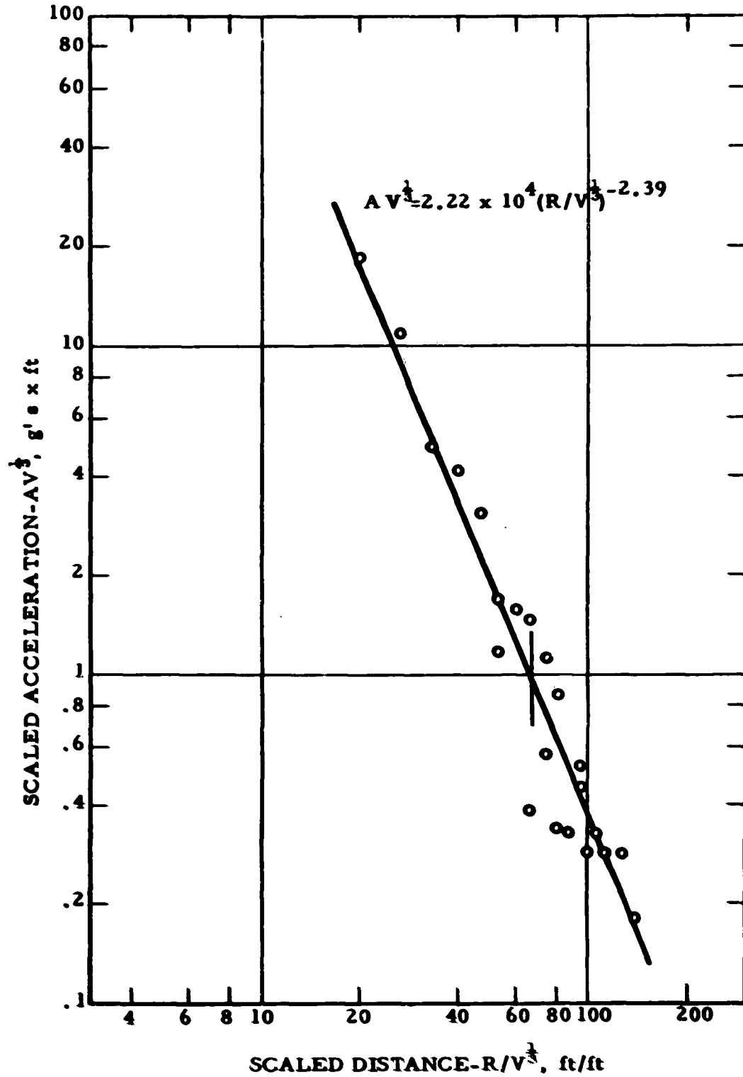
Fig.28 - Scaled Acceleration vs. Scaled Distance for Explosive SG 45
