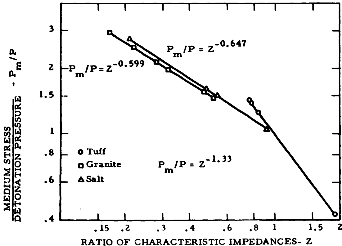
Fig. 69 - Peak Strain/Detonation Pressure vs. Ratio of Characteristic Impedances for Tuff, Granite and Salt.
