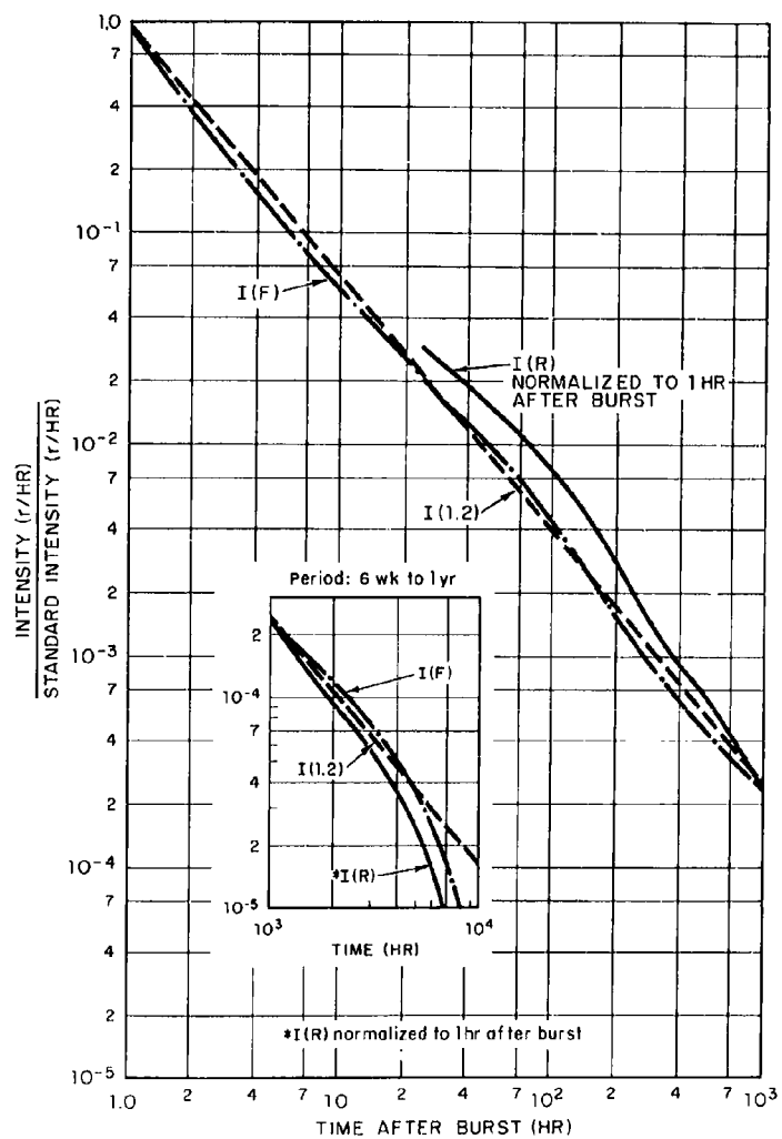
Fig. D.1 A Comparison of Three Decay Rates for Fission Product Activity
