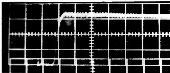
Figure 17. Wave Form of Voltage Transient across SF 6 Capacitor As Recorded with Capacitive Voltage Divider and 30-mc Scope Amplifier
