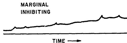
FIG. 8. Pressure-Time Trace From a Strand-Burning Test for a Marginally Inhibited Strand.
