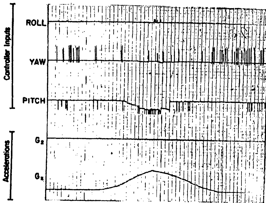
Inadvertent Control Input in the Pitch Axis
