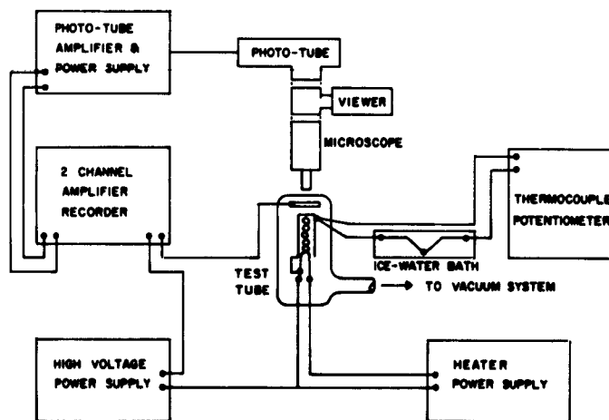
Fig. 1 - Block diagram of the apparatus for measuring the temperature dependence of pre-breakdown emission
