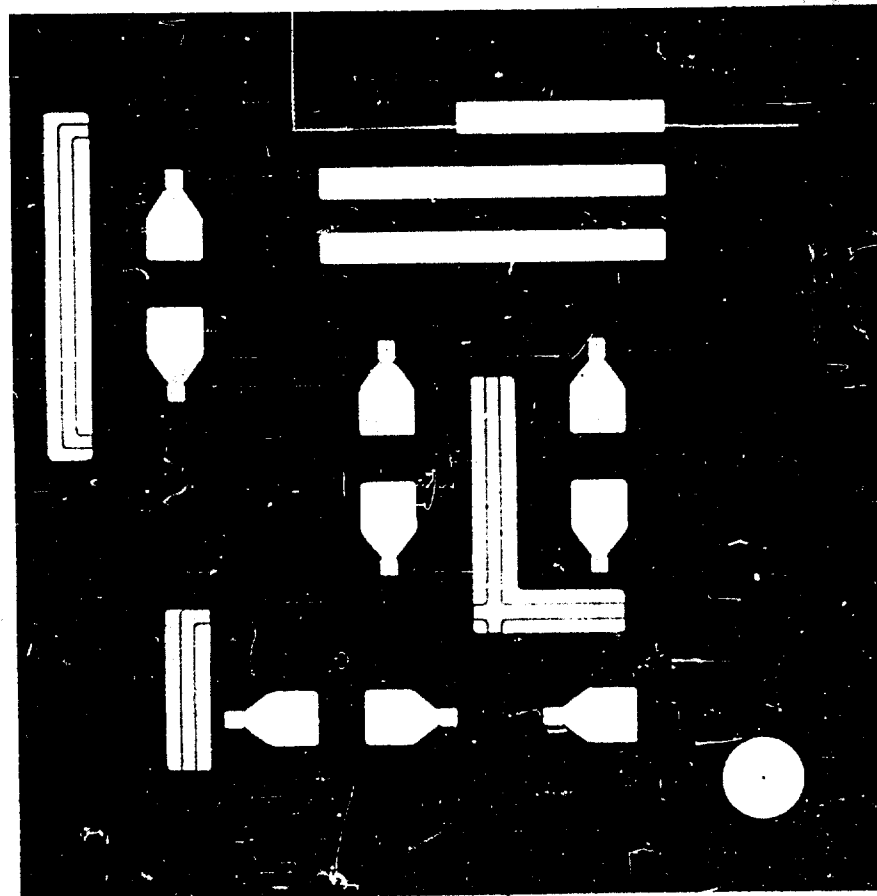
Figure 3. Masking and Base Diffusion
