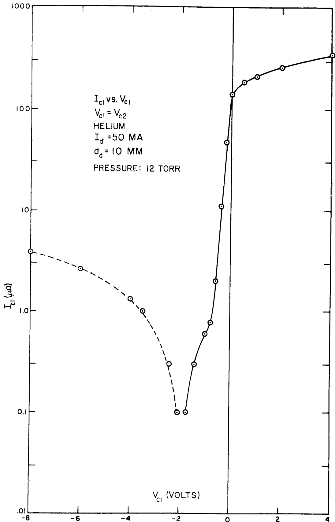
FIG. 6.8 TOTAL RETARDING CURVE
