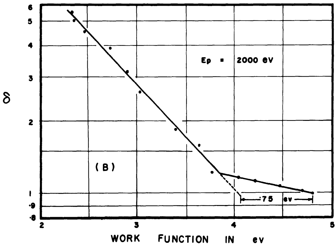
Fig. 17 Yield vs. Work Function
