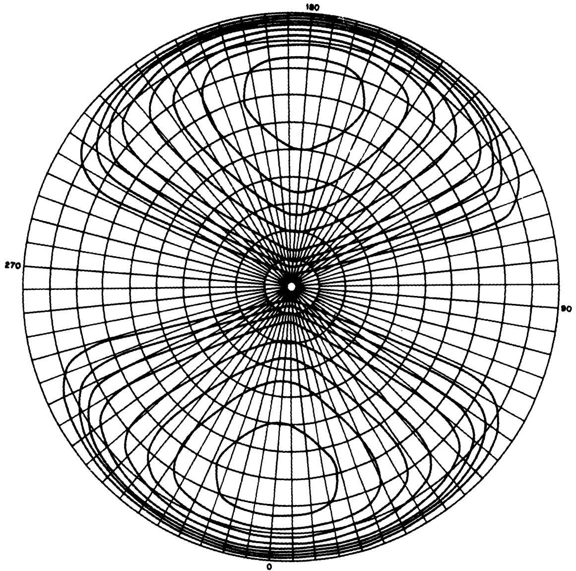
Fig. 4 — The perturbation field lines at t=10 \mu\text{sec}
