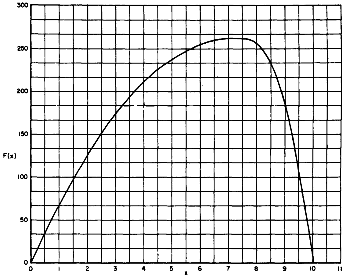
Fig. 3 — F(x) at t = 10 \mu\text{sec}
