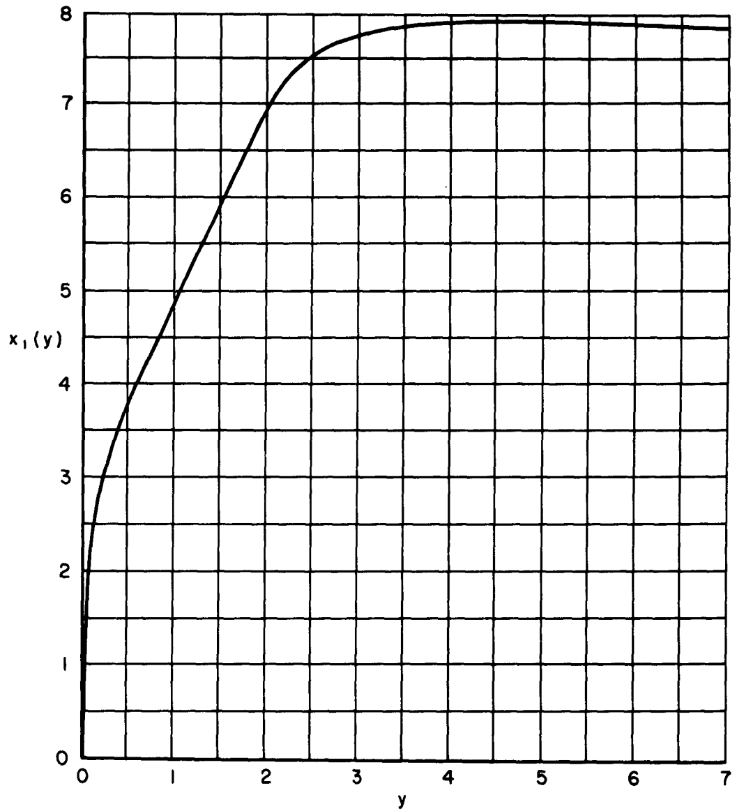
Fig. 1—Characteristic length x_1(y) versus normalized retarded time
