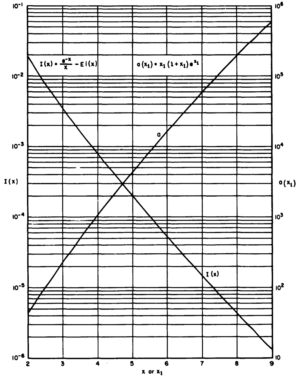
Fig. 5 — The functions I(x) and a(x_1)
