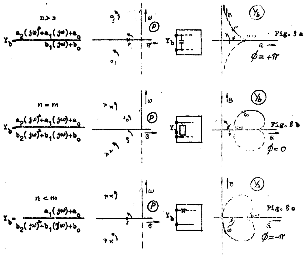
Fig. 8 : Poles and zeros of a network with the corresponding admittance curves.
