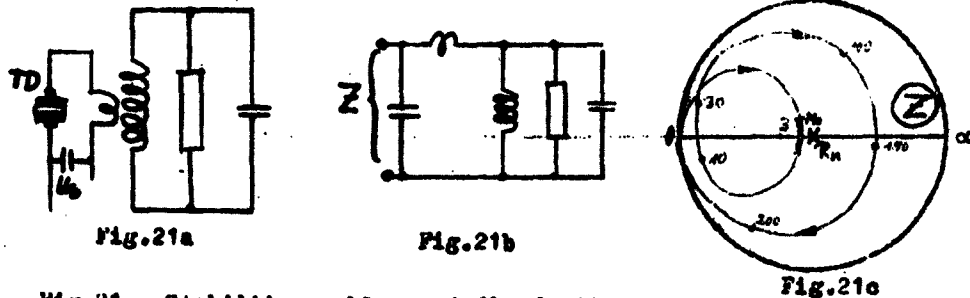
Fig. 21 : Stability problems at the deattenuation of a tank by a Td.
