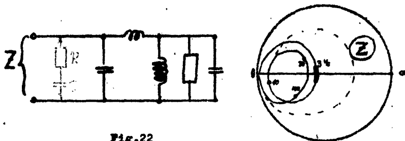
Fig.22 Influencing the impedance curve of an originally unstable circuit by a "two-pole-stabiliser".
