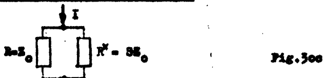
Fig. 30 : Transmission line having a termination which includes a positive or a negative realpart.
