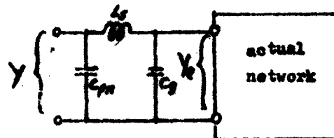
Fig. 13 Transformation of the measured admittance of the actual network into the suitable test function Y .
