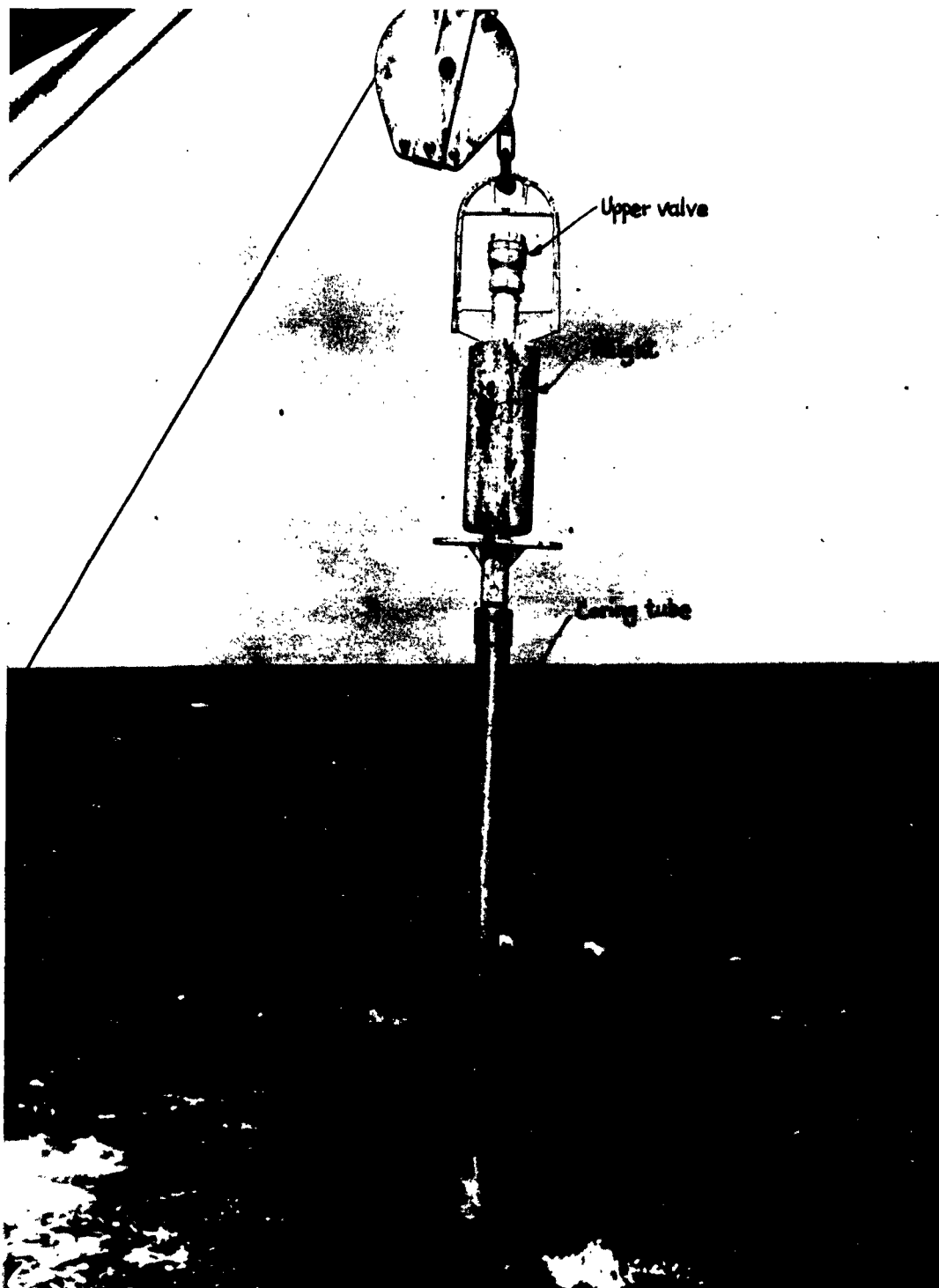
Figure 17. Gravity corer.
