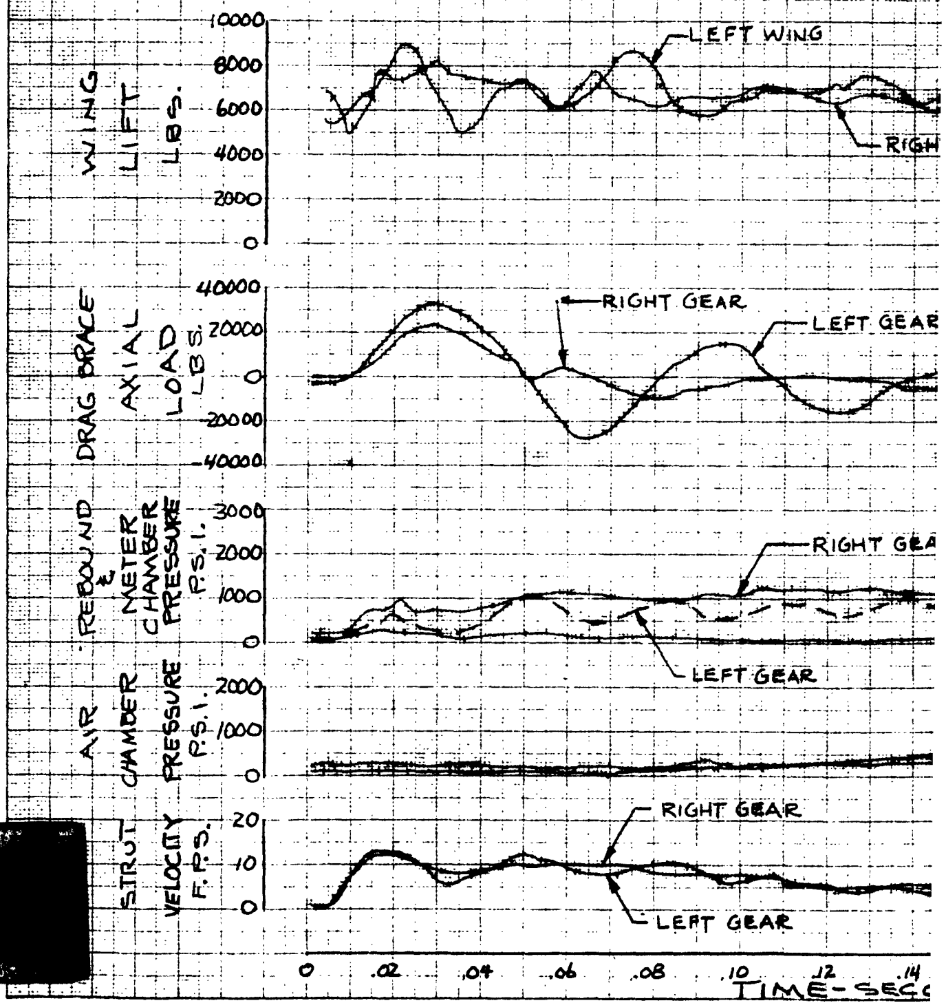
FIGURE 15 (CONT'D) LANDING LOADING AIRPLANE 70
