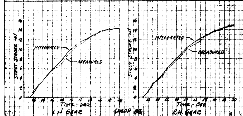
FIGURE 13. STRUT STROKE IN INCHES VERSUS TIME AS DETERMINED FROM THE SLIDE WIRE AND THE VELOCITY GENERATOR.
