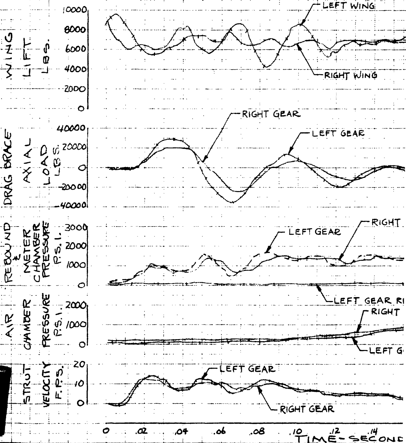
FIGURE 16 (CONT'D) LANDING LOADS AIRPLANE 84
