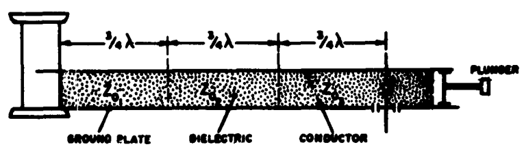
Figure 5. Microstrip Line with the Tunnel Diode at the End of the Third 3/4\lambda Transformer Section
