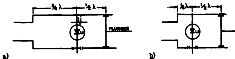
Figure 7. Third 3/4\lambda Section of Transformer with Tunnel Diode a) at the End of this Section and Plunger at the End of an Added \lambda/2 Section; b) at the \lambda/4 Point and Plunger at the End of the 3/4\lambda Section
