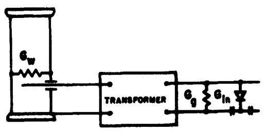
Figure 4. Schematic Circuit of Transformer for Conversion of G_w to G_g
