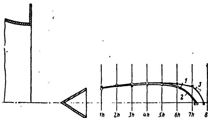
Fig. 11. Dimensions of backflow zone as a function of the initial turbulence of the stream at the rake of the stabilizer (stabilizer with \alpha_1 = 30 mm). 1) \epsilon \approx 2.5\% , \alpha = 1.69 , w = 50.9 m/sec; 2) \epsilon \approx 10\% , \alpha = 1.61 , w = 50 m/sec; 3) \epsilon \approx 15\% , \alpha = 1.57 , w = 50 m/sec.
