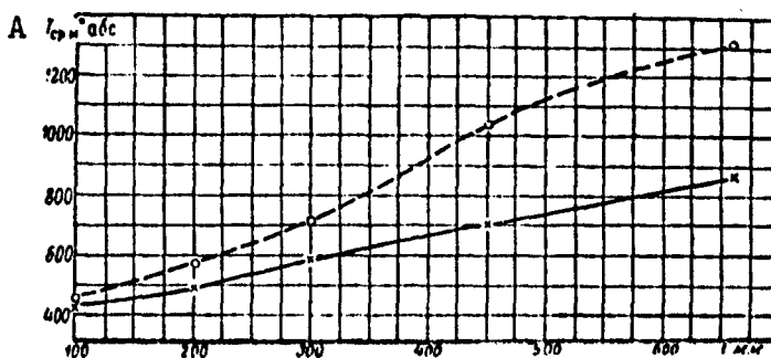
Fig. 28. Heat release along the chamber. Stabilizer No. 1, w = 50 m/sec, \alpha = 1.5 . x) Without turbulizing grid; o) turbulizing grid \phi 10 mm at a distance 350 mm from the stabilizer; A) abs.
