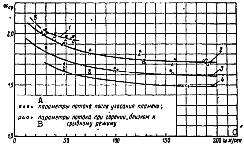
Fig. 3. Flameout characteristics of stabilizers of different dimensions. 1) Stabilizer with 2h = 60 mm; 2) stabilizer with 2h = 30 mm; 3) stabilizer with 2h = 20 mm; 4) stabilizer with 2h = 10 mm. A) Stream parameters after extinction of flame; B) stream parameters during combustion close to flameout mode; C) m/sec.
