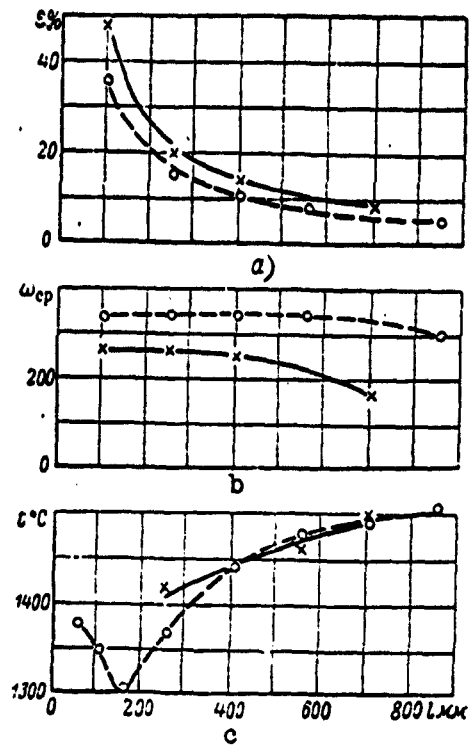
Fig. 13. Variation in the turbulence intensity \epsilon , in the average turbulent pulsation frequency \omega_{sr} , and in the temperature along the stabilizer axis. O) Mode I; x) mode VIII (behind the extreme stabilizer).
