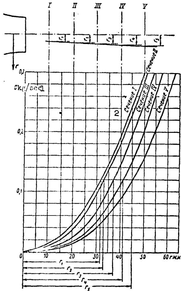
Fig. 5. Variation of gas flow along the radius of the jet (and the torch of the flame) at different sections. 1) kg/sec; 2) section.
