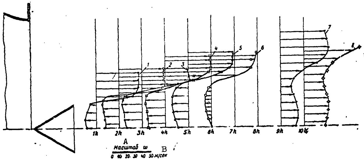
Fig. 15. Fields of axial velocity in the circulation zone behind the stabilizer with 2h = 60 mm at near-flameout mode, w = 50 m/sec, \alpha = 1.74 . 1) For section 1h; 2) for section 2h; 3) for section 3h; 4) for section 4h; 5) for section 5h; 6) for section 6h; 7) for section 9h; 8) for section 10h. A) Scale of w ; B) m/sec.
