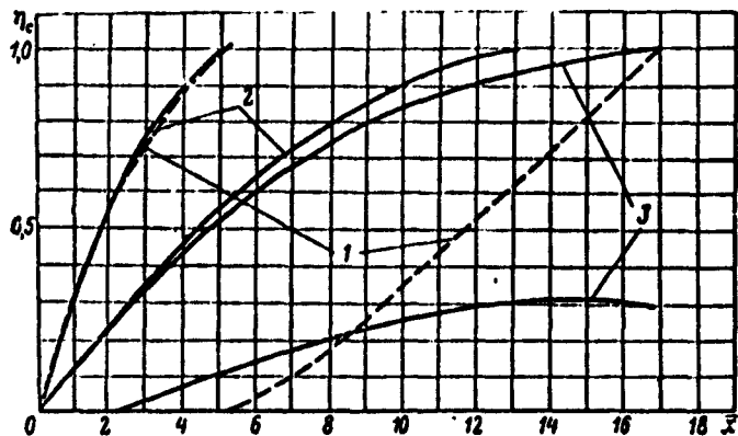
Fig. 6. Position of the flame boundary as calculated by A.V. Talantov (1) and as calculated by the proposed method (2) [3 - results of calculation by the proposed method if one assumes that u_t = 2.26 m/sec (curves 2 are obtained for w = 50 m/sec, u_t = 10 m/sec, T_0 = 288^\circ abs)].
