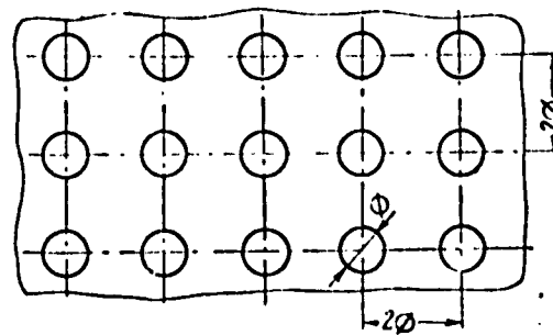
Fig. 4. Turbulizing grids.
