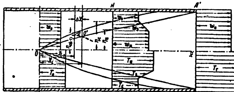
Fig. 1. Diagram of the flame torch in a tube.
