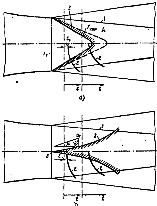
Fig. 1. Illustrating the determination of u_t in a free turbulent jet. a) Direct cone; b) inverted cone; 1) core of jet; 2) flame front; 3) igniting burner. A) Cone.
