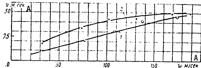
Fig. 8. Variation of axial velocity u in the backflow zone on the velocity of the incoming stream. (Stabilizer with 2h = 30 mm in the free jet.) 1) \alpha = \infty ; 2) \alpha = 0.9\alpha_{sr} . A) m/sec.
