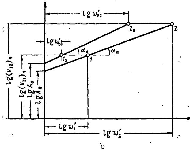
Fig. 2. The dependence u_t = f(w') in logarithmic coordinates.
