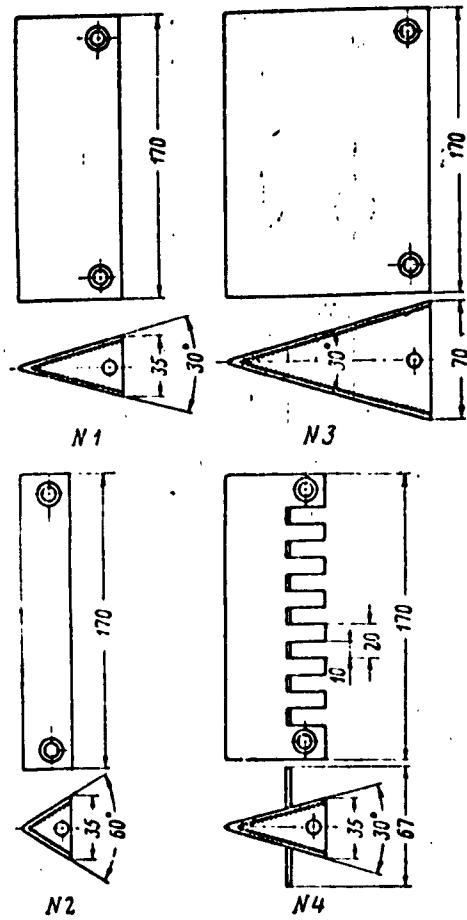
Fig. 3. Stabilizers.
