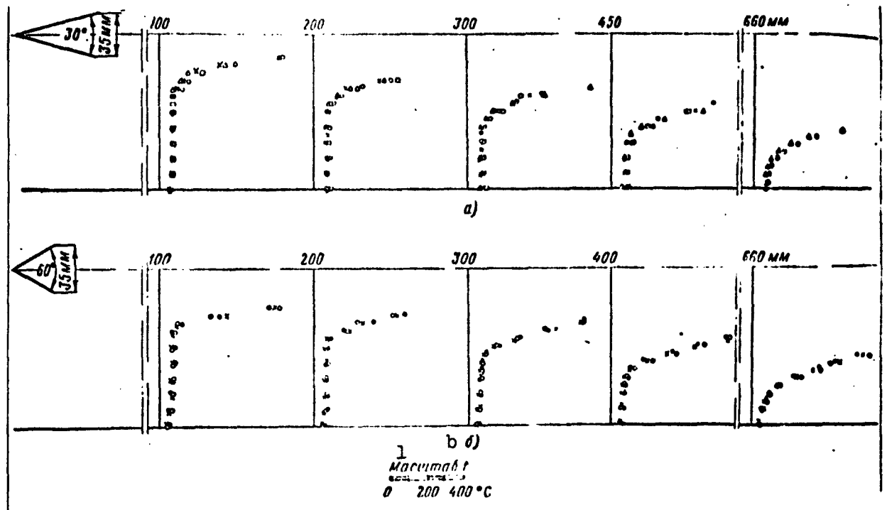
Fig. 11. Temperature fields.
