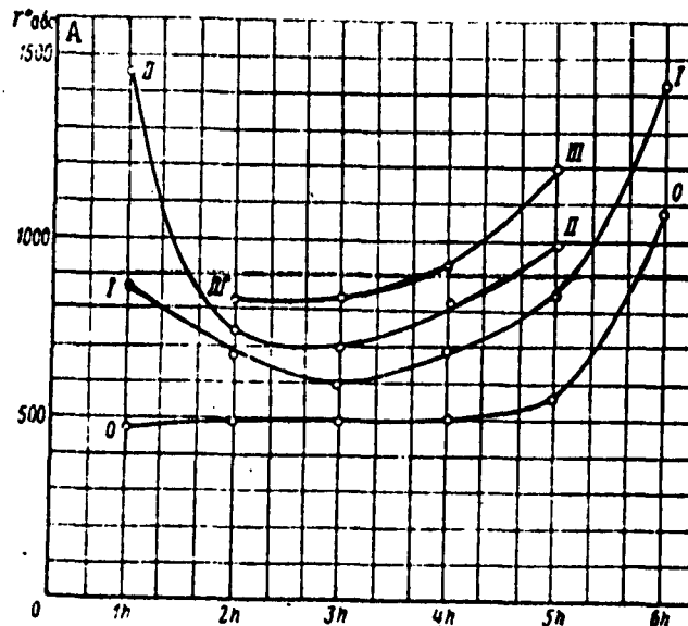
Fig. 18. Variation of gas temperature along the current lines I-I, II-II, III-III in the direct stream of the circulation zone and in the first "jet" of the active stream 0-0 (stabilizer with 2h = 60 mm, w = 50 m/sec, \alpha = 1.74 ). A) Absolute.
