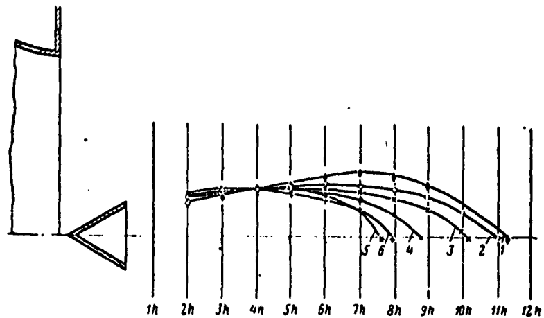
Fig. 6. Dimensions of the backflow zone during combustion, as a function of the velocity of the incoming stream. (Stabilizer with 2h = 30 mm, \alpha = 0.9\alpha_{gr} , in free jet.) 1) w = 170 m/sec, \alpha = 1.44 ; 2) w = 130 m/sec, \alpha = 1.50 ; 3) w = 105 m/sec, \alpha = 1.53 ; 4) w = 74.5 m/sec, \alpha = 1.59 ; 5) w = 50.9 m/sec, \alpha = 1.69 ; 6) w = 29.9 m/sec, \alpha = 1.69 .
