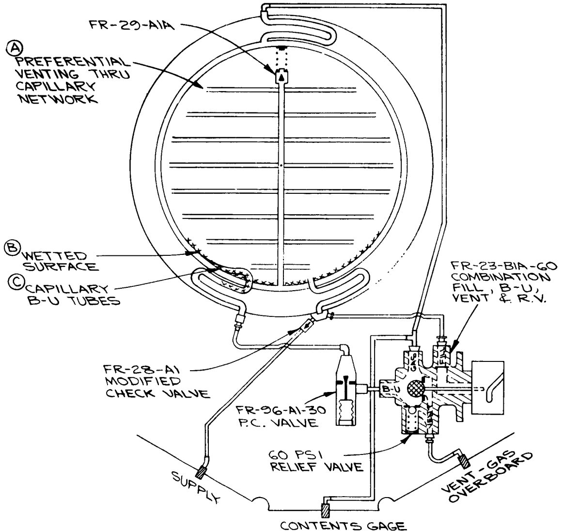
FIGURE 5 - CONVERTER SCHEMATIC
