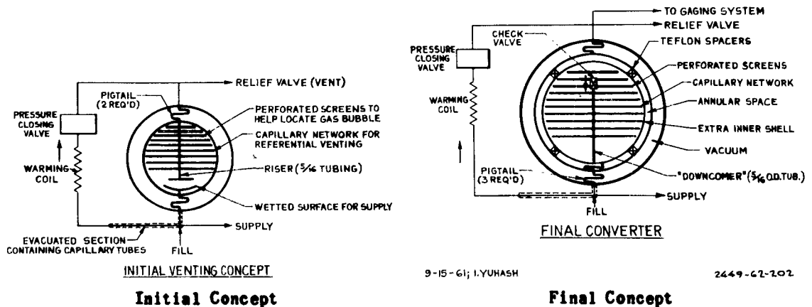
FIGURE 1 - VENTING CONCEPT
