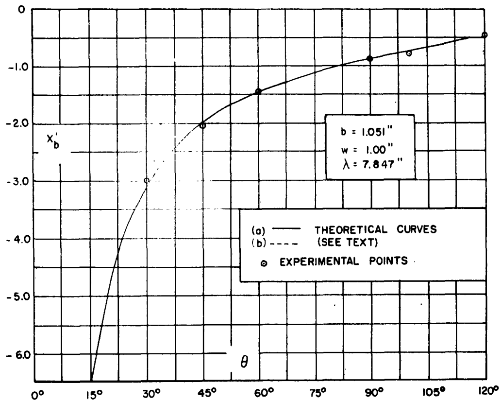
Fig. 8-53b. REACTANCE TEE NETWORK PARAMETERS FOR SHARP ANGLE BENDS
