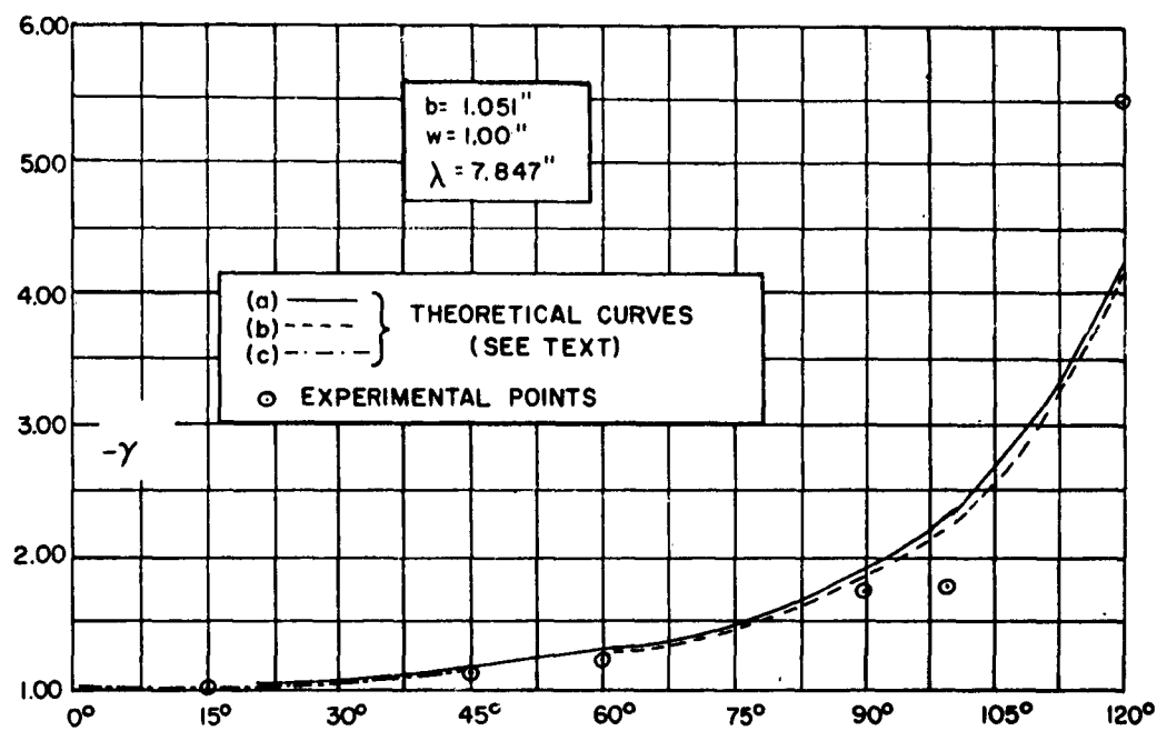
Fig. 8-54 a. TANGENT NETWORK PARAMETERS FOR SHARP ANGLE BENDS
