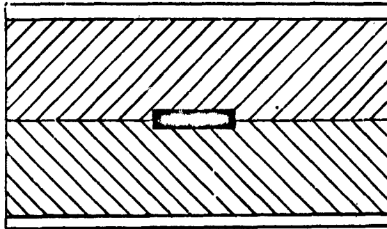
Fig 1-2 "Stripline Cross Section"
