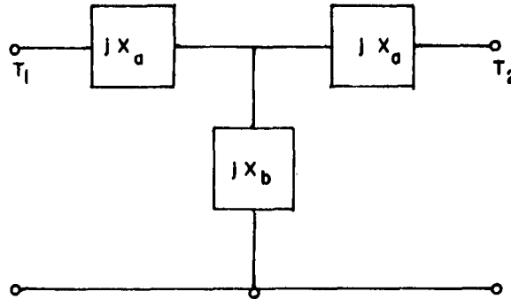
Fig. 8-9: Symmetric Tee Network
