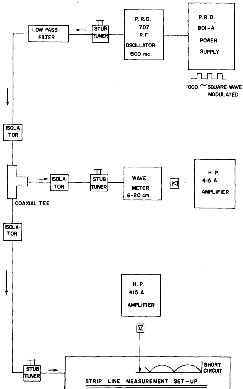
Fig. 8-30 BLOCK DIAGRAM OF MEASUREMENT EQUIPMENT
