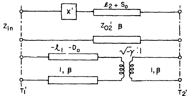
Fig. A11-2: Equivalent Tangent and Reactance Network Representation.
