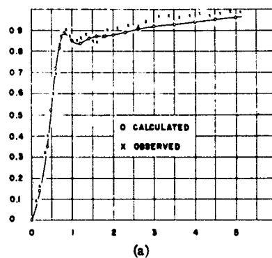
Fig. 10—Response of RG—8/u; A(100 \text{ mc}) = 0.0024 . (a) 150 \mu\text{s} of cable— \beta = 8.14 \times 10^{-11} second. (b) 250 \mu\text{s} of cable— \beta = 2.26 \times 10^{-10} second.
