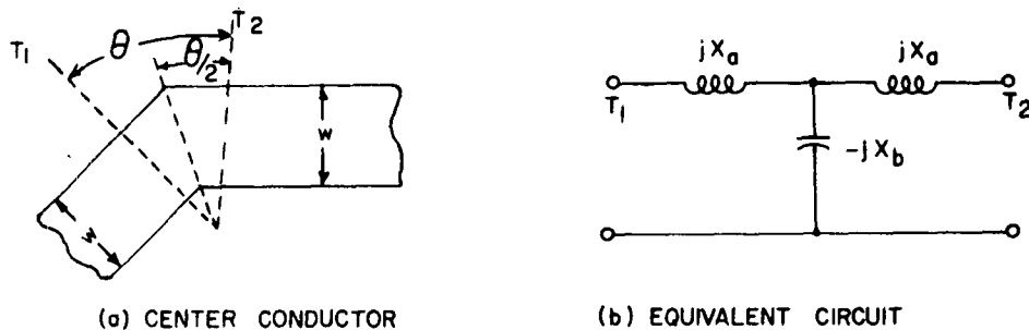
Fig. 8-24: Equivalent Circuit for a Sharp Bend of Any Angle in Stripline.
