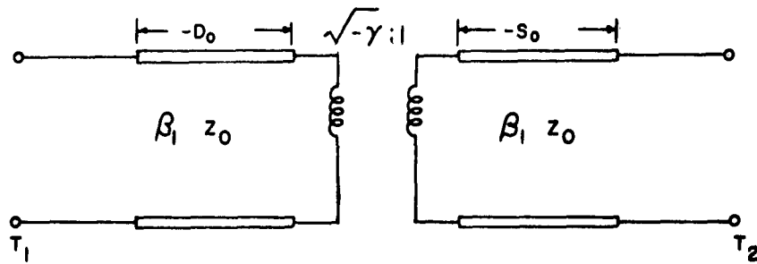
Fig. 8-8: Tangent Relation Network
