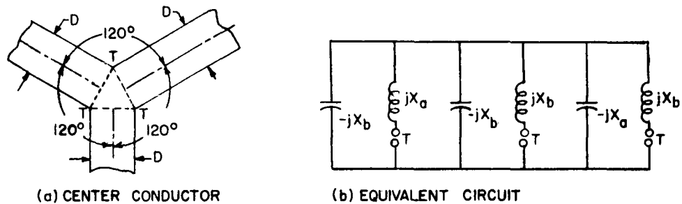
Fig. 8-27: Equivalent Circuit for a 120^\circ Y
