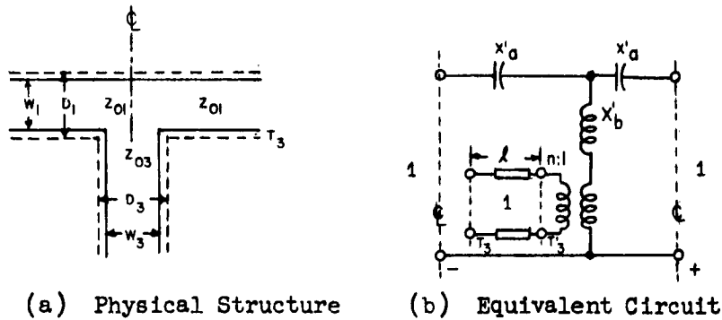
Fig. 8-29: Symmetric Tee Junction
