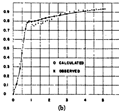
Fig. 11—Response of \frac{1}{4} inch Styroflex; A(100 \text{ mc}) = 0.00057 . (a) 150 \mu\text{s} of cable— \beta = 4.57 \times 10^{-11} second. (b) 250 \mu\text{s} of cable— \beta = 1.27 \times 10^{-11} second.
