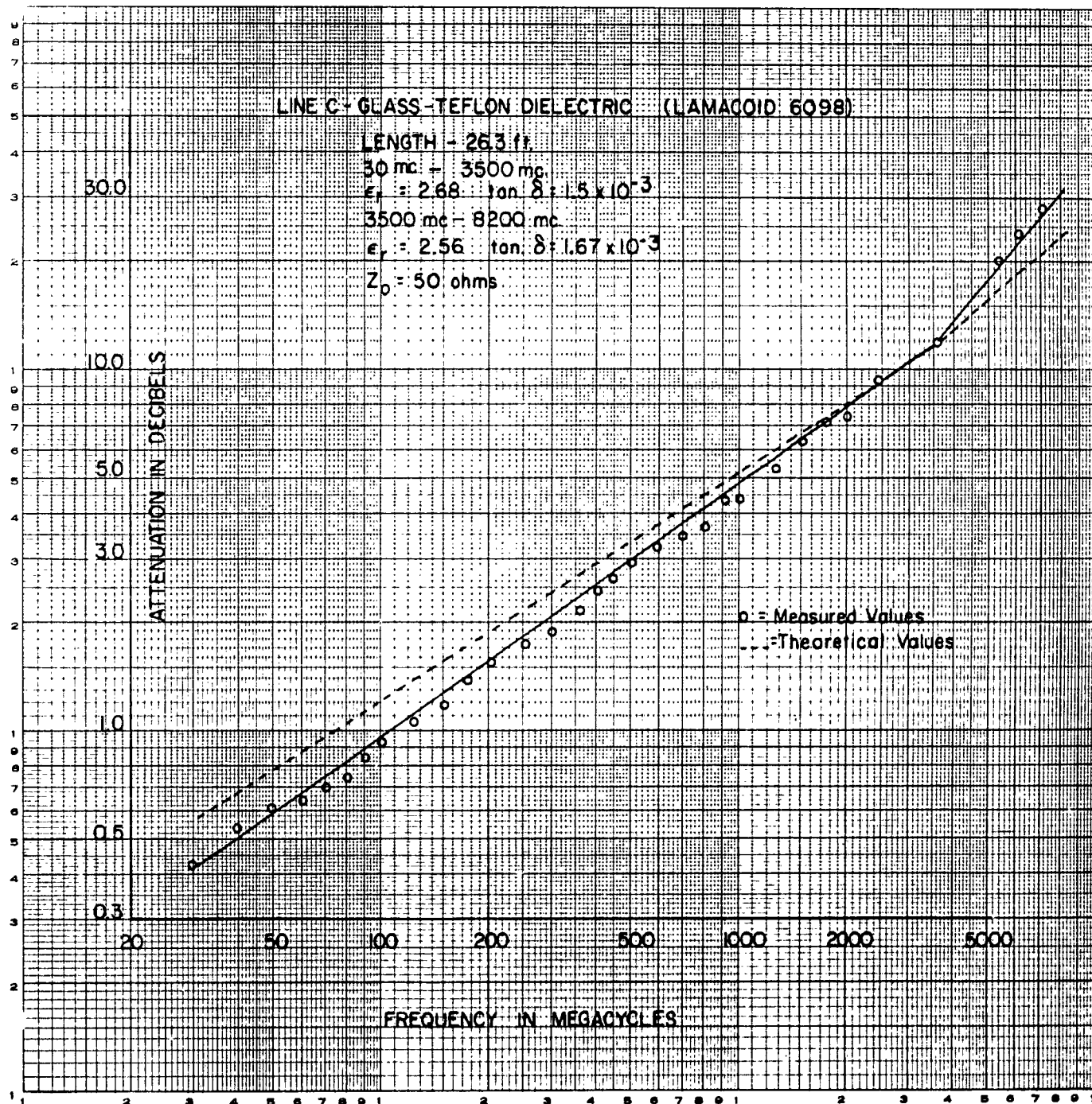
Fig. 4-9b. ATTENUATION MEASUREMENTS FOR LINE C
