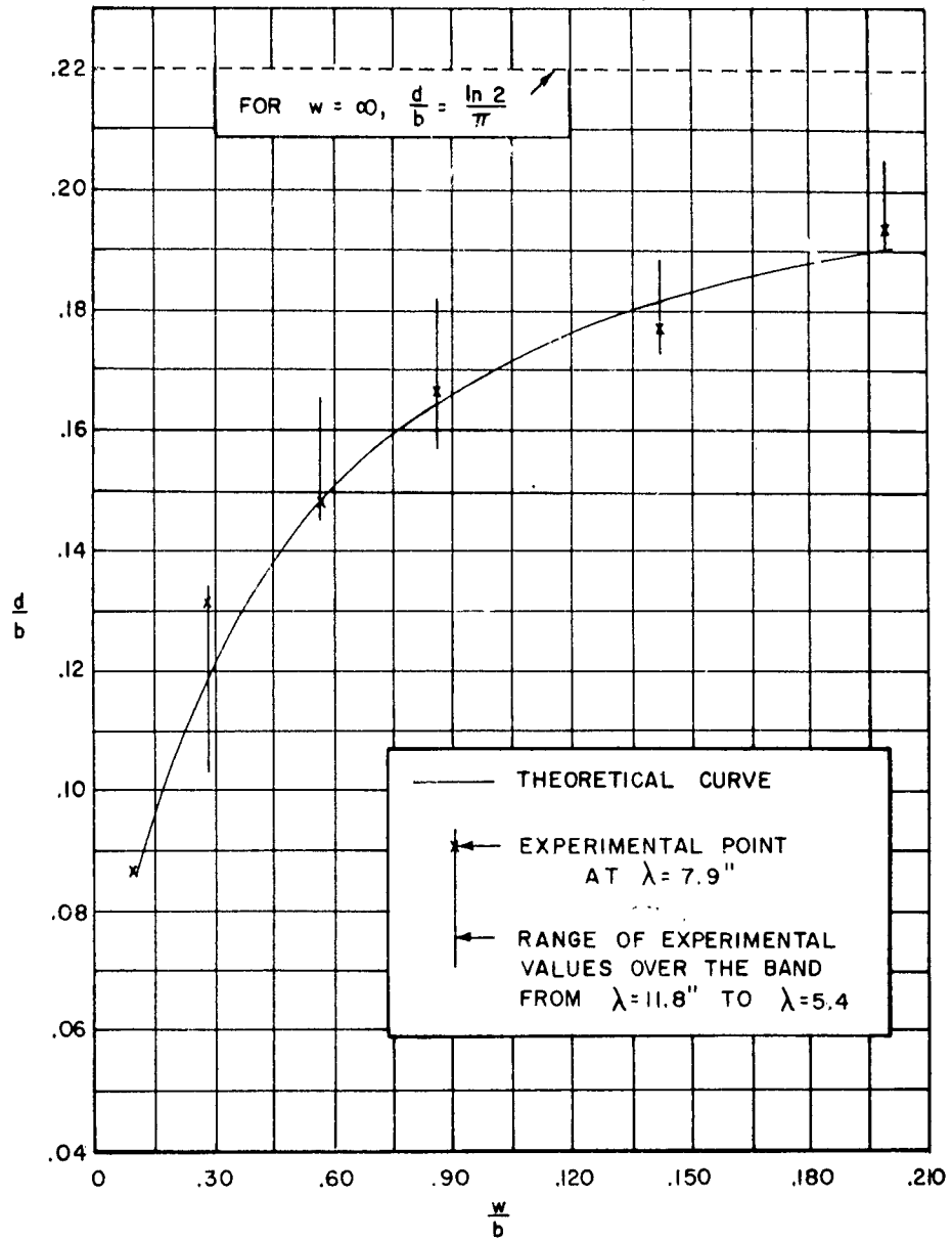
Fig.8-44.LOCATION OF EQUIVALENT OPEN CIRCUIT FOR ABRUPTLY-ENDED CENTER CONDUCTOR
