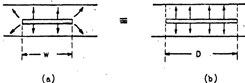
Fig 2-1 Treatment of the low Z_0 Range
