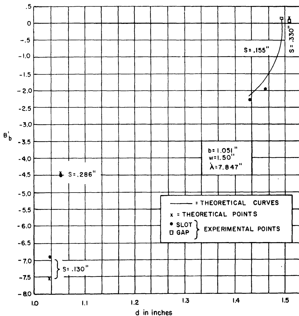
Fig. 8-41. CIRCUIT PARAMETERS OF SLOTS AND GAPS
