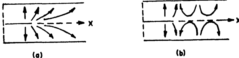
Fig. 9-7: Electric Field Lines for (a) a class of discrete modes, (b) a contribution to the continuous spectrum.
