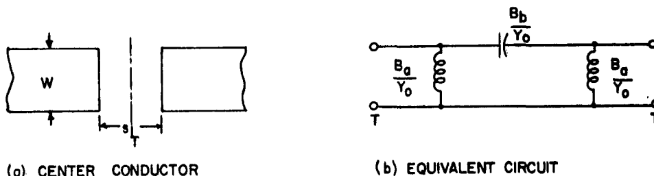
Fig. 8-14: Centerline Representations for a Gap in the Center Conductor of Stripline.
