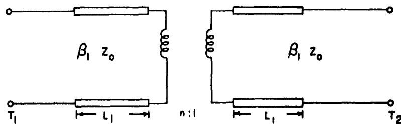
Fig. 8-7: Arbitrary Lossless Transformer Network.
