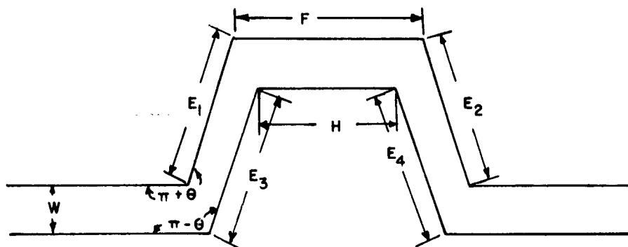
Fig. 51b. DISTANCES TO BE MEASURED FOR FOUR CORNERED BEND MEASUREMENT ( \theta \pm 90^\circ )
