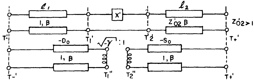
Fig. All-1: Tangent and Series Reactance Networks.
