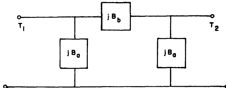
Fig. 8-10: Symmetric Pi Network
