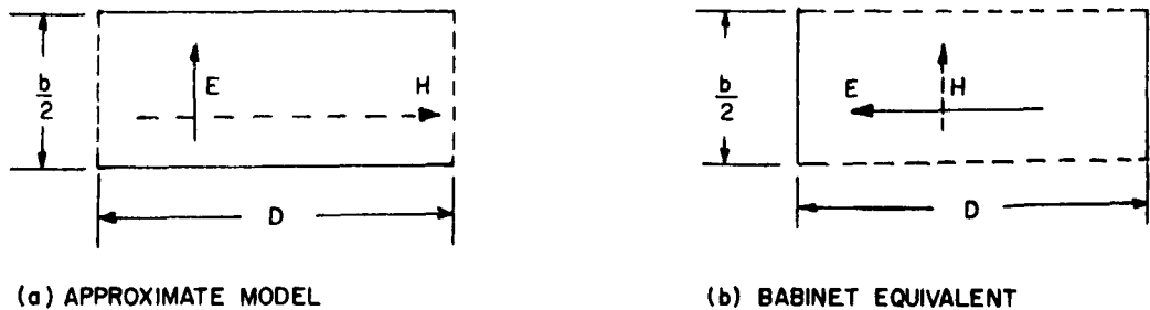
Fig. 8-20: The Stripline Approximate Model and Its Babinet Equivalent.
