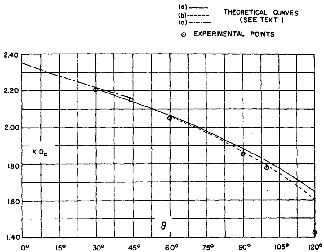
Fig. 8-54b. TANGENT NETWORK PARAMETERS FOR SHARP ANGLE BENDS
