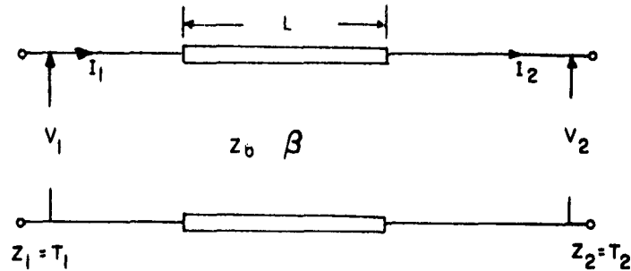
Fig. 8-3: Model of a Lossless Transmission Line.
