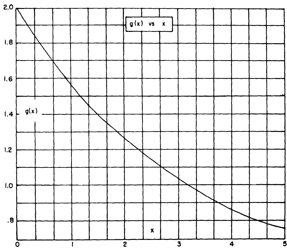
Fig.8-17. FUNCTIONS EMPLOYED IN SLOT FORMULAS
