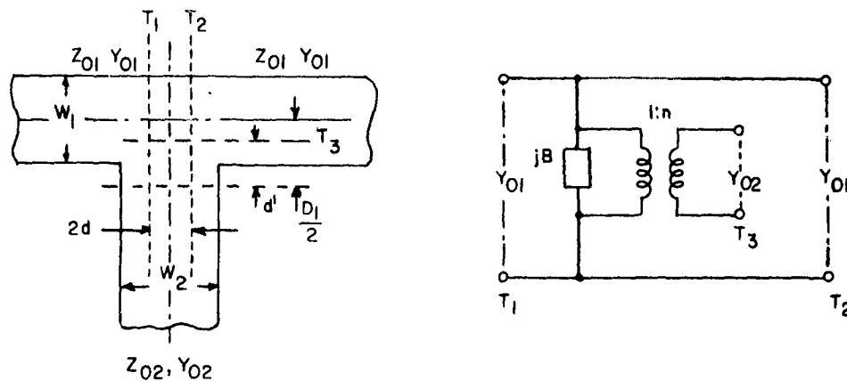
Fig. 8-29a: Recommended Equivalent Circuit for Stripline Tee Junction.
