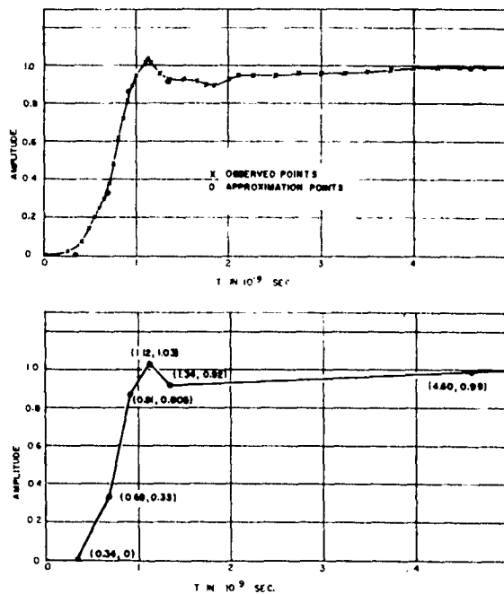
Fig. 7—Standard pulse and linear approximation.
