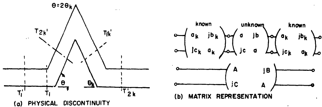
Fig. A13-1: Discontinuity Structure for the Study of Obtuse Angle Bends.
