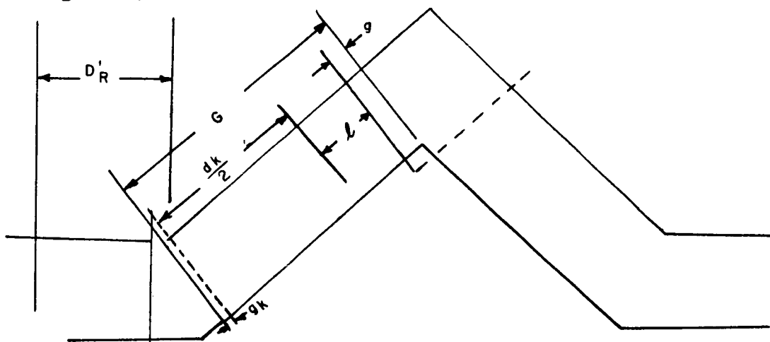
Fig. 8-54: Definition of D_R , d_k , g_k for Three Cornered Bend Measurement.
