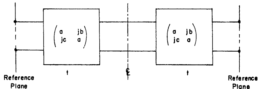
Fig. 8-2: Center Line of Symmetry for Two Cascaded Sections.
