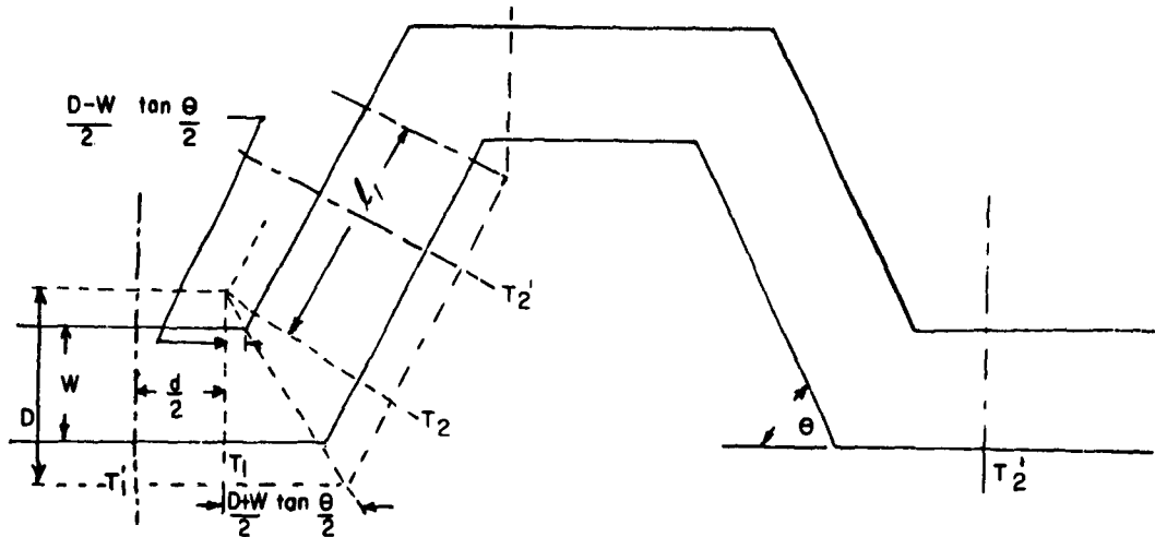
Fig. 8-51a: Four-Cornered Sharp Angle Bend in the Center Conductor.
