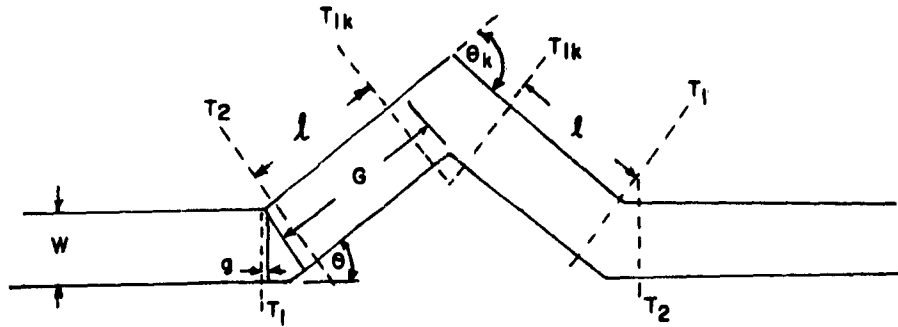
Fig. 8-52a: Three Cornered Bend in the Center Conductor ( \theta < 90^\circ ).
