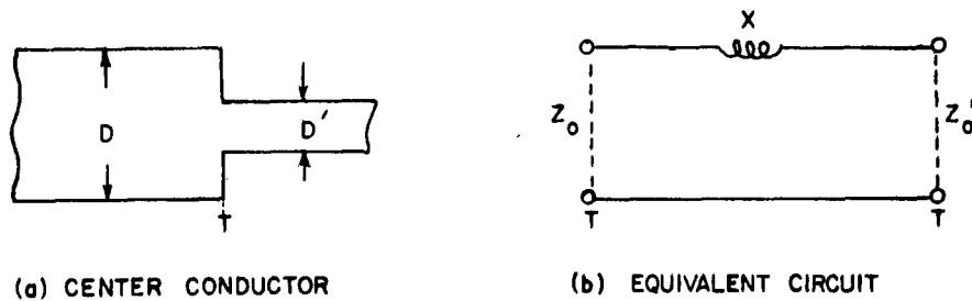
Fig. 8-28: Equivalent Circuit for a Sudden Change in Center Strip Width.
