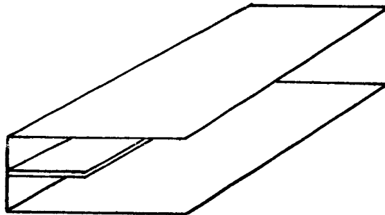
Fig. 9-9: The Trough Waveguide (A.I.L.)
