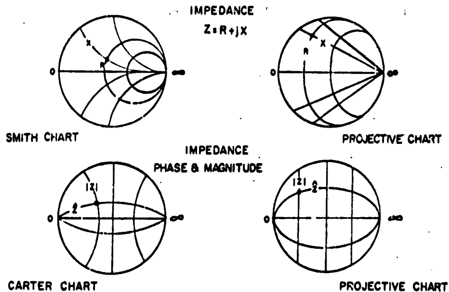
Fig 3-4 Loci on the projective chart and on the Smith and Carter Charts of constant resistance R , reactance X , impedance magnitude |Z| and impedance phase \phi .
