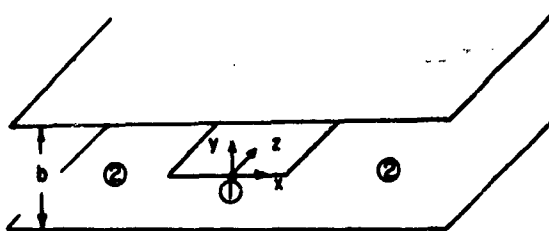
Fig. 9-8: Stripline Geometry.
