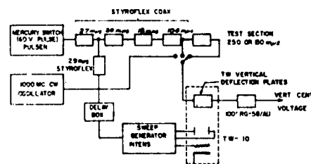
Fig. 6—Cable comparison test circuit.
