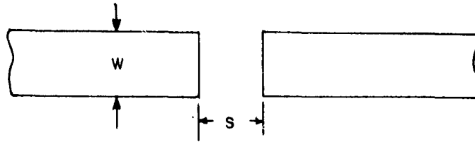
Fig. 8-13: Gap in Inner Conductor of Stripline.
