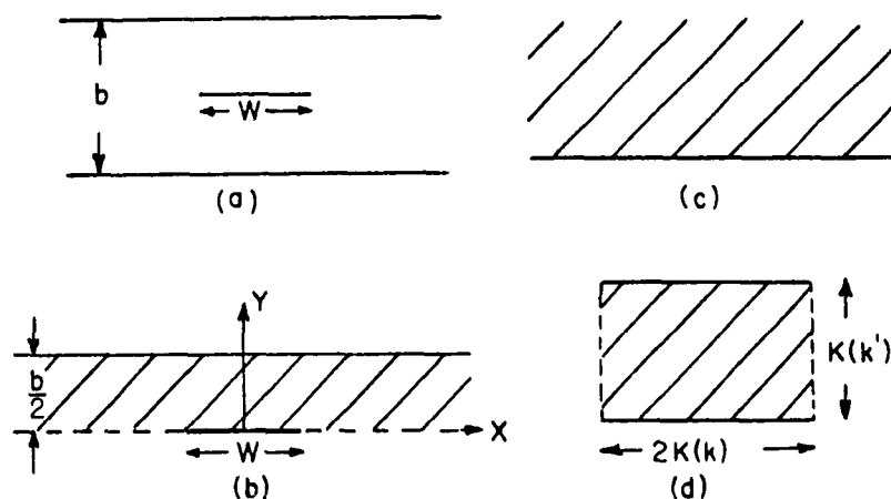
Fig 4-1 - Rigorous Conformal Mapping of Stripline Geometry
