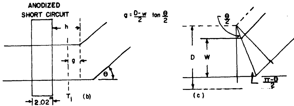
Figs. 8-52b and c: Definitions of D_R ; g for Three Cornered Bend Measurements ( \theta < 90^\circ ).
