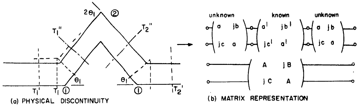
Fig. A12 - 1: Discontinuity Structure for Study of Acute Angle Bends.
