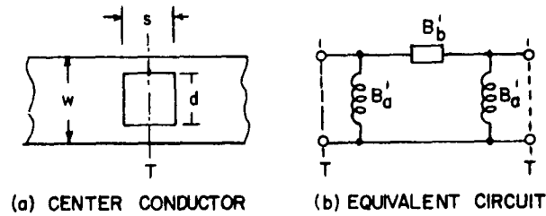
Fig. 8-15: Slot in Center Conductor (a) Physical Structure
