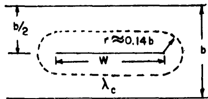
Fig. 9-6: Approximate Rule for Determining \lambda_c in Stripline.
