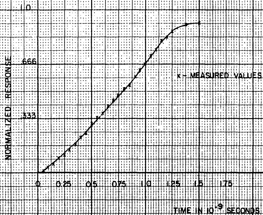
Fig. 5-6 THEORETICAL TRANSIENT RESPONSE FOR A STRIPLINE SPIRAL
