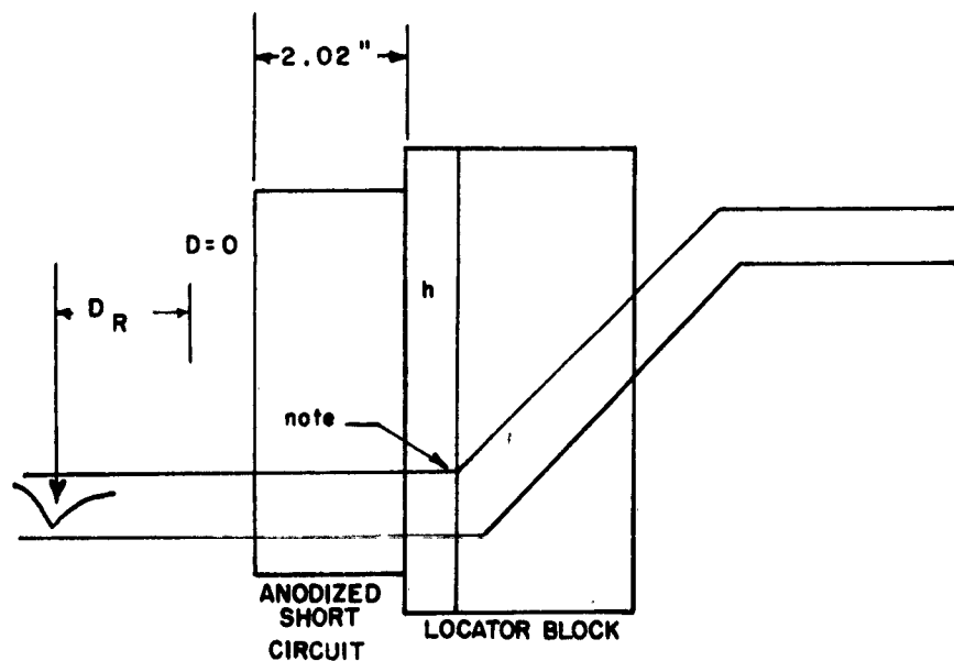
Fig. 51c. DEFINITION OF D_R FOR FOUR CORNERED BEND MEASUREMENT ( \theta \pm 90^\circ )
