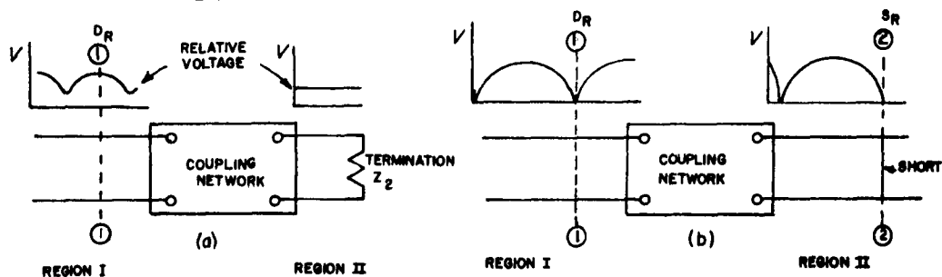
Fig. 8-33: Procedure for choosing reference planes in the two regions, (a) the network is perfectly terminated, (b) region II is shorted.
