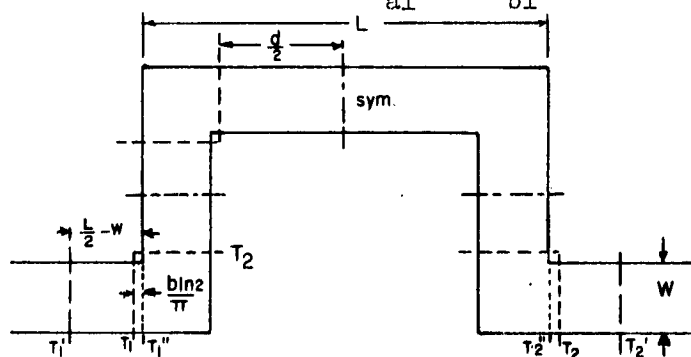
Fig. 8-48: Right Angle Bend in Center Conductor
