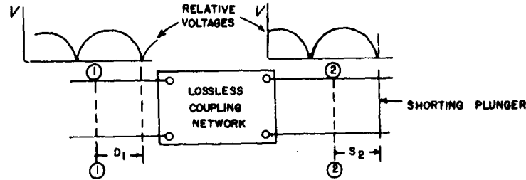
Fig. 8-34: Distribution of electric field on the two sides of the coupling network due to the shorting plunger in region II.
