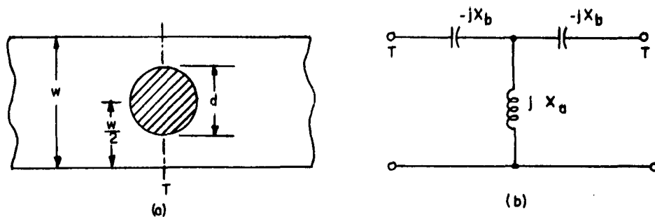
Fig. 8-19: Centerline Representation for a Round Centered Conducting Vertical Post in Stripline.
