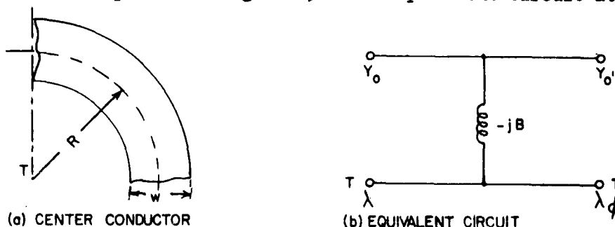
Fig. 8-25: Equivalent Circuit for
