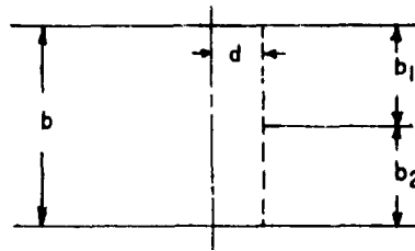
Fig. 9-2: Side View of an E-Plane Bifurcation in Waveguide.
