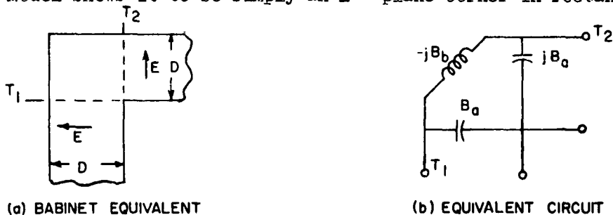
Fig. 8-22: Babinet Equivalent of a Right Angle
