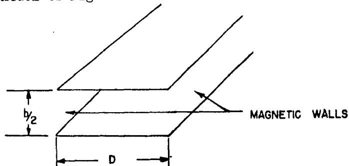
Fig. 8-12: Approximate Model of Stripline.
