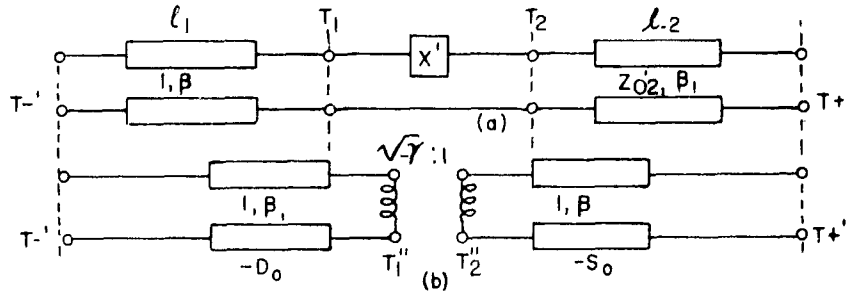
Fig. 8-45: Tangent and Series Reactance Networks.
