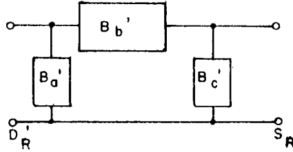
Fig. 8-39: Generalized Equivalent Pi Network.
