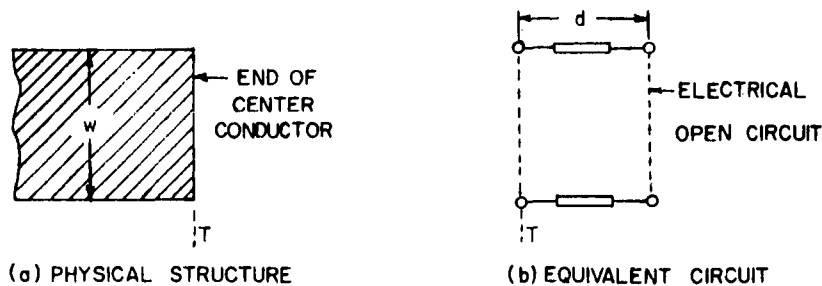
Fig. 8-29f: Abruptly Ended Center Conductor
