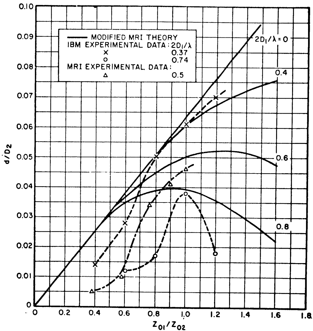
Fig.8-29d Comparison between available experimental data and theory for parameter d , the reference plane shift in the main arms.
