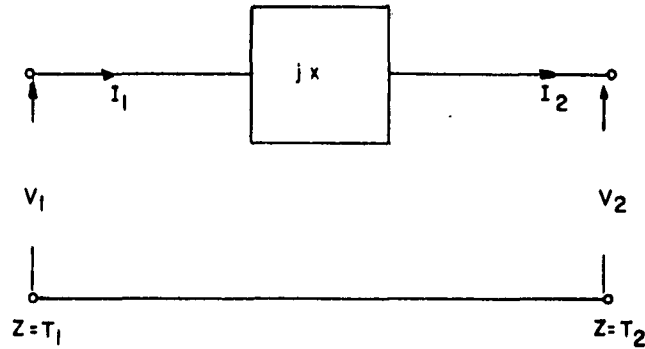
Fig. 8-5: Model of a Pure Series Reactance.
