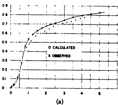
Fig. 8—Response of RG—58 A/u; A(100 \text{ mc}) = 0.056 . (a) 150 \mu\text{s} of cable— \beta = 4.50 \times 10^{-10} second. (b) 250 \mu\text{s} of cable— \beta = 1.25 \times 10^{-9} second.
