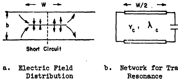
Fig. 9-1: First Higher Mode in Stripline
