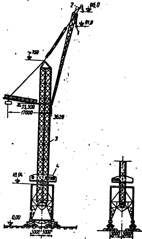
Fig. 1. Diagram of BK-1425 Crane. 1--Main hook; 2--Auxillary hook; 3--Revolving turret; 4--machine section.
