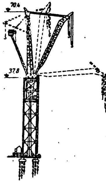
Fig. 7. Tower crane, used in construction of blast furnace in Newcastle.
