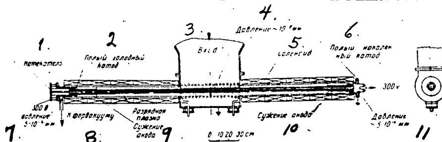
Fig.2. Powerful ion pump with incandescent cathode; mode of operation - forcing out the gas. 1-flow holder; 2-hollow cold cathode; 3-input; 4-pressure \sim 10^{-6} mm 5-solenoid; 6-hollow incandescent cathode; 7-pressure 5 \cdot 10^{-6} mm ; 8-to forevacuum; 9-discharge plasma, narrowing of anode; 10- narrowing of anode; 11-pressure 5 \cdot 10^{-4} mm.
