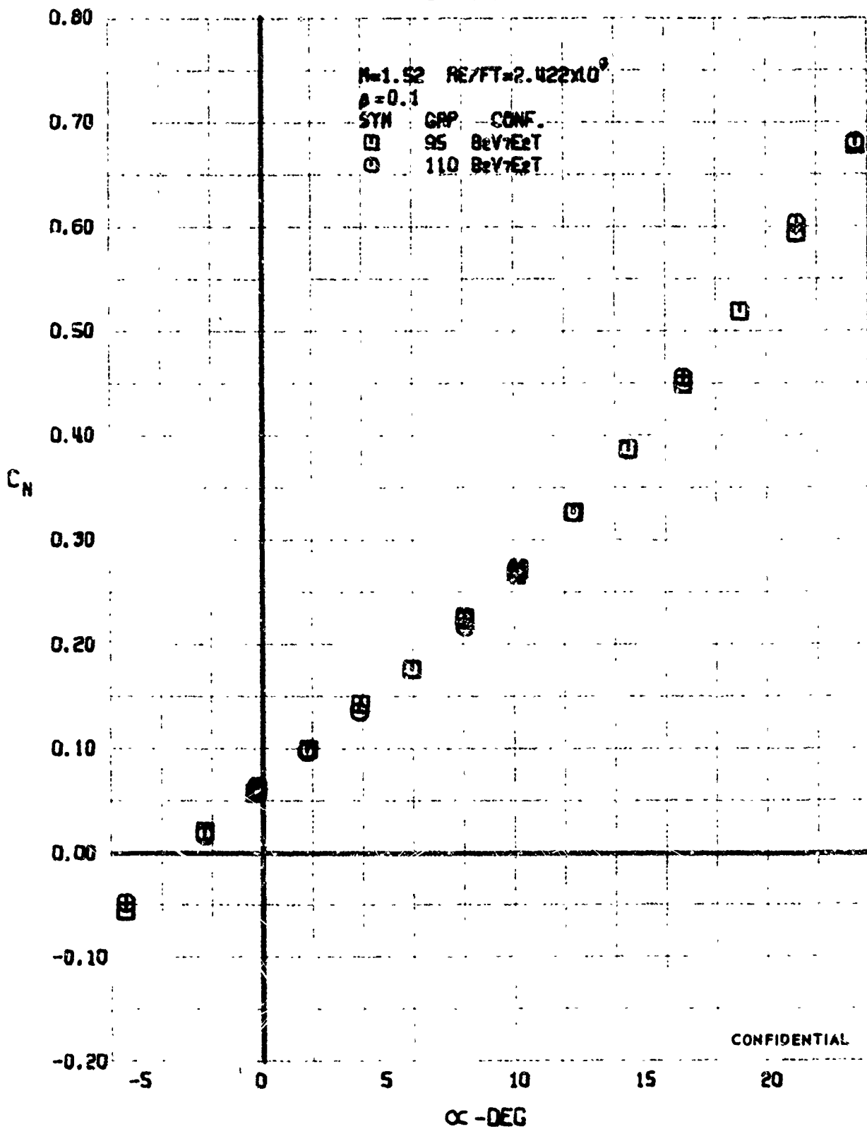
FIGURE 54 (U) REPENTABILITY - NORMAL FORCE COEFFICIENT VARIATION WITH ANGLE OF ATTACK ( M=1.52 )
