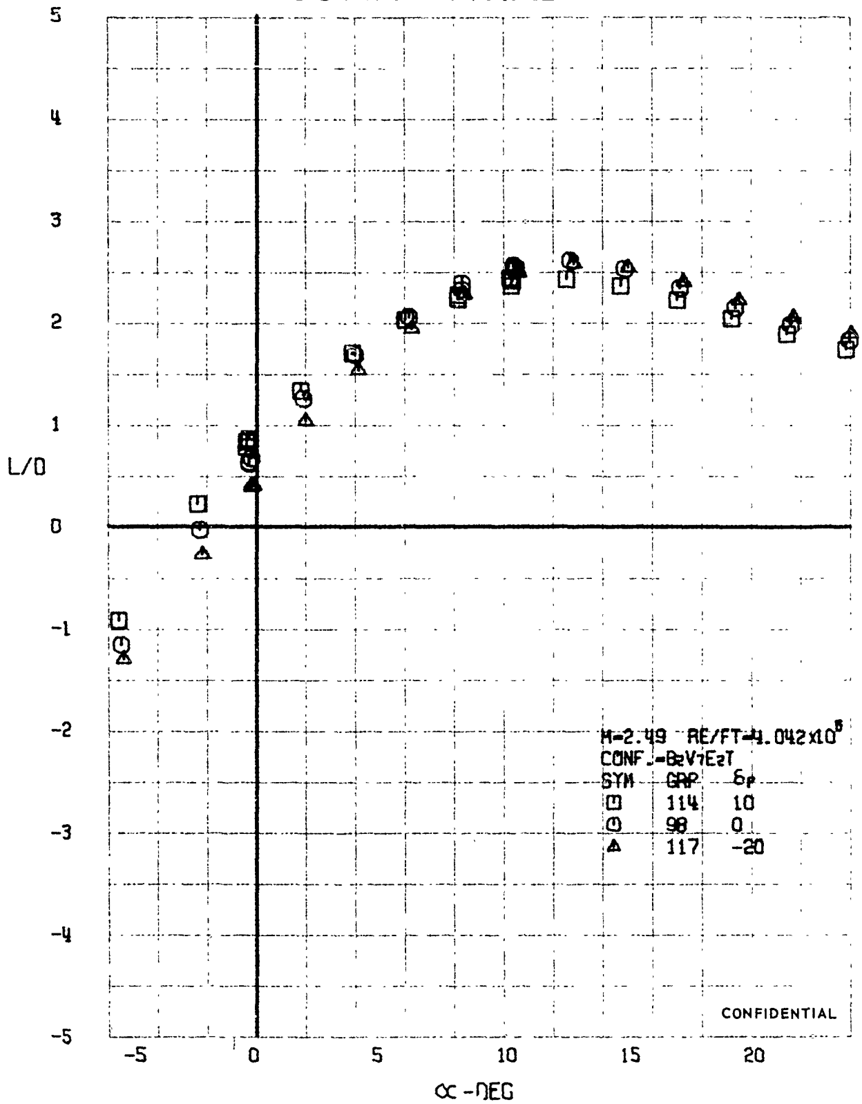
FIGURE 127 (U) ELEVON EFFECTS - LIFT-DRAG RATIO VARIATION WITH ANGLE OF ATTACK (M=2.49)
