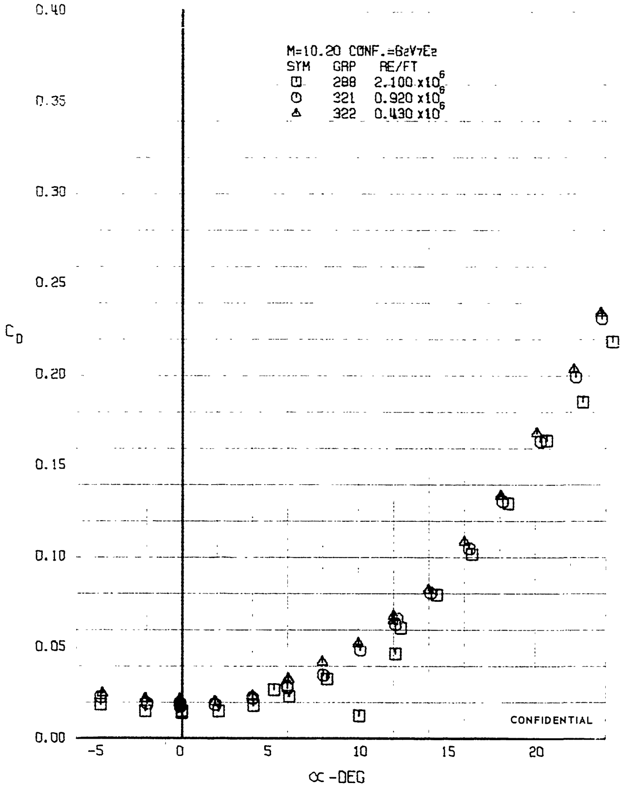
FIGURE 286 (U) REYNOLDS NUMBER EFFECTS - DRAG COEFFICIENT VARIATION WITH ANGLE OF ATTACK (M=10.20)
