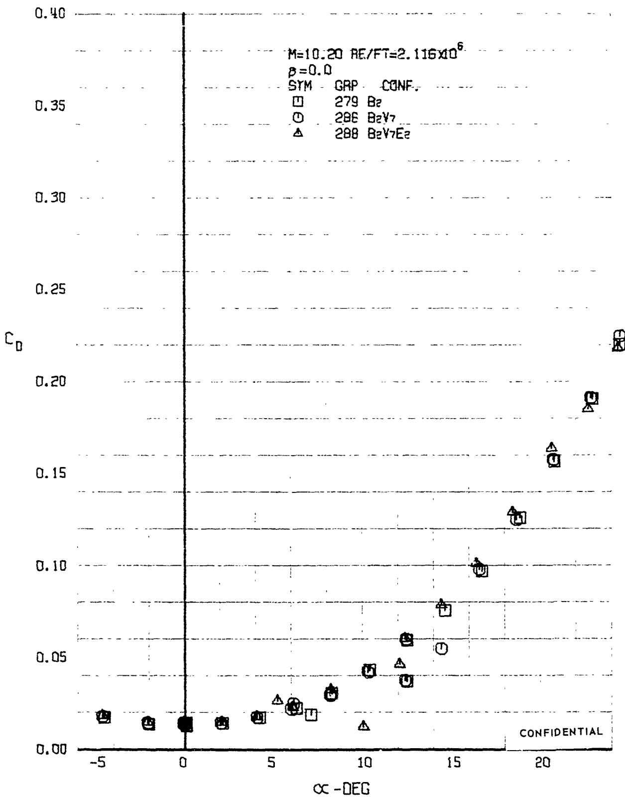
FIGURE 246 (U) CONFIGURATION BUILDUP - DRAG COEFFICIENT VARIATION WITH ANGLE OF ATTACK (M=10.20)
