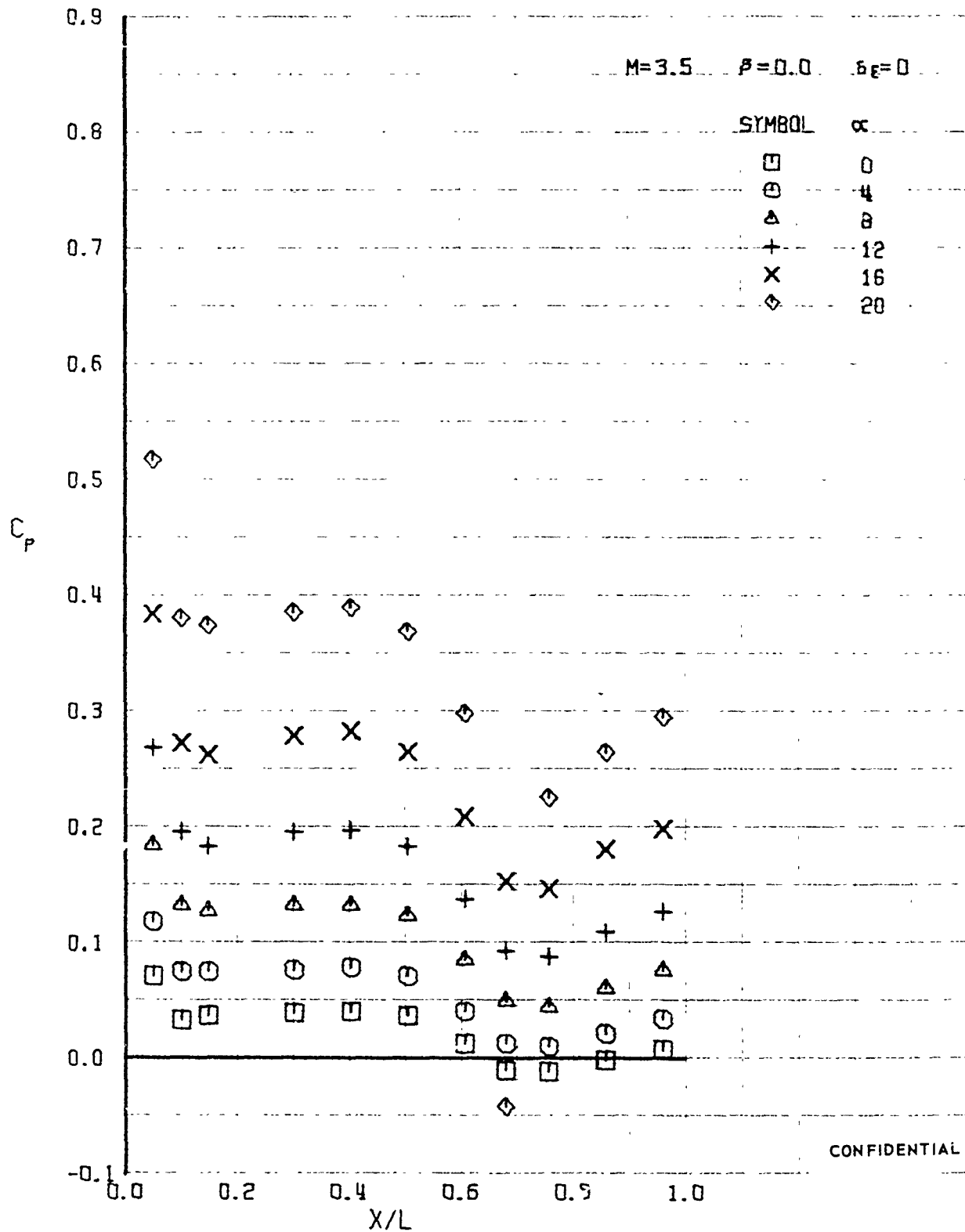
FIGURE 364 (U) LOWER SURFACE CENTERLINE PRESSURES
