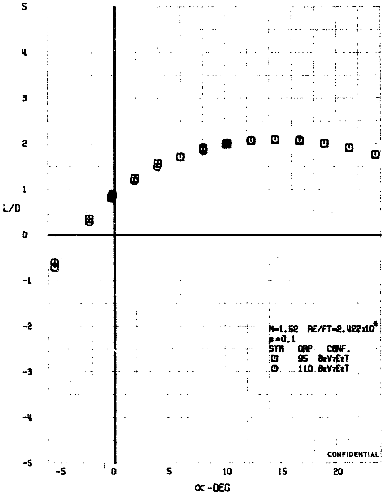
FIGURE 56 (U) REPEATABILITY - LIFT-DRAGE RATIO VARIATION WITH ANGLE OF ATTACK (M=1.52)
