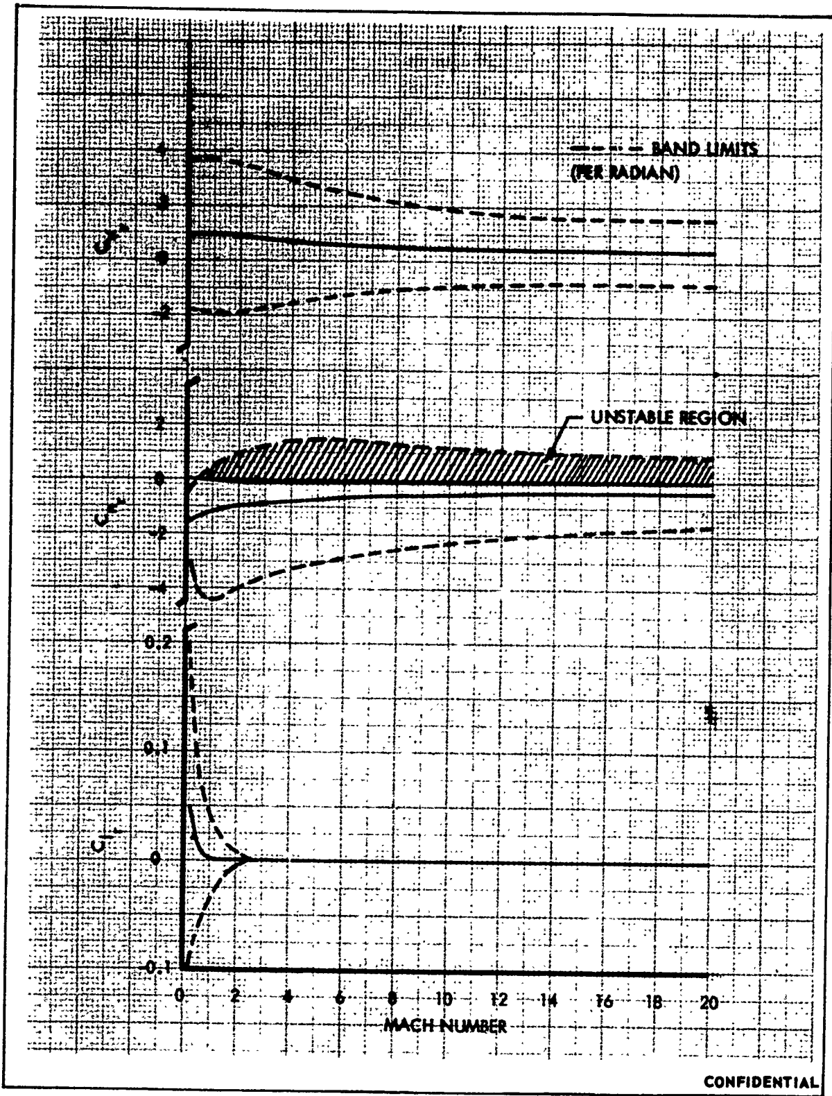
FIGURE 495 (U) VARIATION OF r DERIVATIVES WITH MACH NUMBER
