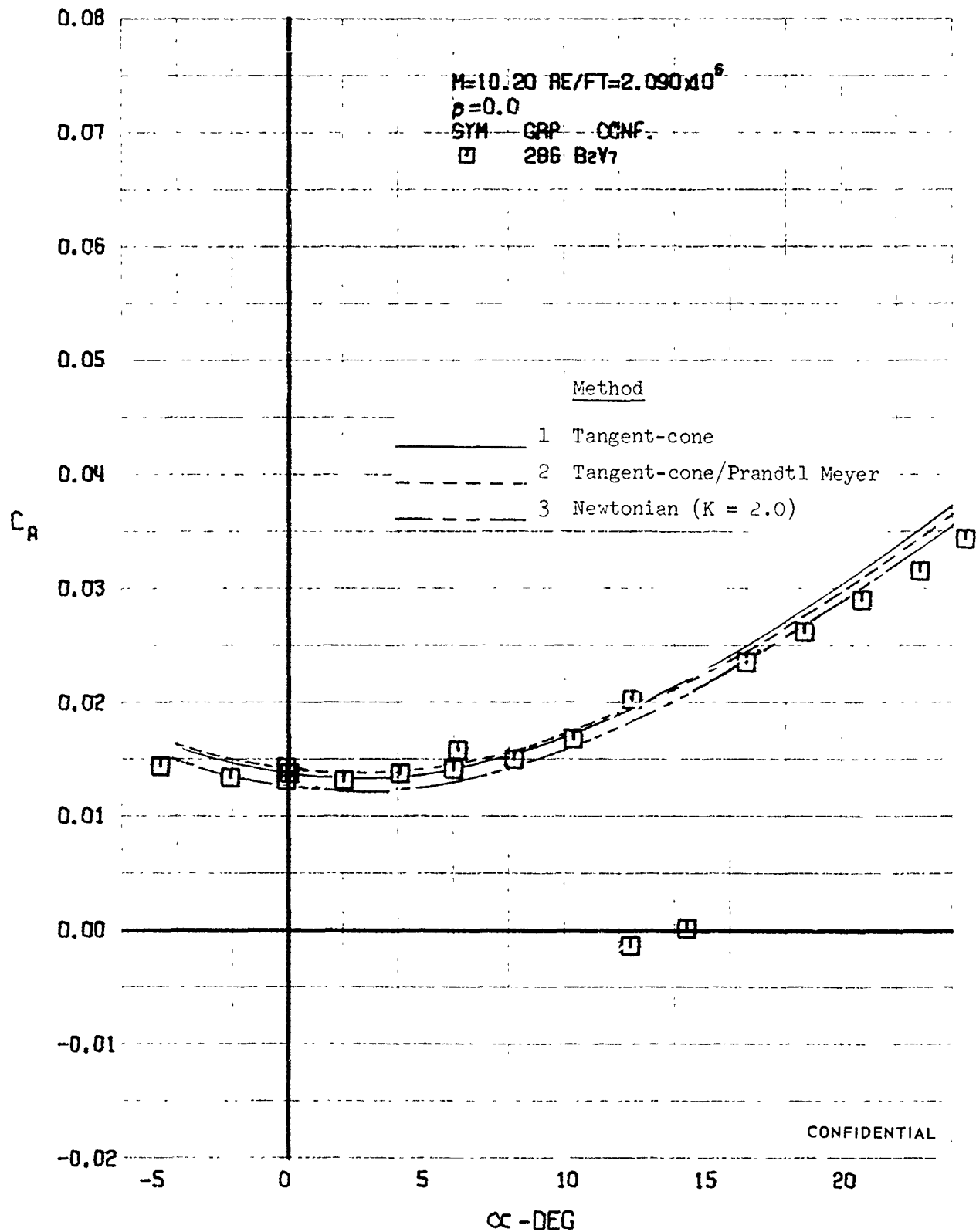
FIGURE 415 (U) COMPARISON OF ESTIMATED AND EXPERIMENTAL COEFFICIENTS - AXIAL FORCE COEFFICIENT VARIATION WITH ANGLE OF ATTACK ( M=10.20 )
