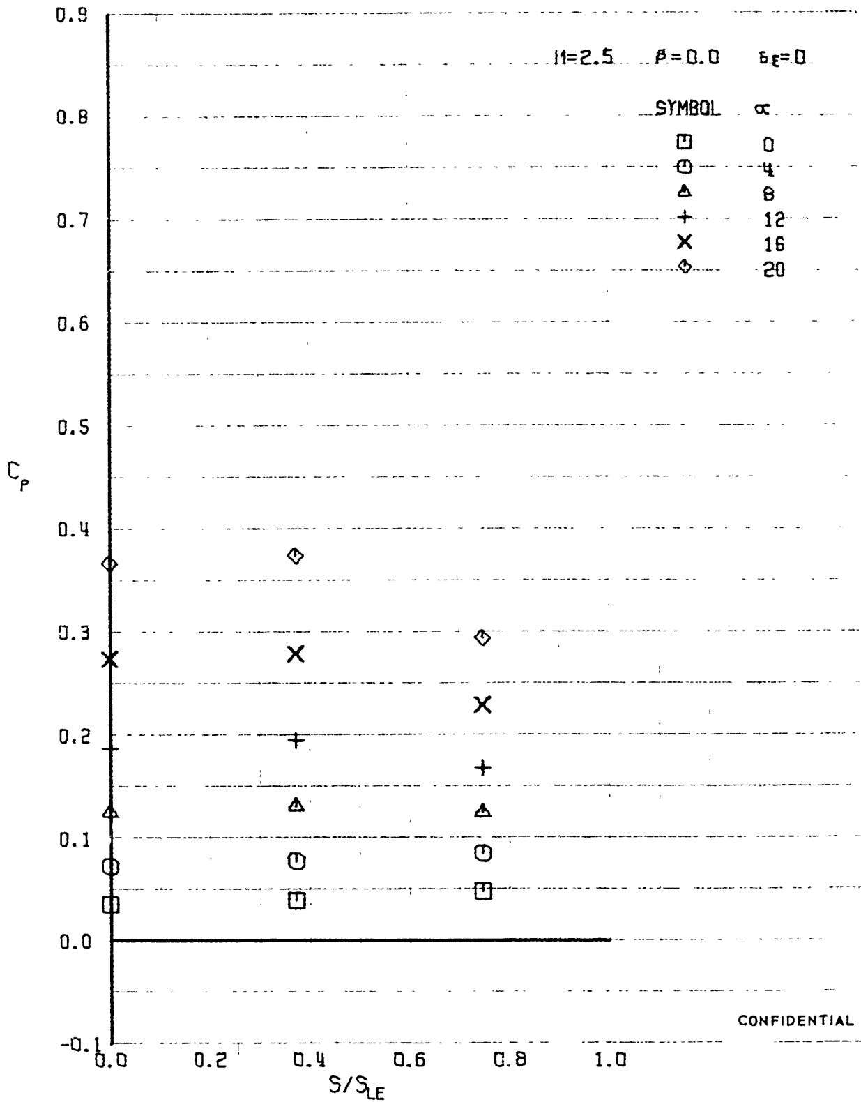
FIGURE 352 (U) LOWER SURFACE SPANWISE PRESSURES AT X/L = 0.15
