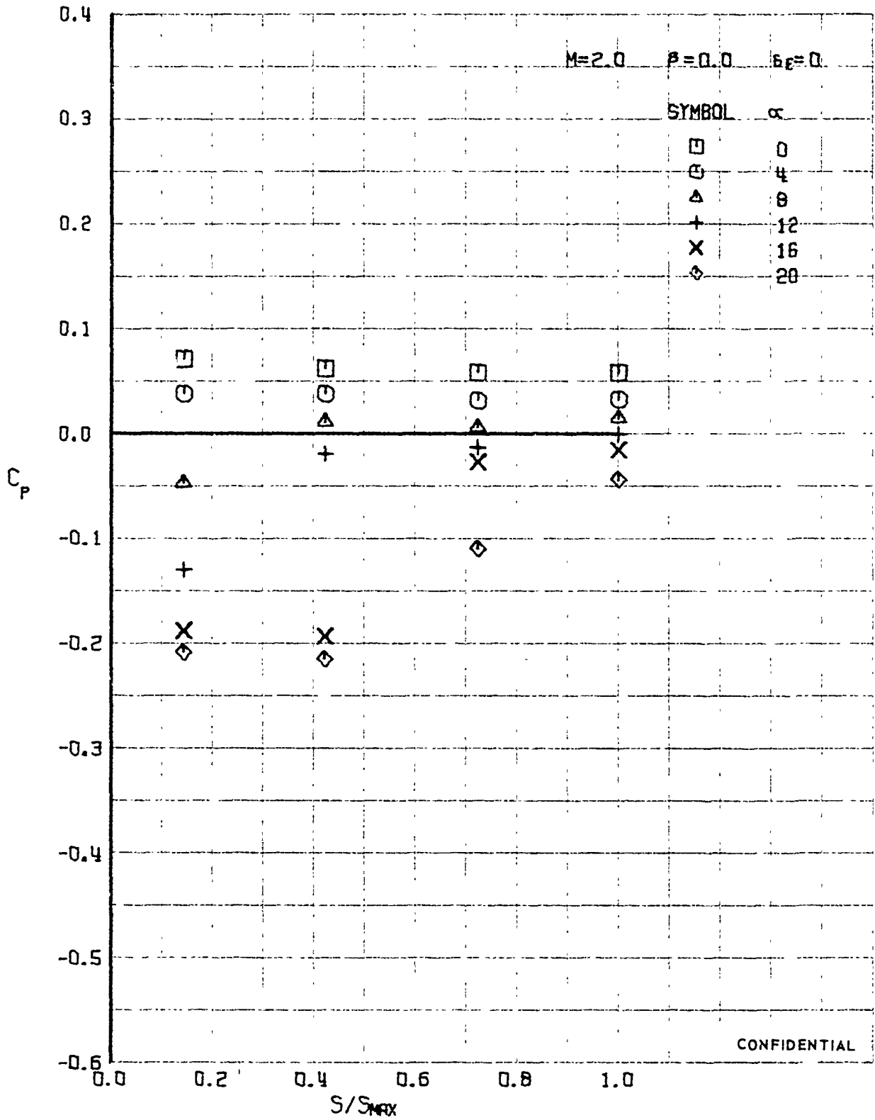
FIGURE 345 (U) UPPER SURFACE SPANWISE PRESSURES AT X/L = 0.15
