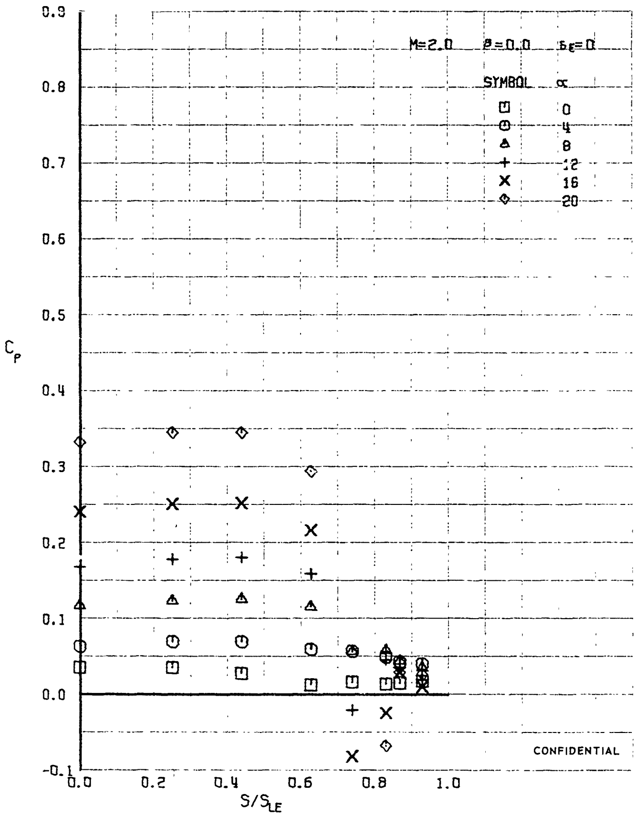
FIGURE 343 (U) LOWER SURFACE SPANWISE PRESSURES AT X/L = 0.96
