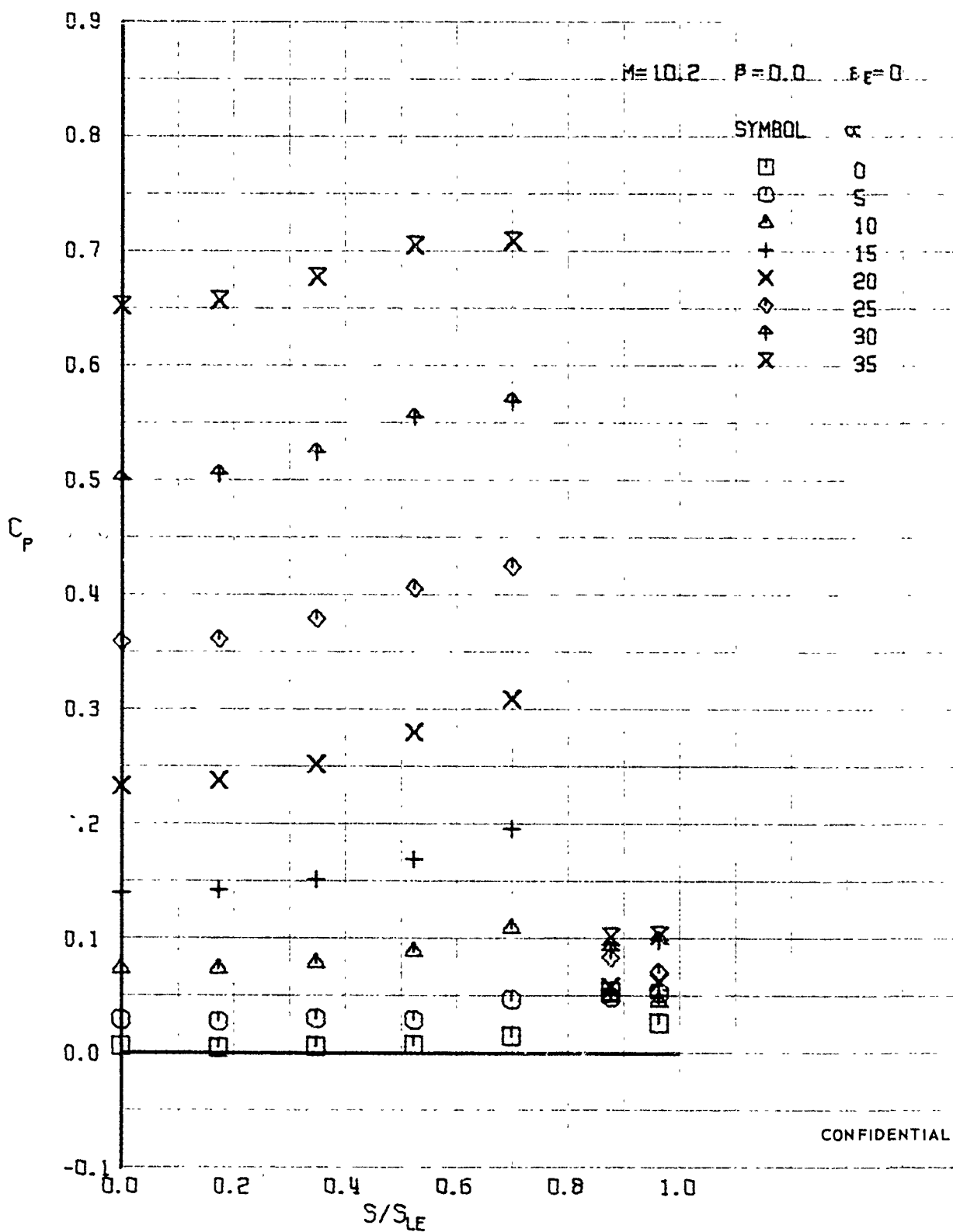
FIGURE 394 (U) LOWER SURFACE SPANWISE PRESSURES AT X/L = 0.76
