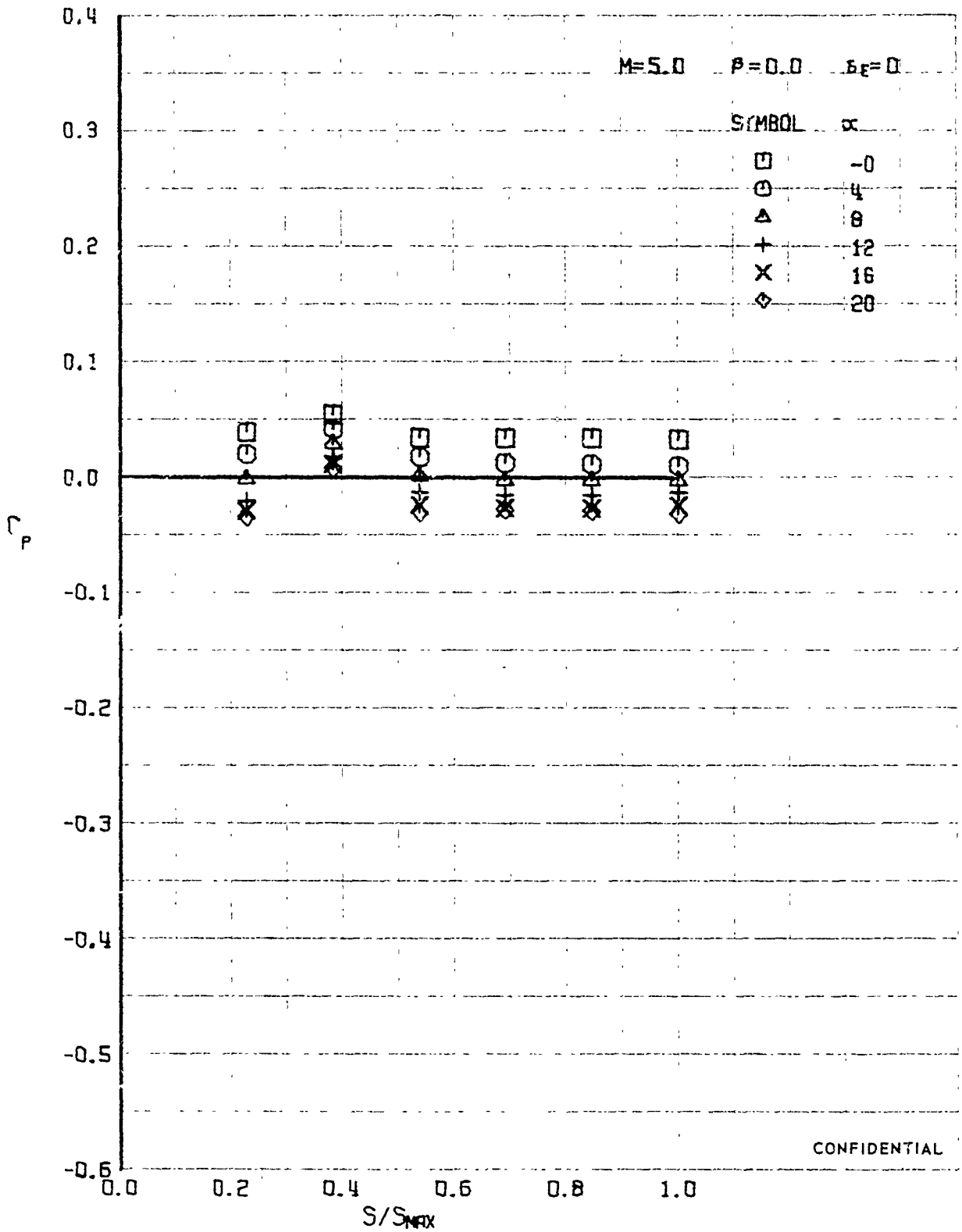
FIGURE 385 (U) UPPER SURFACE SPANWISE PRESSURES AT X/L = 0.30
