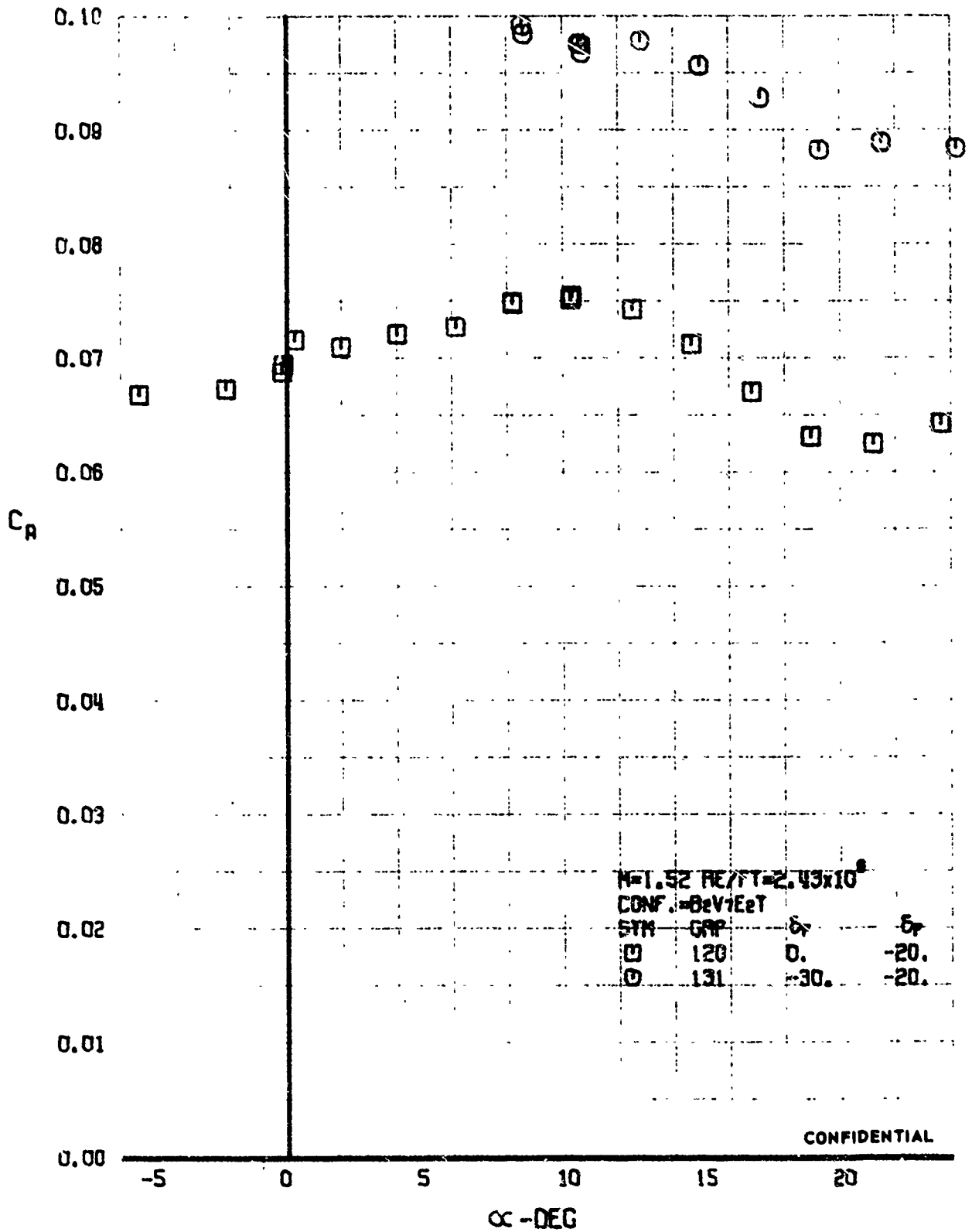
FIGURE 42 (U) FLAP EFFECTS - AXIAL FORCE COEFFICIENT VARIATION WITH ANGLE OF ATTACK ( M=1.52 )
