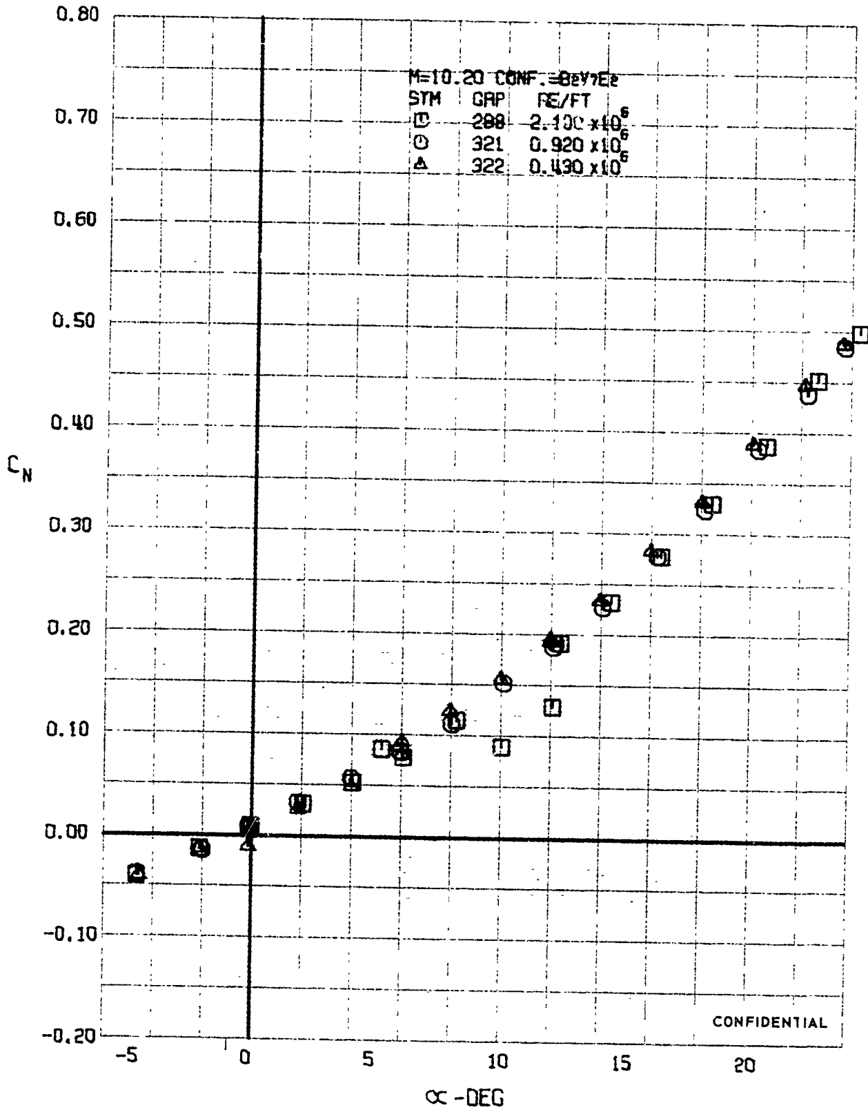
FIGURE 282 (U) REYNOLDS NUMBER EFFECTS - NORMAL FORCE COEFFICIENT VARIATION WITH ANGLE OF ATTACK (M=10.20)
