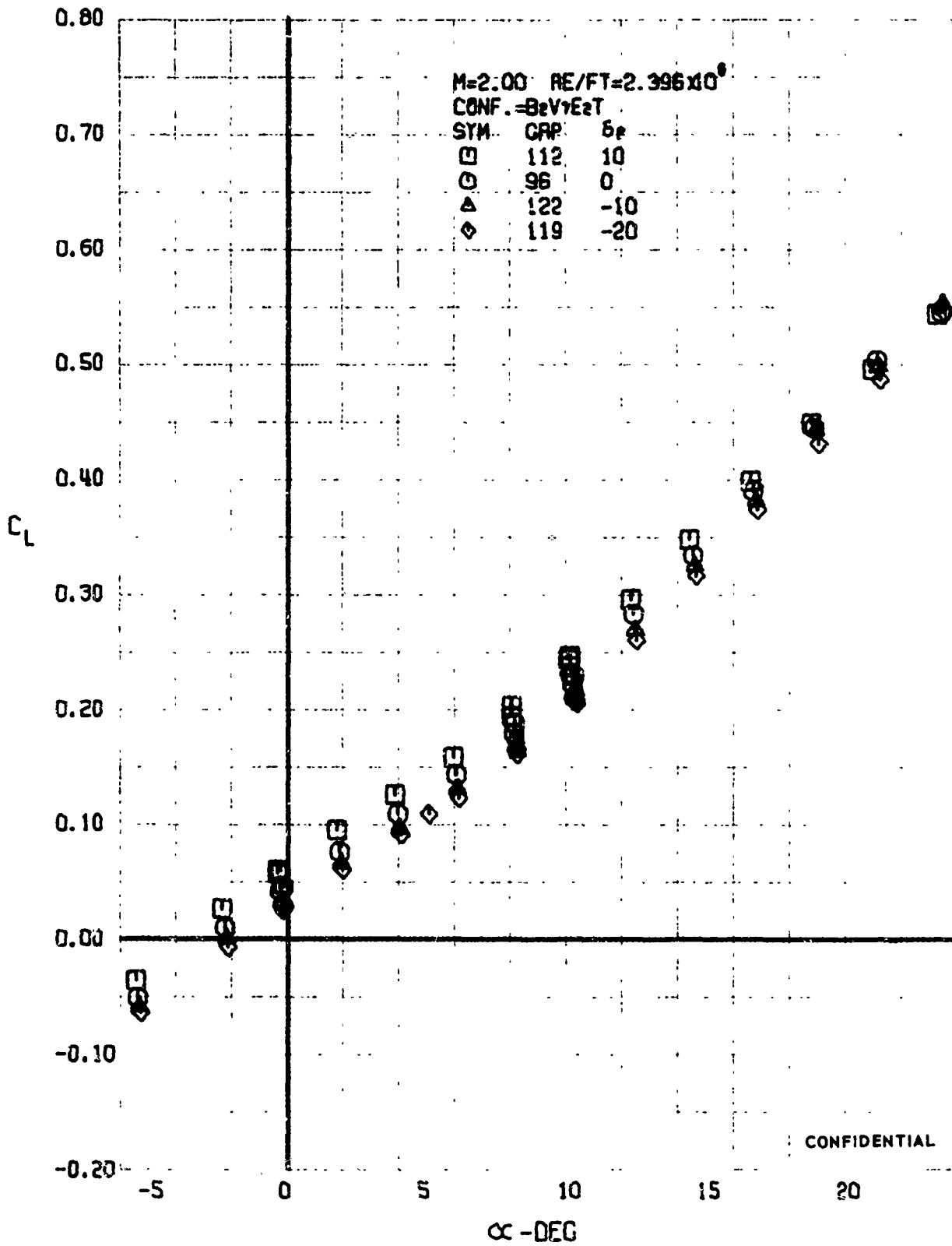
FIGURE 71 (U) ELEVON EFFECTS - LIFT COEFFICIENT VARIATION WITH ANGLE OF ATTACK (M=2.00)
