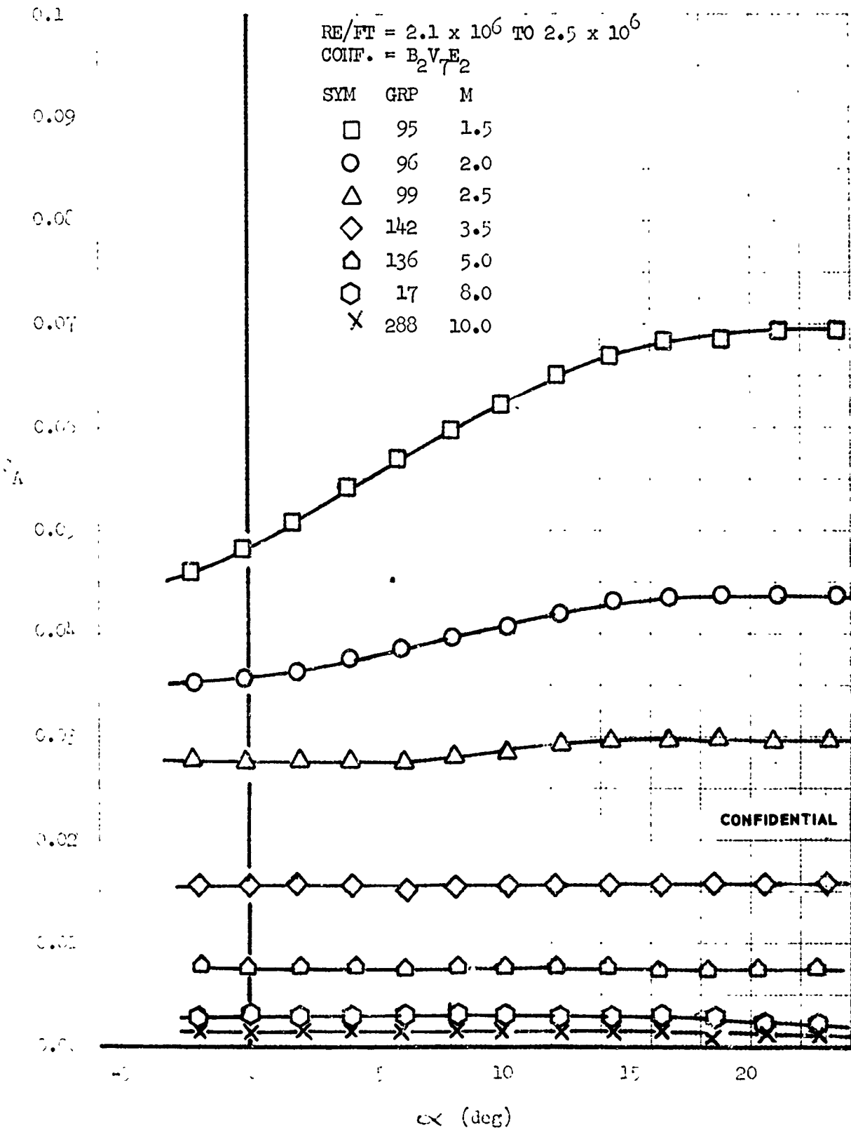
FIGURE 16 (U) BASE AXIAL FORCE - AXIAL FORCE COEFFICIENT VARIATION WITH ANGLE OF ATTACK
