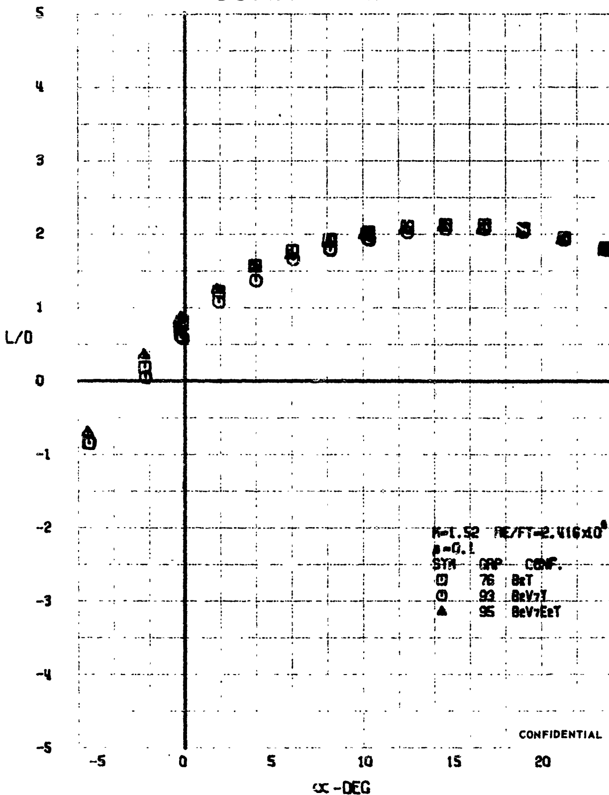
FIGURE 22 (U) CONFIGURATION BUILDUP - LIFT-DRAGE RATIO VARIATION WITH ANGLE OF ATTACK ( M=1.52 )
