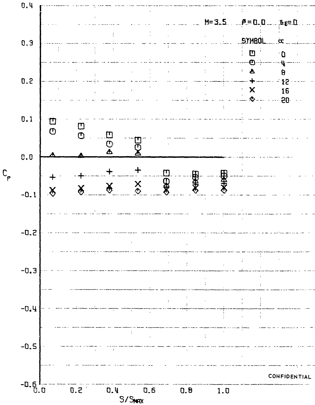
FIGURE 37 b (U) UPPER SURFACE SPANWISE PRESSURES AT X/L = 0.76
