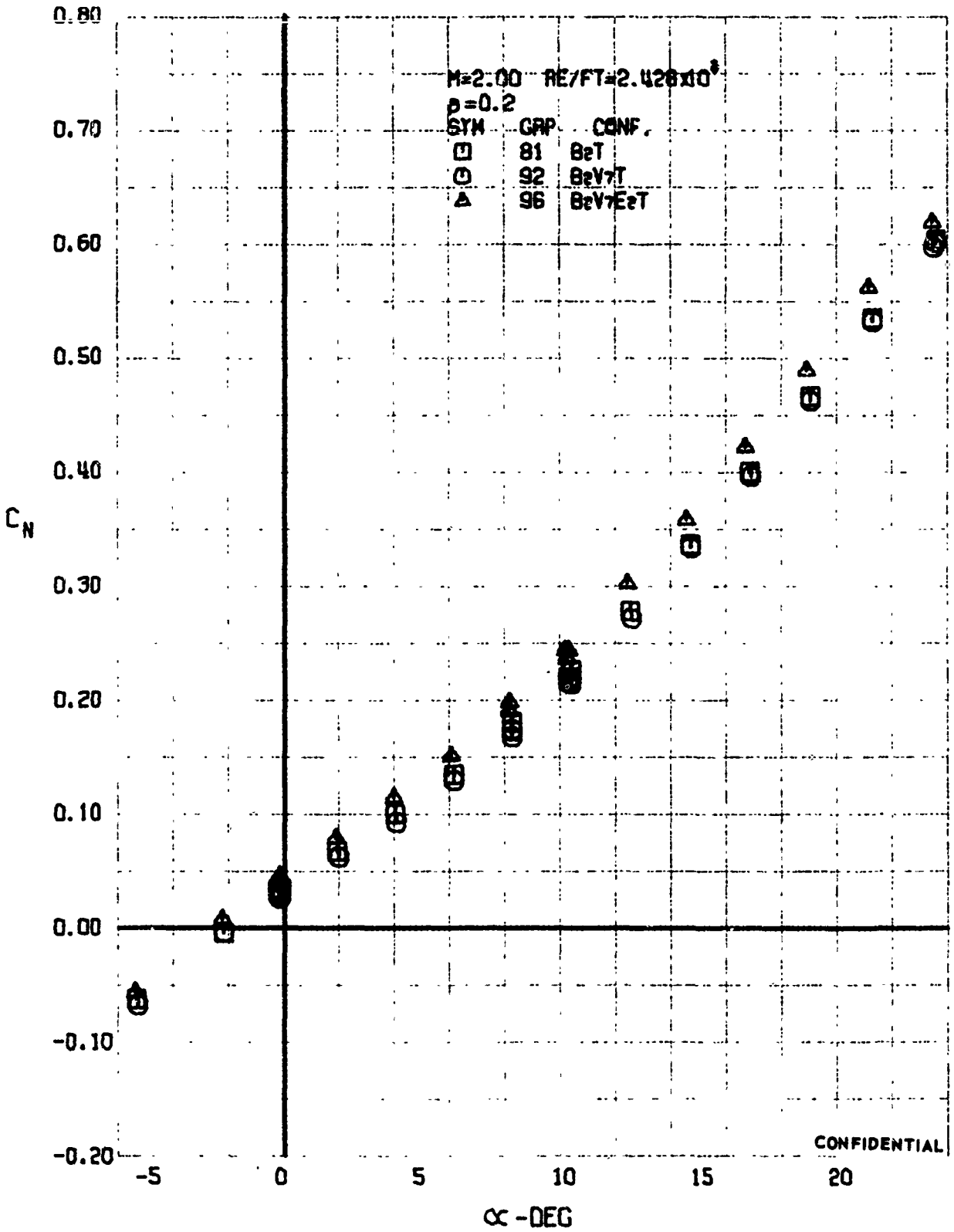
FIGURE 58 (U) CONFIGURATION BUILDUP - NORMAL FORCE COEFFICIENT VARIATION WITH ANGLE OF ATTACK ( M=2.00 )
