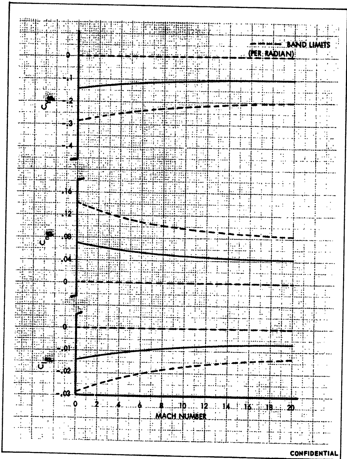
FIGURE 492 (U) VARIATION OF \beta DERIVATIVES WITH MACH NUMBER
