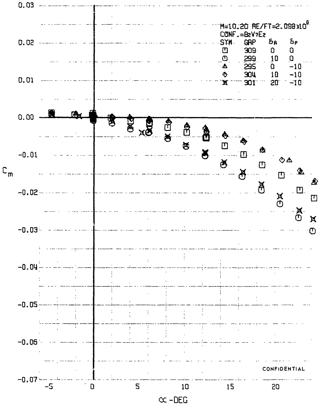
FIGURE 273 (U) AILERON EFFECTS - PITCHING MOMENT COEFFICIENT VARIATION WITH ANGLE OF ATTACK (M=10.20)
