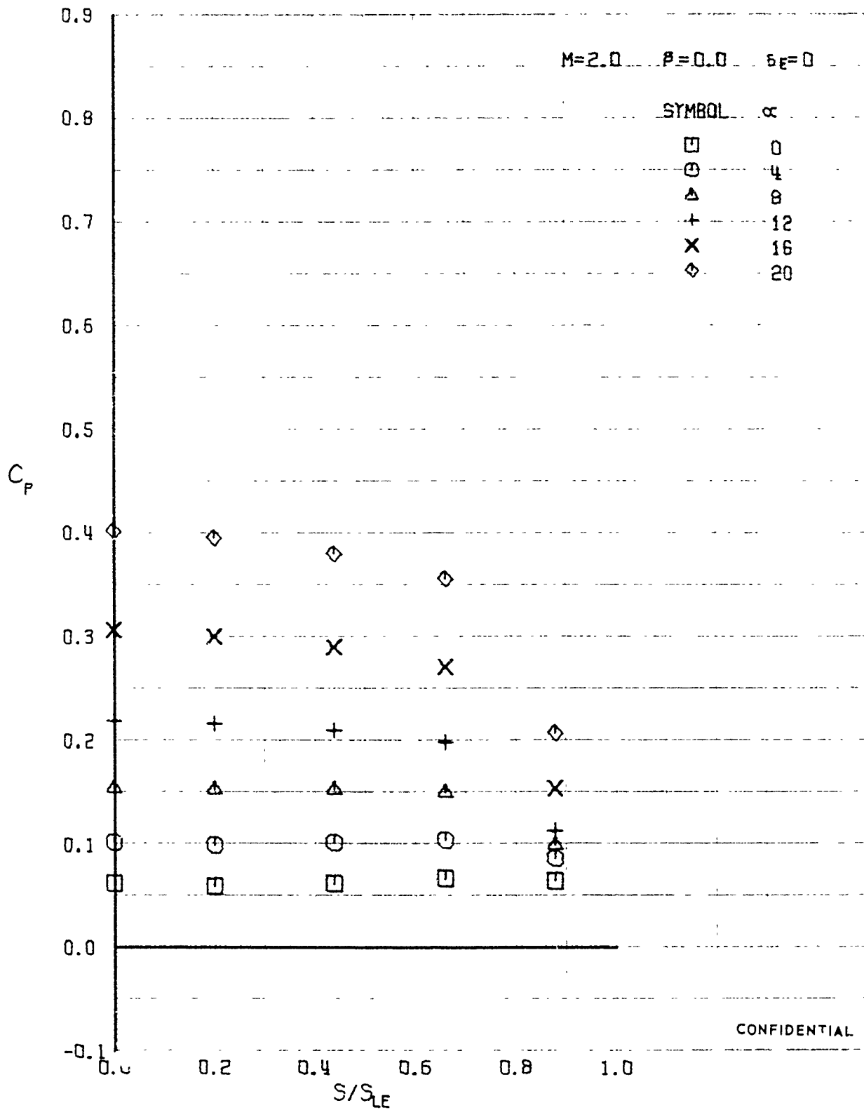
FIGURE 340 (U) LOWER SURFACE SPANWISE PRESSURES AT X/L = 0.30
