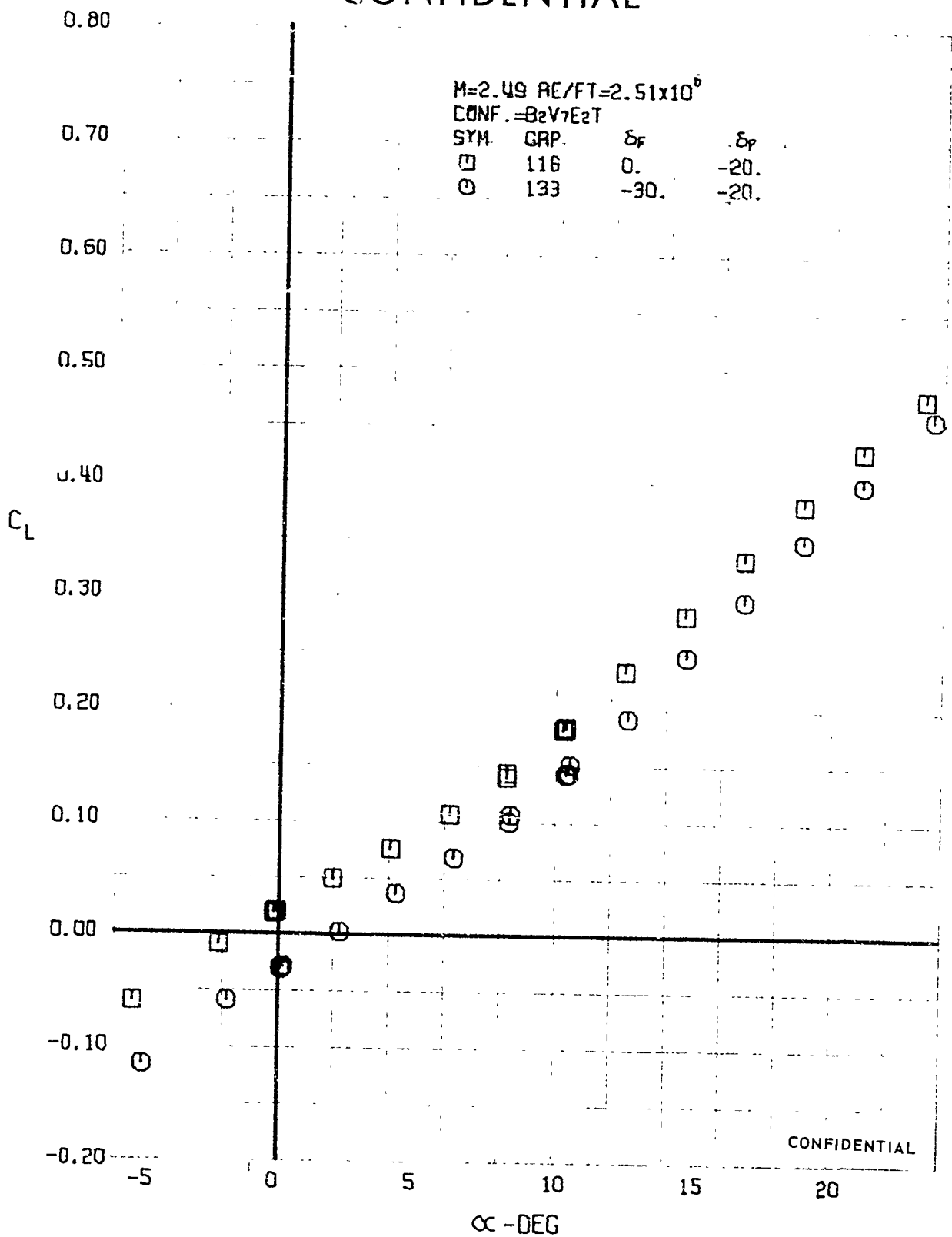
FIGURE 132 (C) FLAP EFFECTS - LIFT COEFFICIENT VARIATION WITH ANGLE OF ATTACK (M=2.49)
