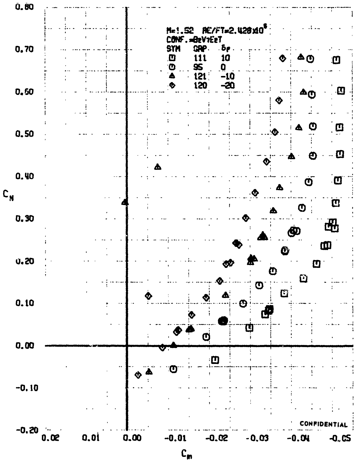
FIGURE 38 (U) ELEVON EFFECTS - LONGITUDINAL STABILITY VARIATION (M=1.52)
