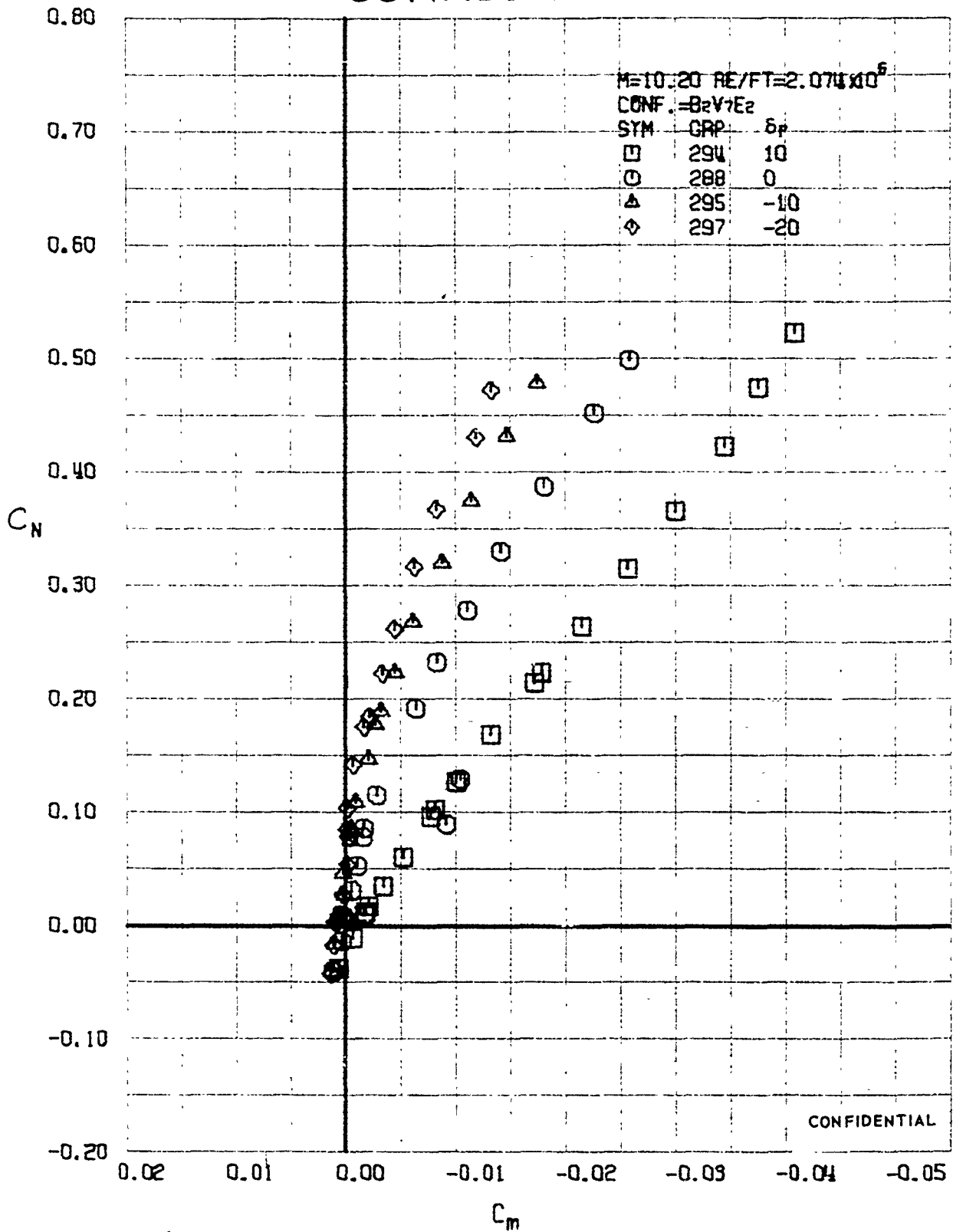
FIGURE 263 (U) ELEVON EFFECTS - LONGITUDINAL STABILITY VARIATION (M=10.20)
