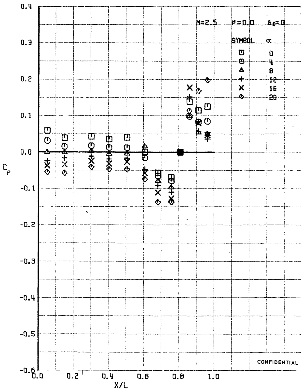
FIGURE 357 (U) UPPER SURFACE CENTERLINE PRESSURES
