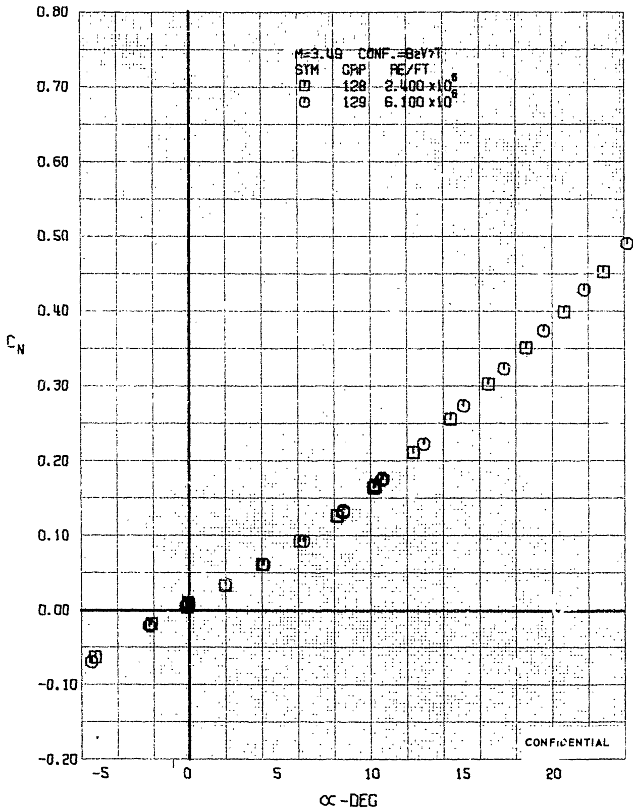
FIGURE 177 (U) REYNOLDS NUMBER EFFECTS - NORMAL FORCE COEFFICIENT VARIATION WITH ANGLE OF ATTACK (M=3.49)
