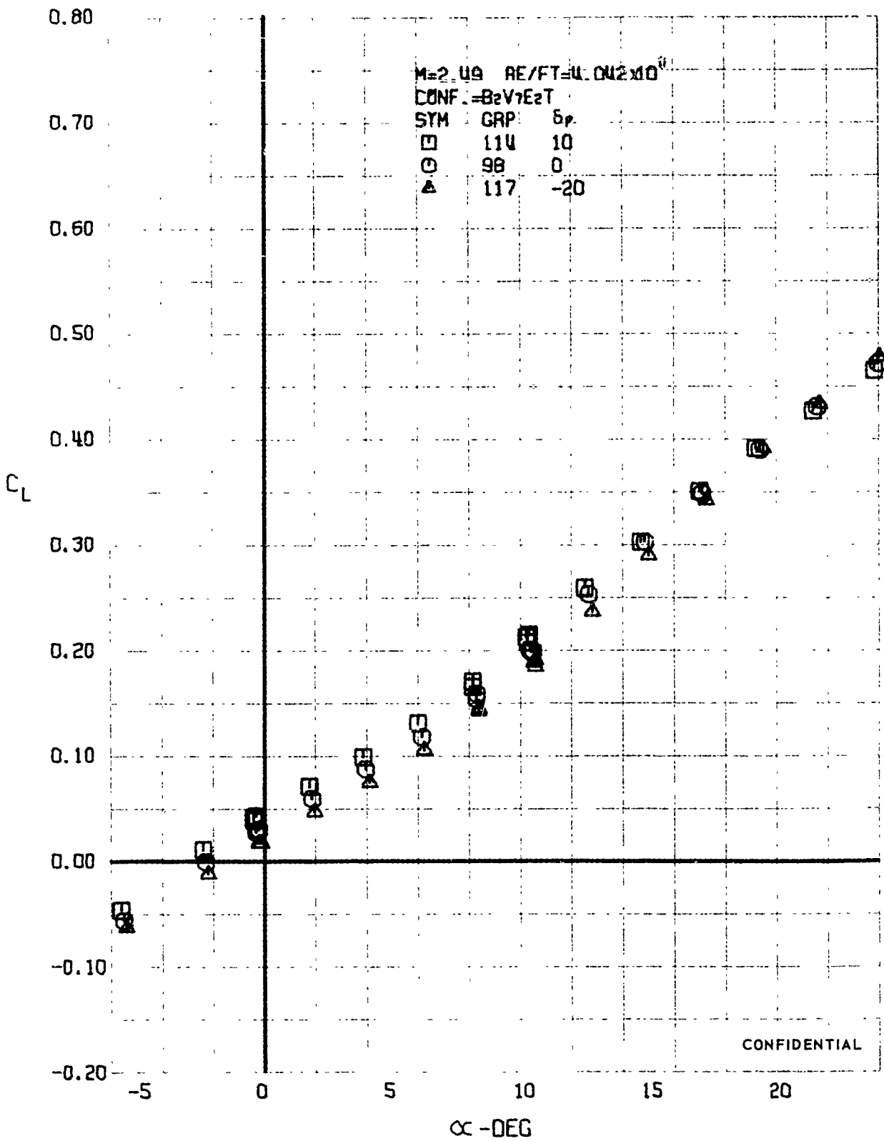
FIGURE 125 (U) ELEVON EFFECTS - LIFT COEFFICIENT VARIATION WITH ANGLE OF ATTACK (M=2.49)
