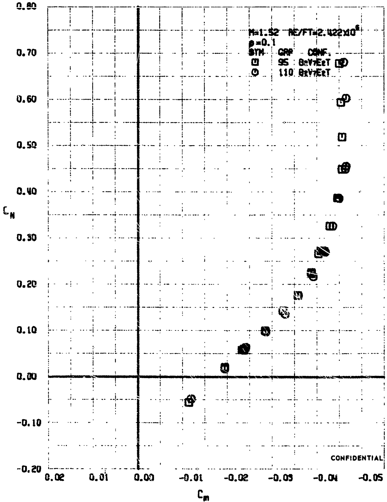
FIGURE 55 (U) REPEATABILITY - LONGITUDINAL STABILITY VARIATION ( M=1.52 )
