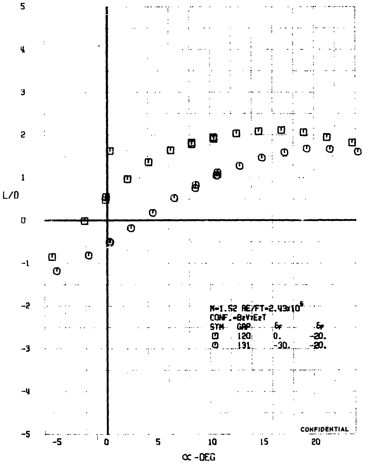
FIGURE 4 (U) FLAP EFFECTS - LIFT-DRAG RATIO VARIATION WITH ANGLE OF ATTACK ( M=1.52 )
