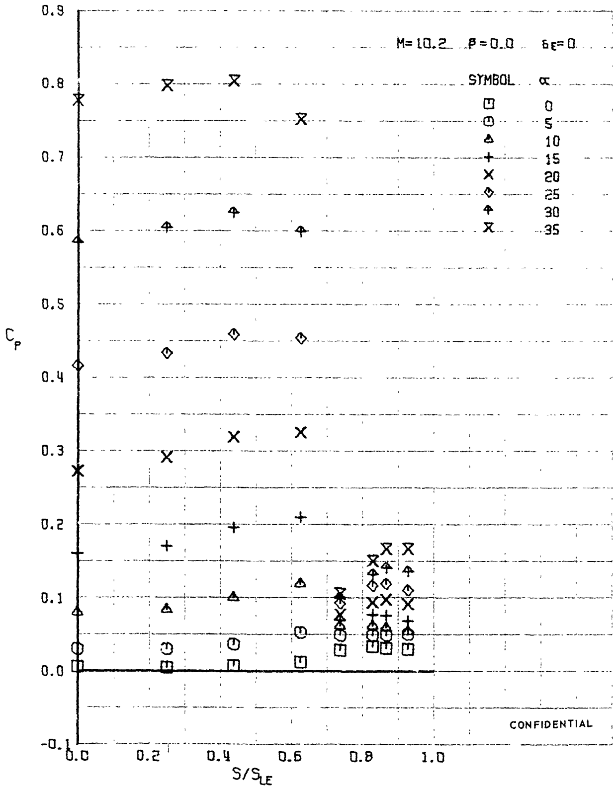
FIGURE 395 (U) LOWER SURFACE SPANWISE PRESSURES AT X/L = 0.96
