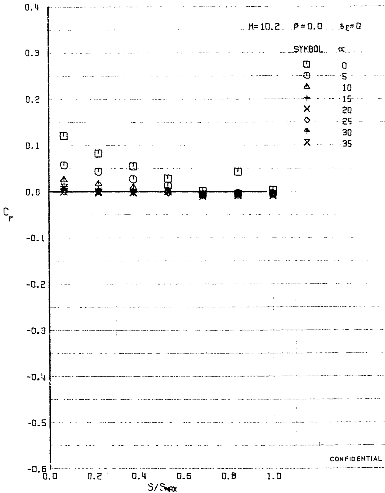
FIGURE 400 (U) UPPER SURFACE SPANWISE PRESSURES AT X/L = 0.76
