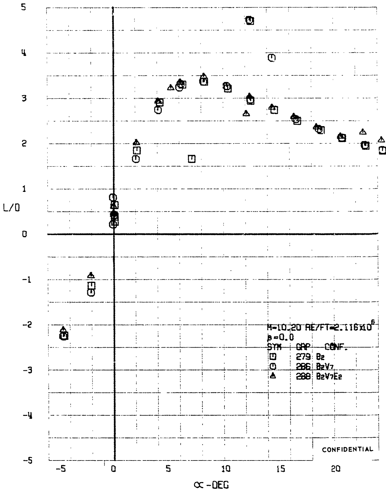
FIGURE 247 (U) CONFIGURATION BUILDUP - LIFT-DRAGE RATIO VARIATION WITH ANGLE OF ATTACK (M=10.20)
