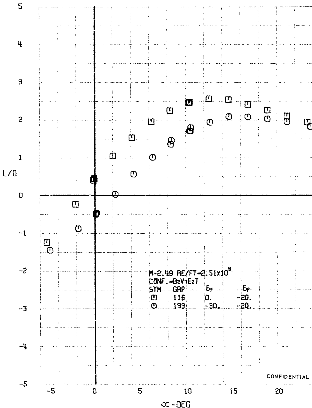
FIGURE 134 (U) FLAP EFFECTS - LIFT-DRAG RATIO VARIATION WITH ANGLE OF ATTACK (M=2.49)
