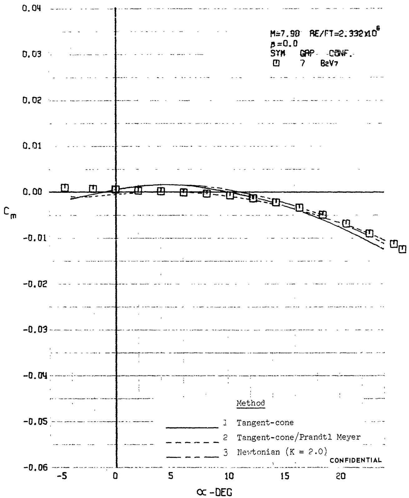
FIGURE 422 (U) COMPARISON OF ESTIMATED AND EXPERIMENTAL COEFFICIENTS - PITCHING MOMENT COEFFICIENT VARIATION WITH ANGLE OF ATTACK ( M=7.98 )
