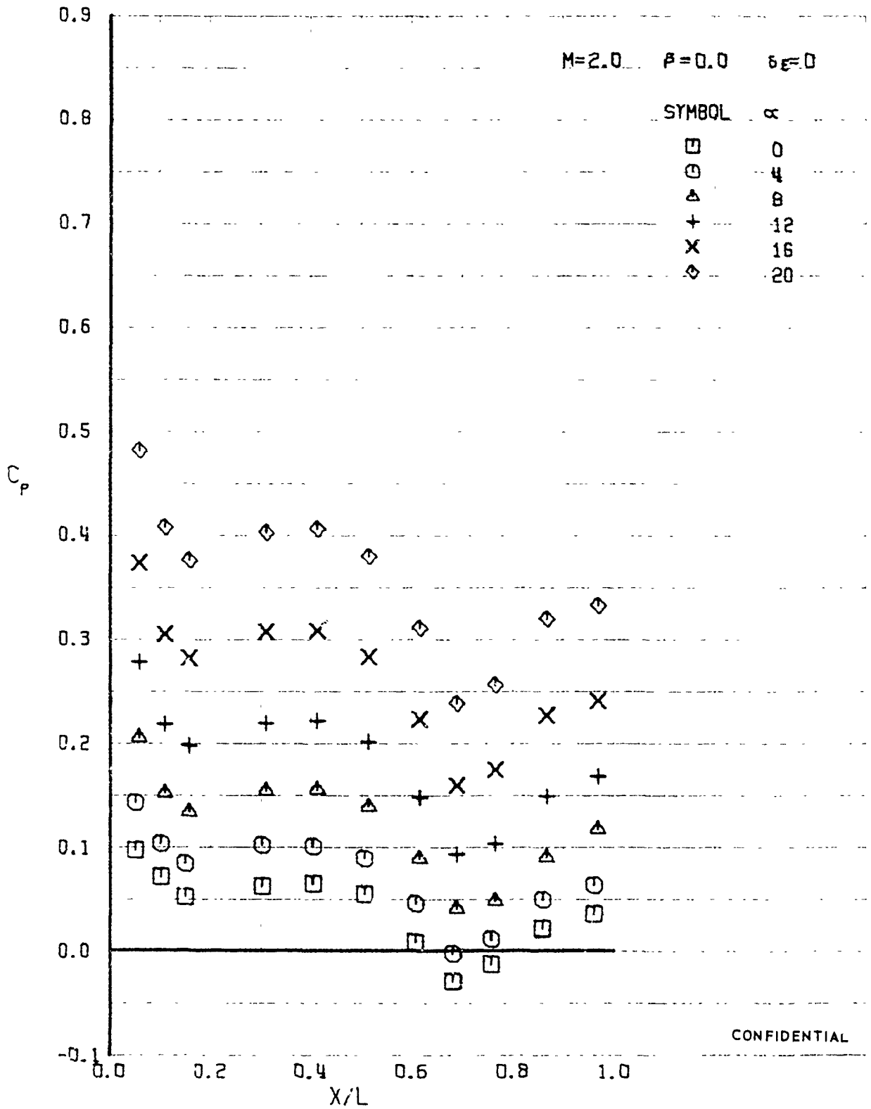
FIGURE 338 (U) LOWER SURFACE CENTERLINE PRESSURES
