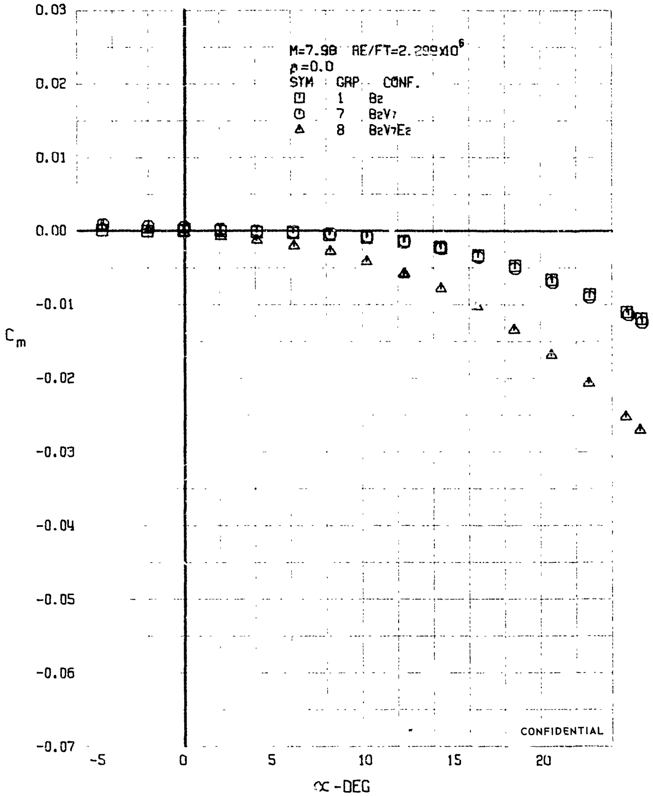
FIGURE 210 (U) CONFIGURATION BUILDUP - PITCHING MOMENT COEFFICIENT VARIATION WITH ANGLE OF ATTACK (M=7.98)
