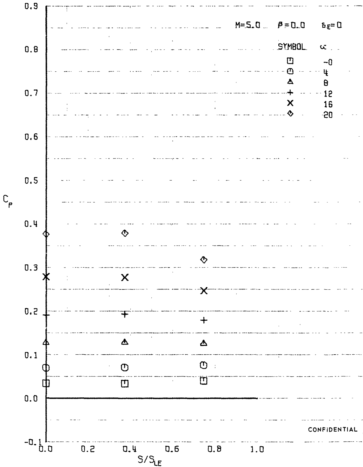
FIGURE 378 (U) LOWER SURFACE SPANWISE PRESSURES AT X/L = 0.15
