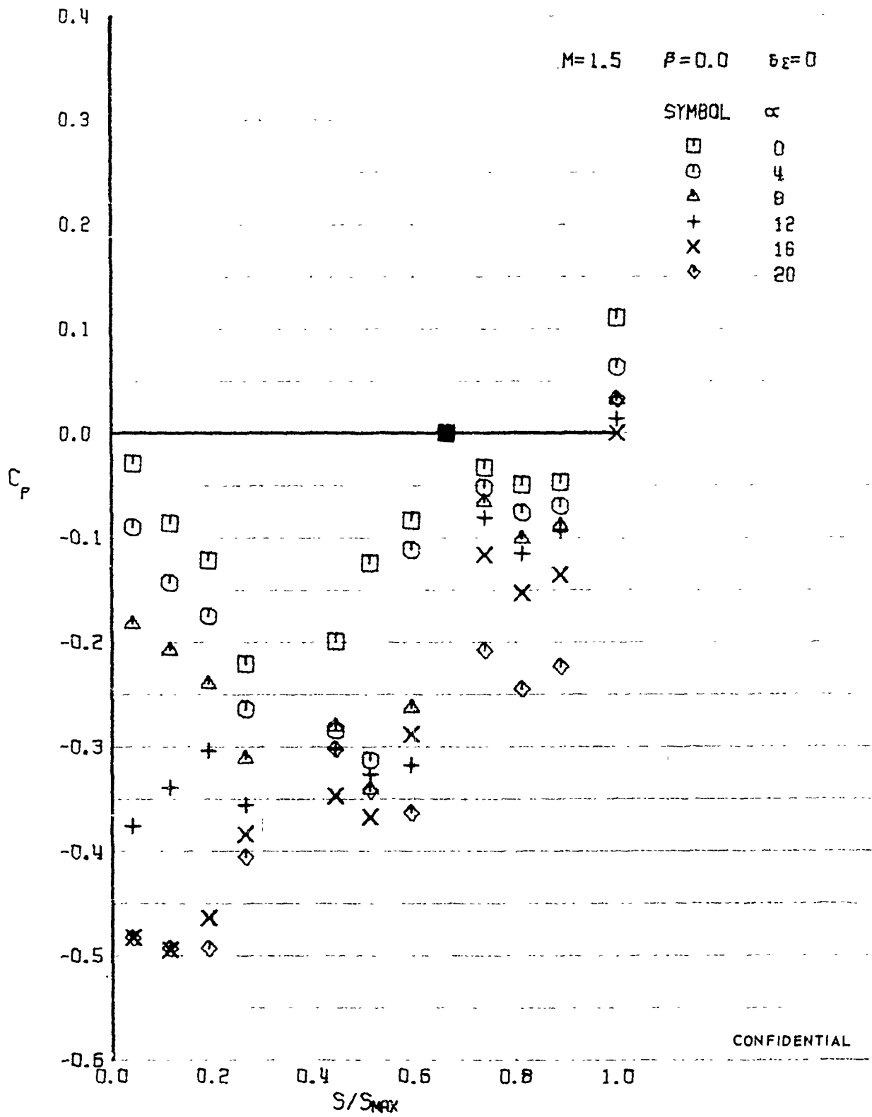
FIGURE 337 (U) UPPER SURFACE SPANWISE PRESSURES AT X/L = 0.96
