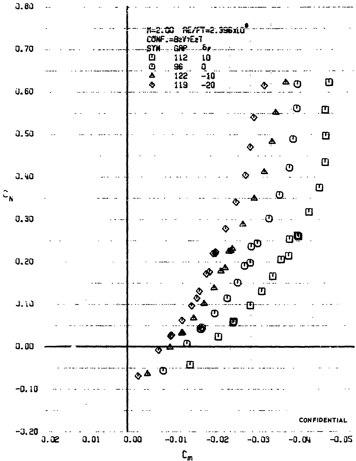
FIGURE 70 (U) ELEVON EFFECTS - LONGITUDINAL STABILITY VARIATION (M=2.00)
