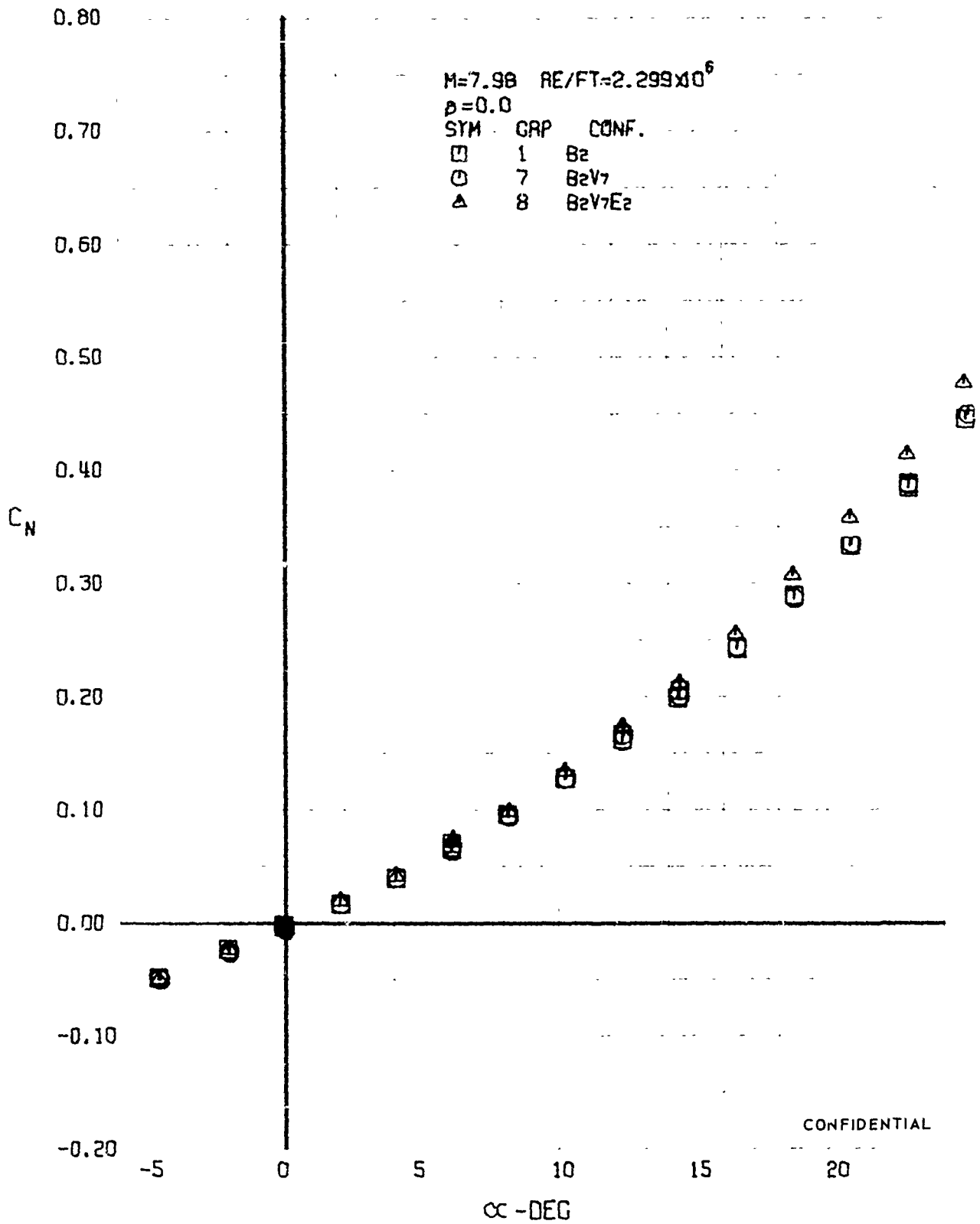
FIGURE 207 (U) CONFIGURATION BUILDUP - NORMAL FORCE COEFFICIENT VARIATION WITH ANGLE OF ATTACK (M=7.98)
