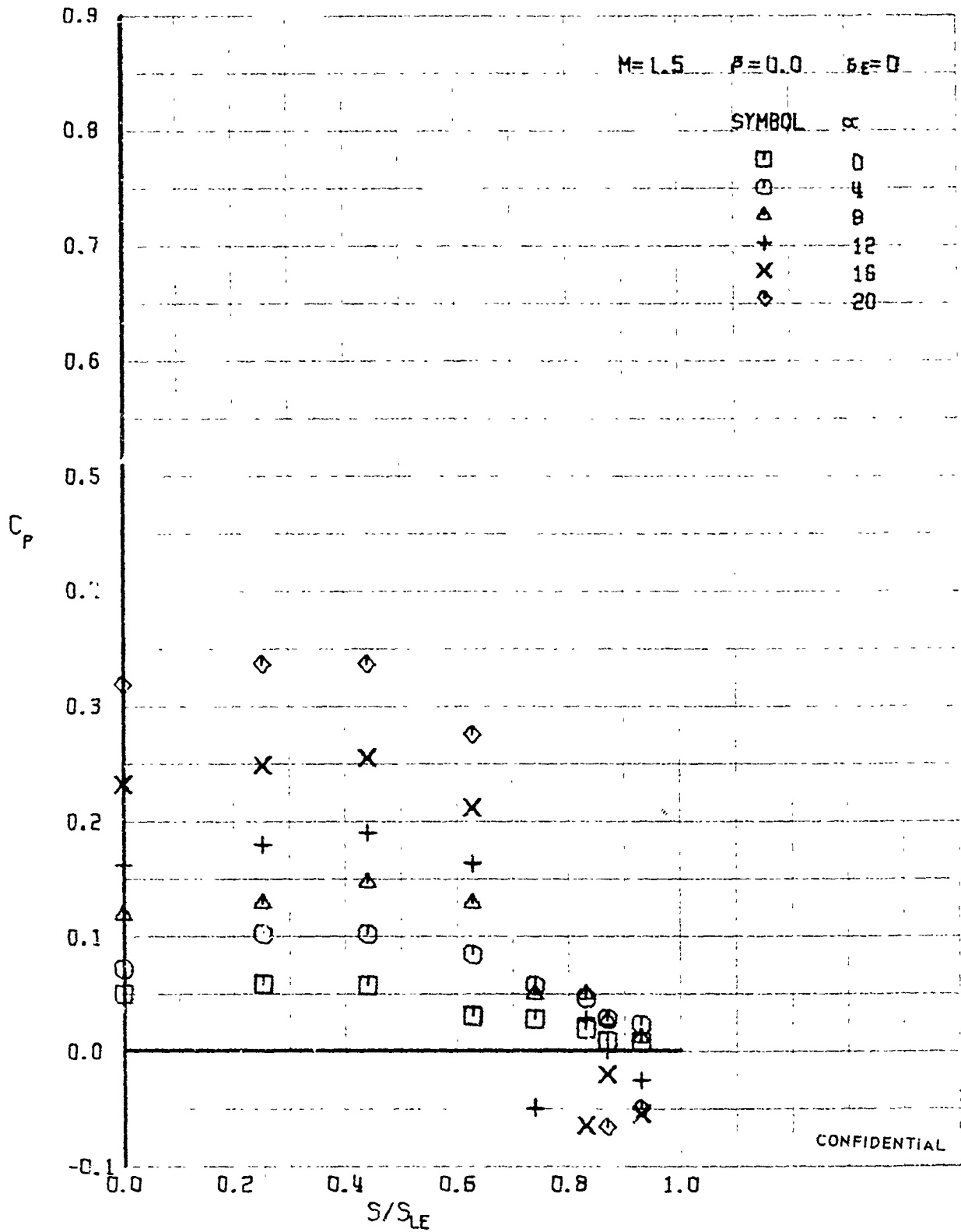
FIGURE 330 (U) LOWER SURFACE SPANWISE PRESSURES AT X/L = 0.96
