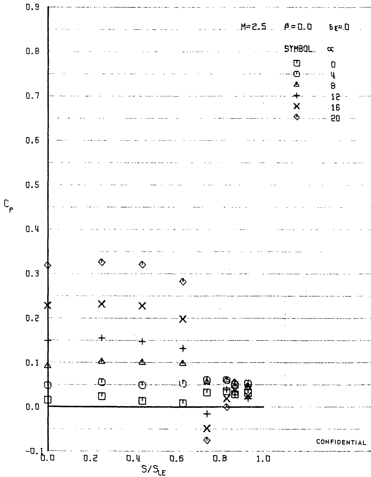
FIGURE 356 (U) LOWER SURFACE SPANWISE PRESSURES AT X/L = 0.96
