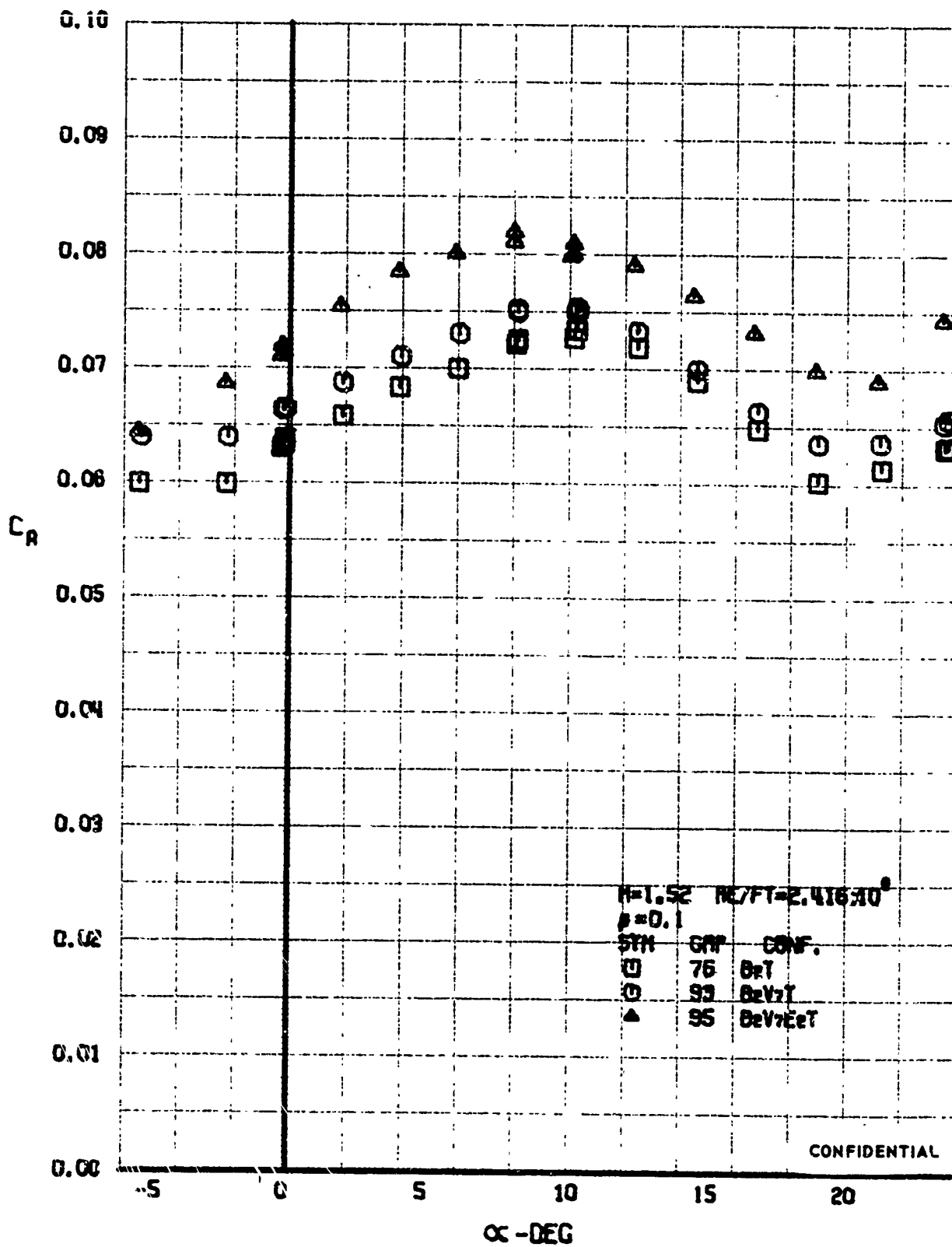
FIGURE 15 (U) CONFIGURATION BUILDUP - AXIAL FORCE COEFFICIENT VARIATION WITH ANGLE OF ATTACK ( H=1.52 )
