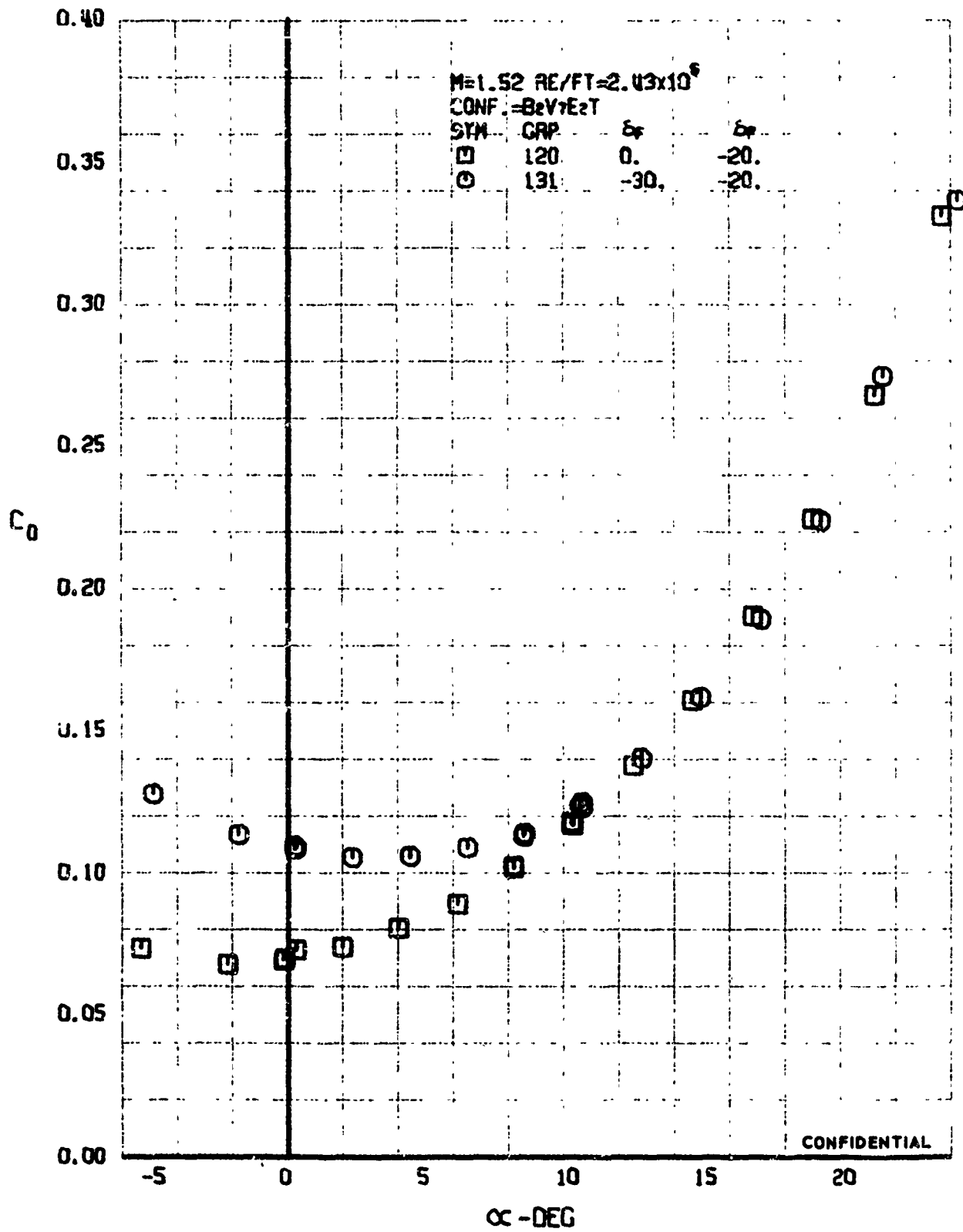
FIGURE 47 (U) FLAP EFFECTS - DRAG COEFFICIENT VARIATION WITH ANGLE OF ATTACK (M=1.52)
