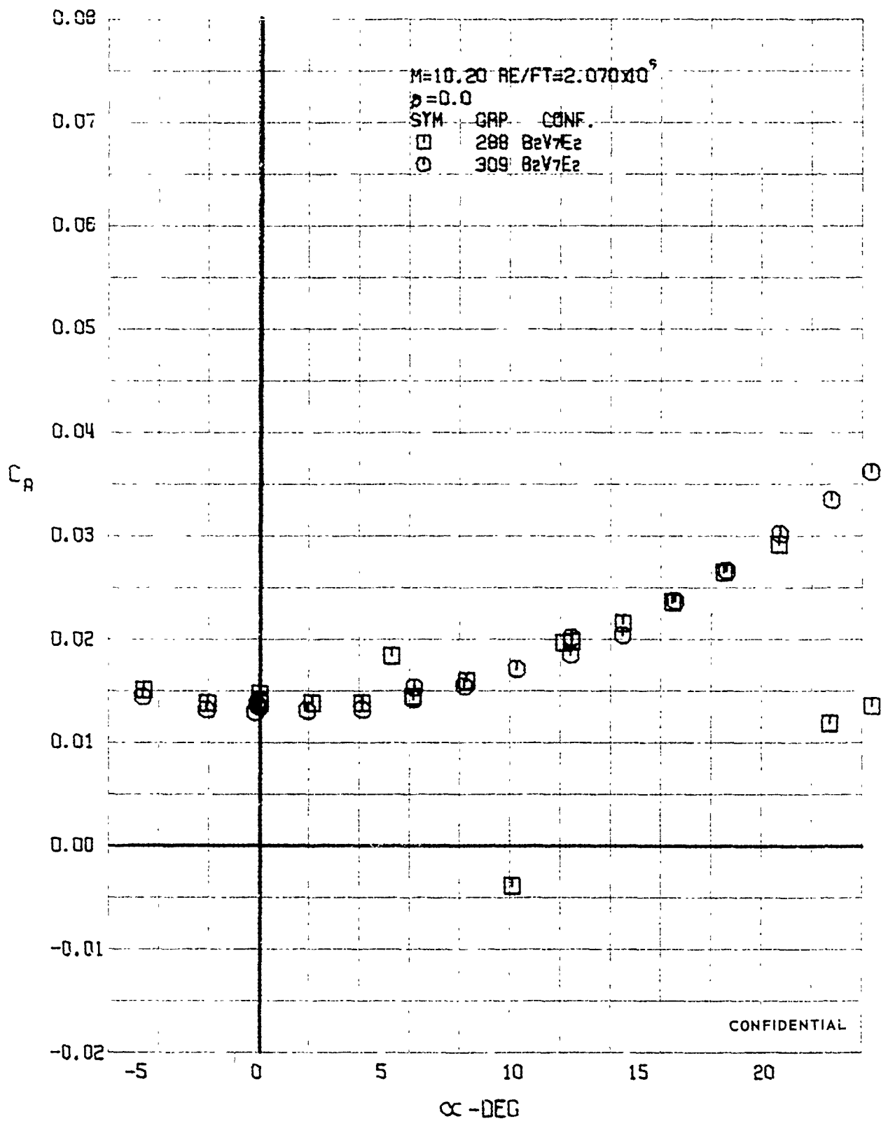
FIGURE 288 (U) REPEATABILITY - AXIAL FORCE COEFFICIENT VARIATION WITH ANGLE OF ATTACK (M=10.20)
