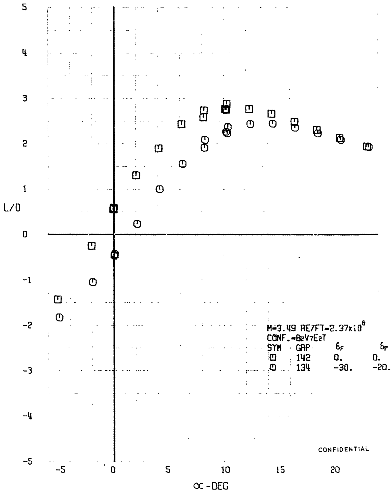
FIGURE 175 (U) COMBINED ELEVON AND FLAP EFFECTS - LIFT-DRAG RATIO VARIATION WITH ANGLE OF ATTACK ( M=3.49 )
