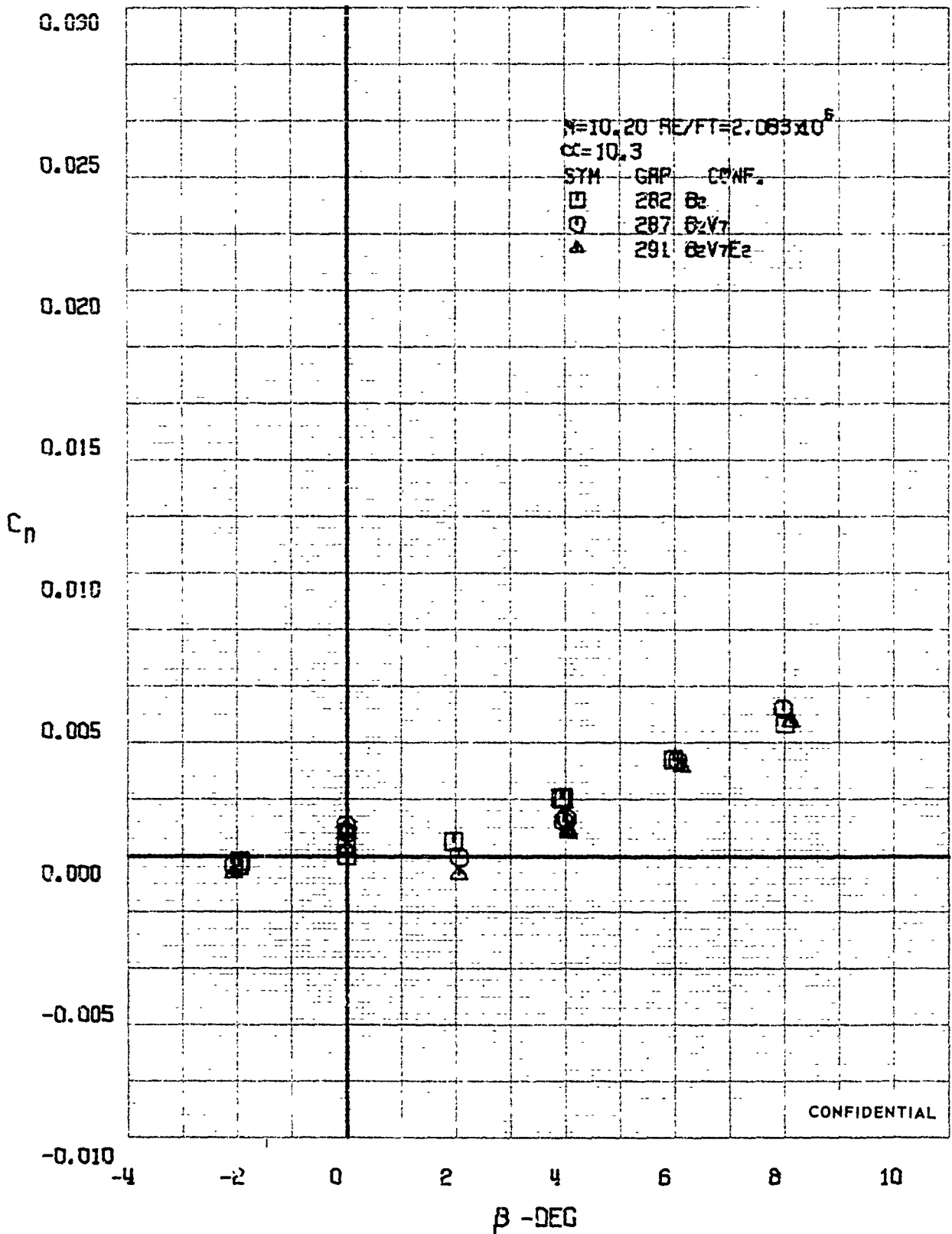
FIGURE 254 (U) CONFIGURATION BUILDUP - YAWING MOMENT COEFFICIENT VARIATION WITH ANGLE OF YAW (M=10.20)
