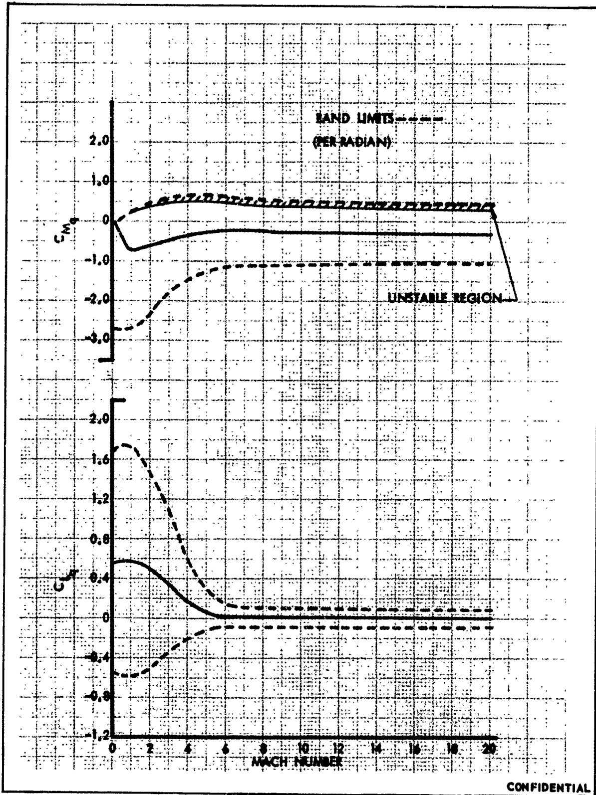
FIGURE 488 (U) VARIATION OF q DERIVATIVES WITH MACH NUMBER
