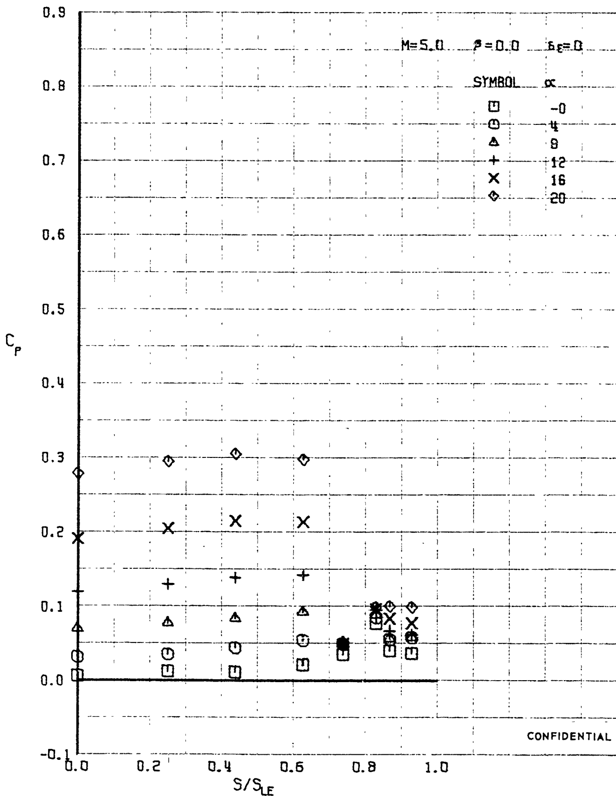
FIGURE 381 (U) LOWER SURFACE SPANWISE PRESSURES AT X/L = 0.76
