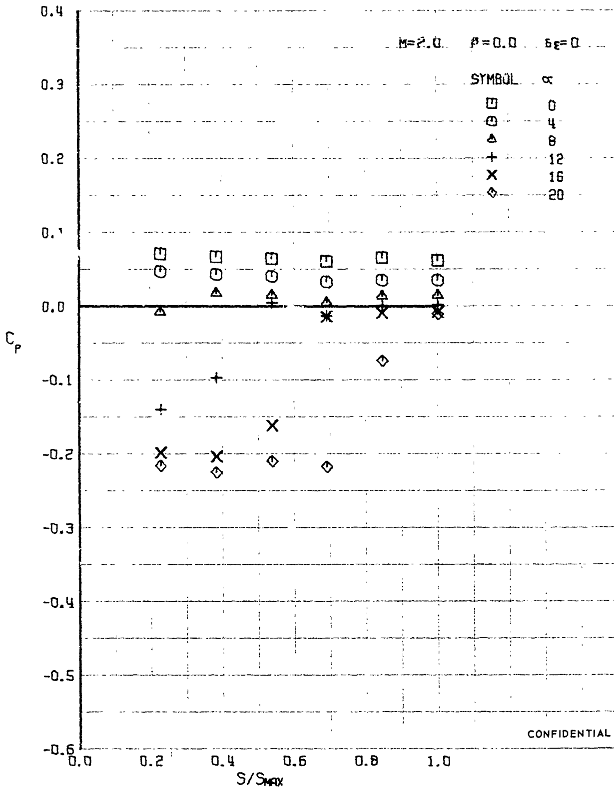
FIGURE 346 (U) UPPER SURFACE SPANWISE PRESSURES AT X/L = 0.30
