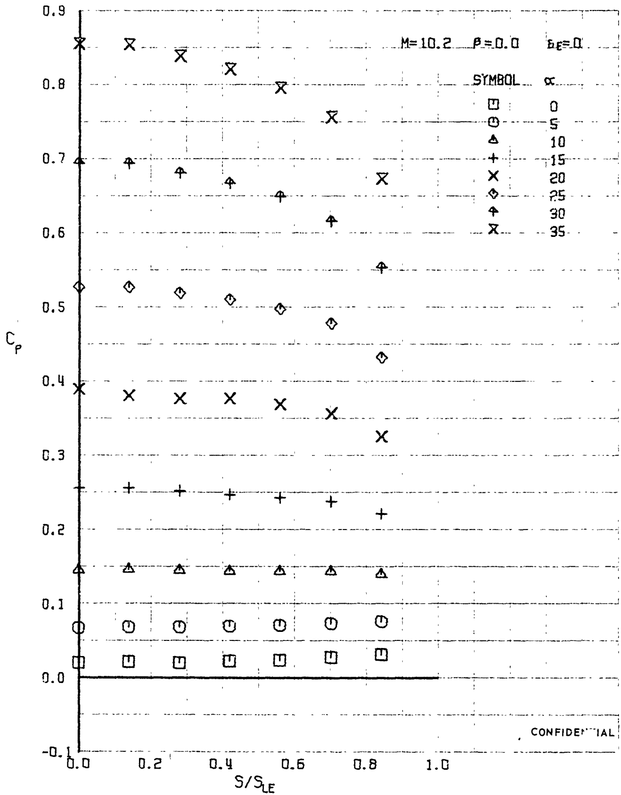
FIGURE 393 (U) LOWER SURFACE SPANWISE PRESSURES AT X/L = 0.50
