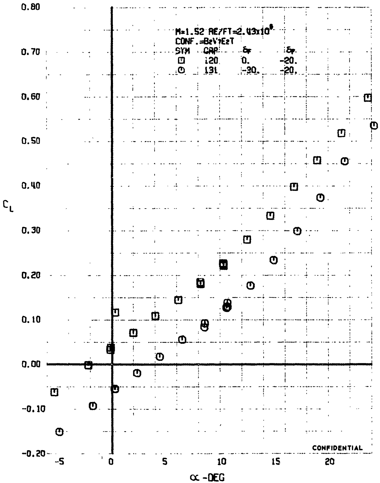
FIGURE 46 (U) FLAP EFFECTS - LIFT COEFFICIENT VARIATION WITH ANGLE OF ATTACK (M=1.52)
