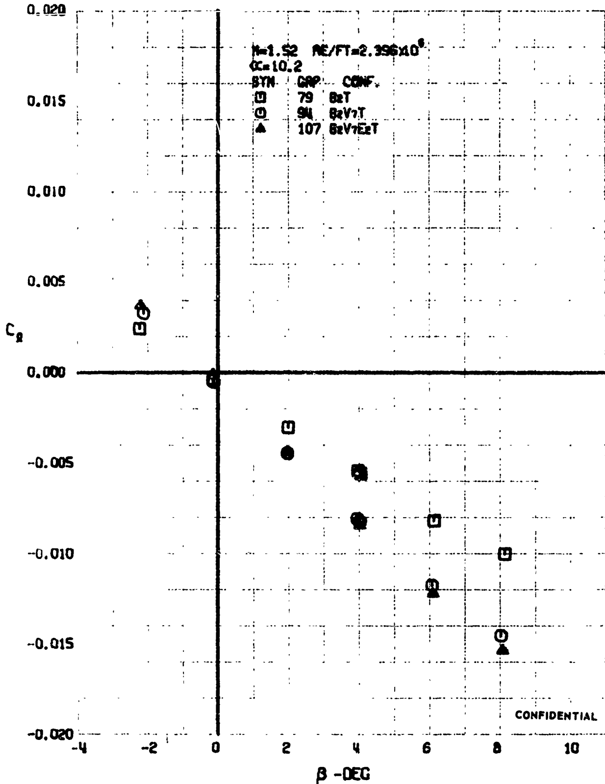
FIGURE 33 (U) CONFIGURATION BUILDUP - ROLLING MOMENT COEFFICIENT VARIATION WITH ANGLE OF YAW ( M=1.52 )
