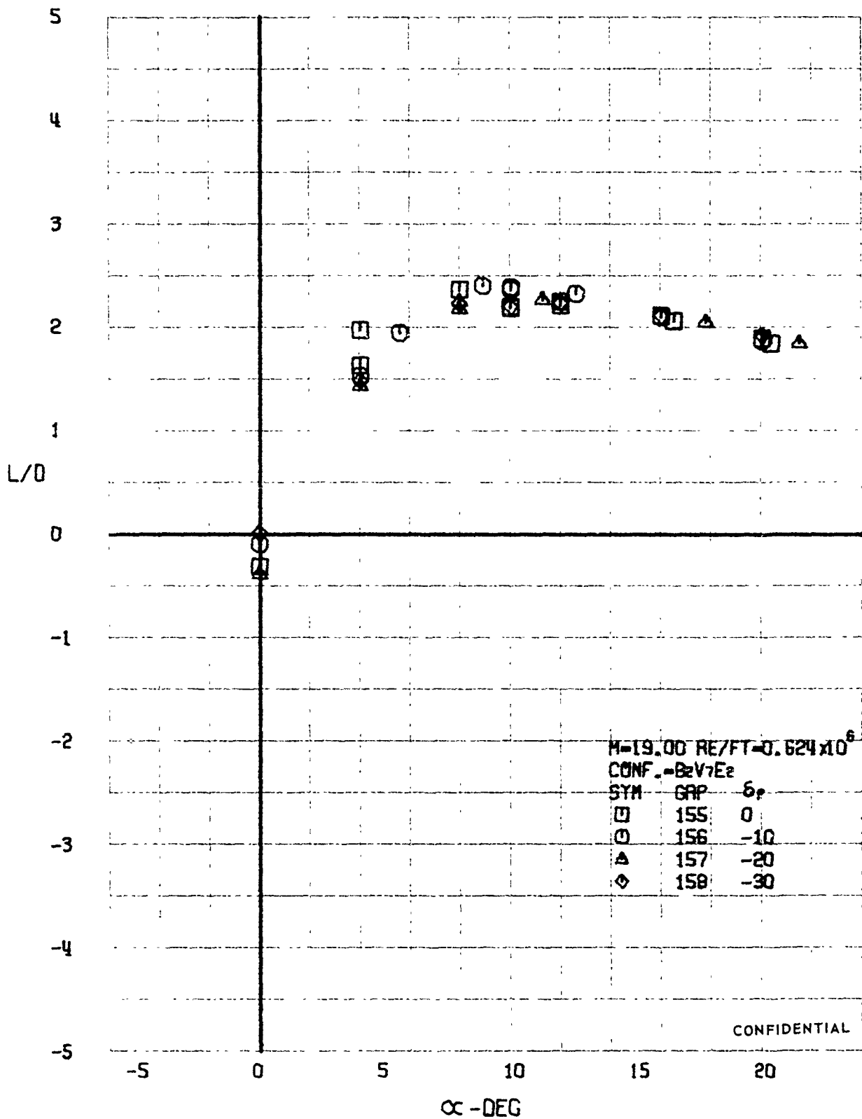
FIGURE 313 (U) ELEVON EFFECTS - LIFT-DRAG RATIO VARIATION WITH ANGLE OF ATTACK (M=19.00)
