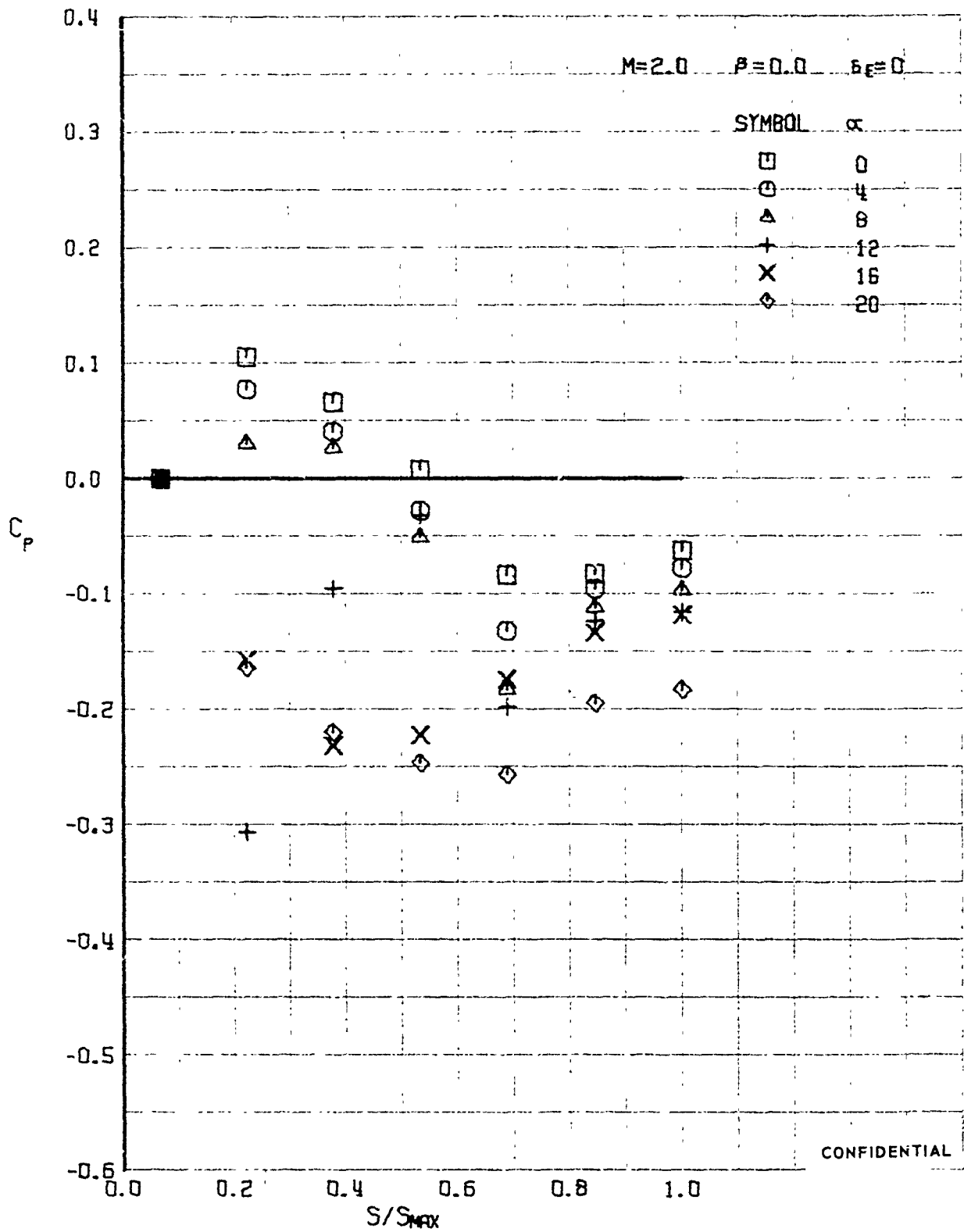
FIGURE 348 (U) UPPER SURFACE SPANWISE PRESSURES AT X/L = 0.75
