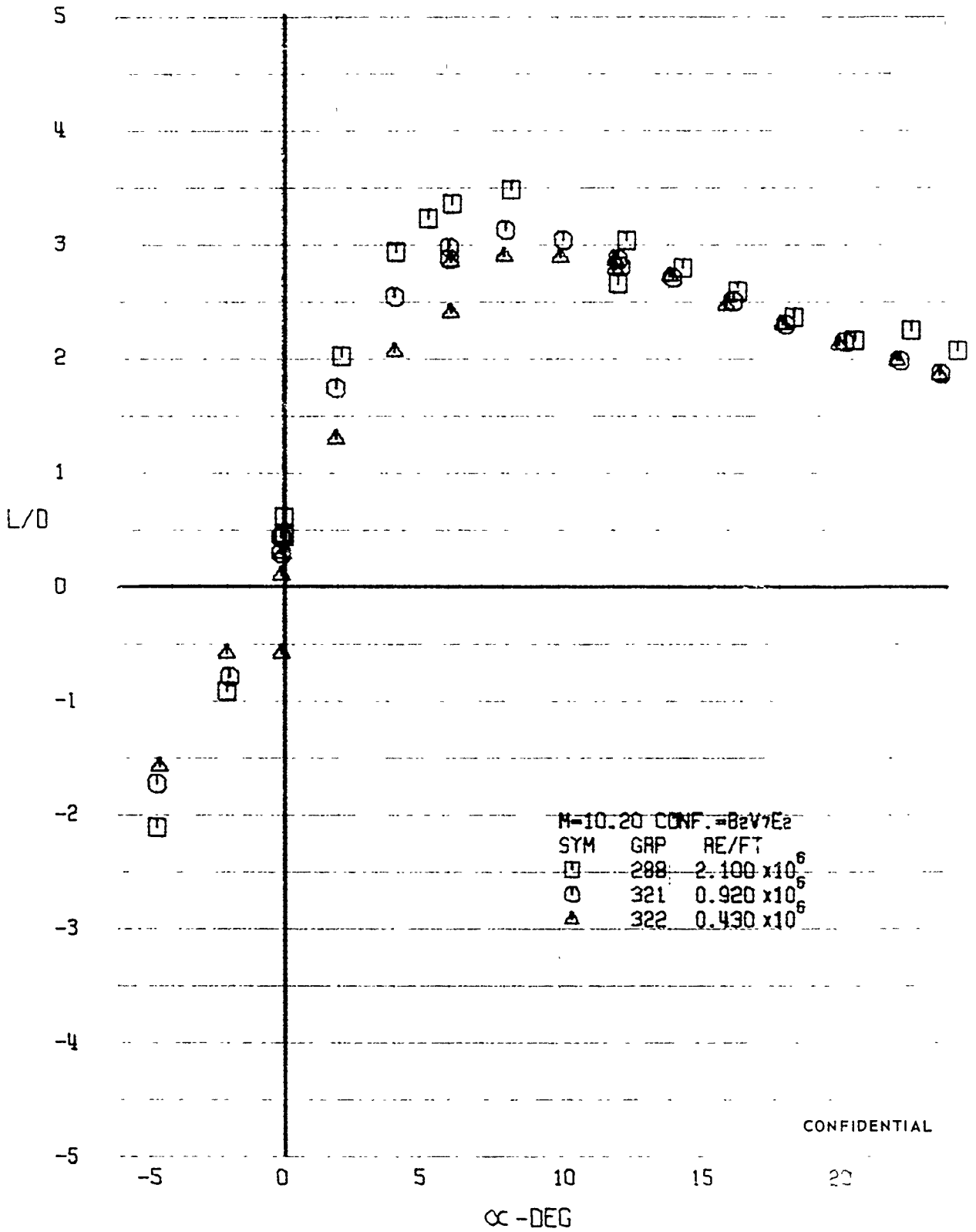
FIGURE 287 (U) REYNOLDS NUMBER EFFECTS - LIFT-DRAG RATIO VARIATION WITH ANGLE OF ATTACK (M=10.20)
