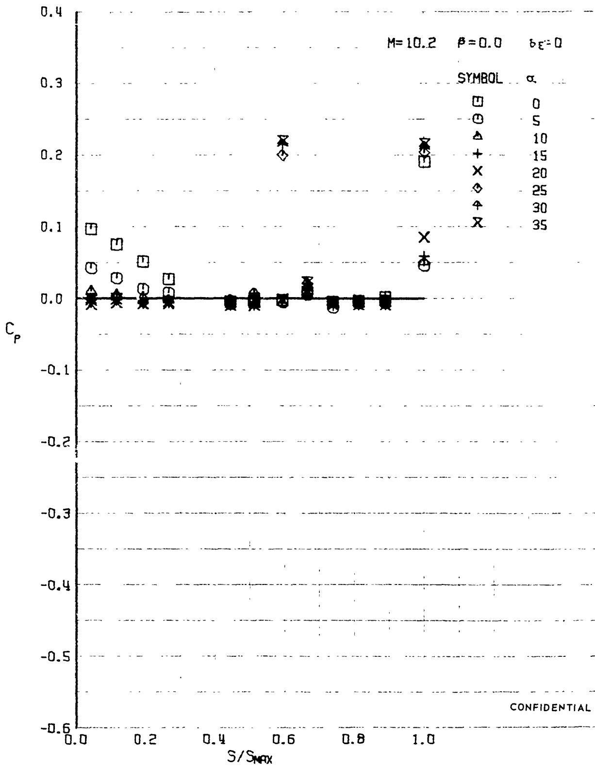
FIGURE 402 (U) UPPER SURFACE SPANWISE PRESSURES AT X/L = 0.96
