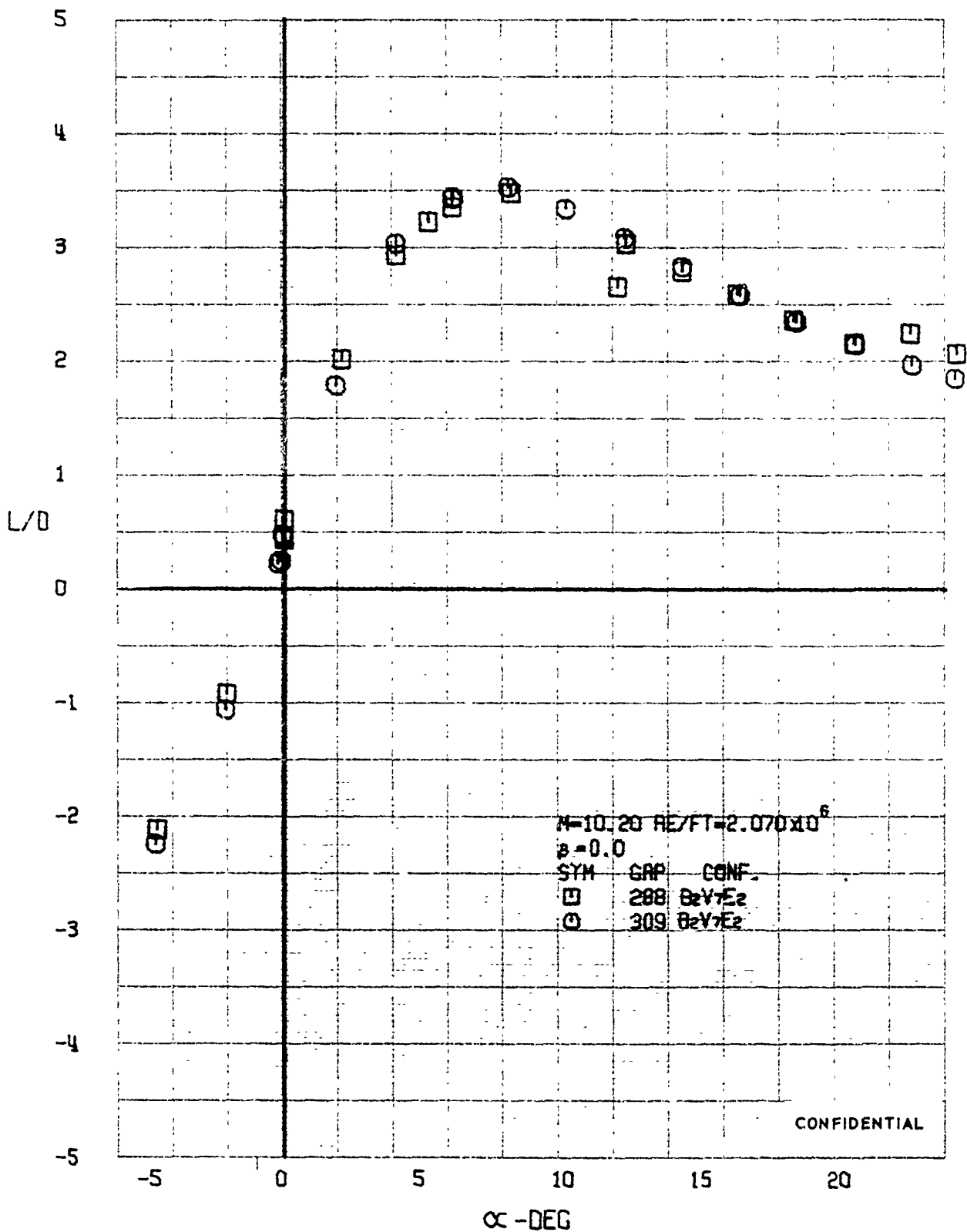
FIGURE 291 (U) REPEATABILITY - LIFT-DRAGE RATIO VARIATION WITH ANGLE OF ATTACK ( M=10.20 )
