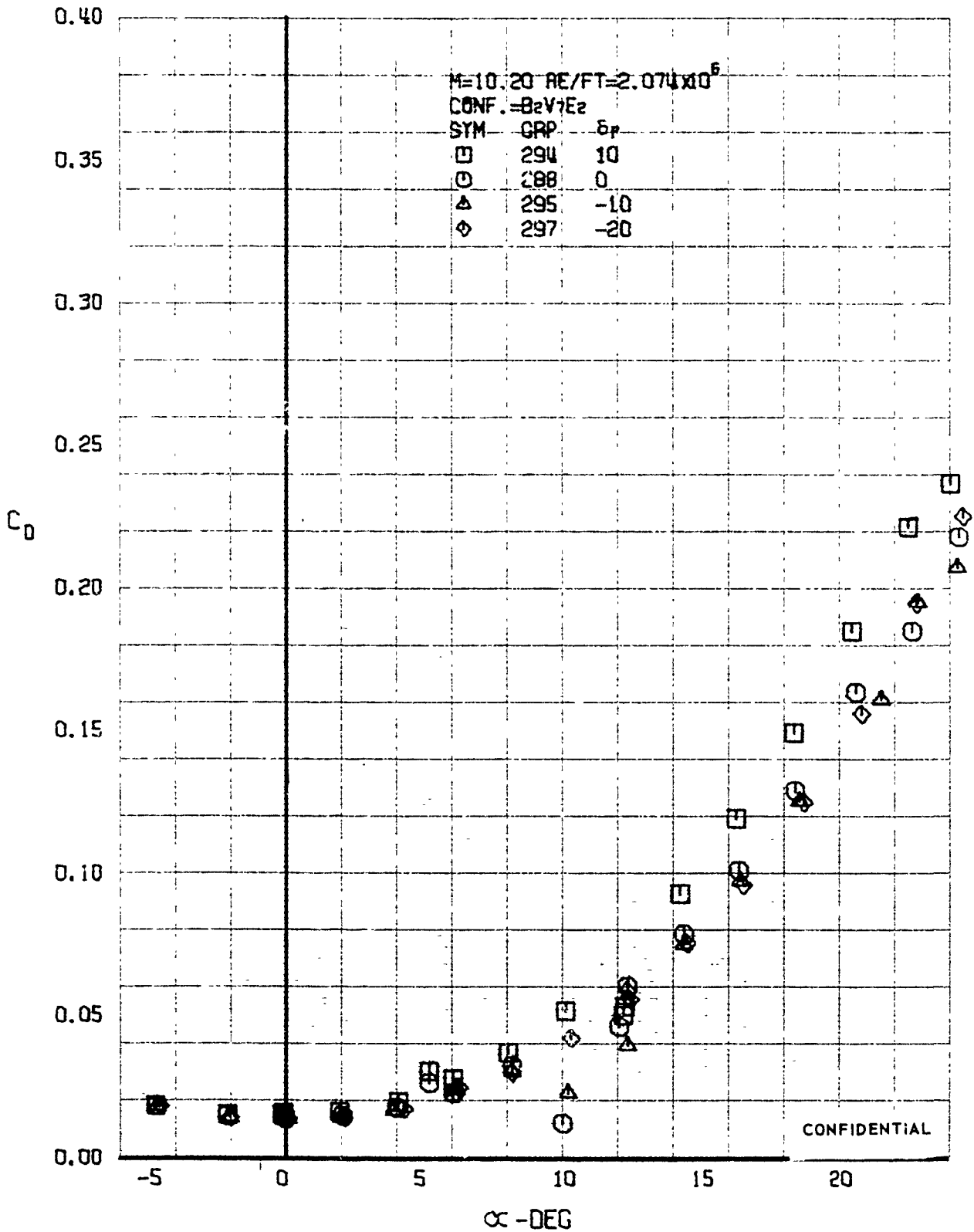
FIGURE 265 (U) ELEVON EFFECTS - DRAG COEFFICIENT VARIATION WITH ANGLE OF ATTACK ( M=10.20 )
