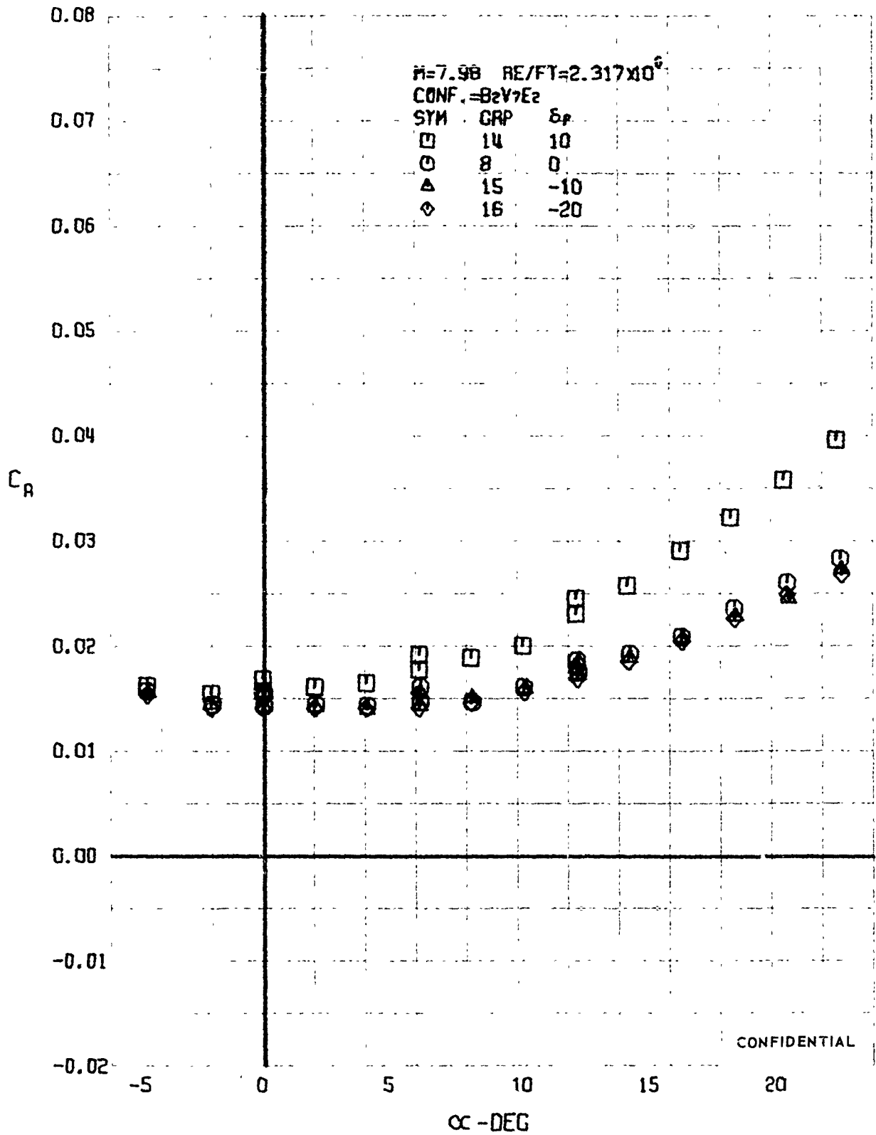
FIGURE 230 (U) ELEVON EFFECTS - AXIAL FORCE COEFFICIENT VARIATION WITH ANGLE OF ATTACK ( M=7.98 )
