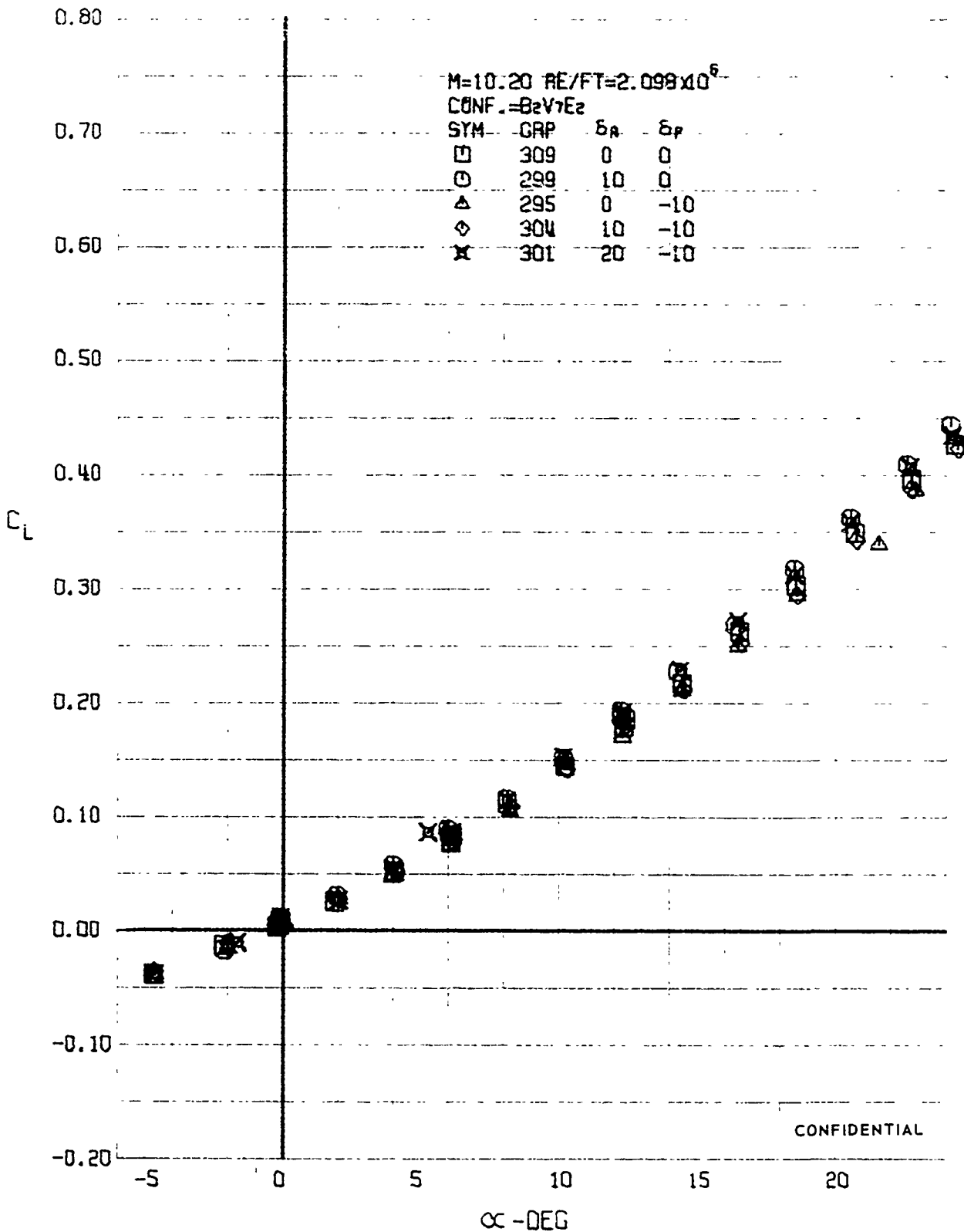
FIGURE 275 (U) AILERON EFFECTS - LIFT COEFFICIENT VARIATION WITH ANGLE OF ATTACK (M=10.20)
