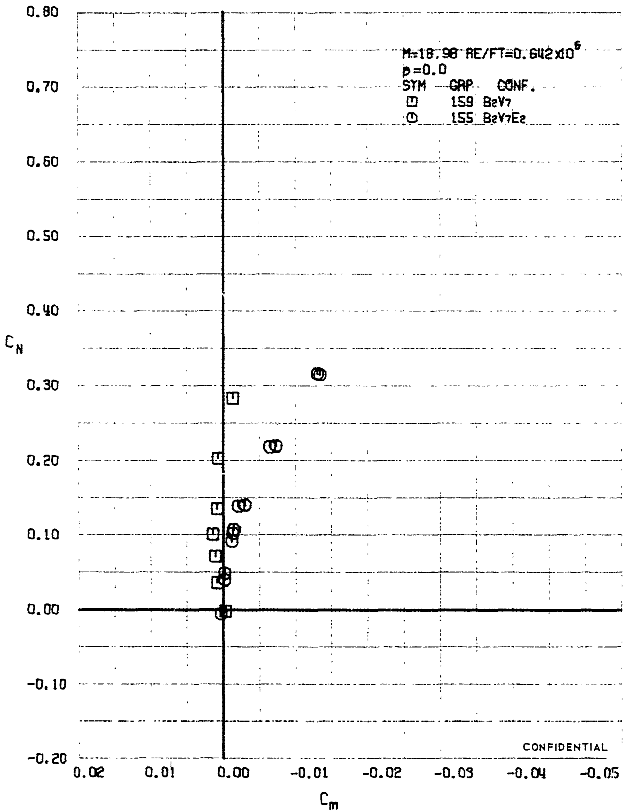
FIGURE 299. (U) CONFIGURATION BUILDUP - LONGITUDINAL STABILITY VARIATION (M=18.98)
