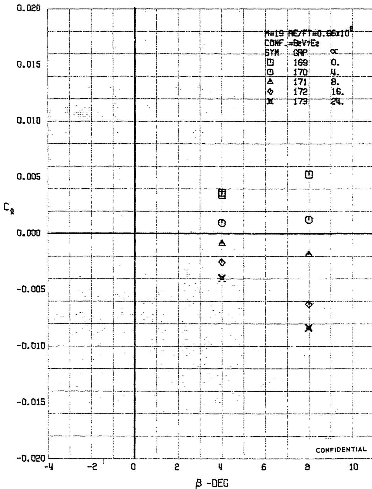
FIGURE 305 (U) COMPLETE CONFIGURATION - ROLLING MOMENT COEFFICIENT VARIATION WITH ANGLE OF YAW ( M=18.73 )
