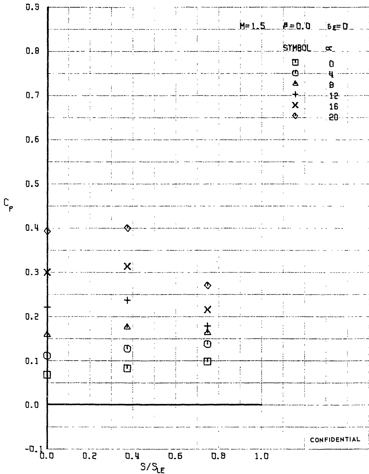
FIGURE 326 (U) LOWER SURFACE SPANWISE PRESSURES AT X/L = 0.15
