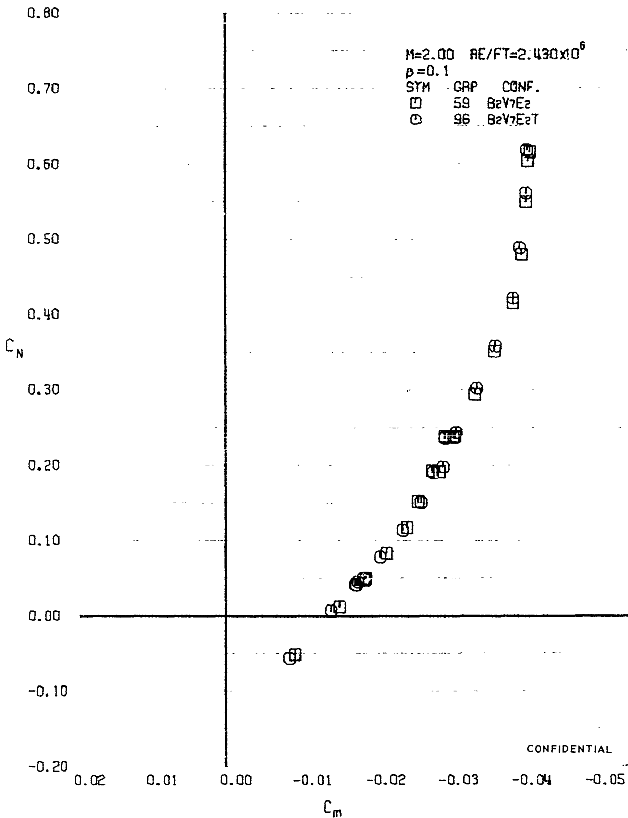
FIGURE (U) FORCED TRANSITION EFFECTS - LONGITUDINAL STABILITY VARIATION (M=2.00)
