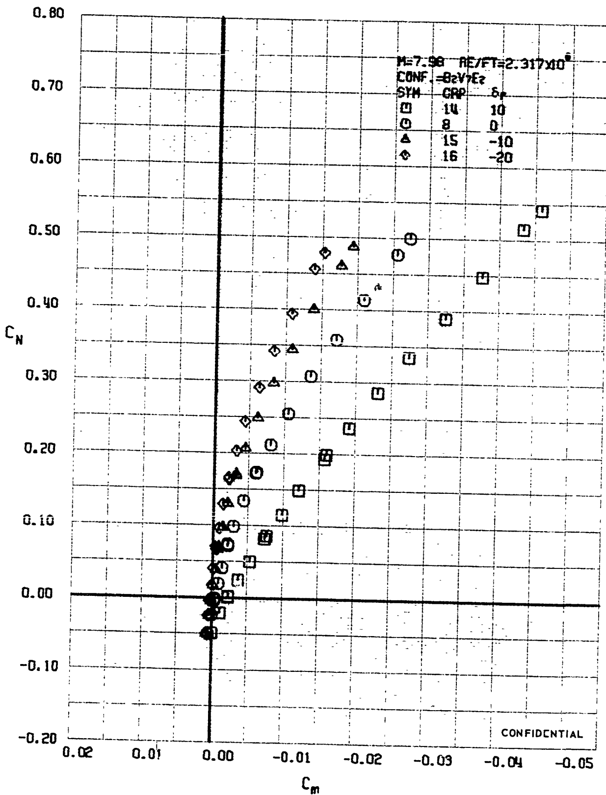
FIGURE 233 (U) ELEVON EFFECTS - LONGITUDINAL STABILITY VARIATION (M=7.98)
