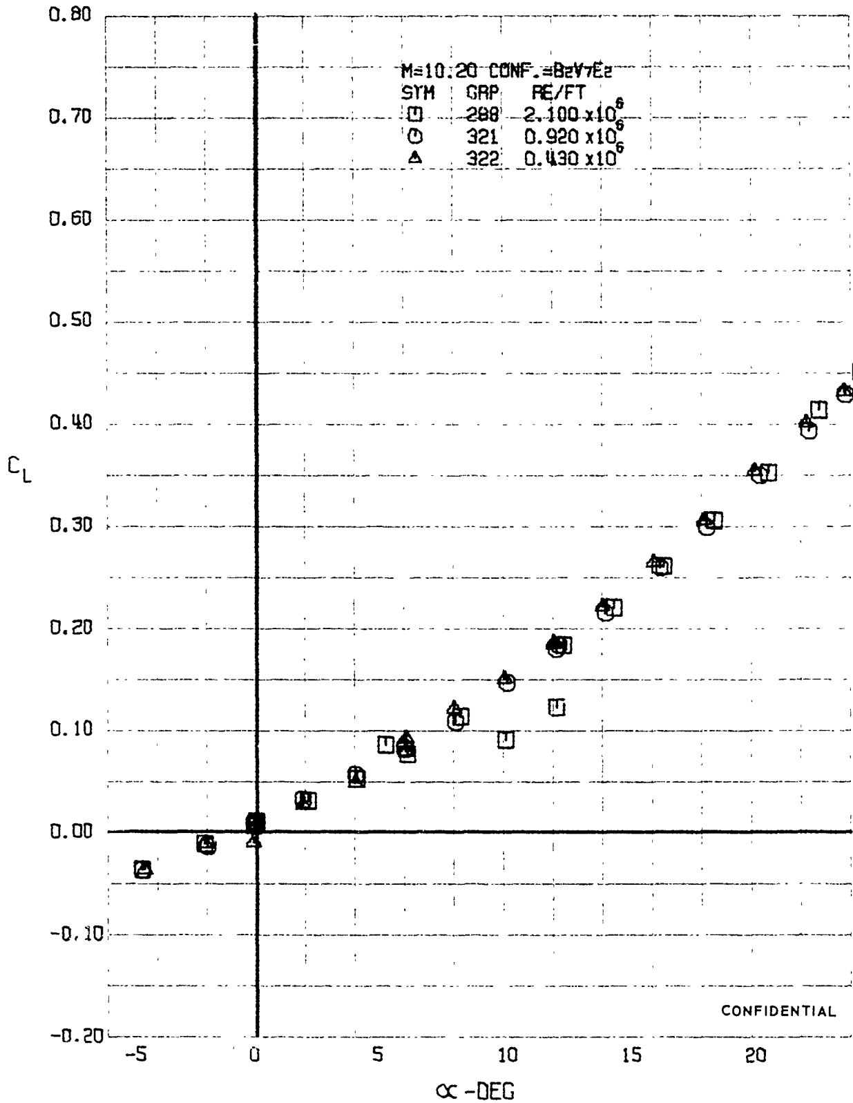
FIGURE 285 (U) REYNOLDS NUMBER EFFECTS - LIFT COEFFICIENT VARIATION WITH ANGLE OF ATTACK (M=10.20)
