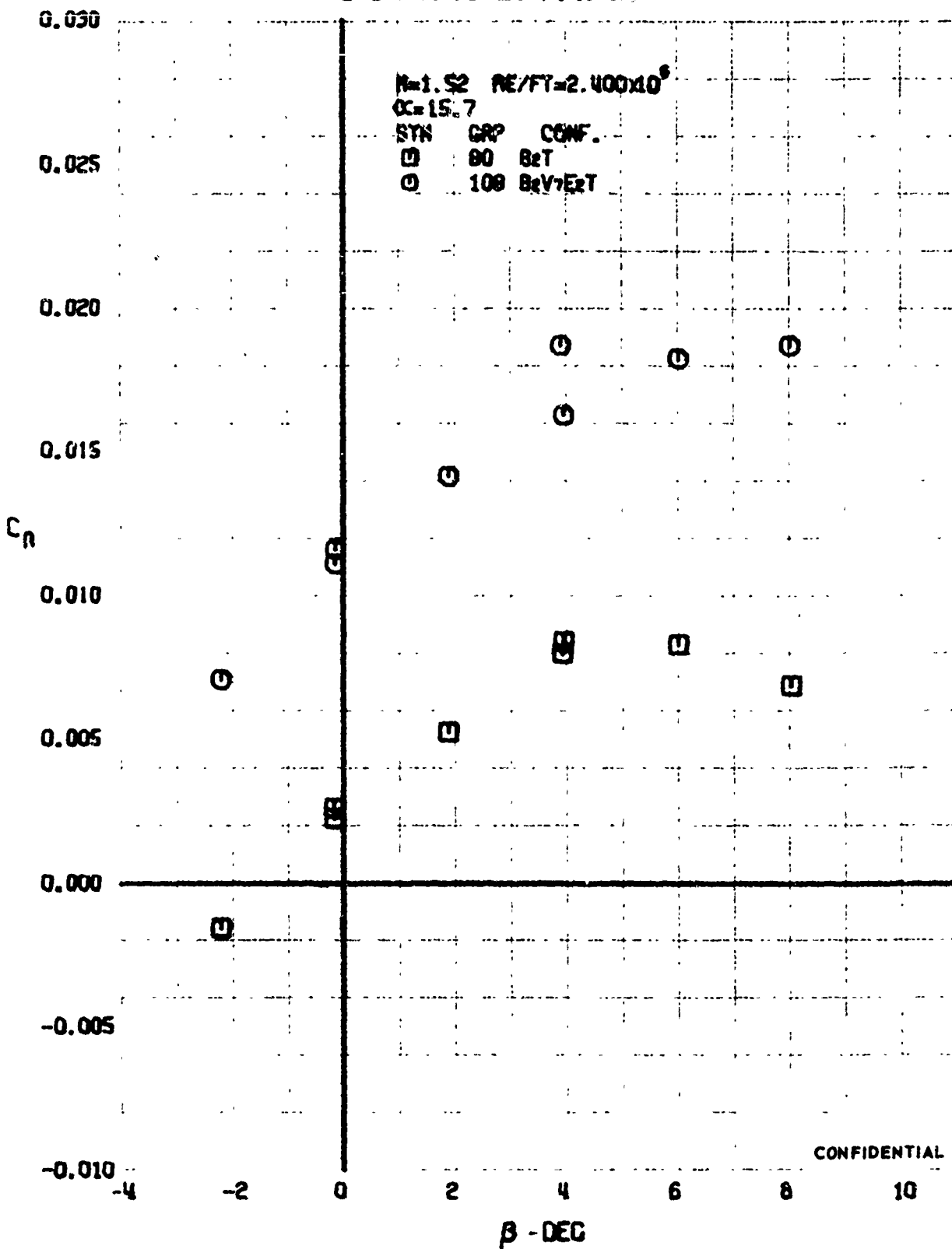
FIGURE 30 (U) CONFIGURATION BUILDUP - YAWING MOMENT COEFFICIENT VARIATION WITH ANGLE OF YAW ( N=1.52 )
