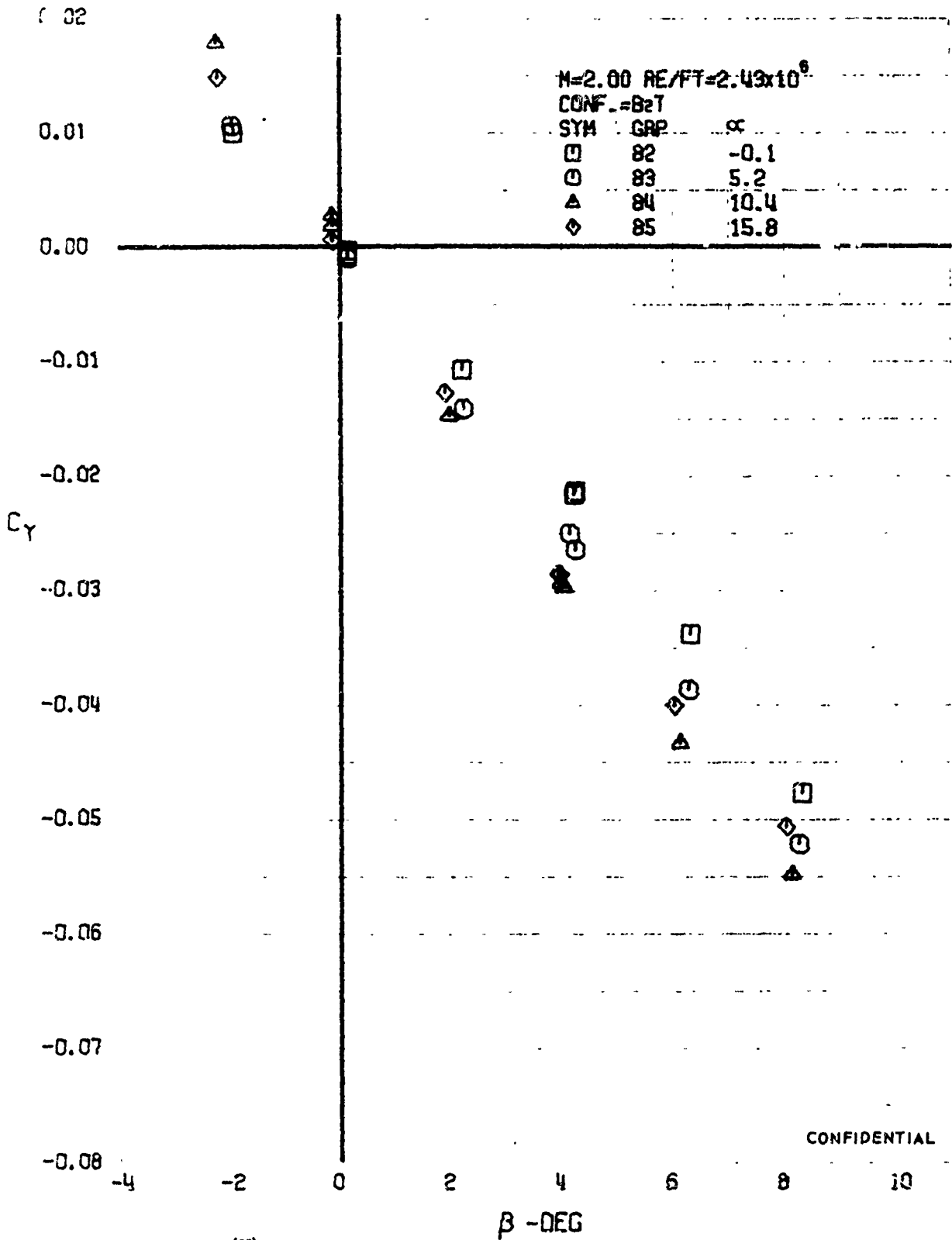
FIGURE 64 (U) BODY ALONE - SIDE FORCE COEFFICIENT VARIATION WITH ANGLE OF YAW (M=2.00)
