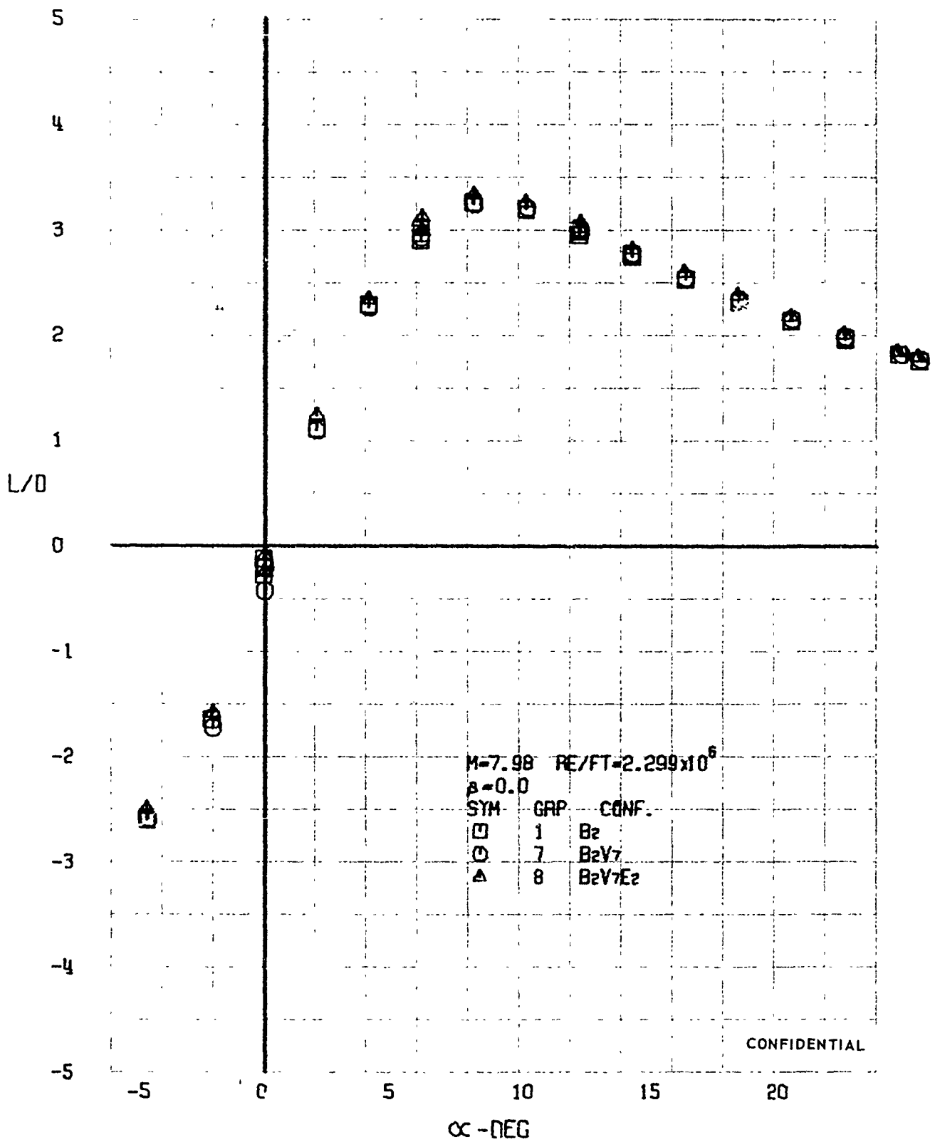
FIGURE 214 (U) CONFIGURATION BUILDUP - LIFT-DRAG RATIO VARIATION WITH ANGLE OF ATTACK ( M=7.98 )
