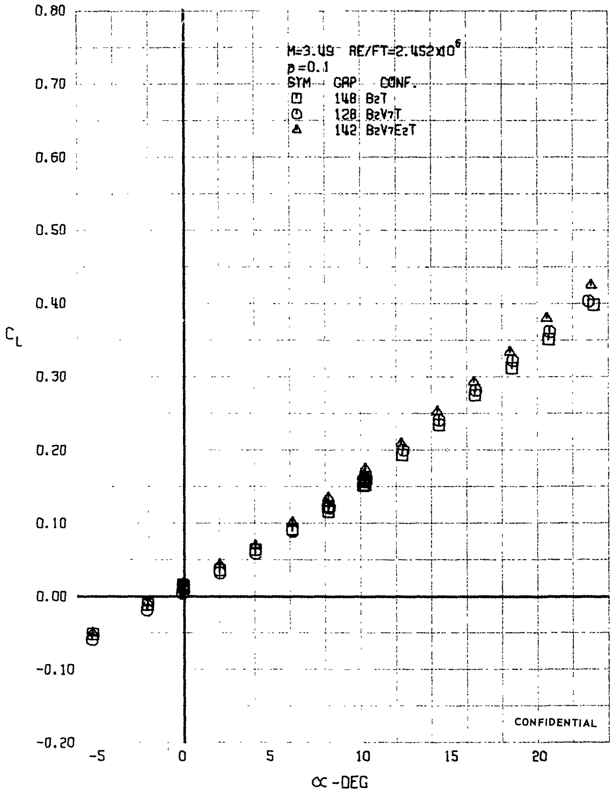
FIGURE 154 (U) CONFIGURATION BU10P - LIFT COEFFICIENT VARIATION WITH ANGLE OF ATTACK (M=3.49)
