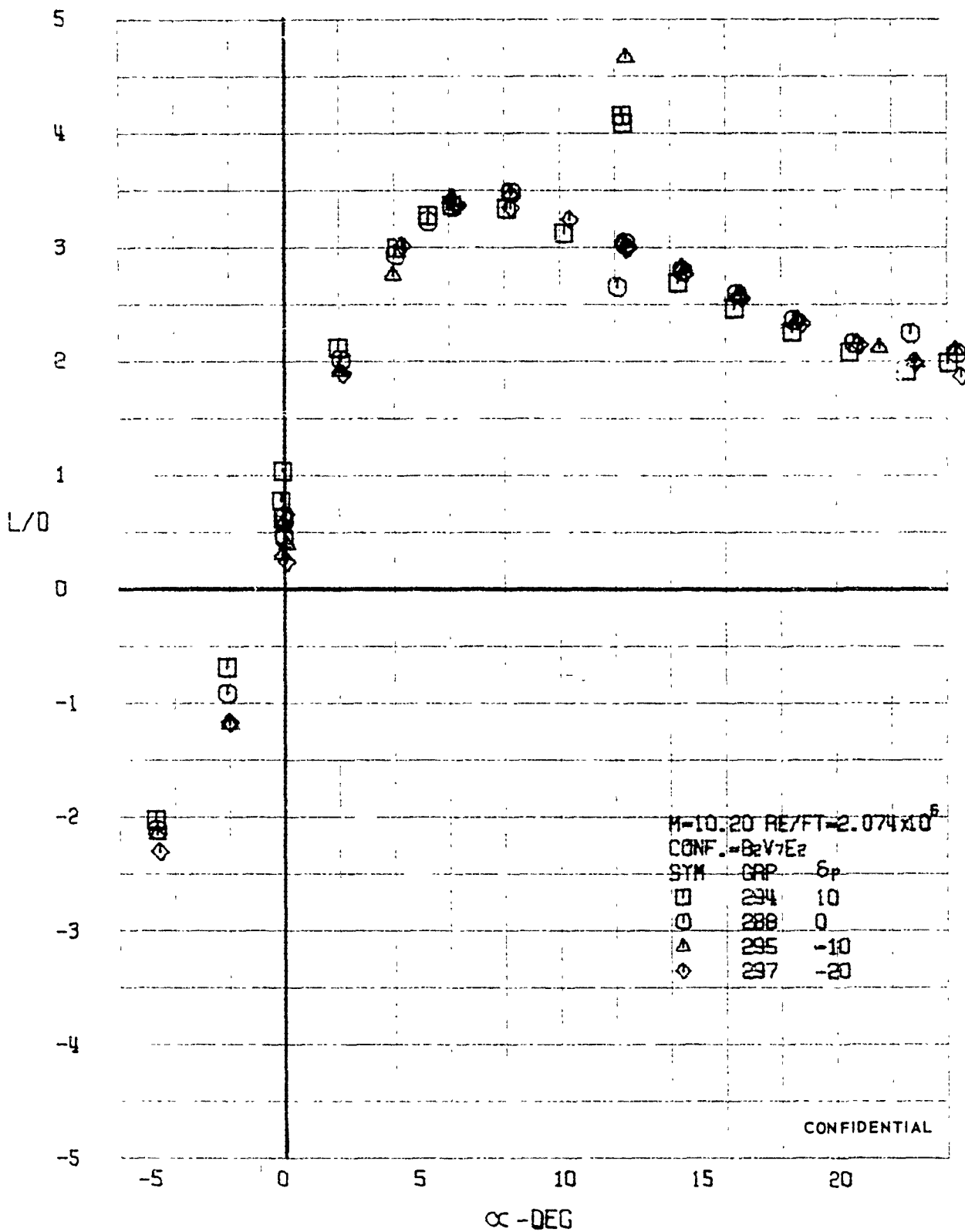
FIGURE 266 (U) ELEVON EFFECTS - LIFT-DRAG RATIO VARIATION WITH ANGLE OF ATTACK ( M=10.20 )
