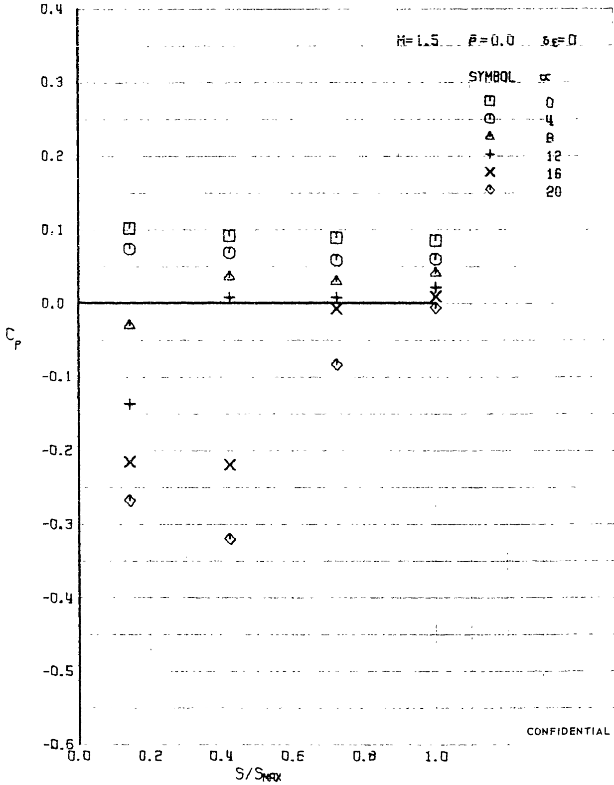
FIGURE 332 (U) UPPER SURFACE SPANWISE PRESSURES AT X/L = 0.15
