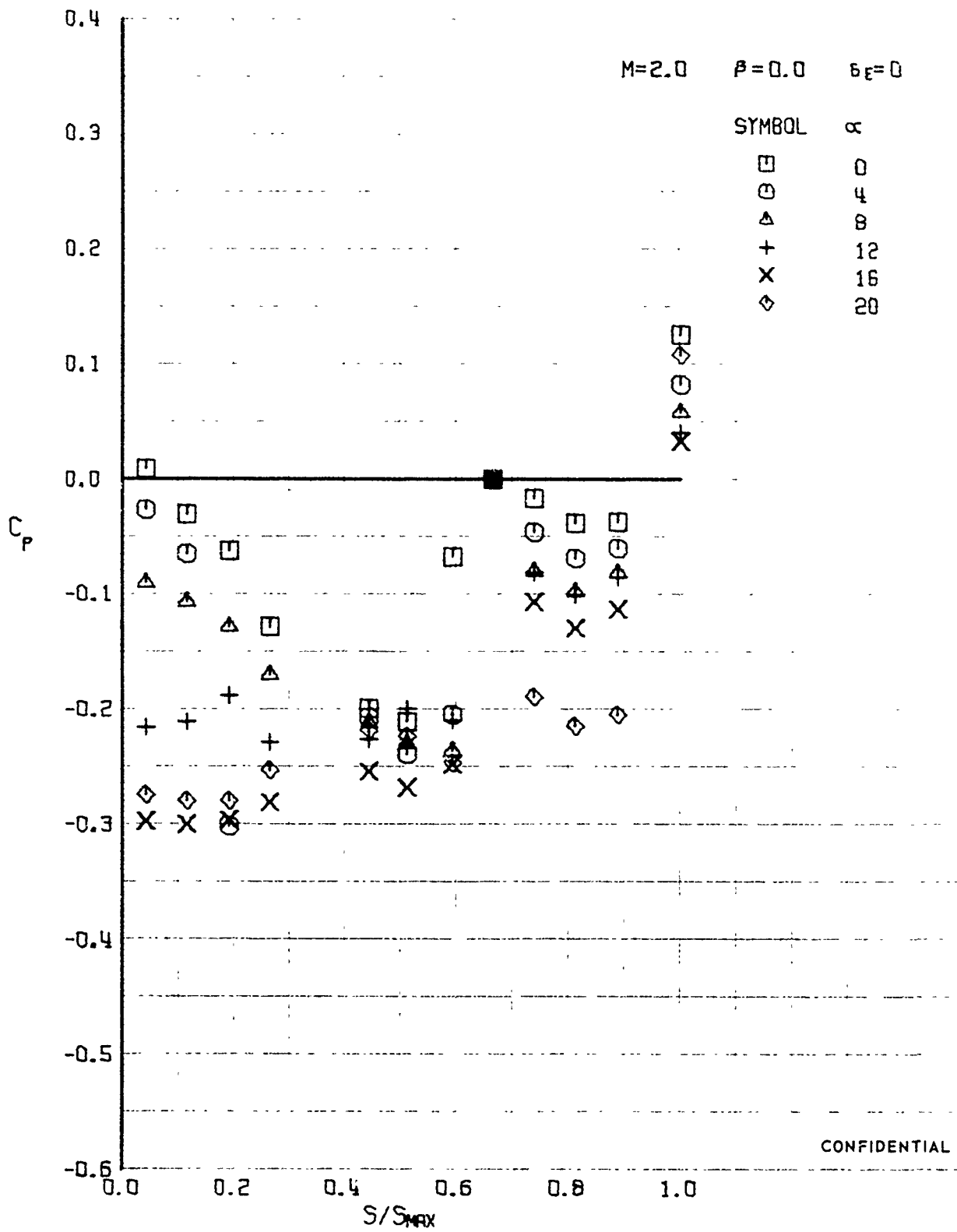
FIGURE 350 (U) UPPER SURFACE SPANWISE PRESSURES AT x/L = 0.96
