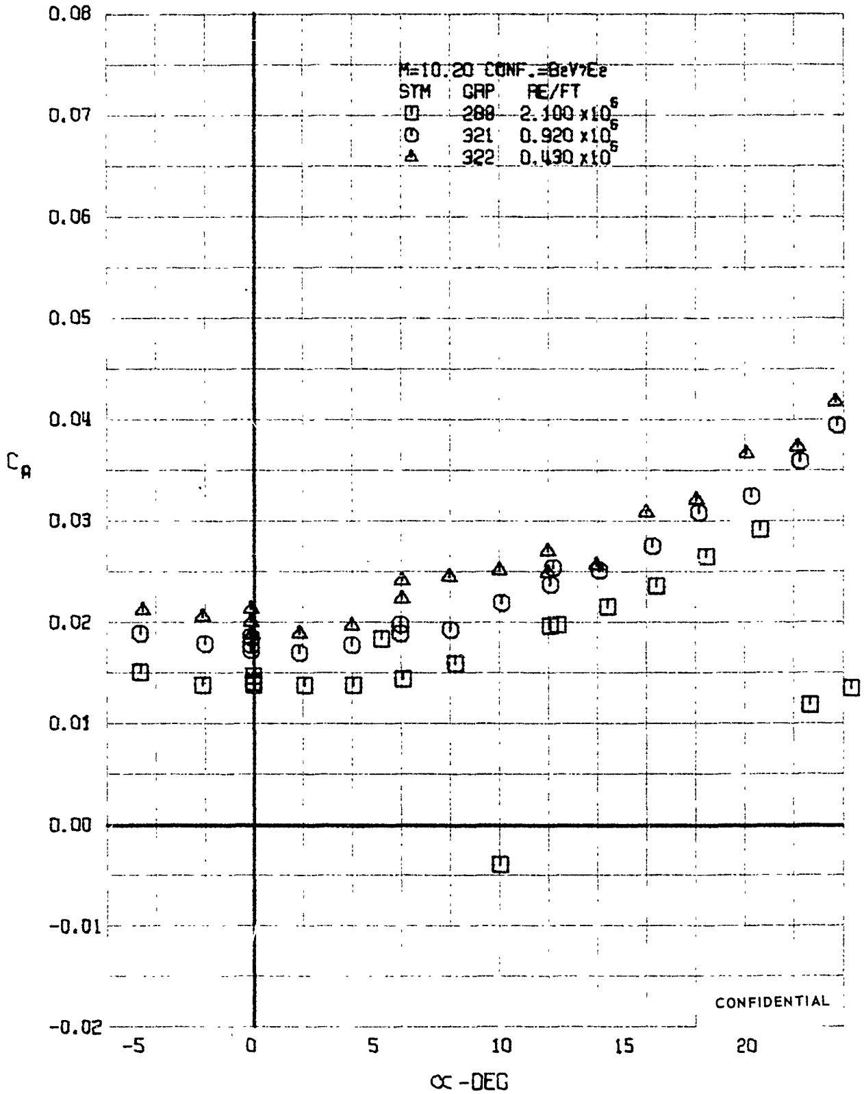
FIGURE 281 (U) REYNOLDS NUMBER EFFECTS - AXIAL FORCE COEFFICIENT VARIATION WITH ANGLE OF ATTACK (M=10.20)
