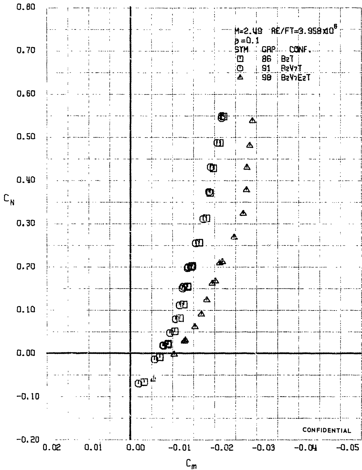
FIGURE 105 (U) CONFIGURATION BUILDUP - LONGITUDINAL STABILITY VARIATION (M=2.49)
