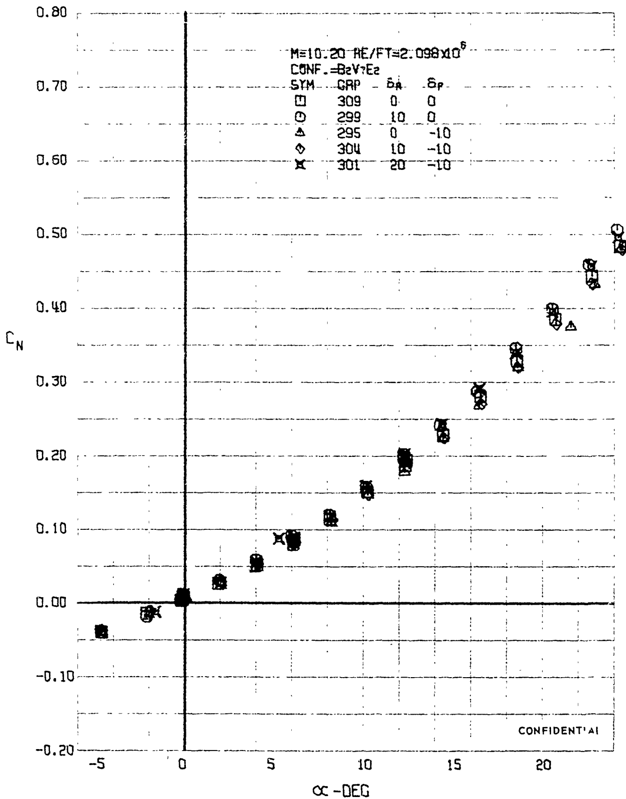
FIGURE 272 (U) AILERON EFFECTS - NORMAL FORCE COEFFICIENT VARIATION WITH ANGLE OF ATTACK (M=10.20)
