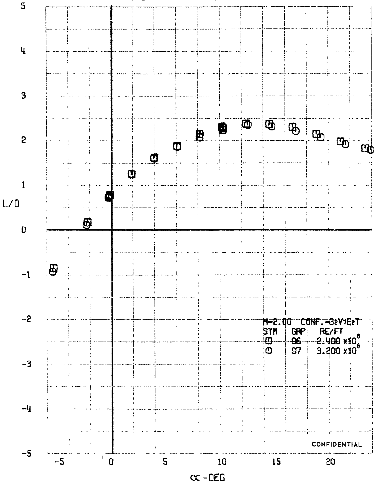
FIGURE 97 (U) REYNOLDS NUMBER EFFECTS - LIFT-DRAGE RATIO VARIATION WITH ANGLE OF ATTACK ( M=2.00 )
