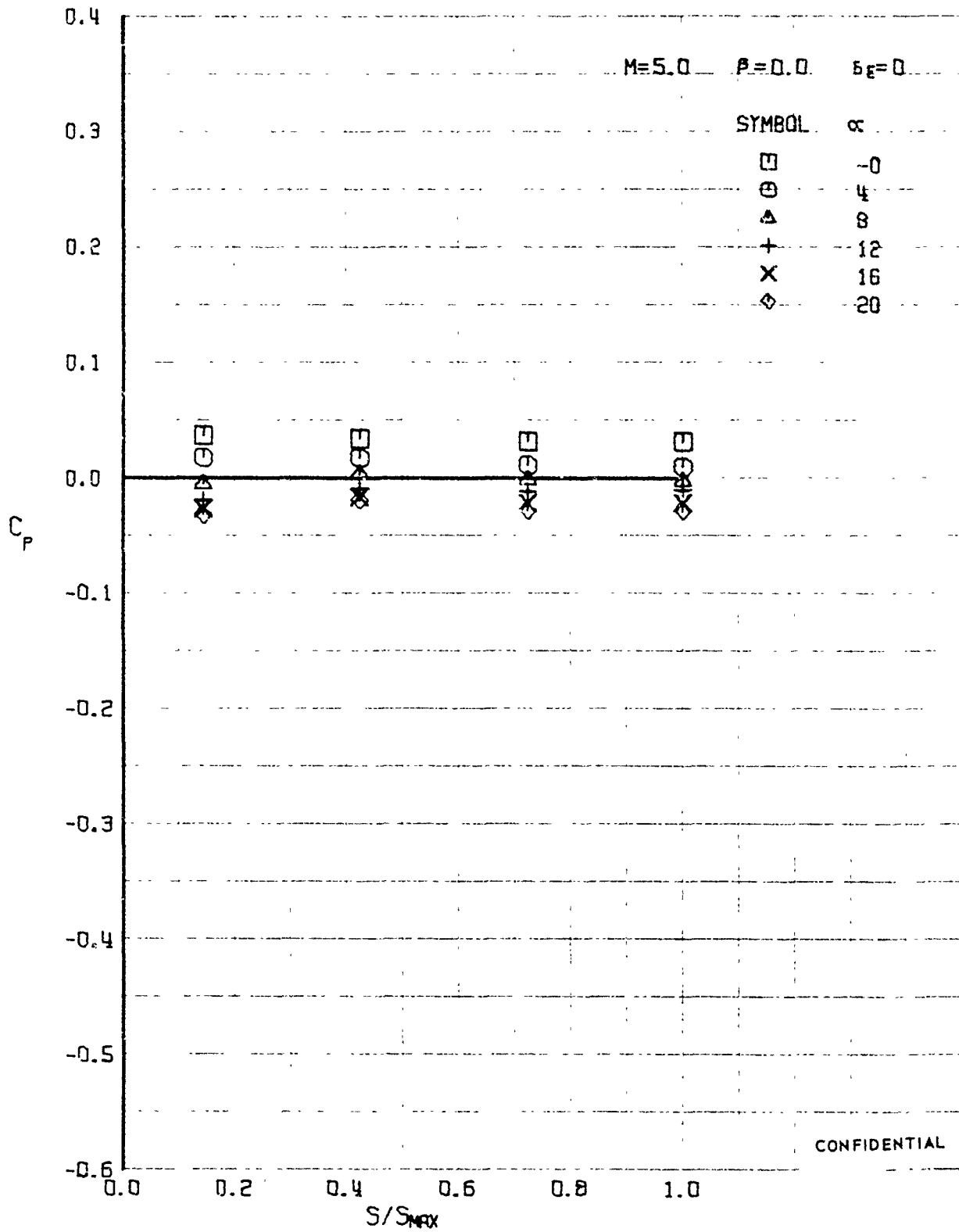
FIGURE 384 (U) UPPER SURFACE SPANWISE PRESSURES AT x/L = 0.15
