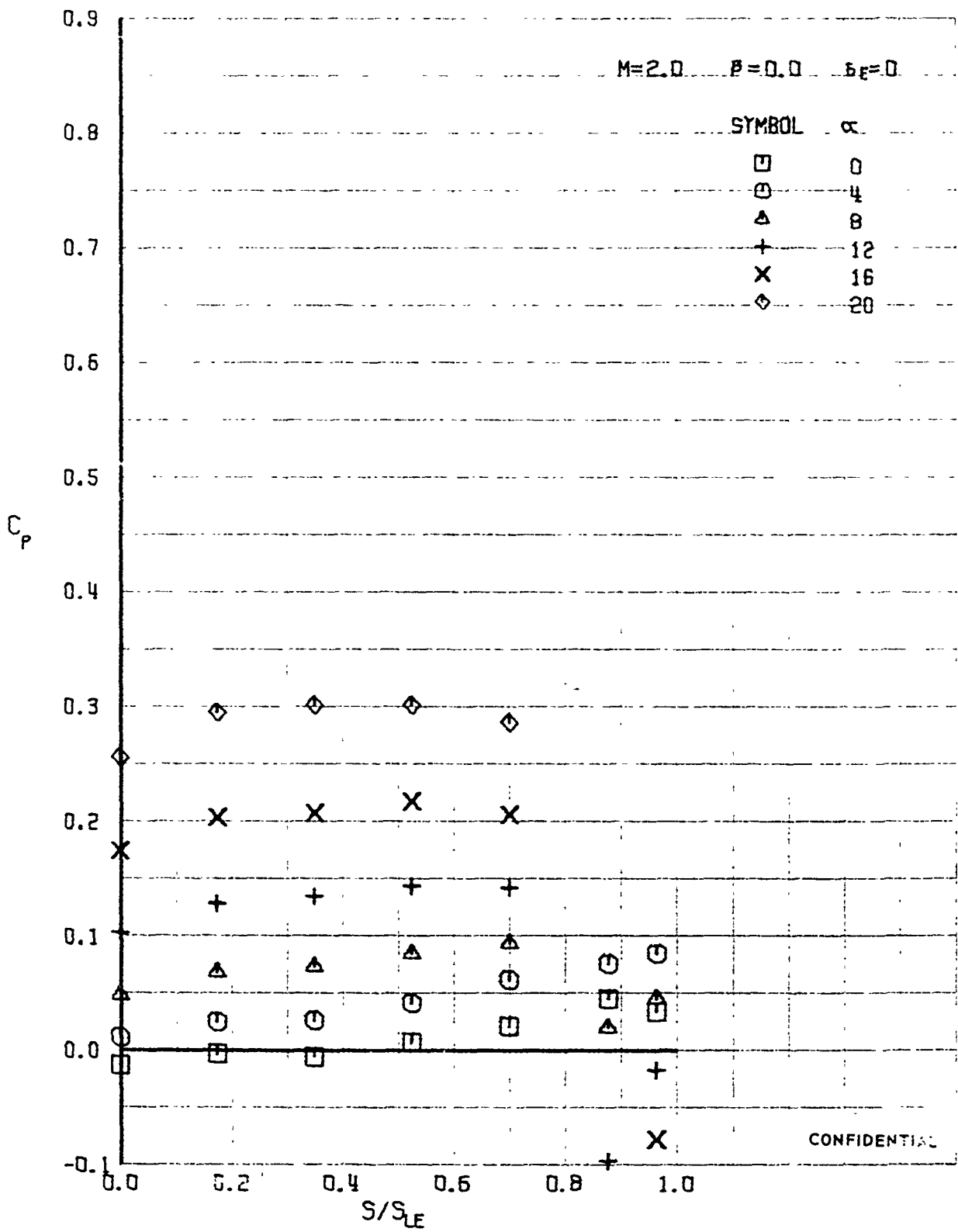
FIGURE 342 (U) LOWER SURFACE SPANWISE PRESSURES AT X/L = 0.7
