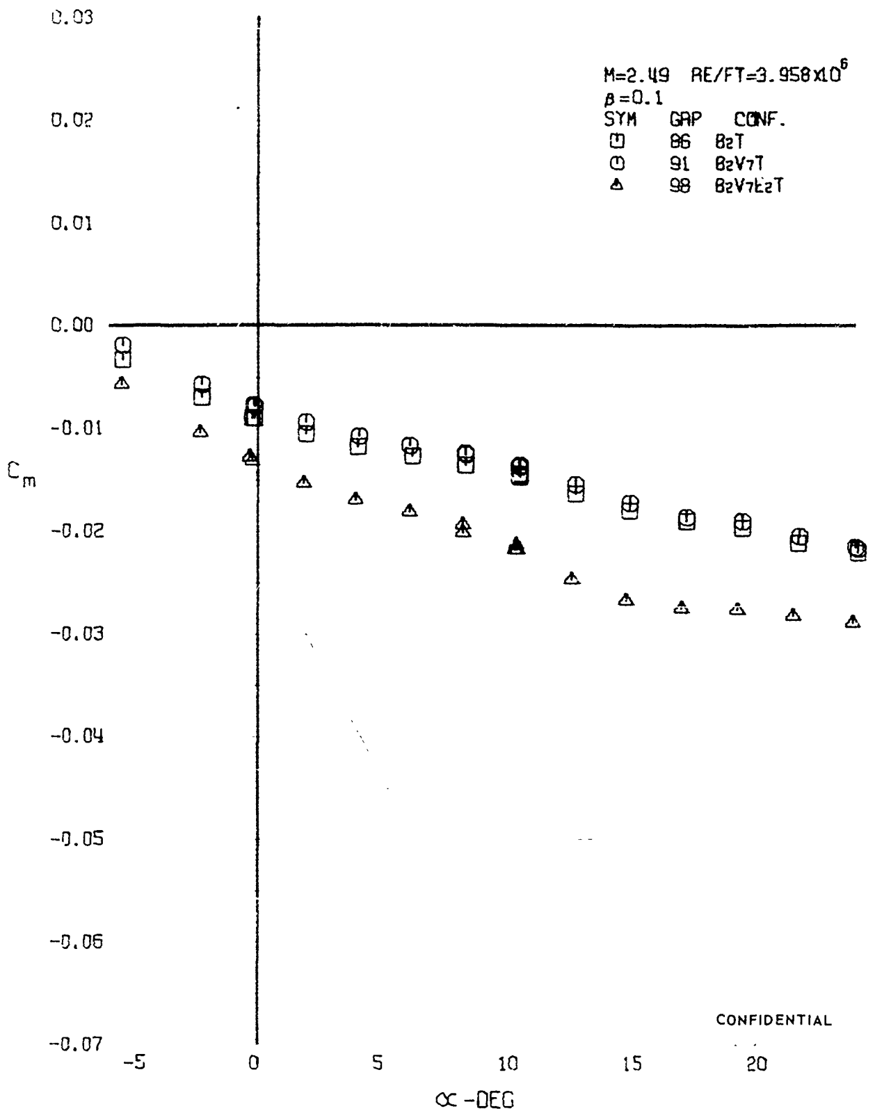
FIGURE 1 (U) CONFIGURATION BUILDUP - PITCHING MOMENT COEFFICIENT VARIATION WITH ANGLE OF ATTACK (M=2.49)
