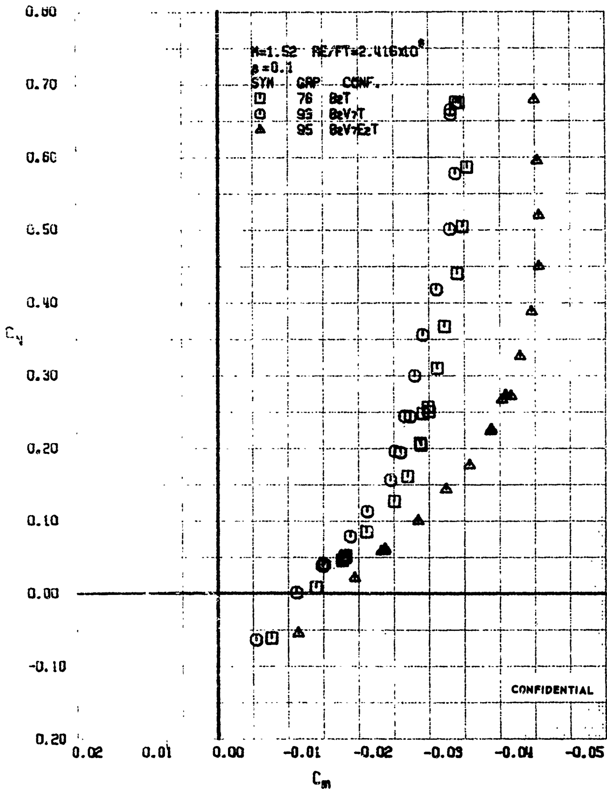
FIGURE 19 (U) CONFIGURATION BUILDUP - LONGITUDINAL STABILITY VARIATION (M=1.52)
