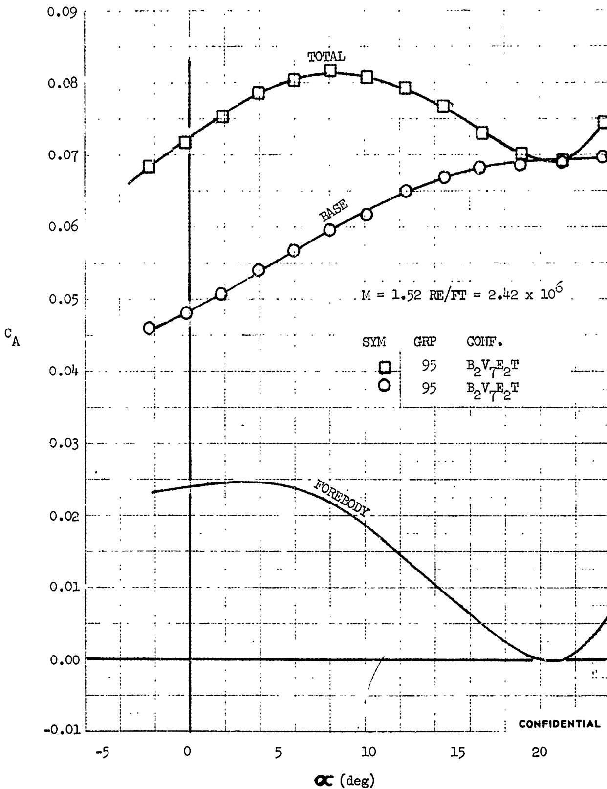
FIGURE 14 (U) AXIAL FORCE BUILDUP - AXIAL FORCE COEFFICIENT VARIATION WITH ANGLE OF ATTACK ( M = 1.52 )
