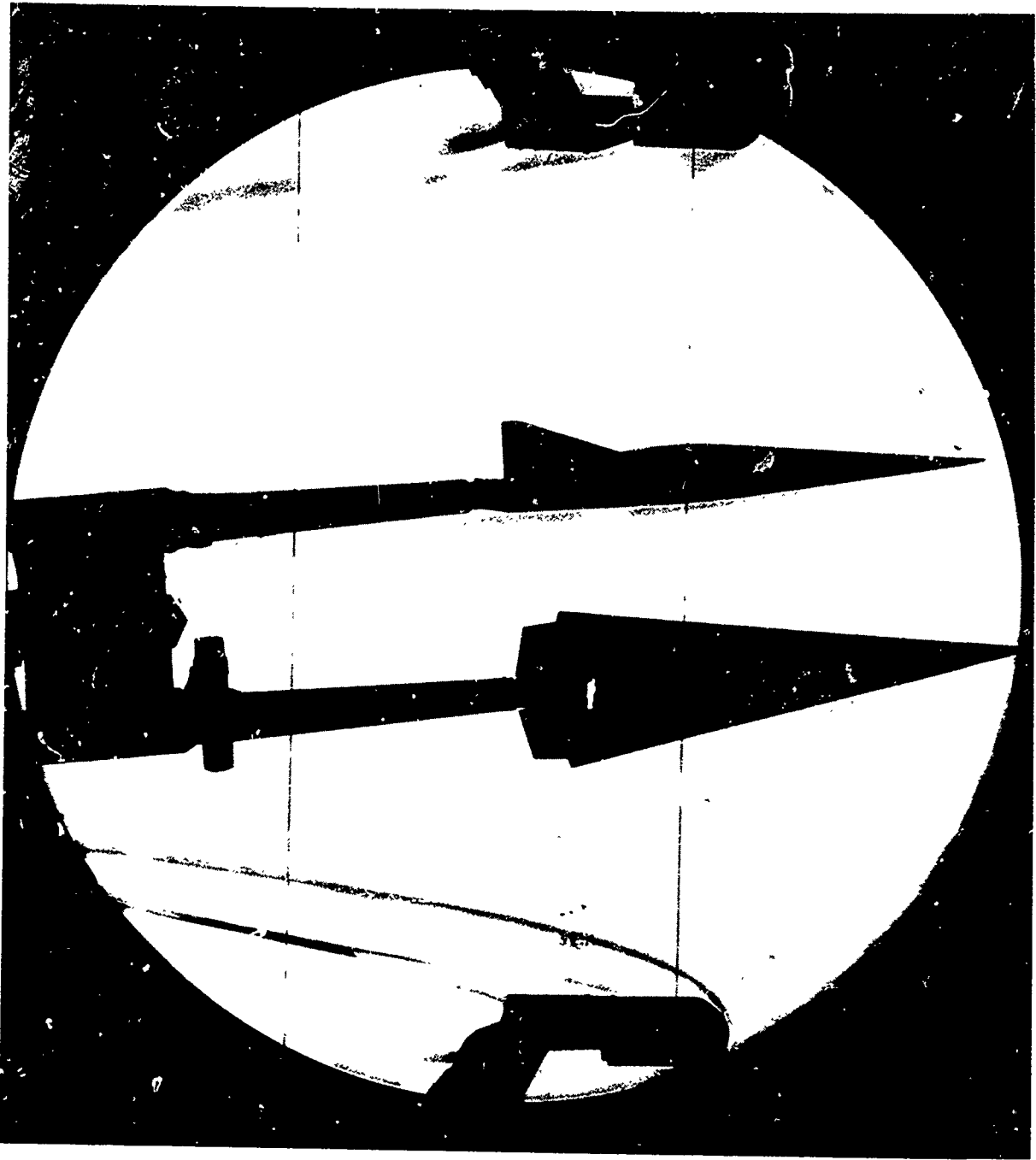
UNCLASSIFIED FIGURE 411 (U) SCHLIEREN PHOTO, 15-INCH FIBER GLASS MODEL FDL-5 DUAL INSTALLATION, M = 18.1 Upper model: \alpha = 4 \text{ deg} \beta = 0 \text{ deg} Lower model: \alpha = 0 \text{ deg} \beta = 4 \text{ deg}
