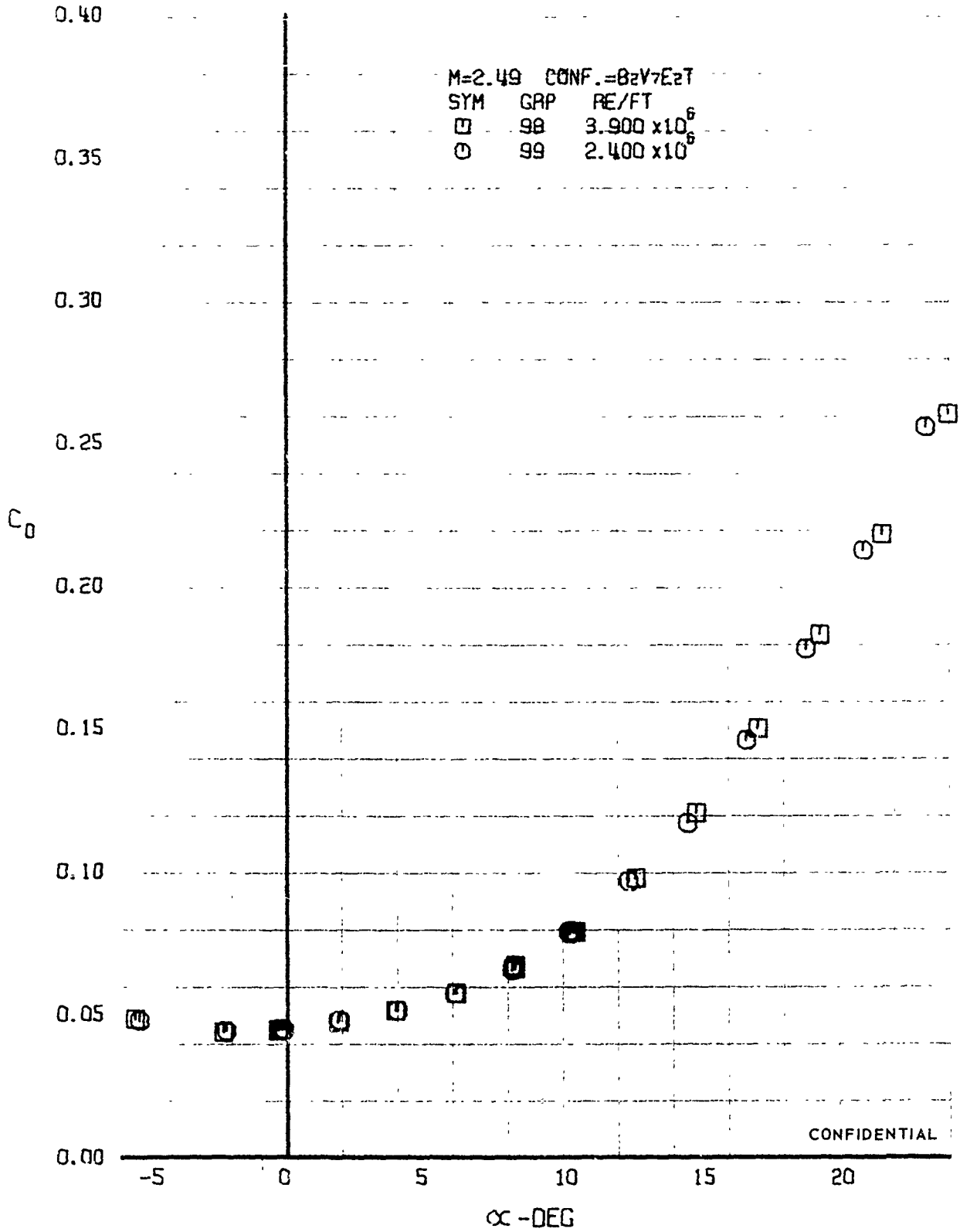
FIGURE 1-0 (U) REYNOLDS NUMBER EFFECTS - DRAG COEFFICIENT VARIATION WITH ANGLE OF ATTACK (M=2.49)
