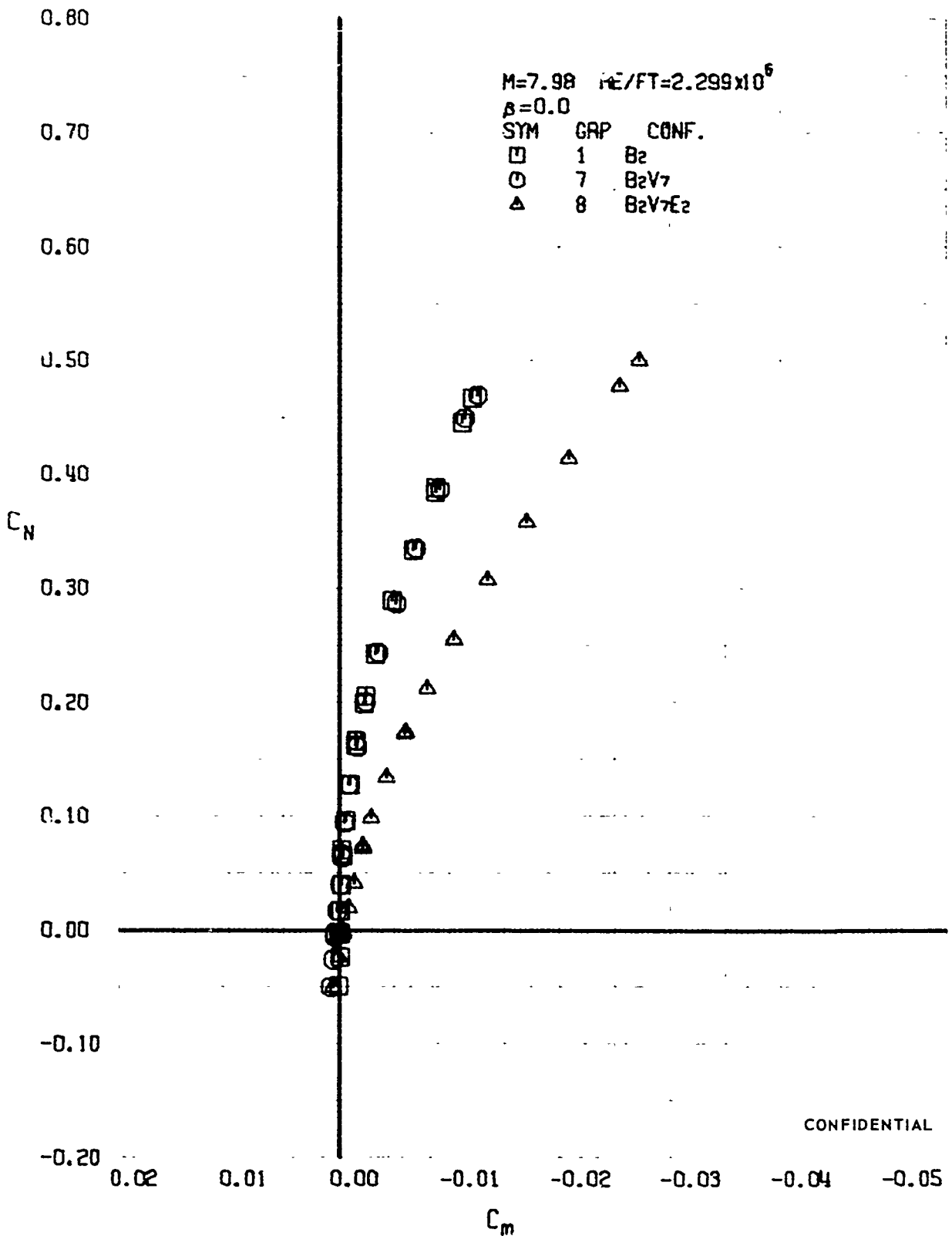
FIGURE 211 (U) CONFIGURATION BUILDUP - LONGITUDINAL STABILITY VARIATION (M=7.98)
