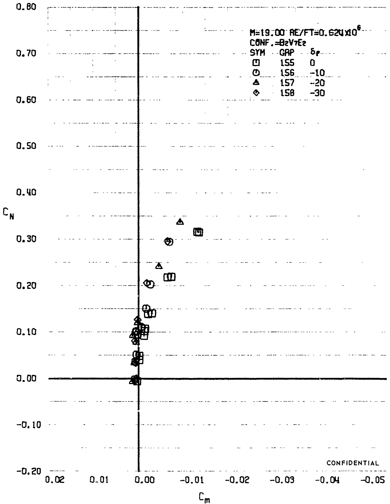
FIGURE 309 (U) ELEVON EFFECTS - LONGITUDINAL STABILITY VARIATION (M=19.00)
