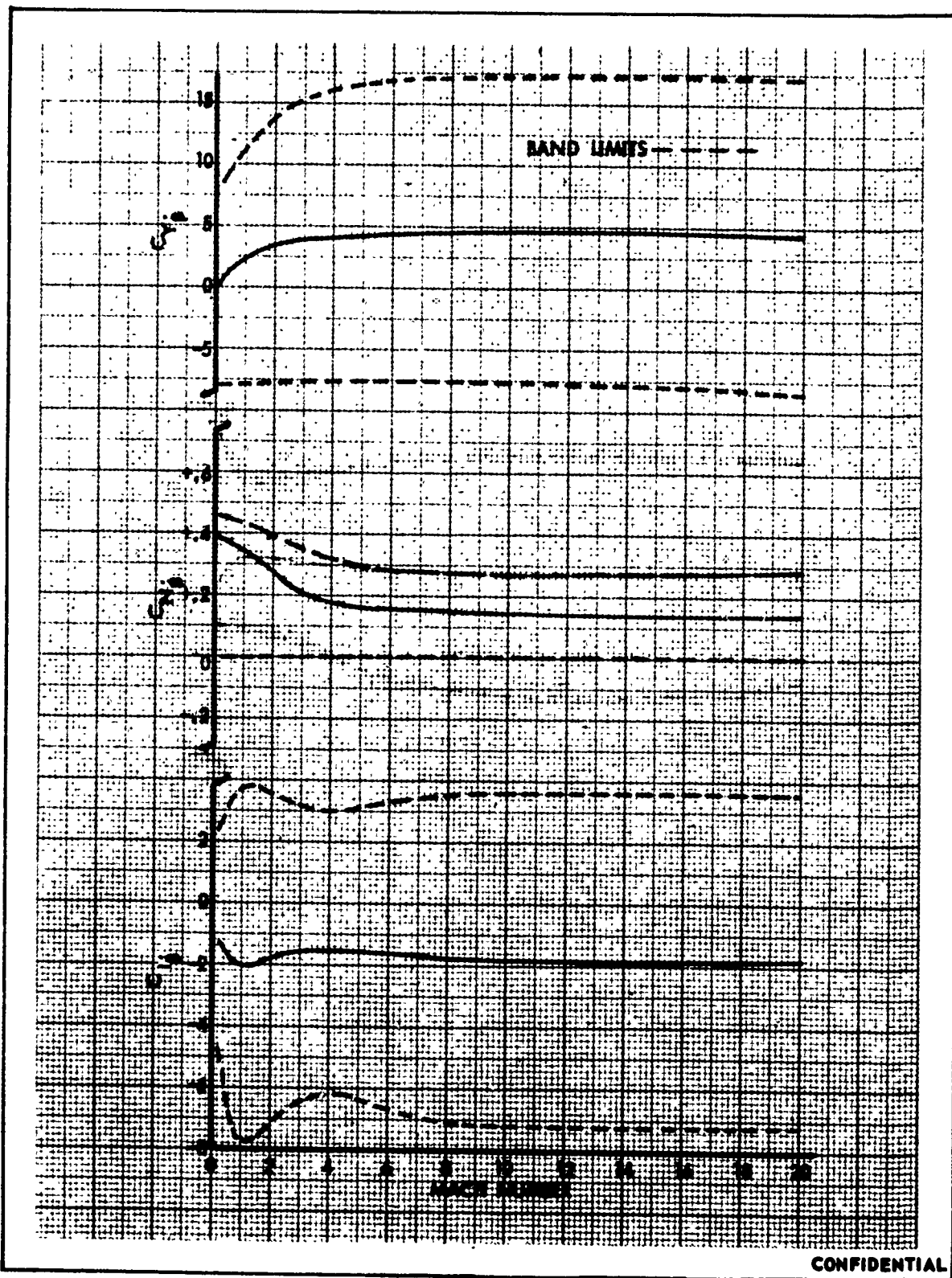
FIGURE 496 (U) VARIATION OF \beta DERIVATIVES WITH MACH NUMBER
