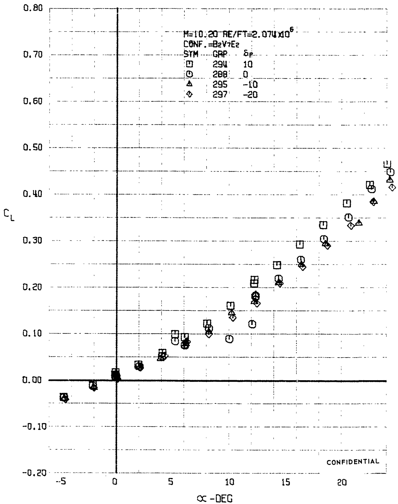
FIGURE 264 (U) ELEVON EFFECTS - LIFT COEFFICIENT VARIATION WITH ANGLE OF ATTACK (M=10.20)
