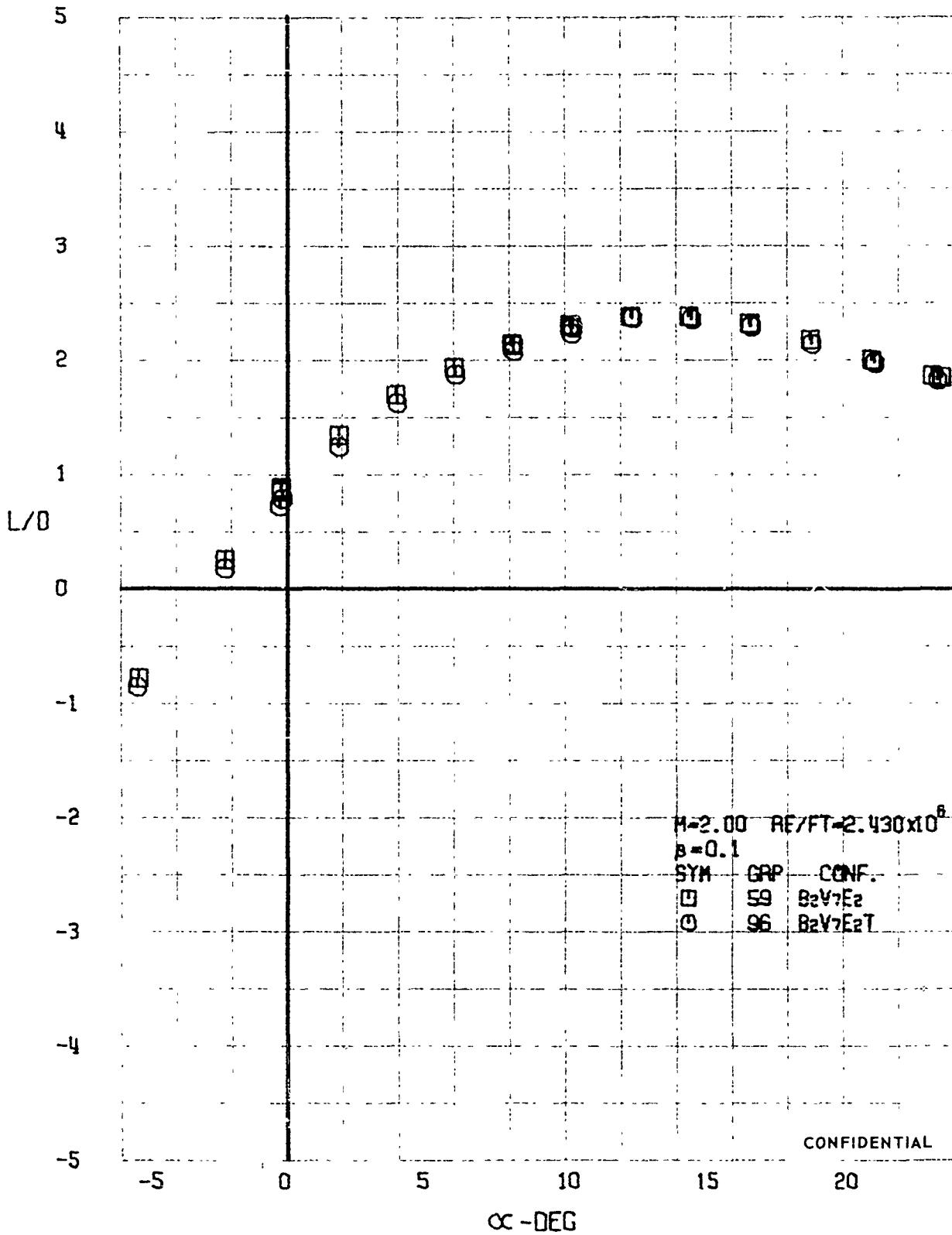
FIGURE 101 (U) FORCED TRANSITION EFFECTS - LIFT-DRAG RATIO VARIATION WITH ANGLE OF ATTACK (M=2.00)
