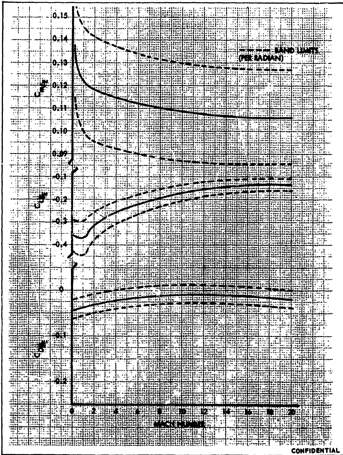
FIGURE 490 (U) VARIATION OF \delta_E DERIVATIVES WITH MACH NUMBER
