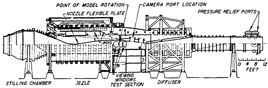
Assembly
