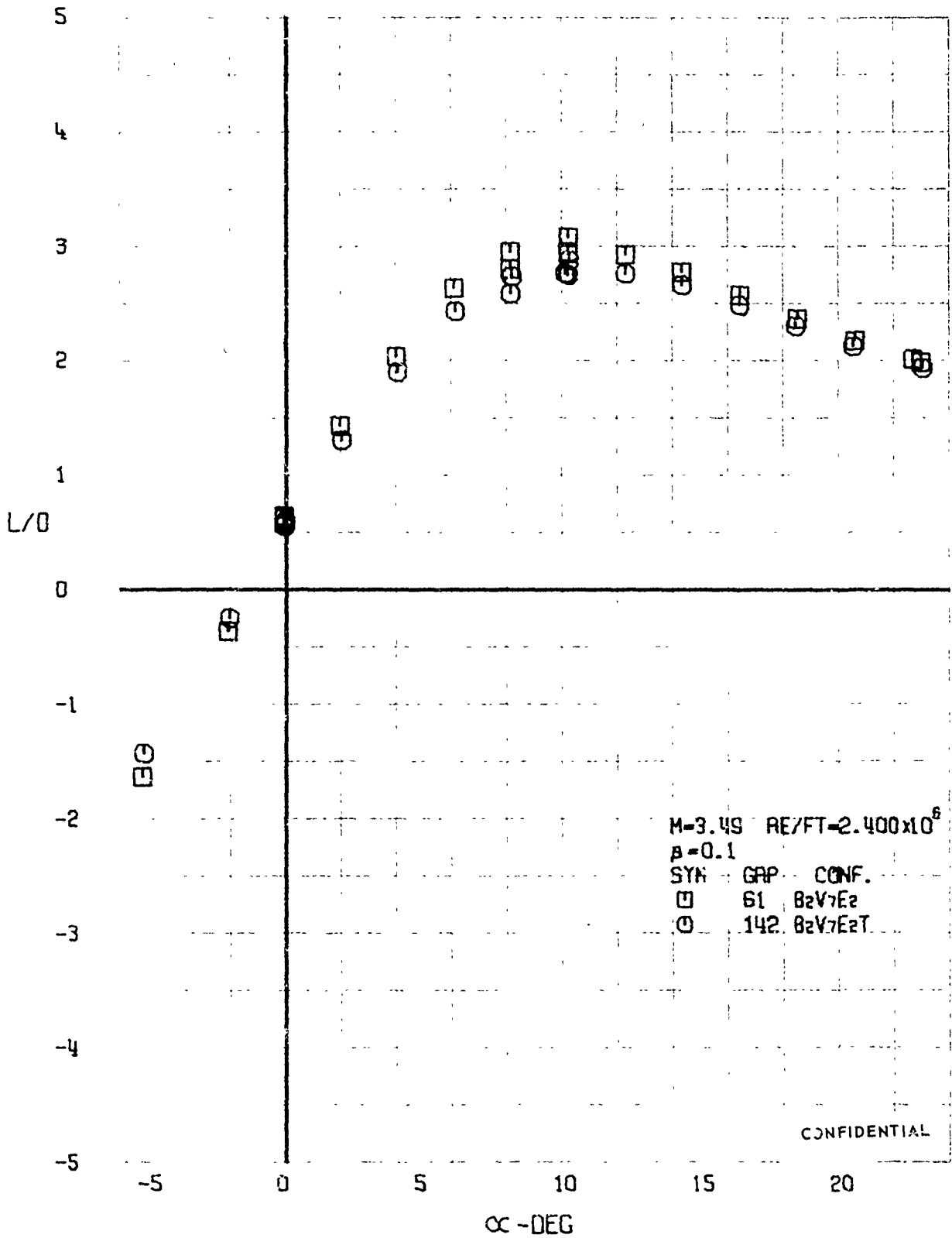
FIGURE 136 - (U) FORCED TRANSITION EFFECTS - LIFT-DRAGE RATIO VARIATION WITH ANGLE OF ATTACK ( M=3.49 )
