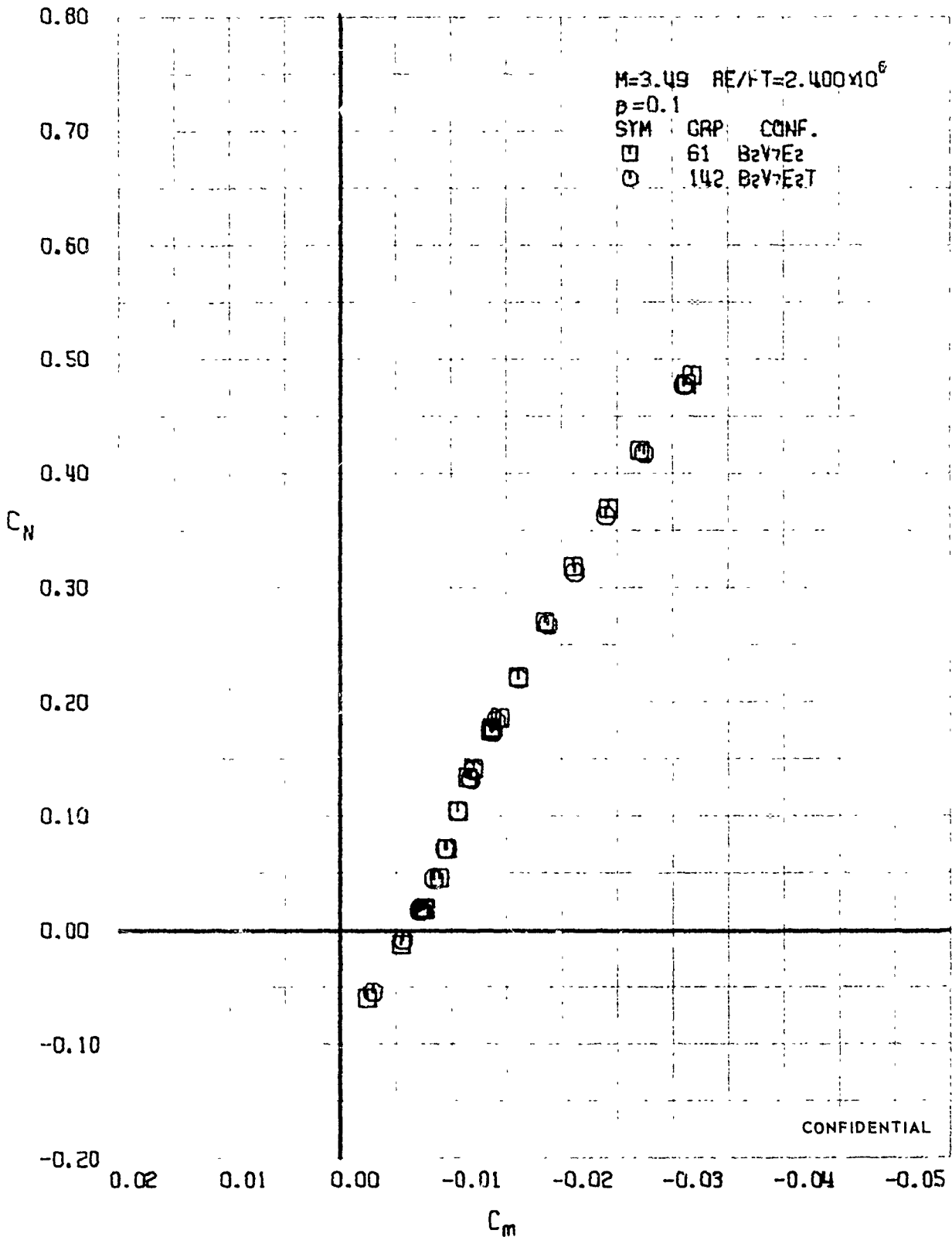
FIGURE 185 (U) FORCED TRANSITION EFFECTS - LONGITUDINAL STABILITY VARIATION (M=3.49)
