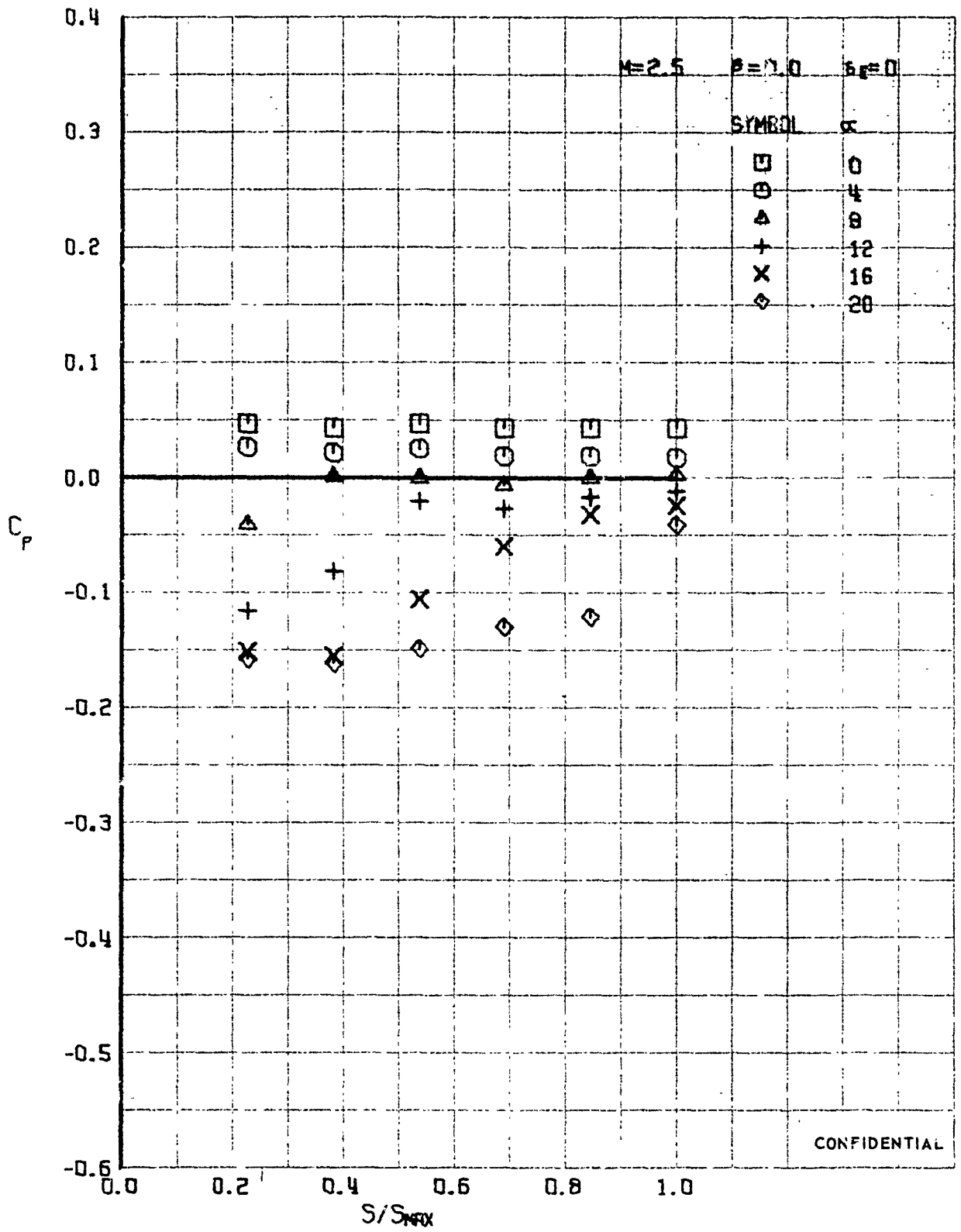
FIGURE 359 (U) UPPER SURFACE SPANWISE PRESSURES AT X/L = 0.30
