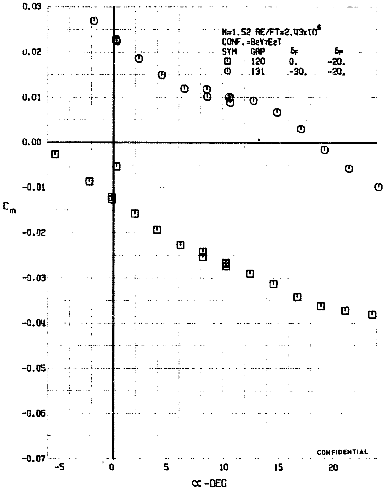
FIGURE 41 (U) FLAP EFFECTS - PITCHING MOMENT COEFFICIENT VARIATION WITH ANGLE OF ATTACK ( M=1.52 )
