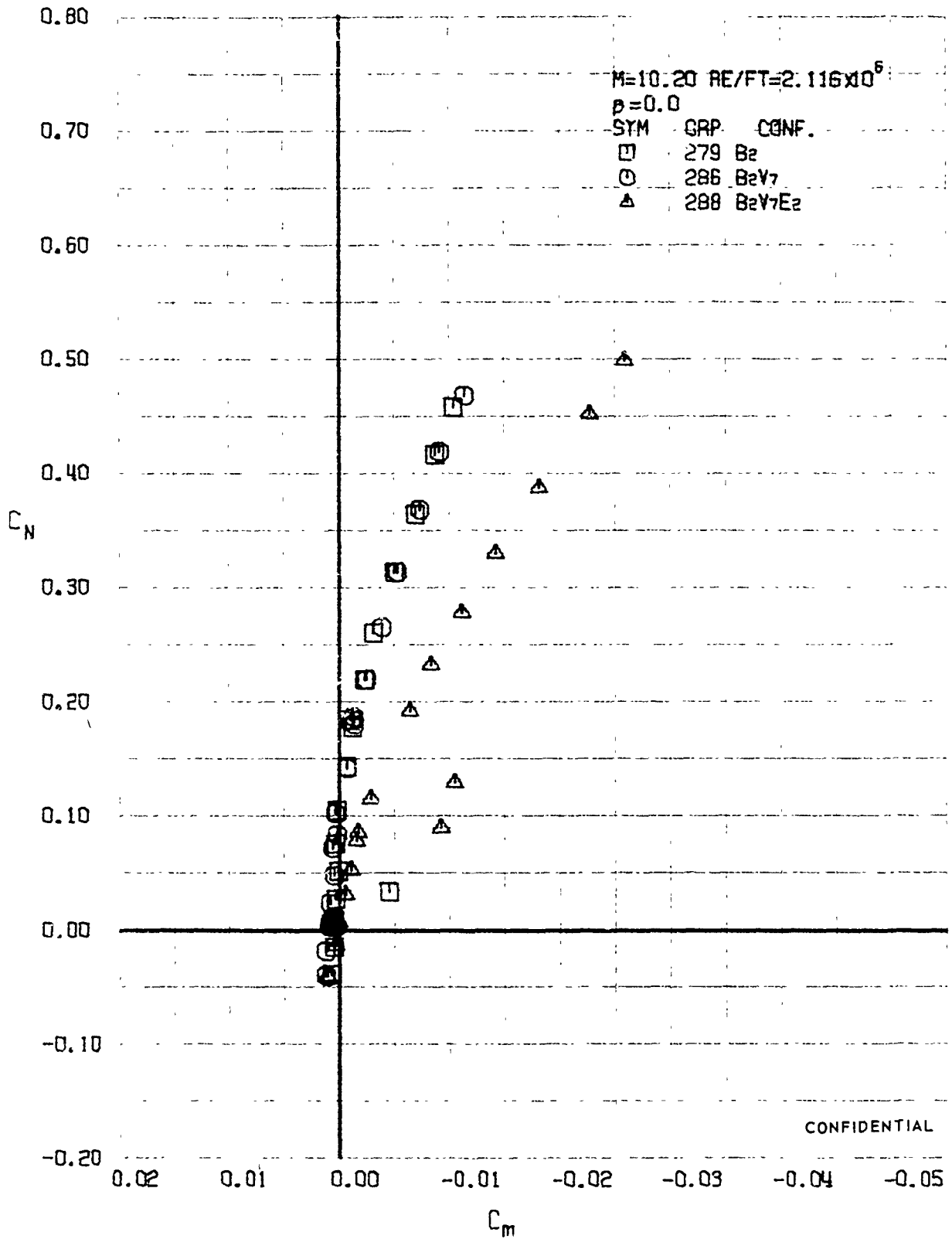
FIGURE 244 (U) CONFIGURATION BUILDUP - LONGITUDINAL STABILITY VARIATION (M=10.20)
