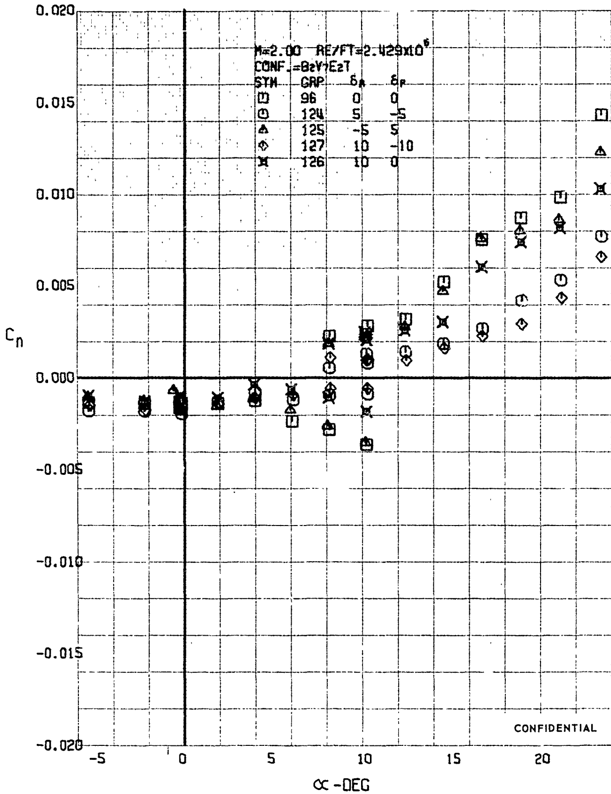
FIGURE 89 (U) RILERON EFFECTS - YAWING MOMENT COEFFICIENT VARIATION WITH ANGLE OF ATTACK ( M=2.00 )
