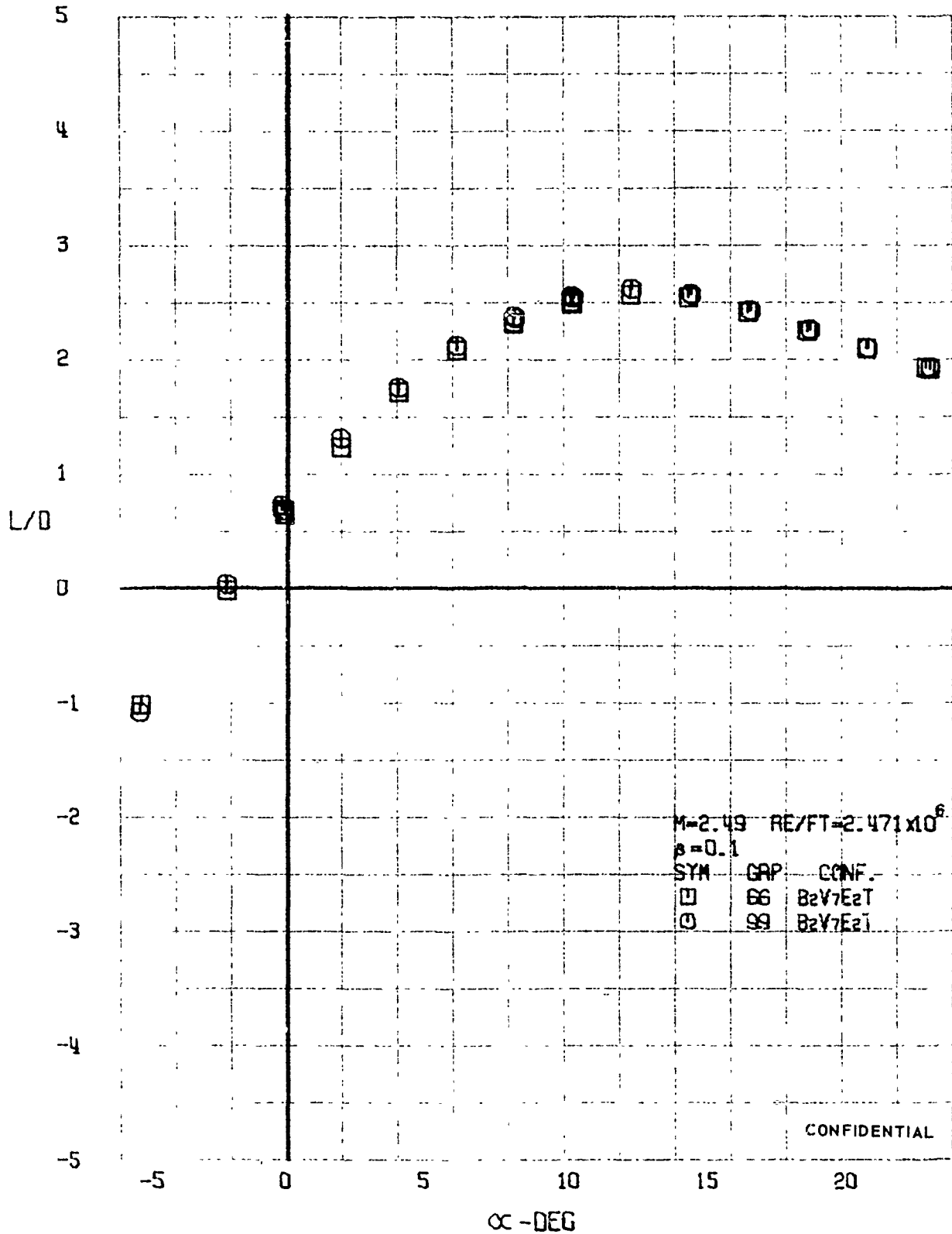
FIGURE 149 (U) REPEATABILITY - LIFT-DRAG RATIO VARIATION WITH ANGLE OF ATTACK (M=2.49)
