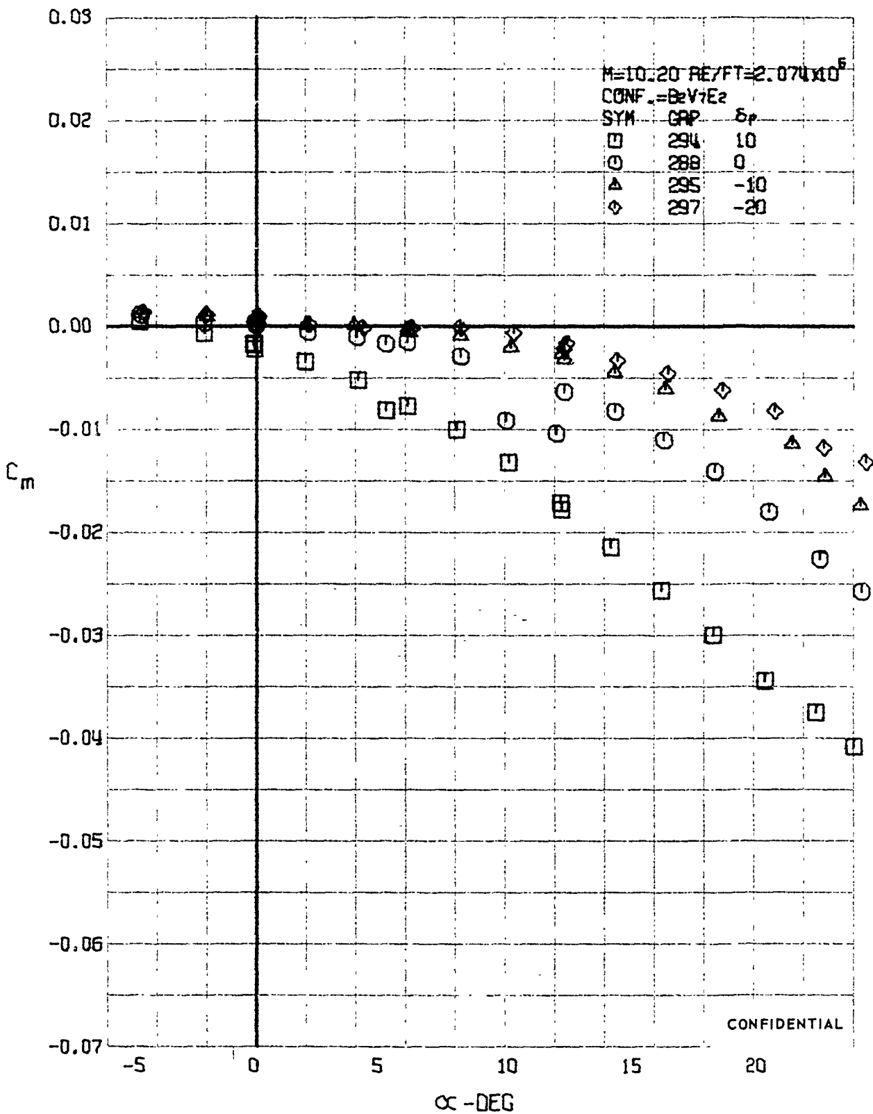
FIGURE 262 (U) ELEVON EFFECTS - PITCHING MOMENT COEFFICIENT VARIATION WITH ANGLE OF ATTACK (M=10.20)
