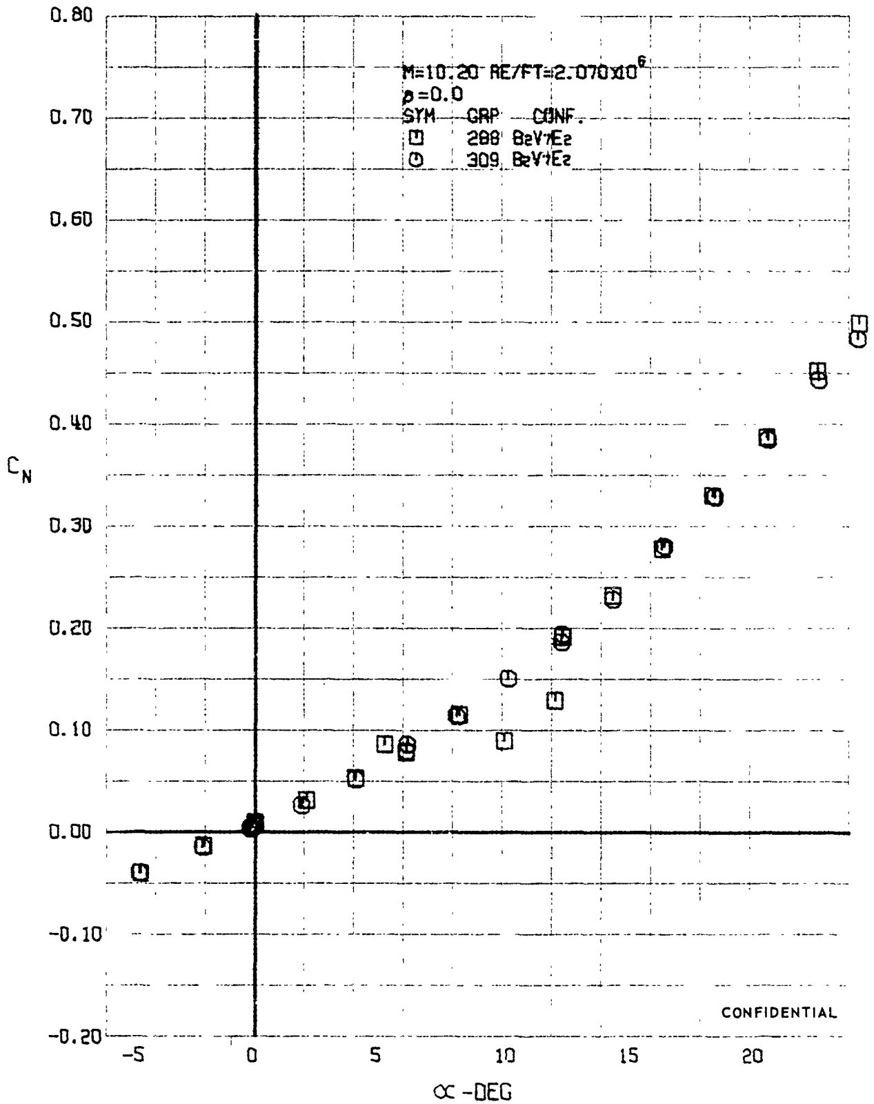
FIGURE 289 (U) REPEATABILITY - NORMAL FORCE COEFFICIENT VARIATION WITH ANGLE OF ATTACK (M=10.20)
