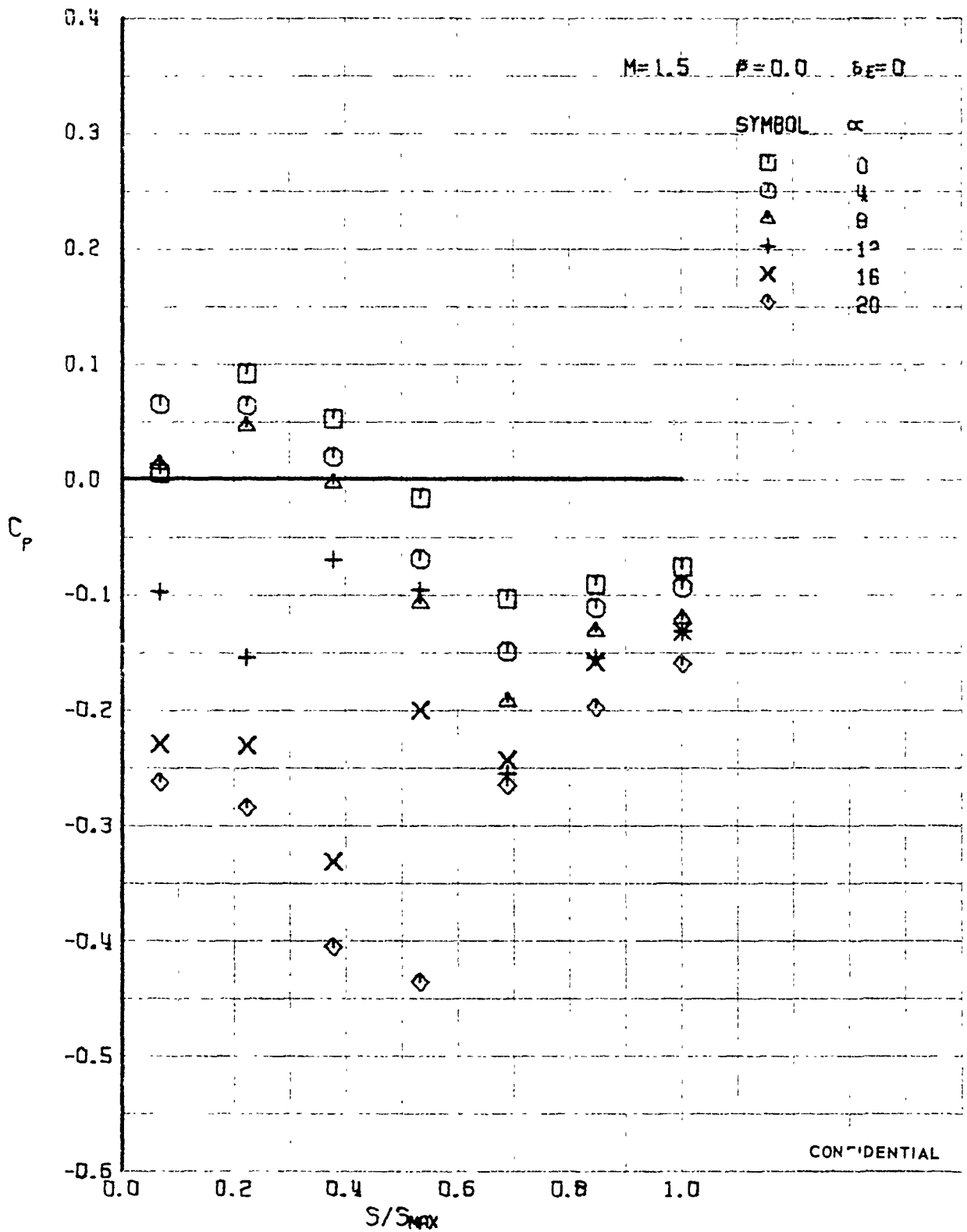
FIGURE 335 (U) UPPER SURFACE SPANWISE PRESSURES AT X/L = 0.76
