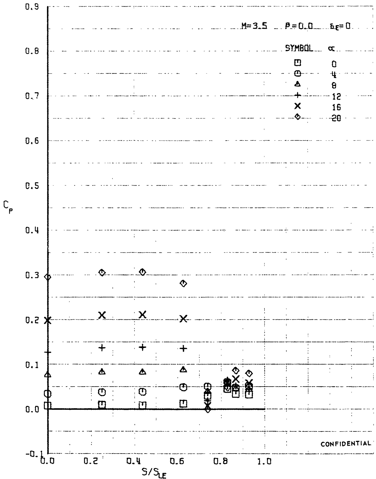
FIGURE 369 (U) LOWER SURFACE SPANWISE PRESSURES AT X/L = 0.96
