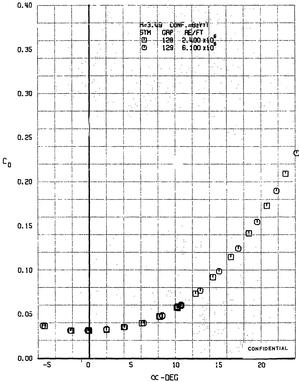
FIGURE 181 (U) REYNOLDS NUMBER EFFECTS - DRAG COEFFICIENT VARIATION WITH ANGLE OF ATTACK ( M=3.49 )
