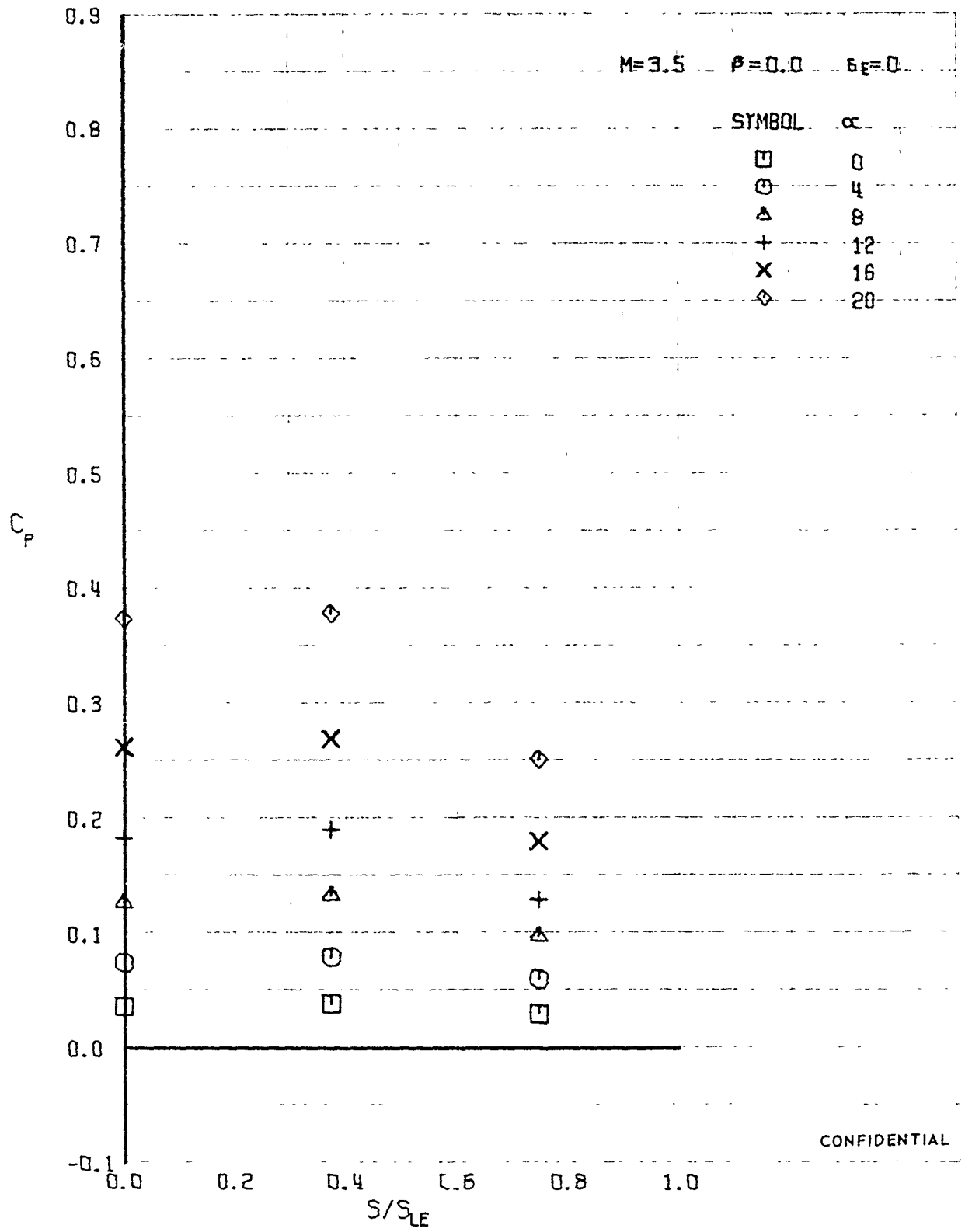
FIGURE 365 (U) LOWER SURFACE SPANWISE PRESSURES AT X/L = 0.15
