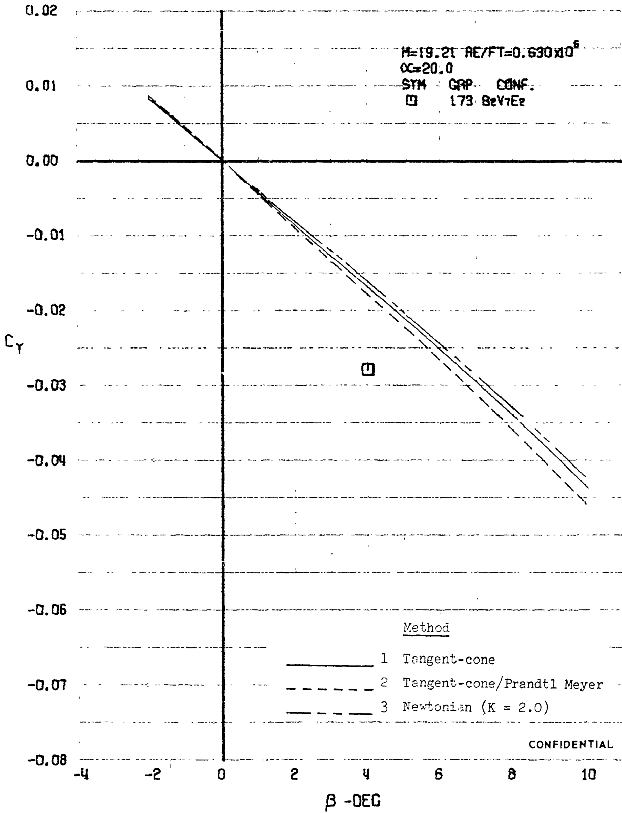
FIGURE 436 (U) COMPARISON OF ESTIMATED AND EXPERIMENTAL COEFFICIENTS - SIDE FORCE COEFFICIENT VARIATION WITH ANGLE OF YAW ( M=19.20 )
