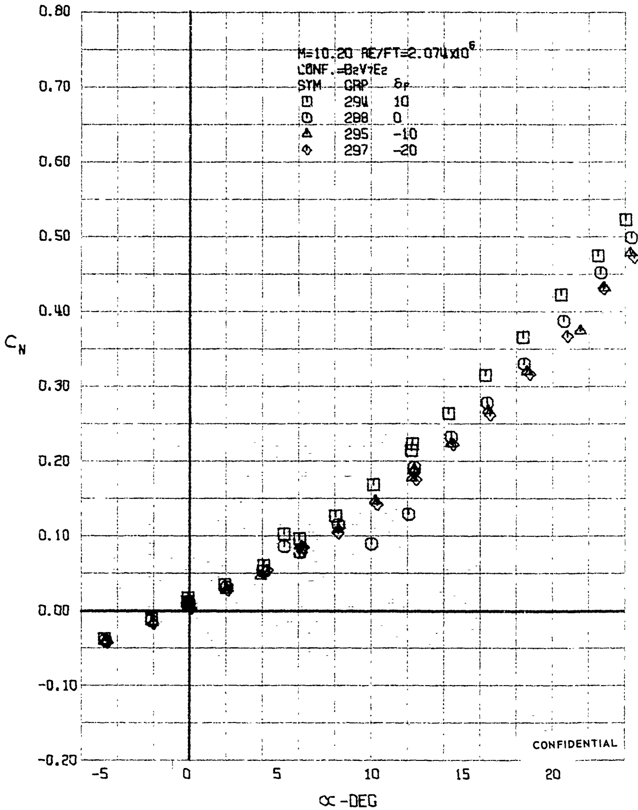
FIGURE 261 (U) ELEVON EFFECTS - NORMAL FORCE COEFFICIENT VARIATION WITH ANGLE OF ATTACK (M=10.20)
