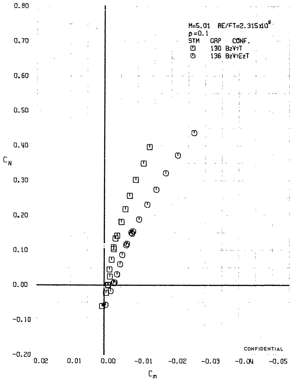
FIGURE 10 (U) CONFIGURATION BUILDUP - LONGITUDINAL STABILITY VARIATION (M=5.01)
