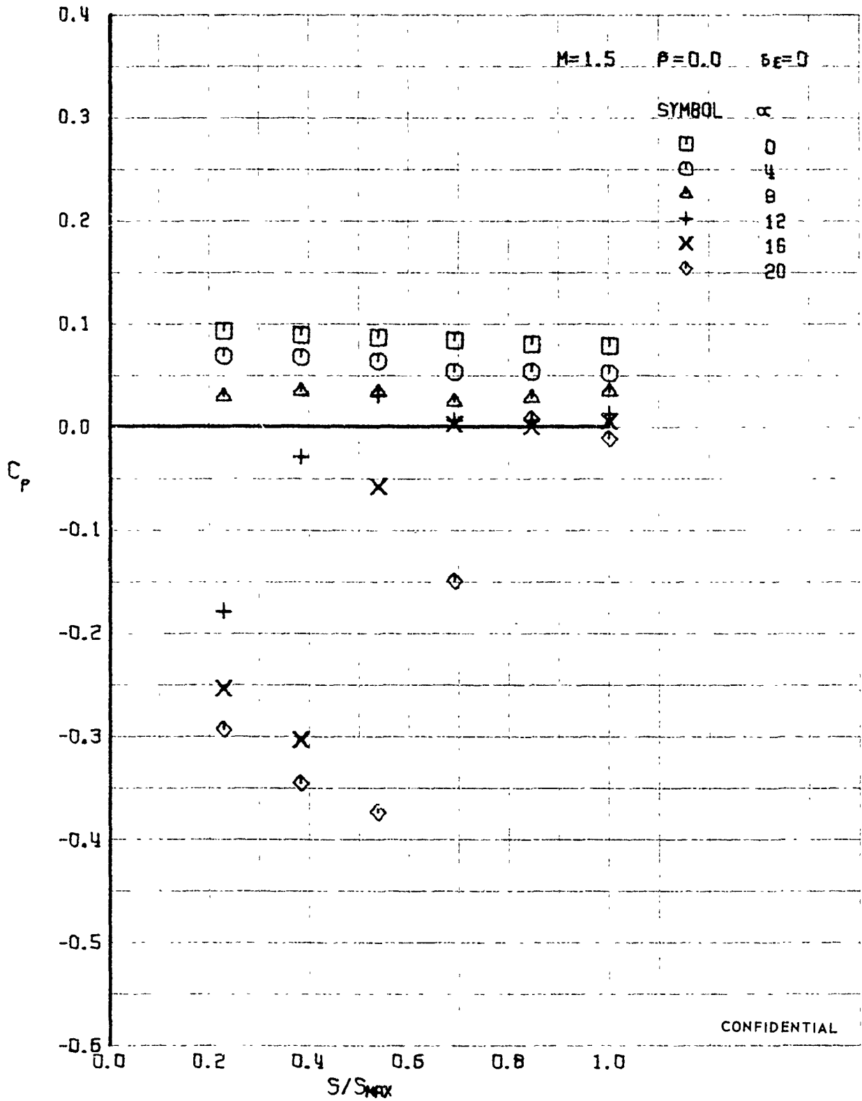
FIGURE 333 (U) UPPER SURFACE SPANWISE PRESSURES AT X/L = 0.30
