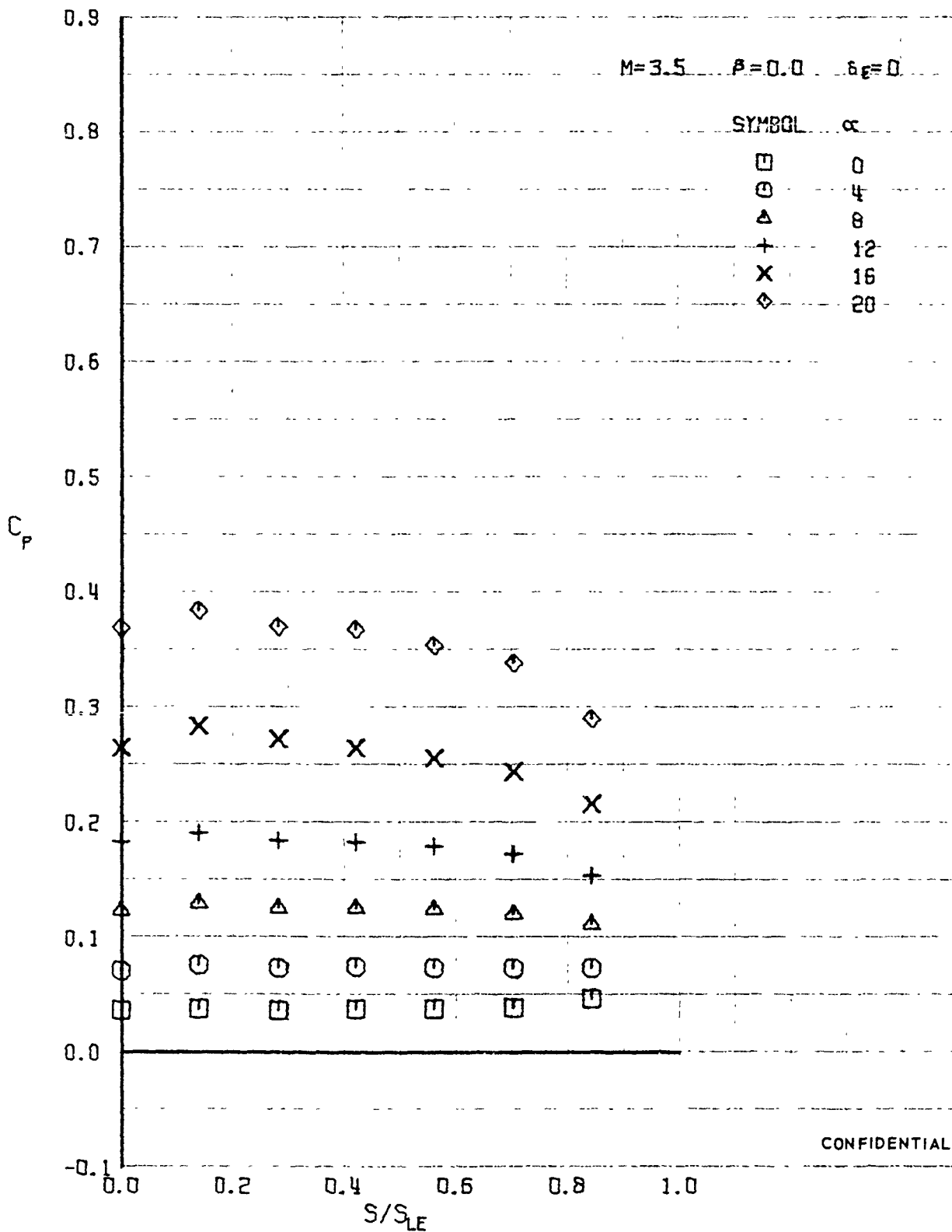
FIGURE 367 (U) LOWER SURFACE SPANWISE PRESSURES AT X/L = 0.50
