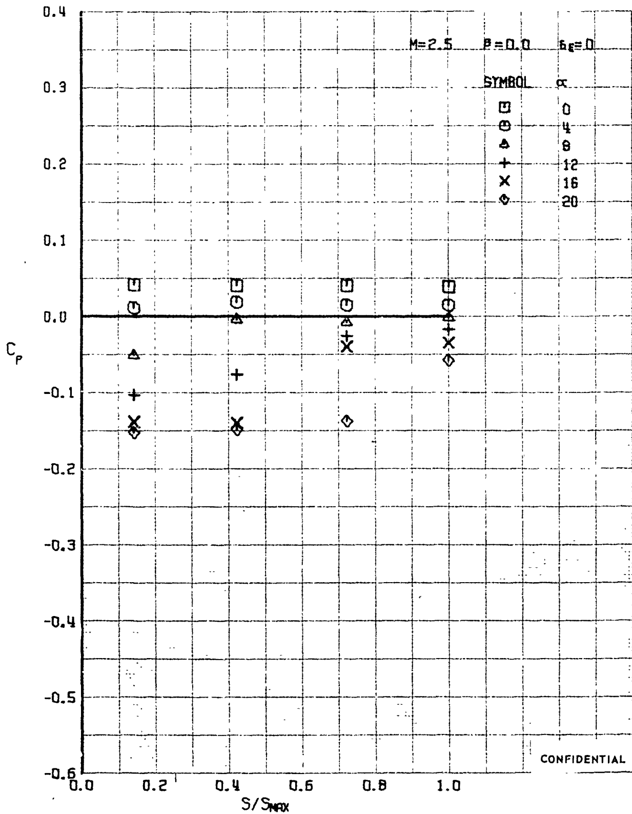
FIGURE 358 (U) UPPER SURFACE SPANWISE PRESSURES AT X/L = 0.15
