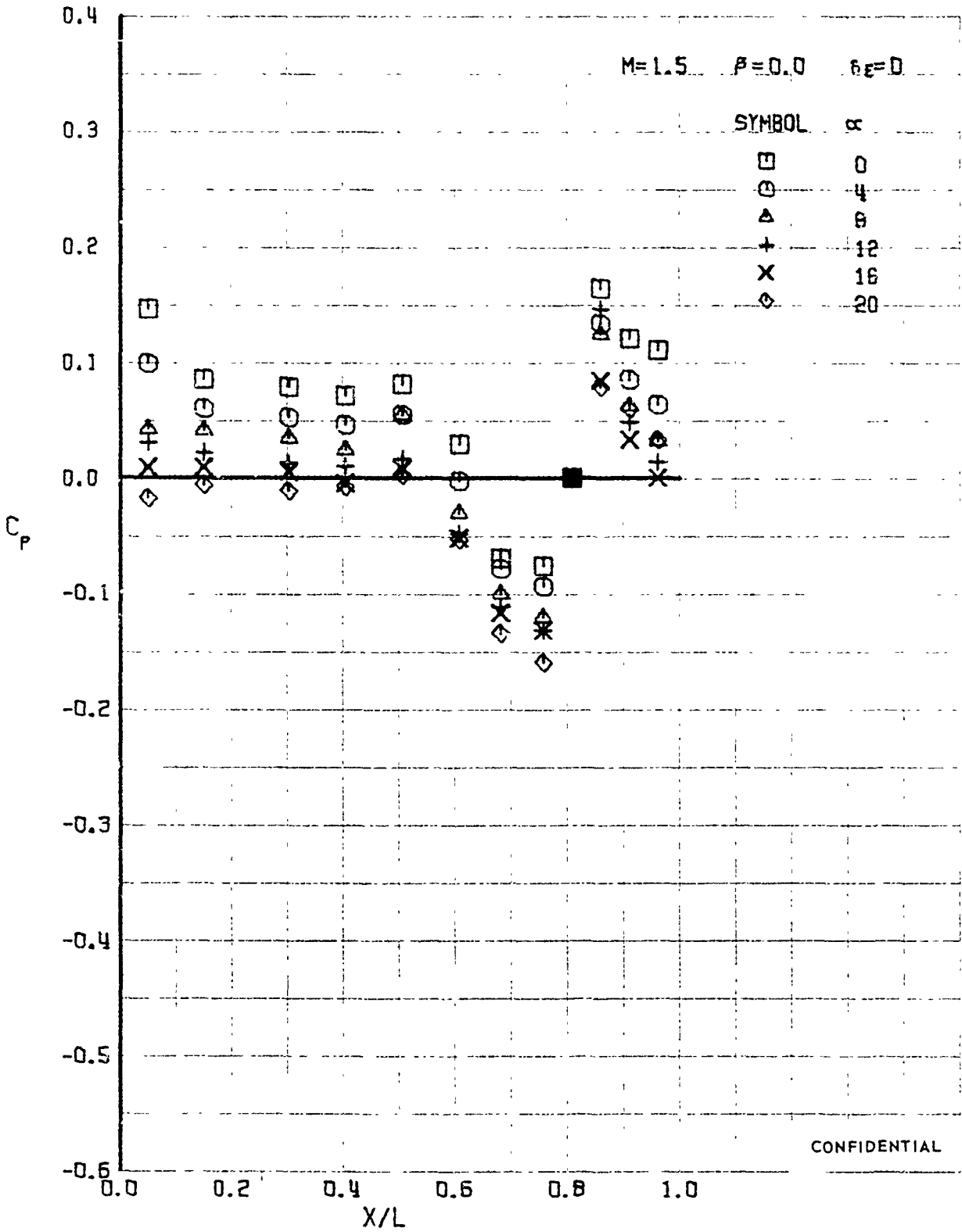
FIGURE 331 (U) UPPER SURFACE CENTERLINE PRESSURES
