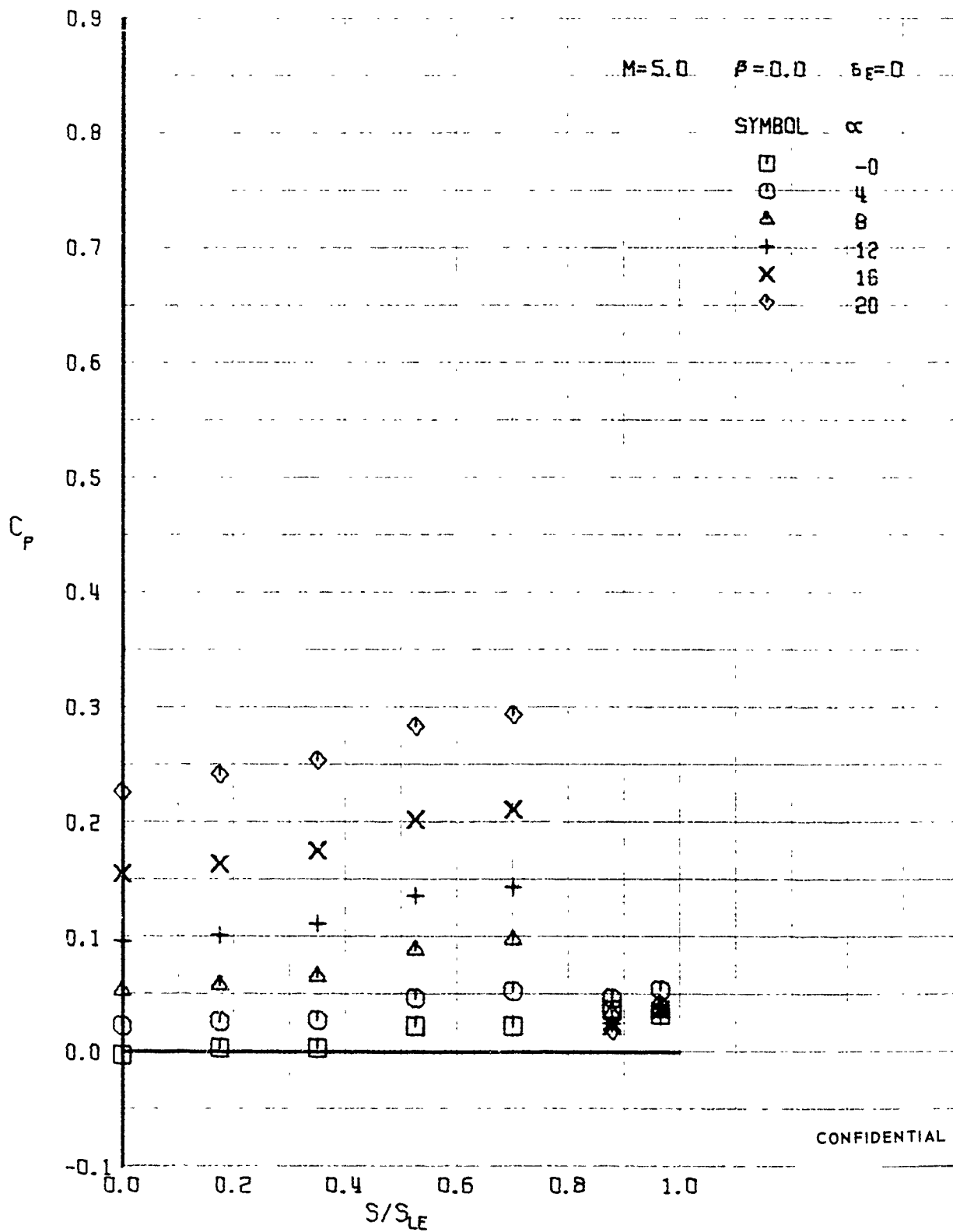
FIGURE 382 (U) LOWER SURFACE SPANWISE PRESSURES AT X/L = 0.96
