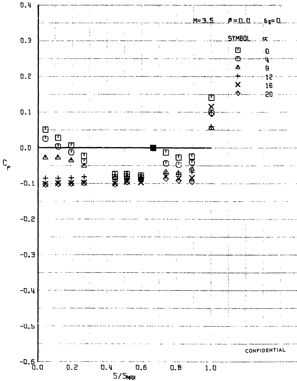
FIGURE 376 (U) UPPER SURFACE SPANWISE PRESSURES AT x/L = 0.96
