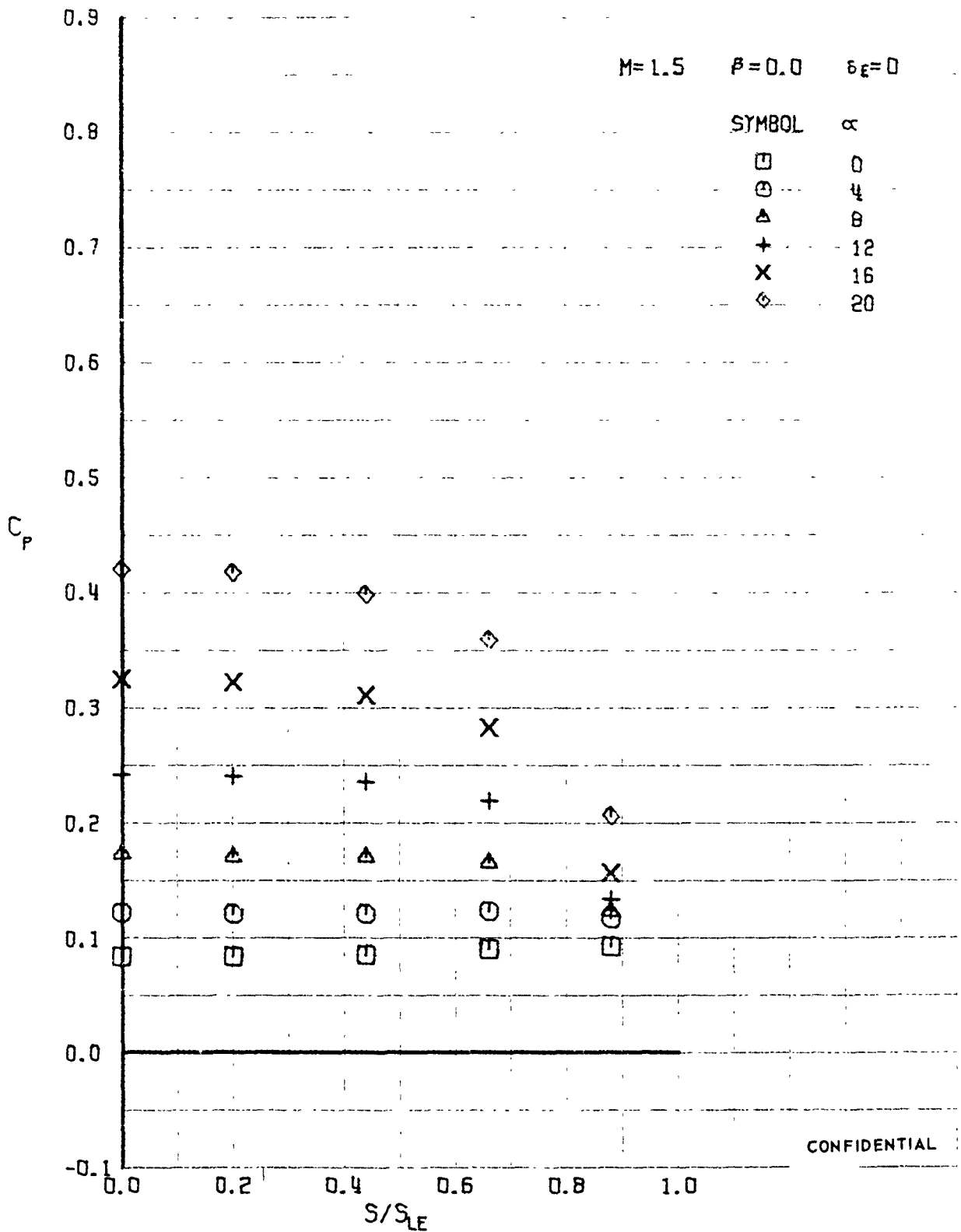
FIGURE 327 (U) LOWER SURFACE SPANWISE PRESSURES AT X/L = 0.30
