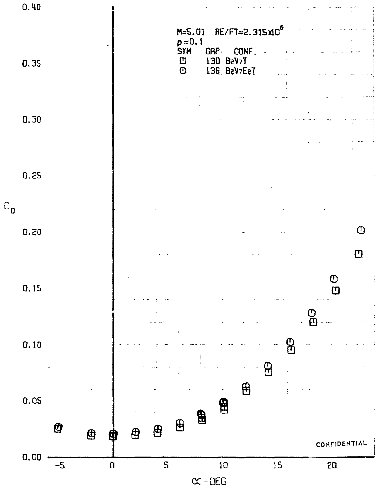
FIGURE 102 (U) CONFIGURATION BUILDUP - DRAG COEFFICIENT VARIATION WITH ANGLE OF ATTACK (M=5.01)
