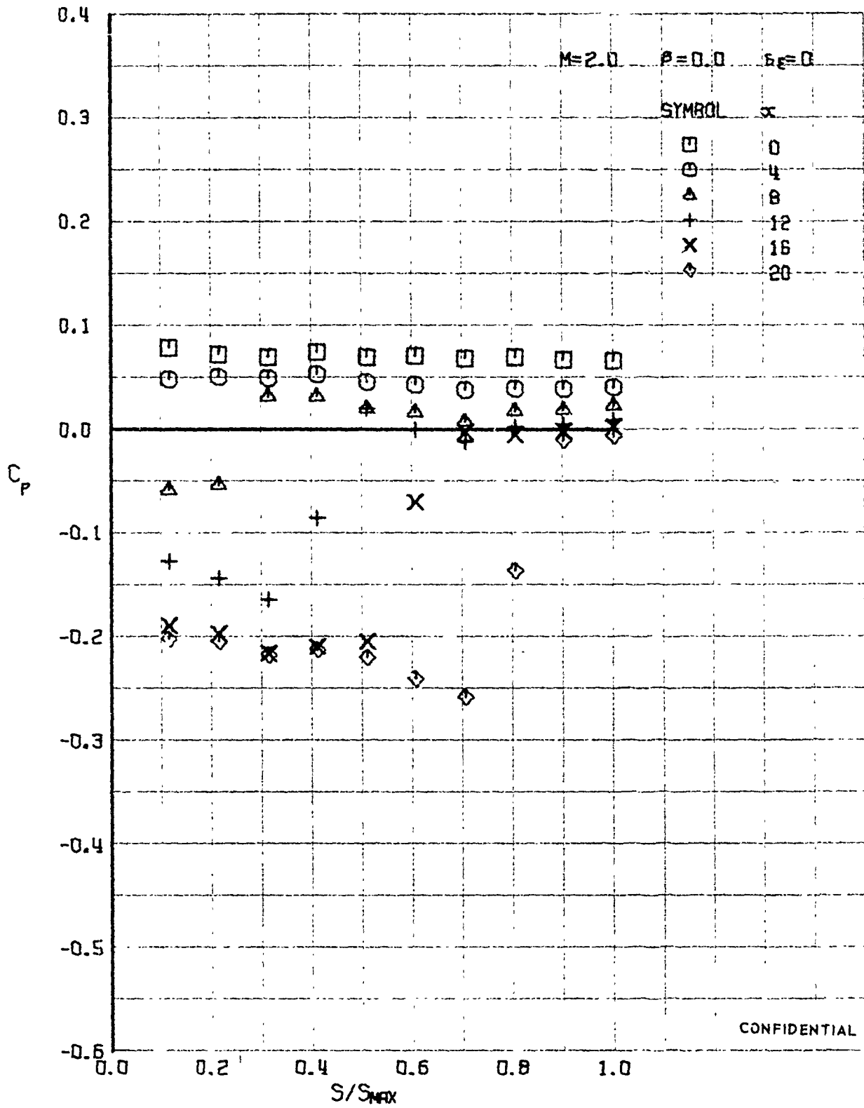
FIGURE 347 (U) UPPER SURFACE SPANWISE PRESSURES AT X/L = 0.50
