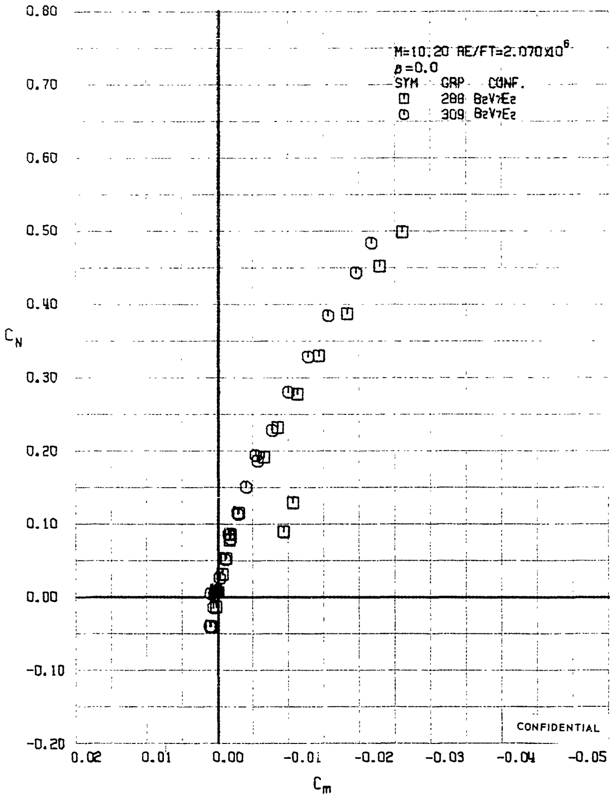
FIGURE 290 (U) REPEATABILITY - LONGITUDINAL STABILITY VARIATION (M=10.20)
