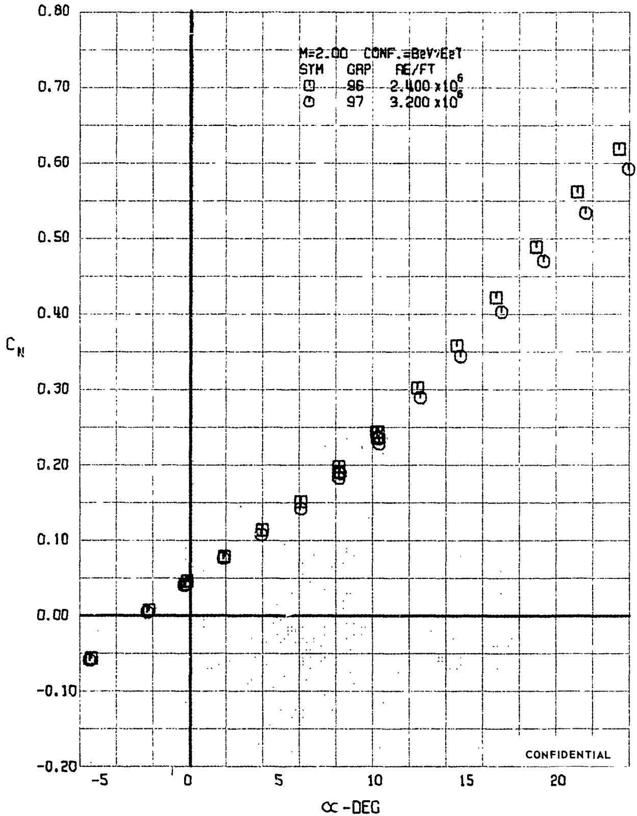
FIGURE 92 (U) REYNOLDS NUMBER EFFECTS - NORMAL FORCE COEFFICIENT VARIATION WITH ANGLE OF ATTACK (M=2.00)
