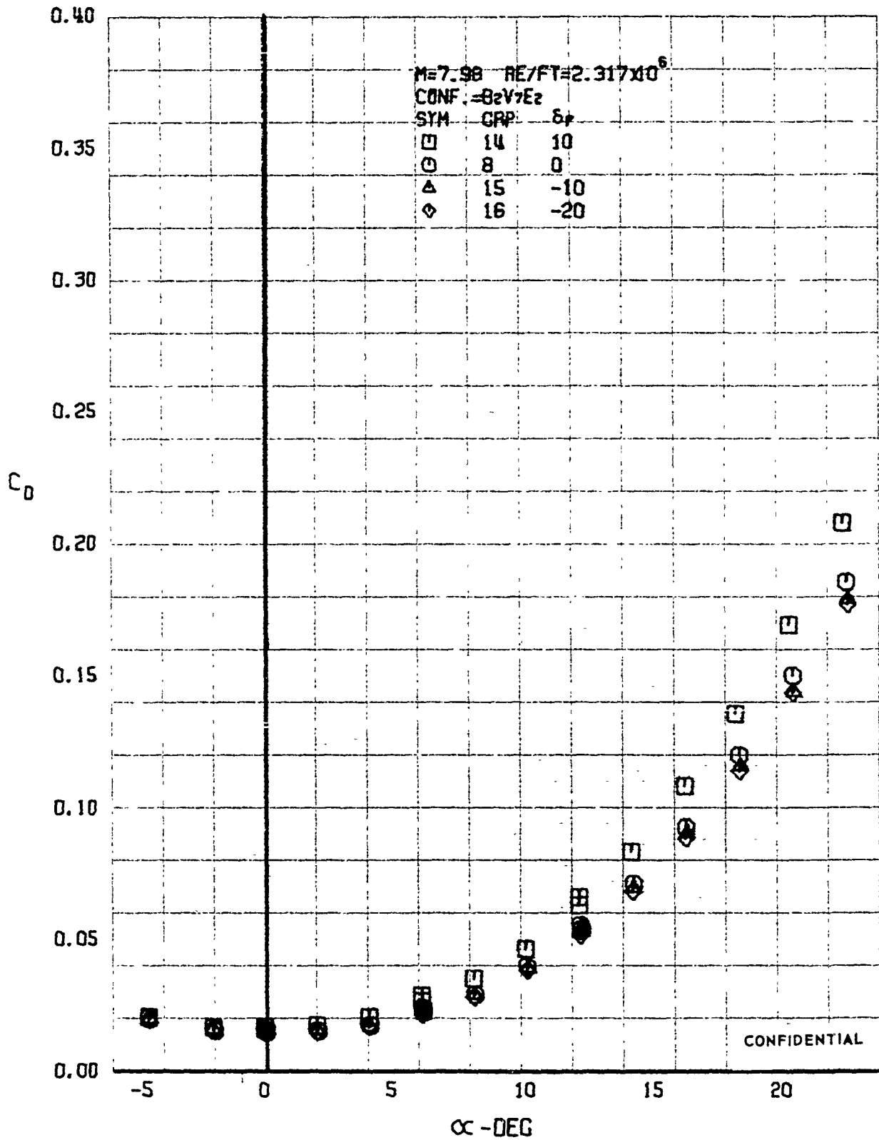
FIGURE 235 (U) ELEVON EFFECTS - DRAG COEFFICIENT VARIATION WITH ANGLE OF ATTACK (M=7.98)
