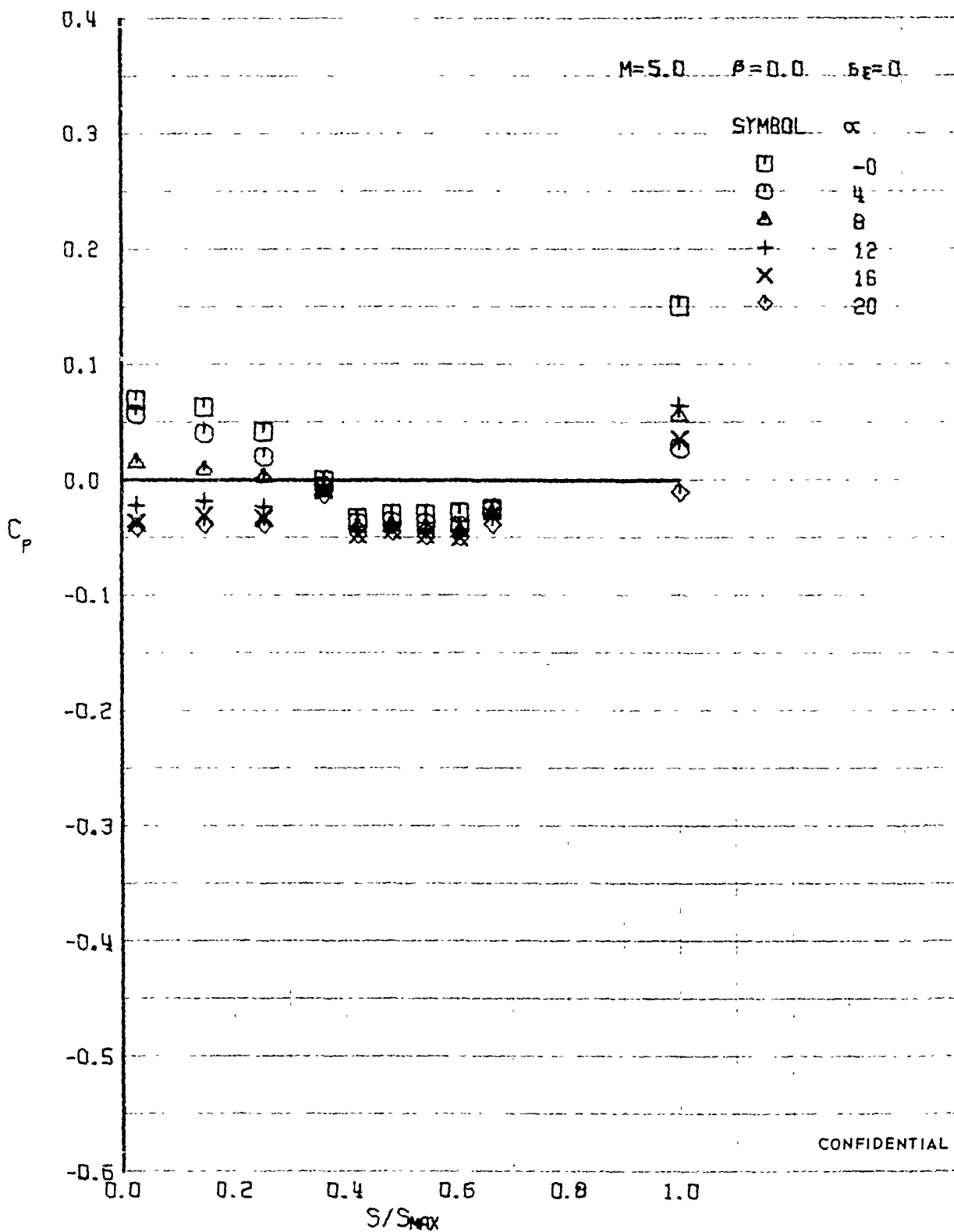
FIGURE 388 (U) UPPER SURFACE SPANWISE PRESSURES AT x/L = 0.86
