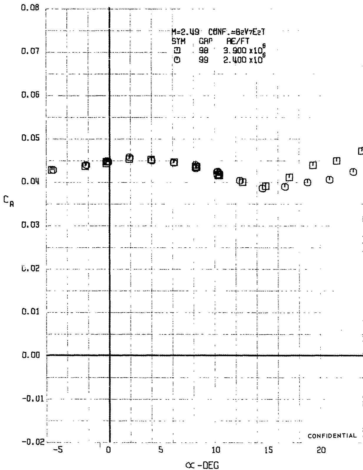
FIGURE 135 (U) REYNOLDS NUMBER EFFECTS - AXIAL FORCE COEFFICIENT VARIATION WITH ANGLE OF ATTACK (M=2.49)
