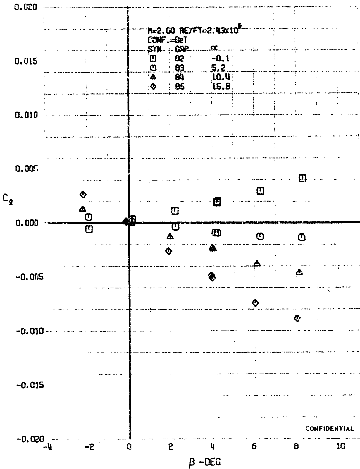
FIGURE 66 (U) BODY ALONE - ROLLING MOMENT COEFFICIENT VARIATION WITH ANGLE OF YAW (M=2.00)
