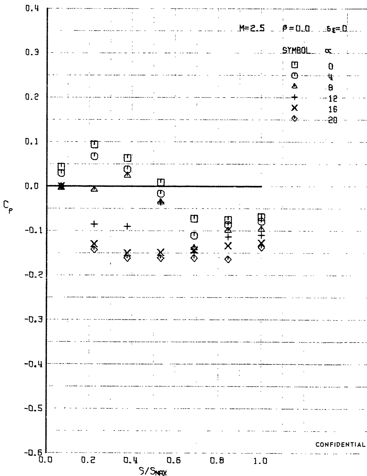
FIGURE 361 (U) UPPER SURFACE SPANWISE PRESSURES AT X/L = 0.76
