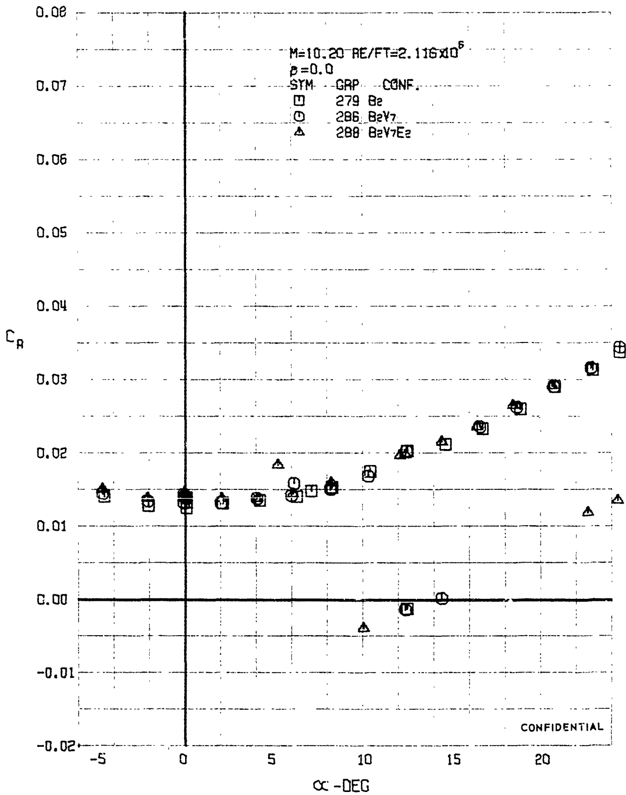
FIGURE 241 (U) CONFIGURATION BUILDUP - AXIAL FORCE COEFFICIENT VARIATION WITH ANGLE OF ATTACK (M=10.20)
