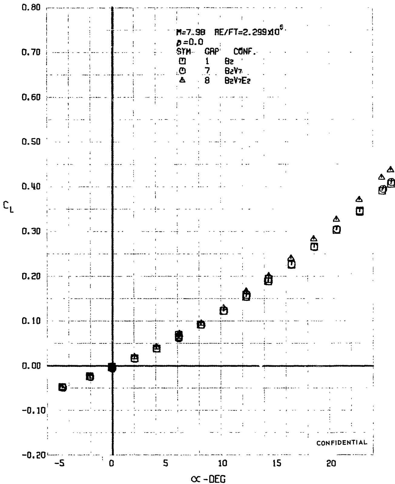
FIGURE 212 (U) CONFIGURATION BUILDUP - LIFT COEFFICIENT VARIATION WITH ANGLE OF ATTACK ( M=7.98 )
