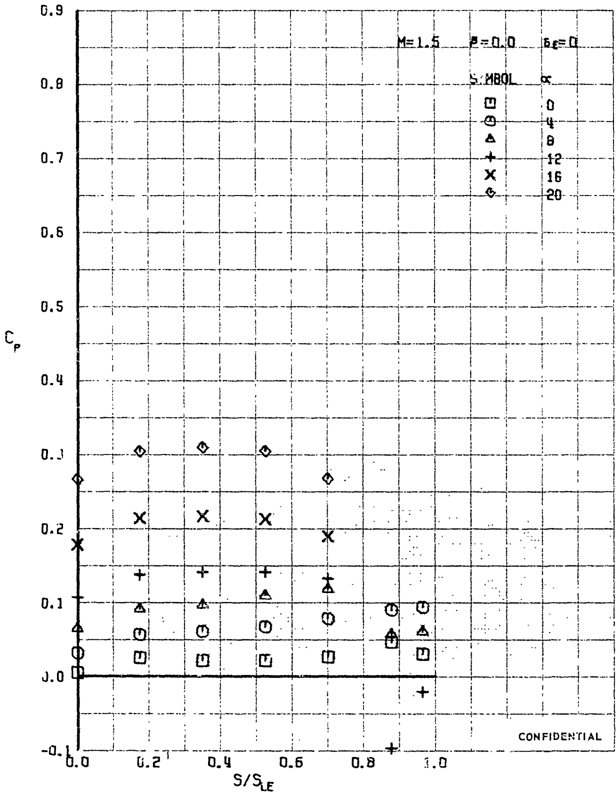
FIGURE 329 (U) LOWER SURFACE SPANWISE PRESSURES AT X/L = 0.76
