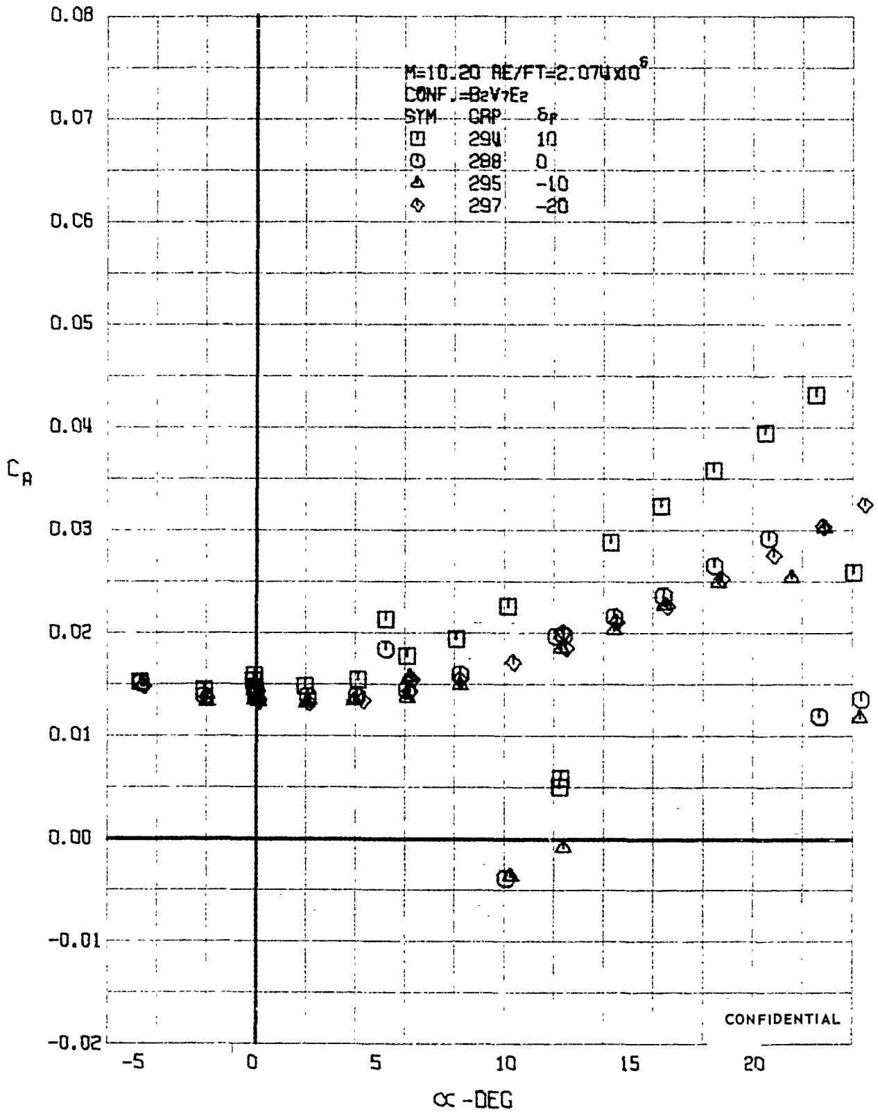
FIGURE 260 (U) ELEVON EFFECTS - AXIAL FORCE COEFFICIENT VARIATION WITH ANGLE OF ATTACK (M=10.20)
