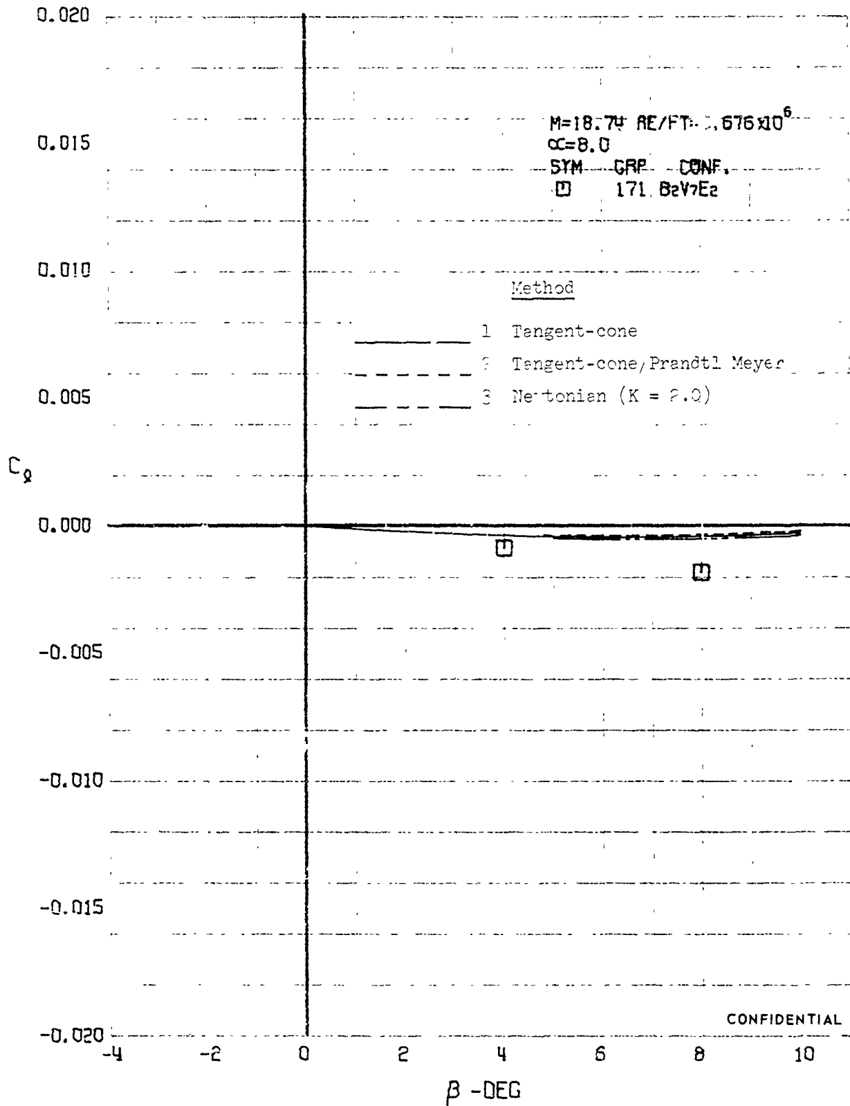
FIGURE 45. (U) COMPARISON OF ESTIMATED AND EXPERIMENTAL COEFFICIENTS ROLLING MOMENT COEFFICIENT VARIATION WITH ANGLE OF YAW ( M=18.74 )
