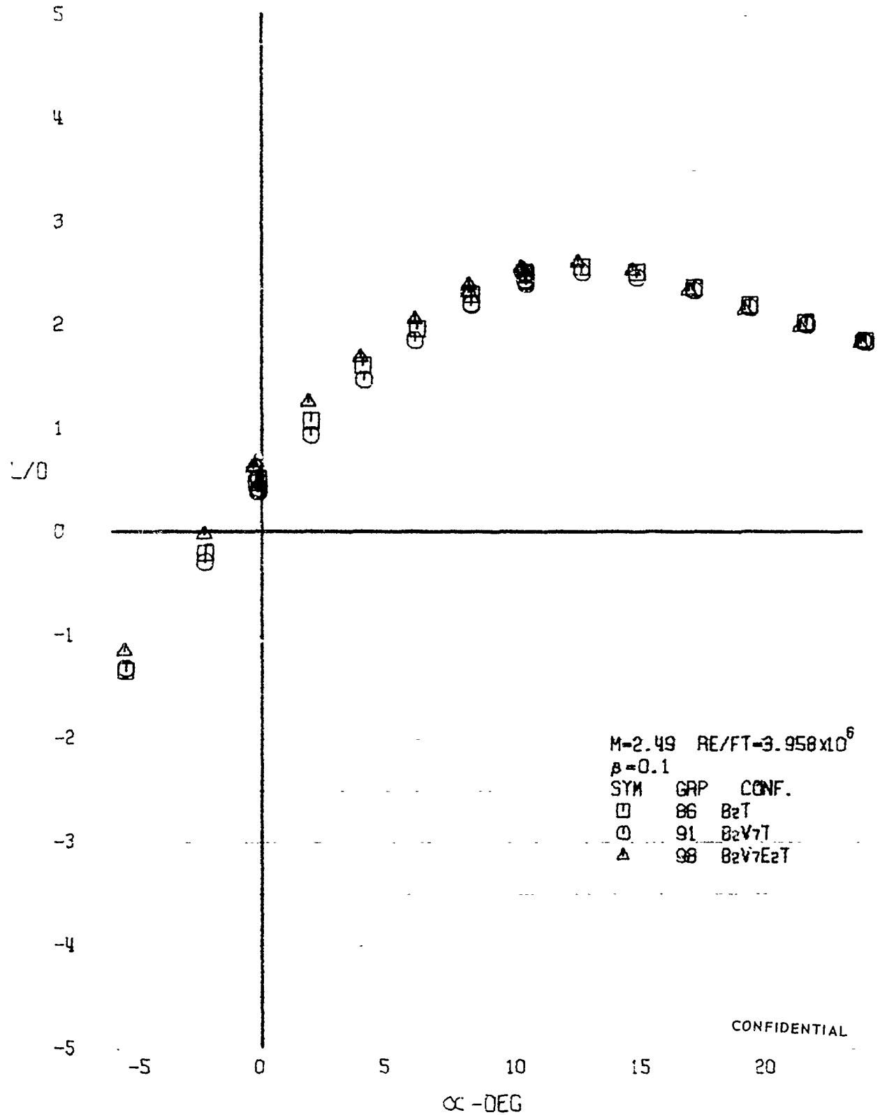
FIGURE 108 (U) CONFIGURATION BUJLOUP - LIFT-DRAG RATIO VARIATION WITH ANGLE OF ATTACK (M=2.49)
