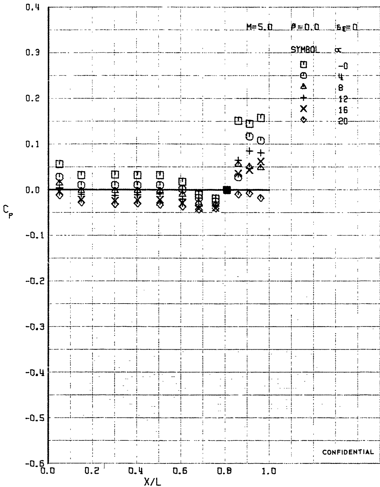
FIGURE 383 (U) UPPER SURFACE CENTERLINE PRESSURES
