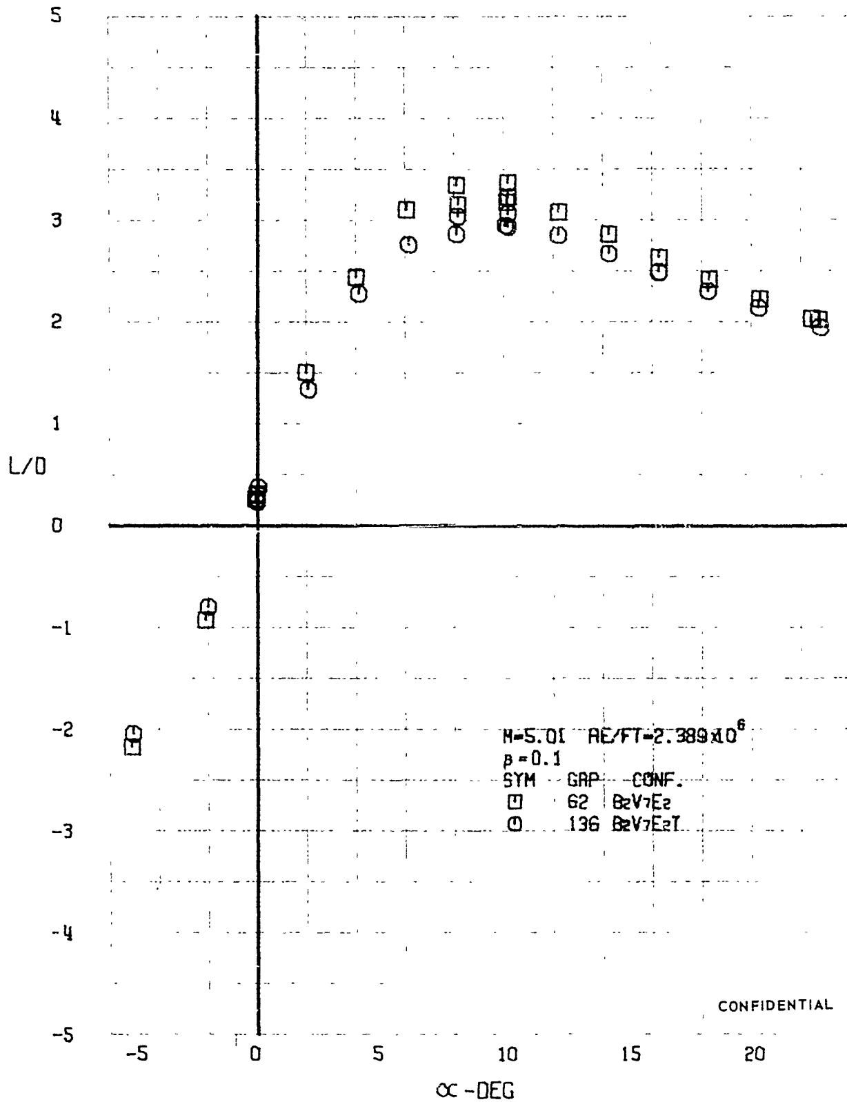
FIGURE 207 (U) FORCED TRANSITION EFFECTS - LIFT-DRAG RATIO VARIATION WITH ANGLE OF ATTACK ( N=5.01 )
