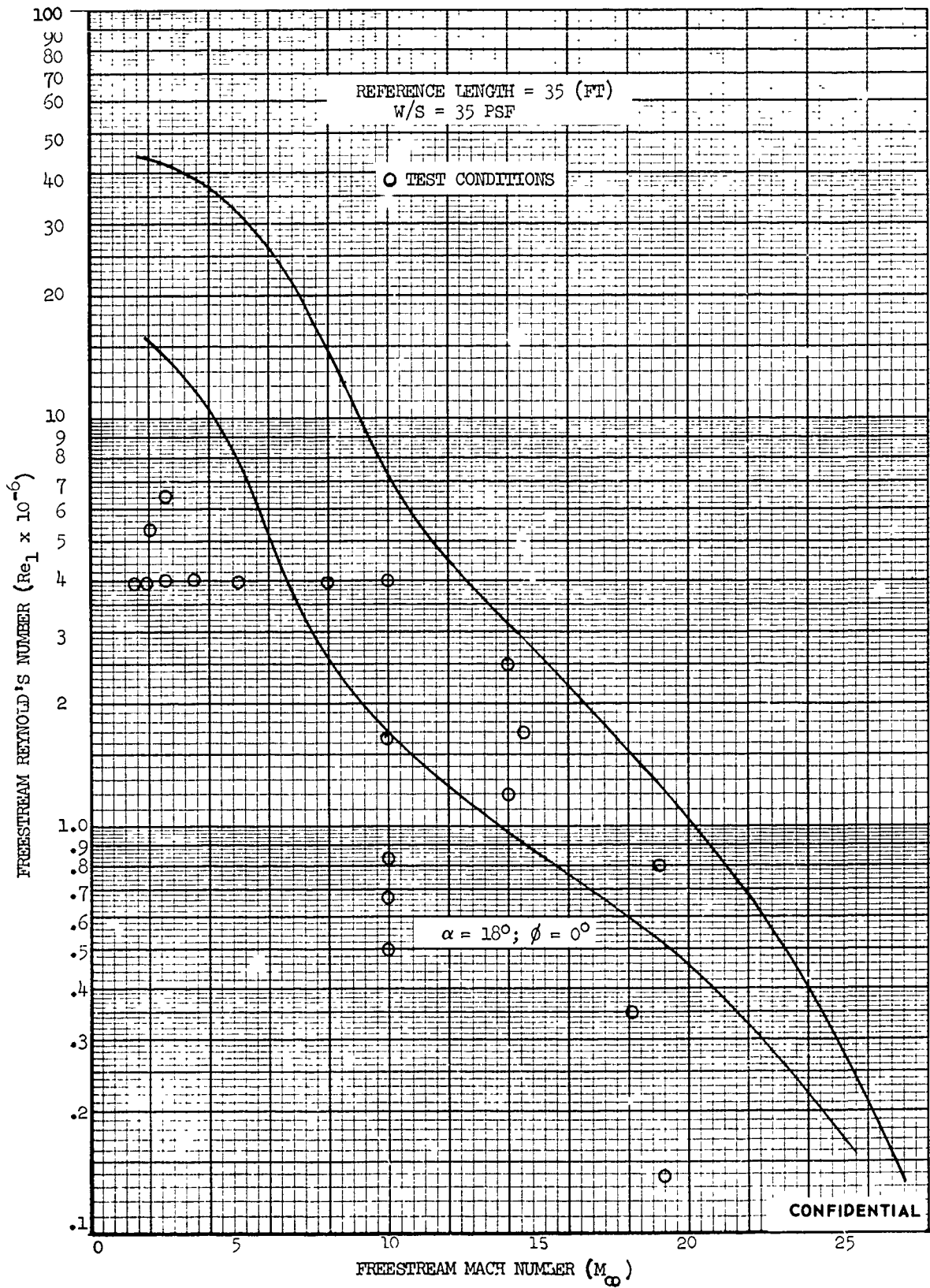
FIGURE 2 (U) AMR REFERENCE TRAJECTORIES
