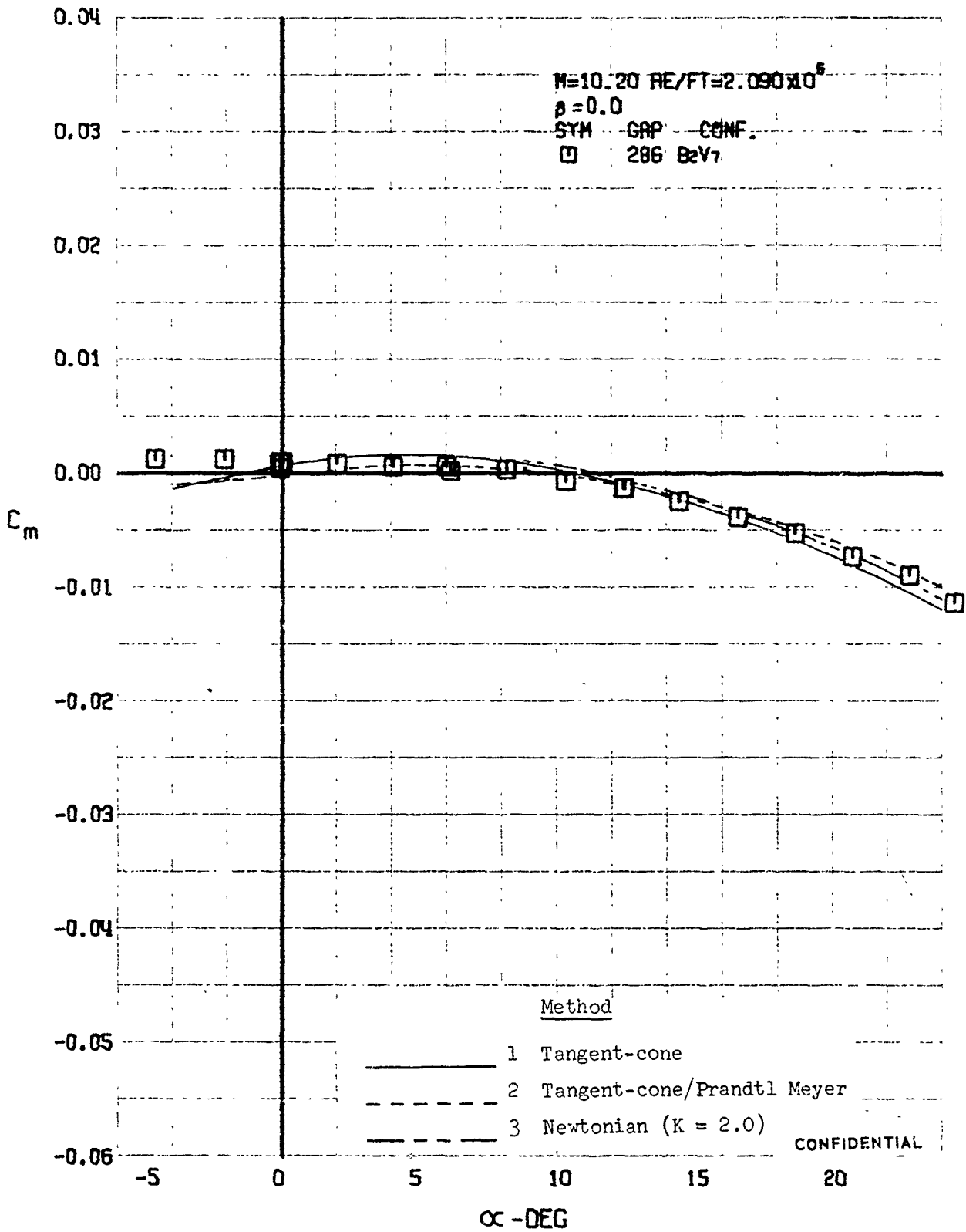
FIGURE 423 (U) COMPARISON OF ESTIMATED AND EXPERIMENTAL COEFFICIENTS - PITCHING MOMENT COEFFICIENT VARIATION WITH ANGLE OF ATTACK ( M=10.20 )
