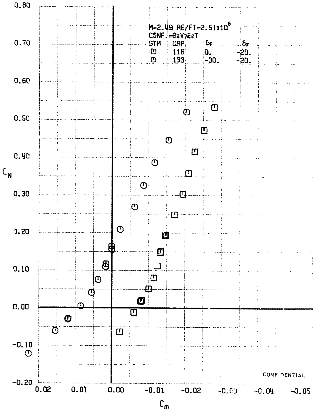
FIGURE 131 (U) FLAP EFFECTS - LONGITUDINAL STABILITY VARIATION (M=2.49)
