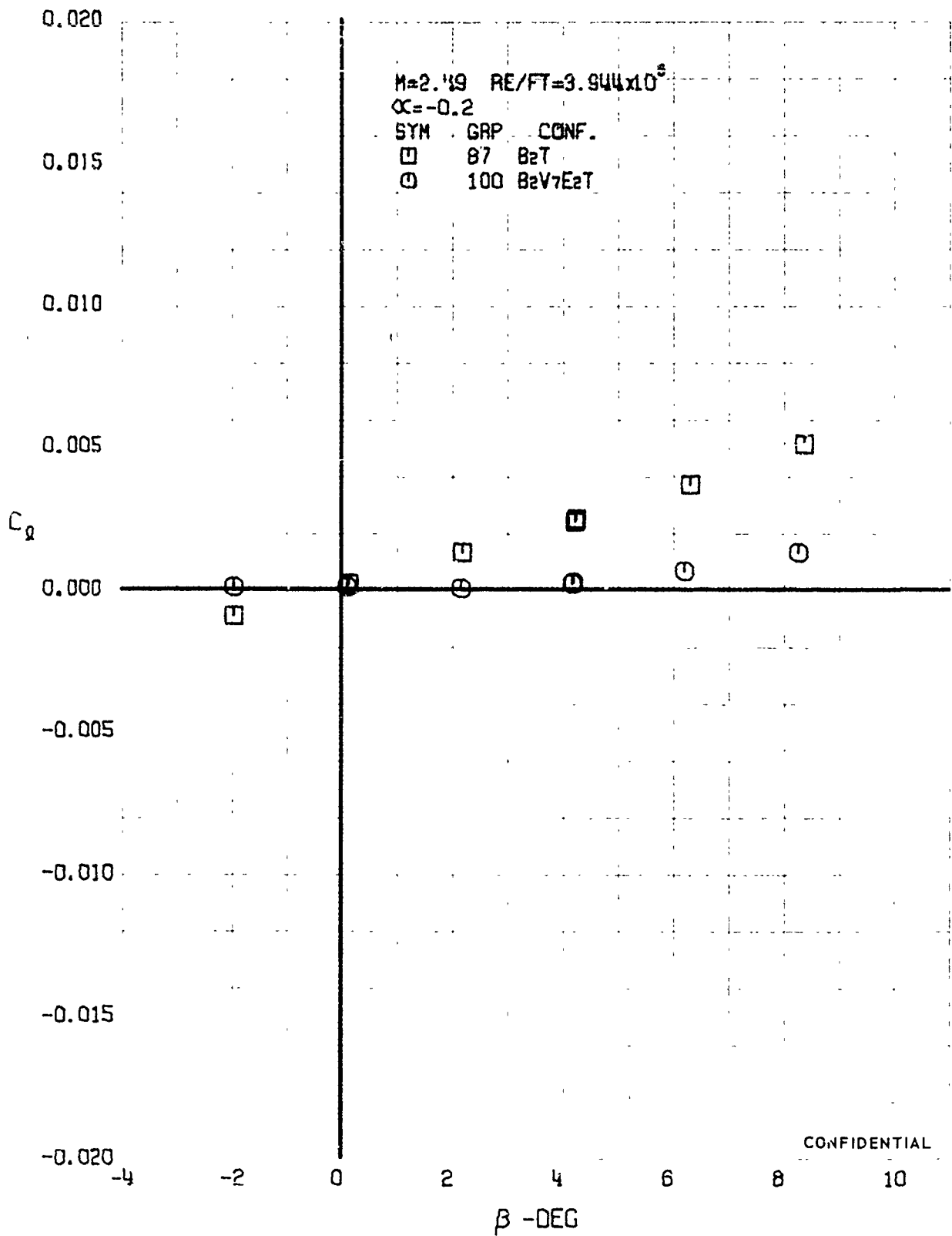
FIGURE 17 (U) CONFIGURATION BUILDUP - ROLLING MOMENT COEFFICIENT VARIATION WITH ANGLE OF YAW ( M=2.49 )
