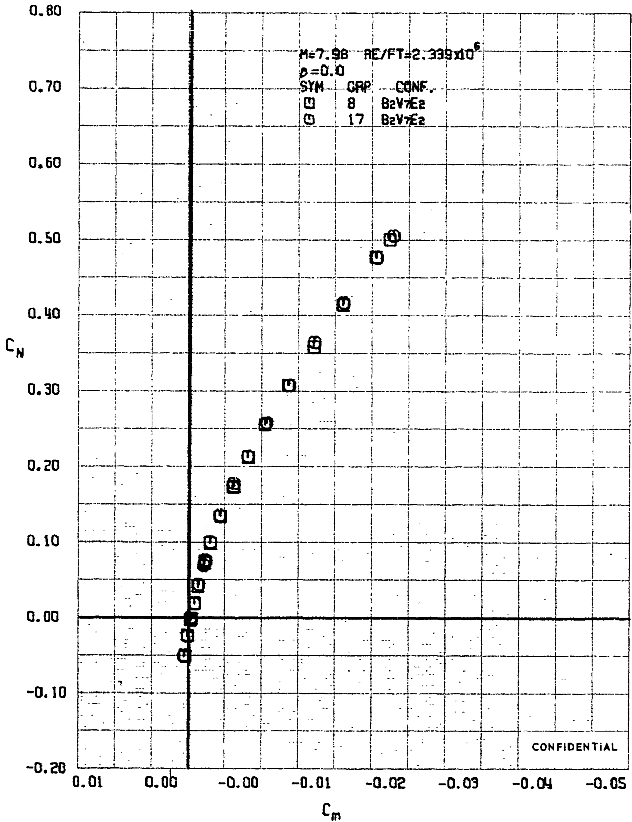
FIGURE 239 (U) REPEATABILITY - LONGITUDINAL STABILITY VARIATION ( M=7.98 )
