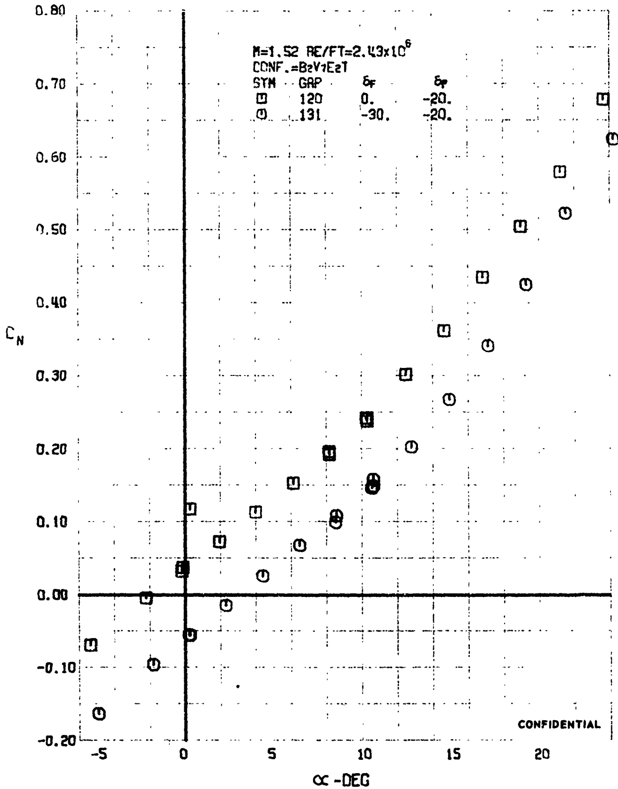
FIGURE 43 (U) FLAP EFFECTS - NORMAL FORCE COEFFICIENT VARIATION WITH ANGLE OF ATTACK ( M=1.52 )
