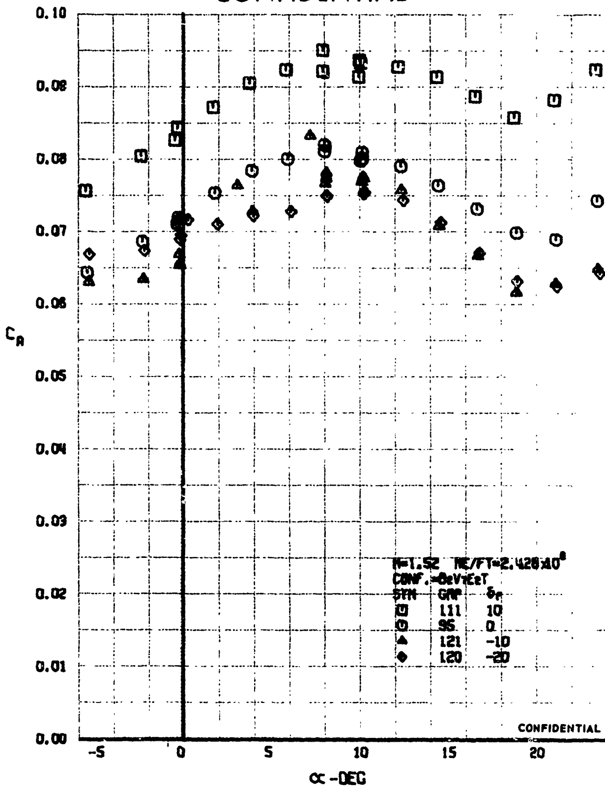
FIGURE 5. (U) ELEVON EFFECTS - AXIAL FORCE COEFFICIENT VARIATION WITH ANGLE OF ATTACK ( M=1.52 )
