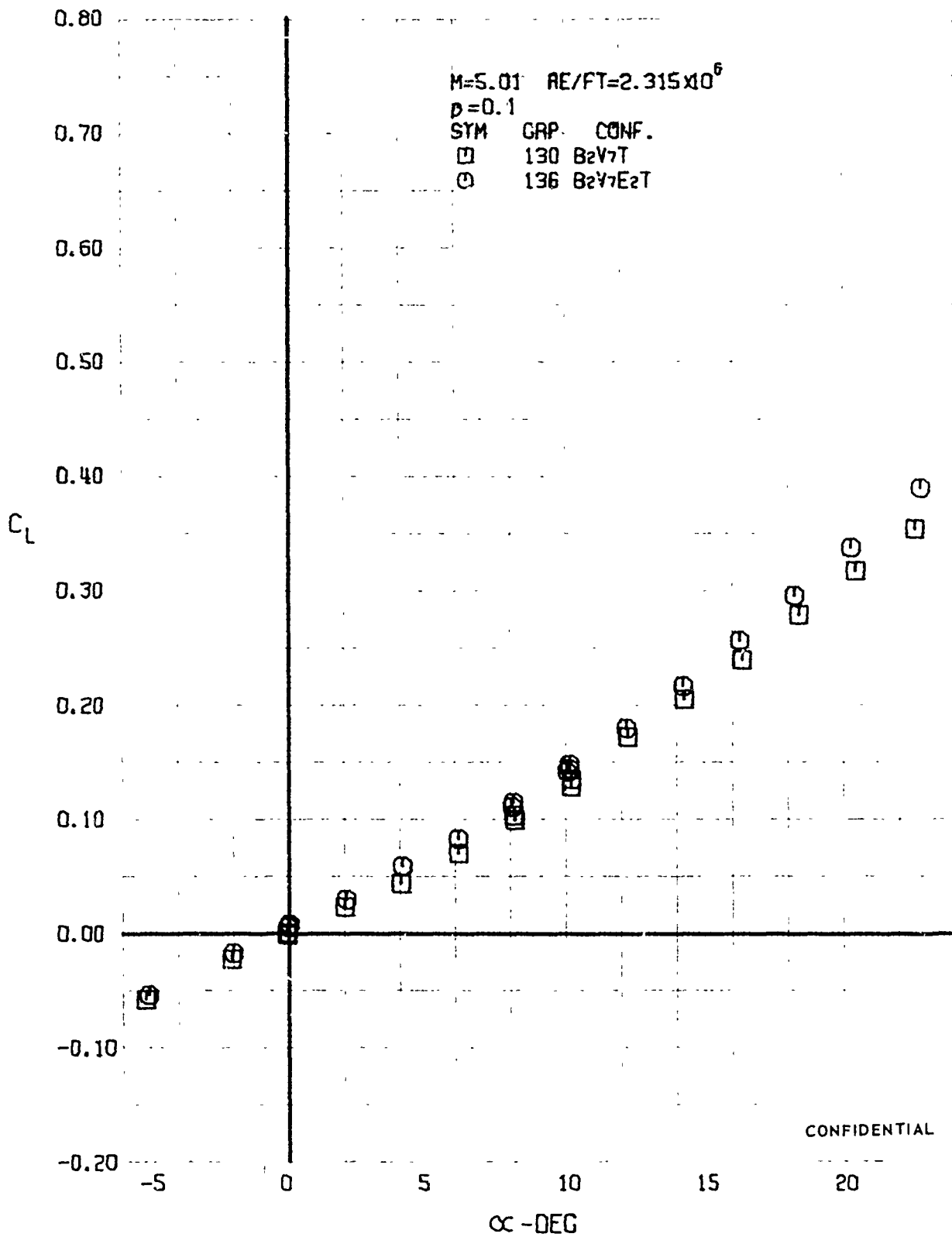
FIGURE 102 (U) CONFIGURATION BUILDUP - LIFT COEFFICIENT VARIATION WITH ANGLE OF ATTACK (M=5.01)
