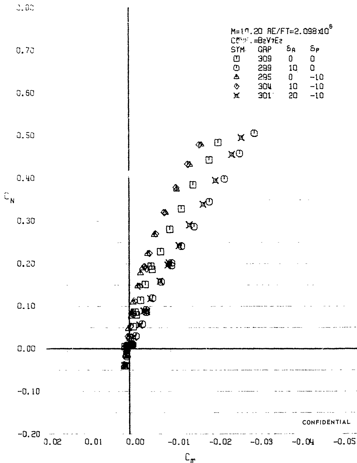
FIGURE 274 (U) AILERON EFFECTS - LONGITUDINAL STABILITY VARIATION ( M=10.20 )
