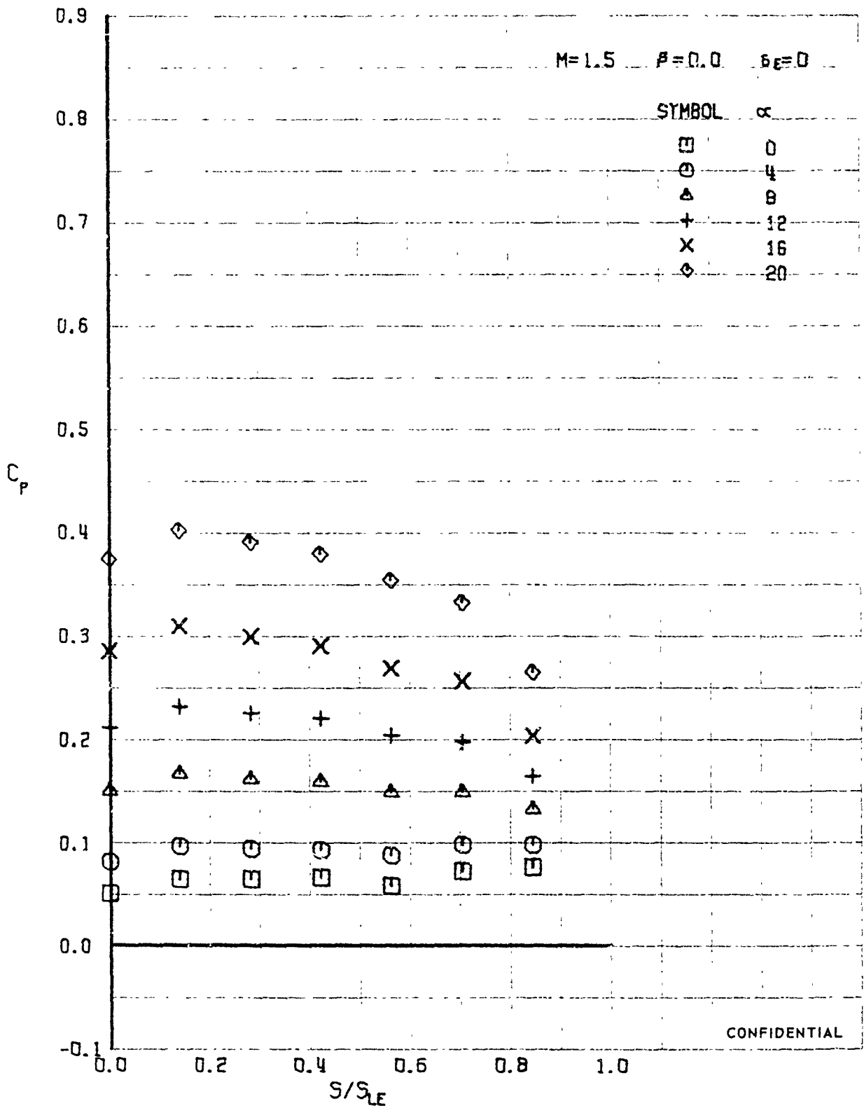
FIGURE 328 (U) LOWER SURFACE SPANWISE PRESSURES AT X/L = 0.50
