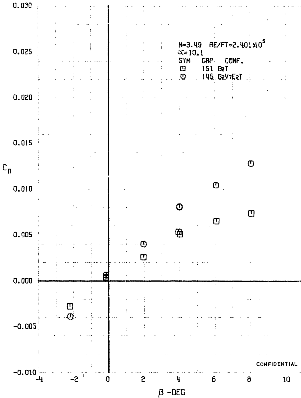
FIGURE 163 (U) CONFIGURATION BUILDUP - YAWING MOMENT COEFFICIENT VARIATION WITH ANGLE OF YAW ( M=3.49 )
