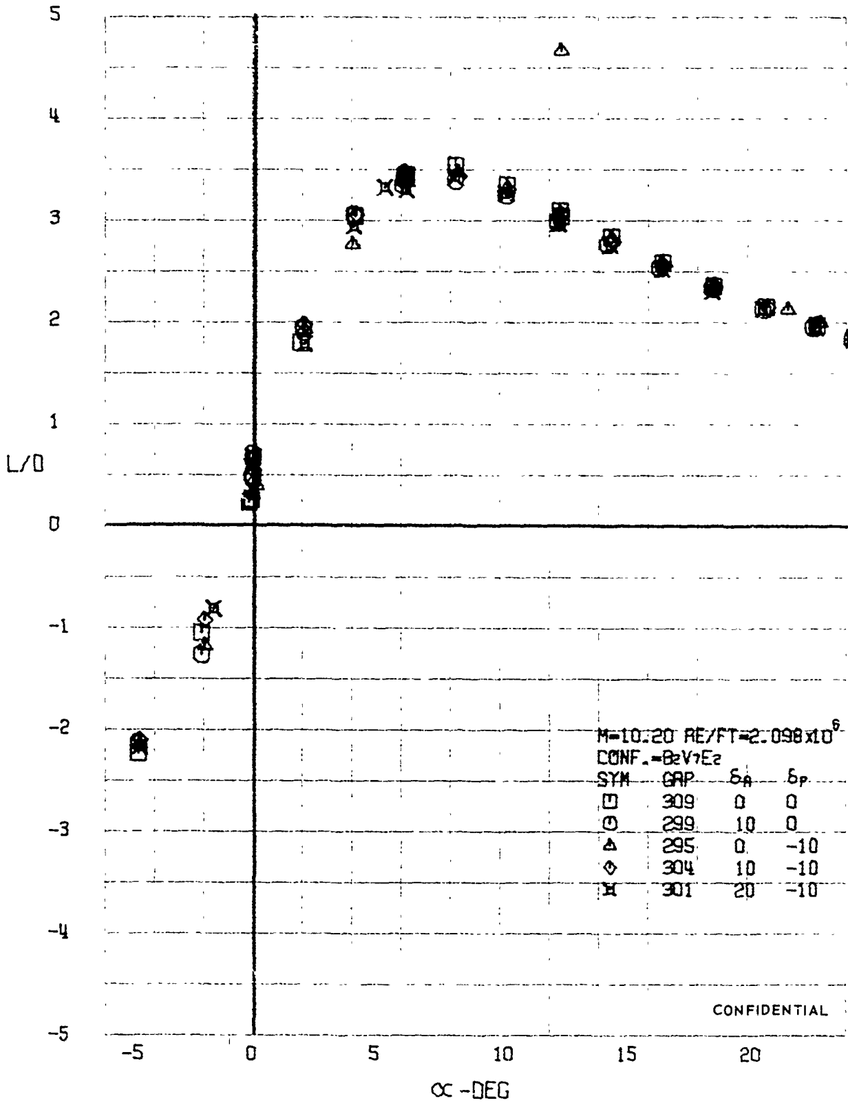
FIGURE 277 (U) AILERON EFFECTS - LIFT-DRAG RATIO VARIATION WITH ANGLE OF ATTACK ( M=10.20 )
