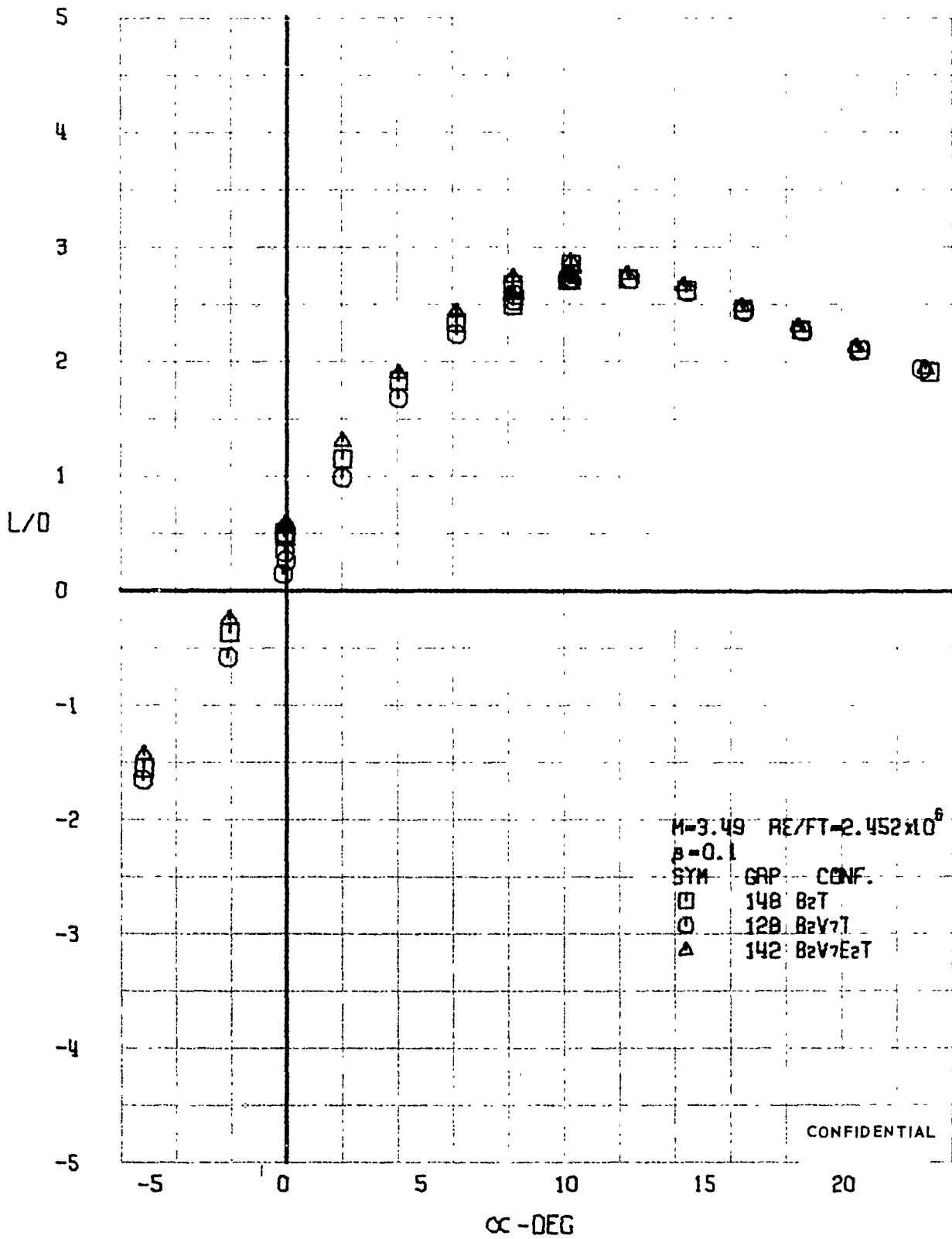
FIGURE 156 (U) CONFIGURATION BUILDUP - LIFT-DRAGE RATIO VARIATION WITH ANGLE OF ATTACK (M=3.49)
