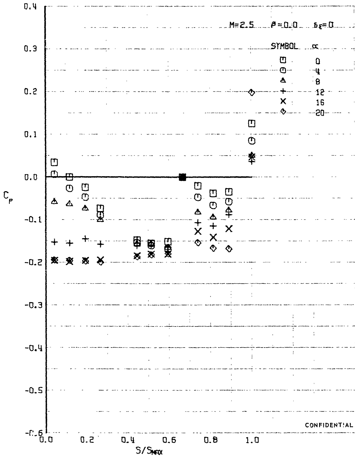
FIGURE 363 (U) UPPER SURFACE SPANWISE PRESSURES AT X/L = 0.96
