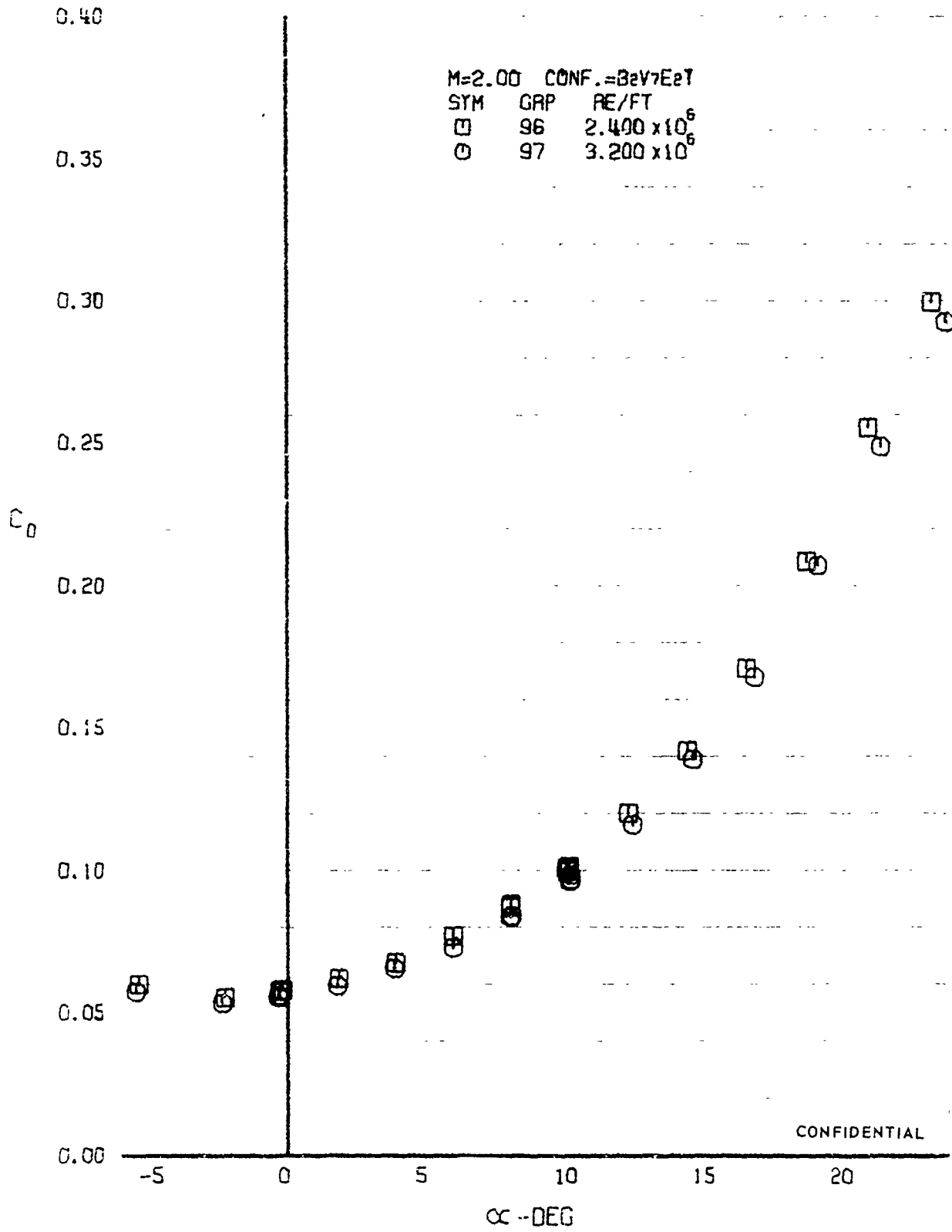
FIGURE 16 (U) REYNOLDS NUMBER EFFECTS - DRAG COEFFICIENT VARIATION WITH ANGLE OF ATTACK (M=2.00)
