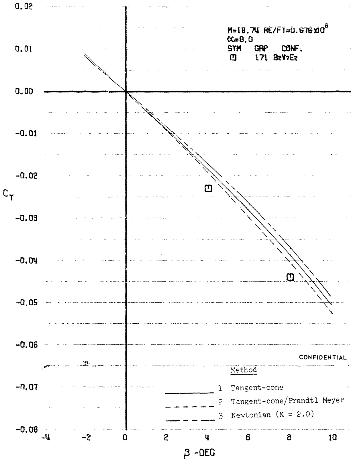
FIGURE 435 (U) COMPARISON OF ESTIMATED AND EXPERIMENTAL COEFFICIENTS - SIDE FORCE COEFFICIENT VARIATION WITH ANGLE OF YAW ( M=18.74 )
