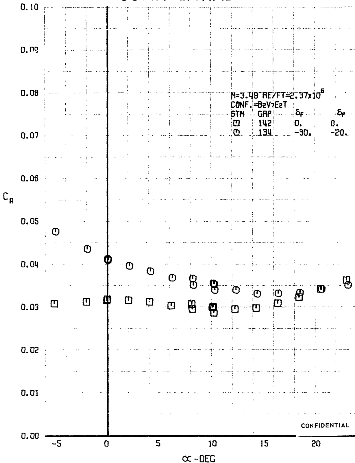
FIGURE 16 (U) COMBINED ELEVON AND FLAP EFFECTS - AXIAL FORCE COEFFICIENT VARIATION WITH ANGLE OF ATTACK (M=3.49)
