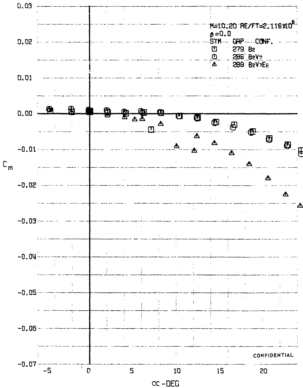
FIGURE 243 (U) CONFIGURATION BUILDUP - PITCHING MOMENT COEFFICIENT VARIATION WITH ANGLE OF ATTACK (M=10.20)
