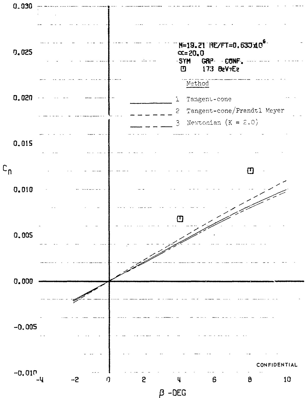
FIGURE 448 (U) COMPARISON OF ESTIMATED AND EXPERIMENTAL COEFFICIENTS - ROLLING MOMENT COEFFICIENT VARIATION WITH ANGLE OF YAW ( M=19.21 )
