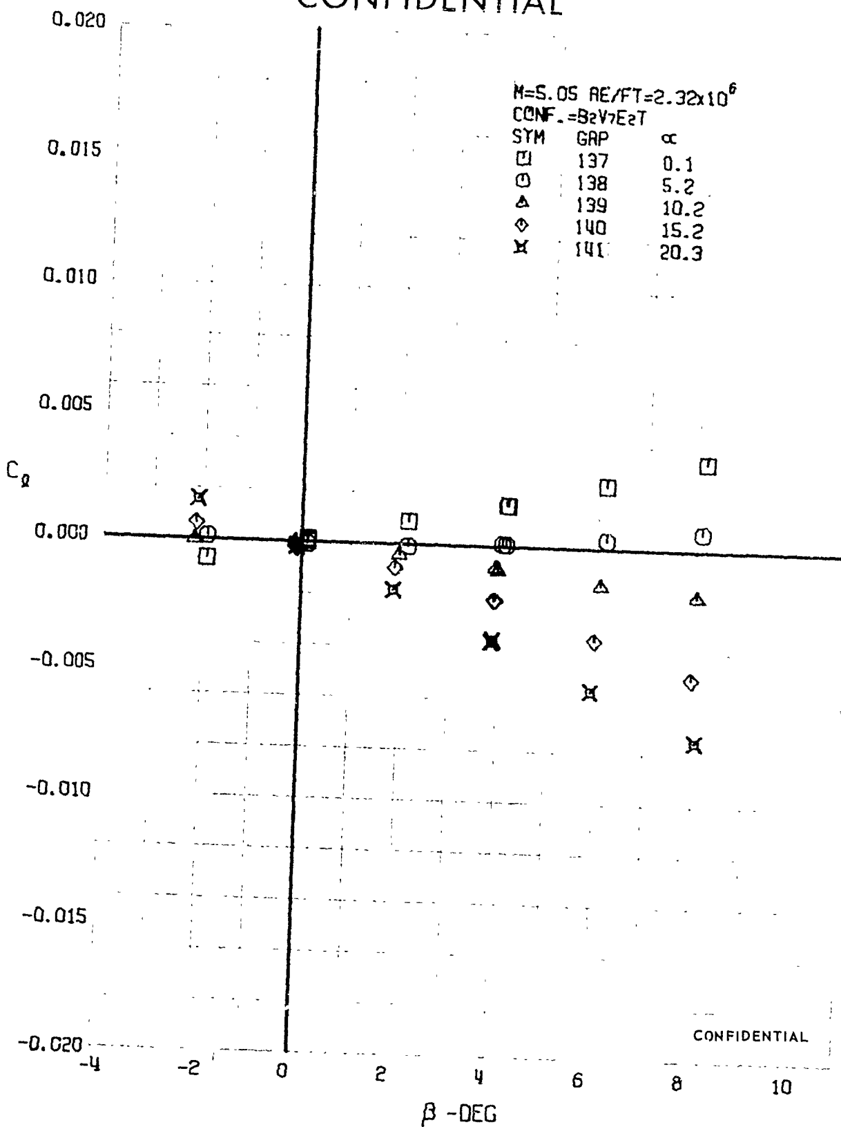
FIGURE 196 (U) COMPLETE CONFIGURATION - ROLLING MOMENT COEFFICIENT VARIATION WITH ANGLE OF YAW (M=5.05)
