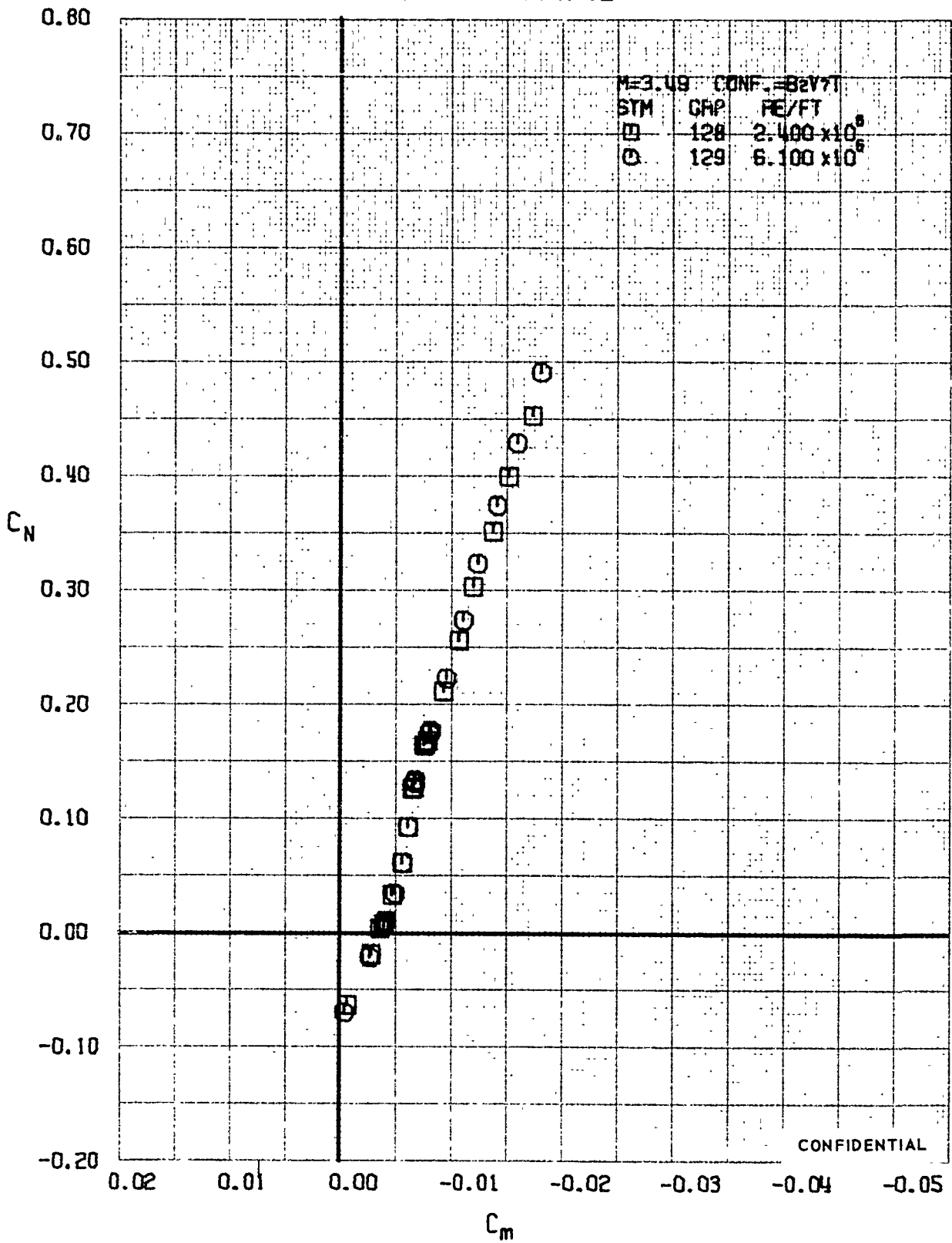
FIGURE 179 (U) REYNOLDS NUMBER EFFECTS - LONGITUDINAL STABILITY VARIATION (N=3.49)
