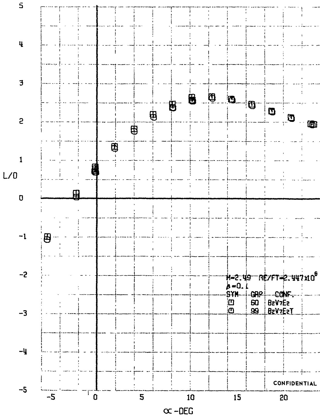
FIGURE 145 (U) FORCED TRANSITION EFFECTS - LIFT-DRAG RATIO VARIATION WITH ANGLE OF ATTACK (M=2.49)
