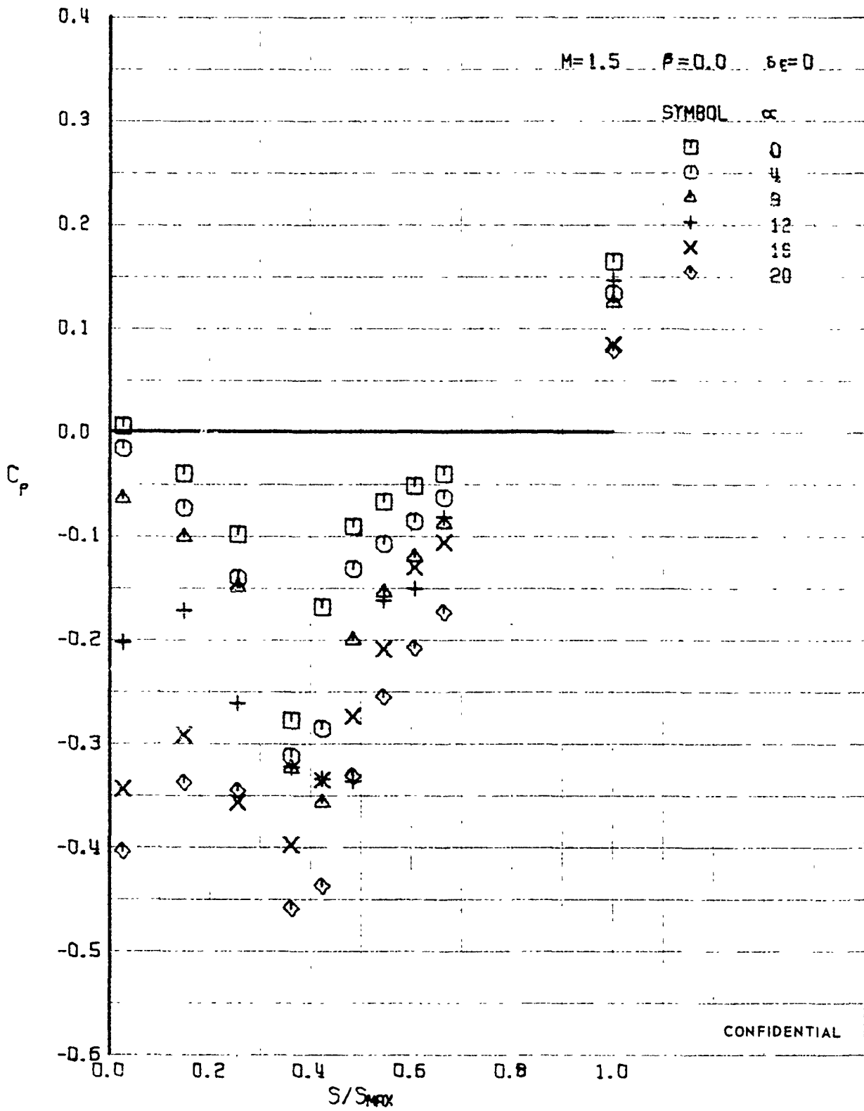
FIGURE 336 (U) UPPER SURFACE SPANWISE PRESSURES AT X/L = 0.86
