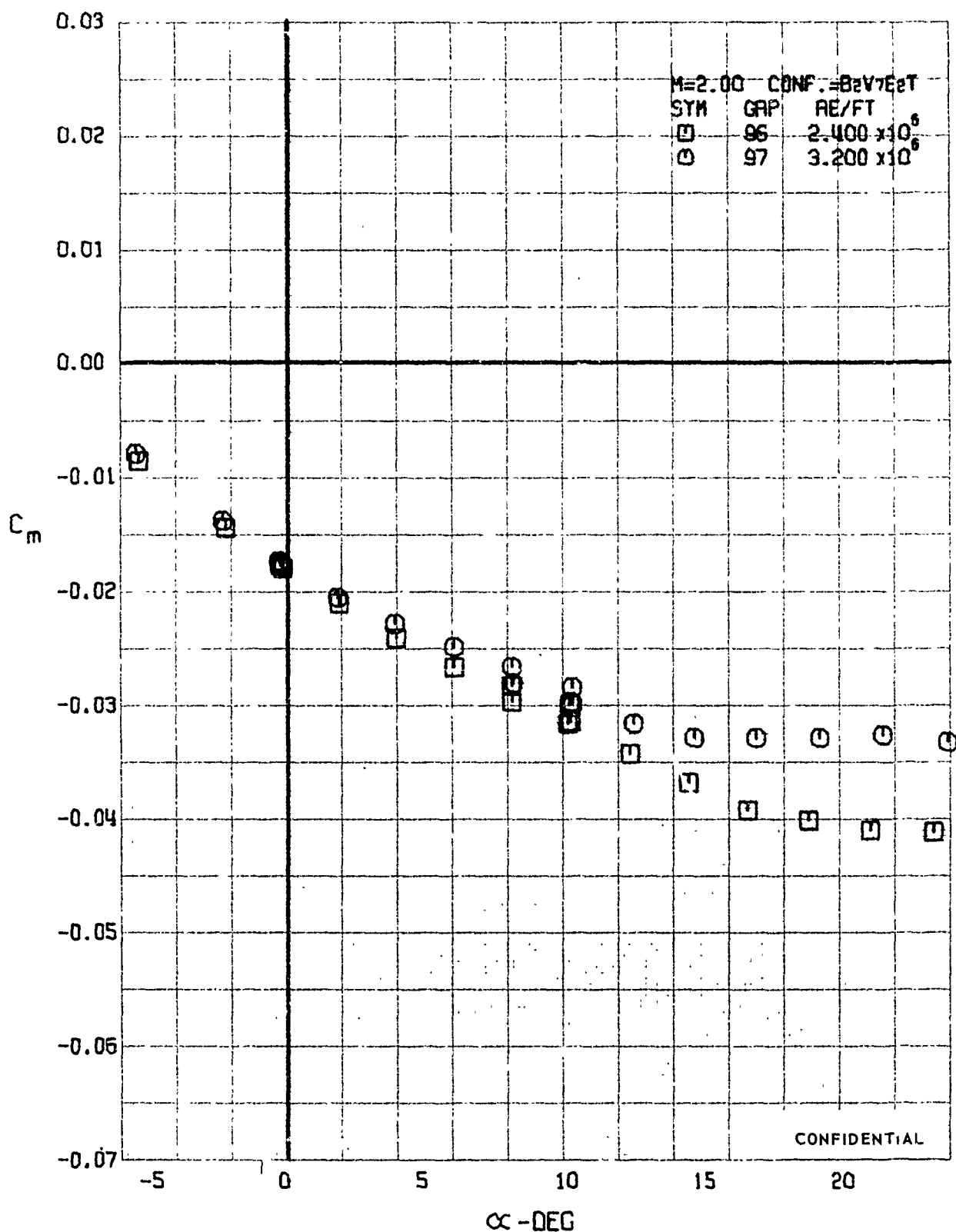
FIGURE 93 (U) REYNOLDS NUMBER EFFECTS - FITTING MOMENT COEFFICIENT VARIATION WITH ANGLE OF ATTACK (M=2.00)
