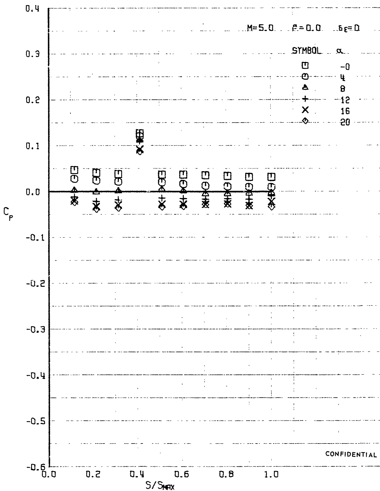
FIGURE 386 (U) UPPER SURFACE SPANWISE PRESSURES AT X/L = 0.50
