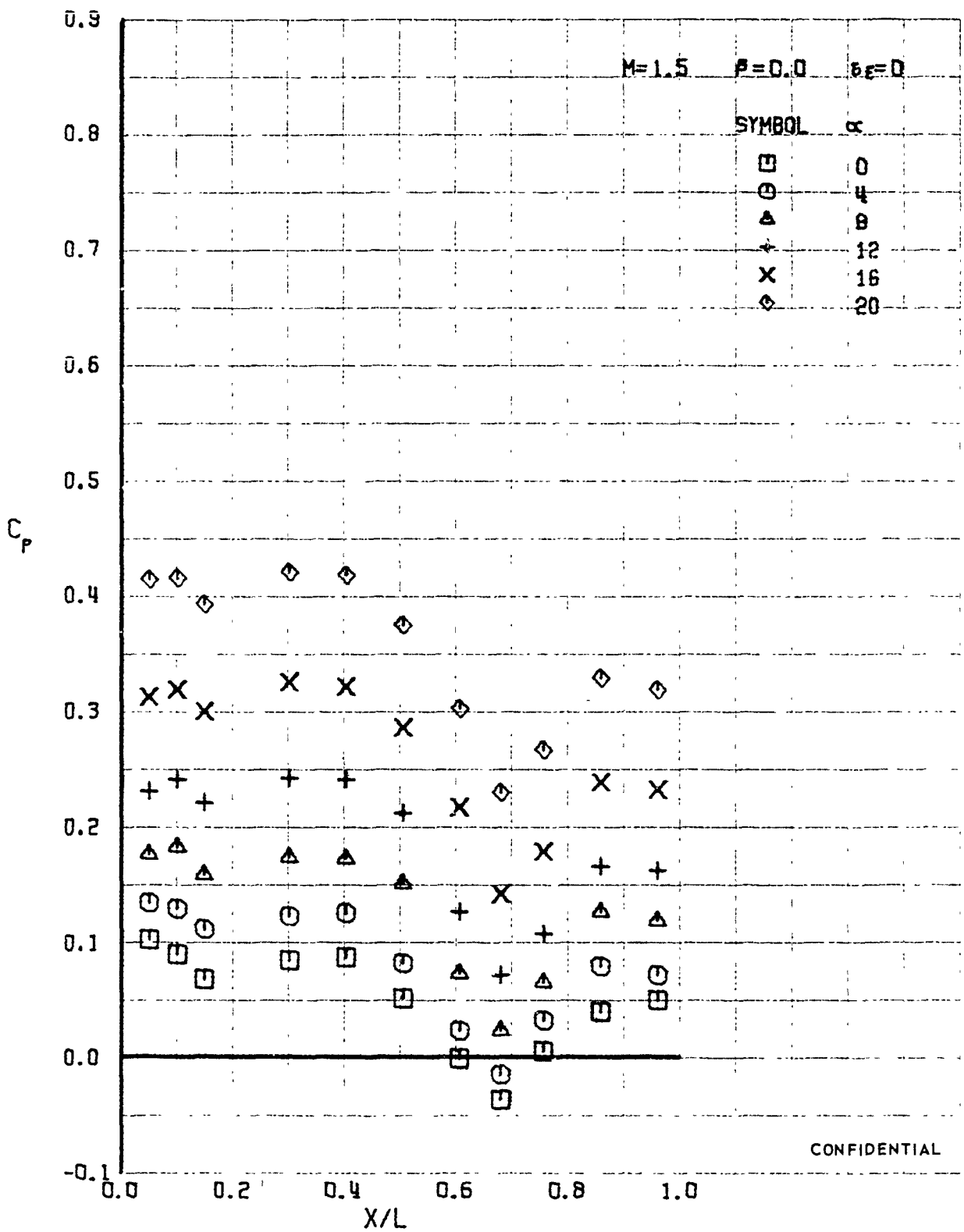
FIGURE 325 (U) LOWER SURFACE CENTERLINE PRESSURES
