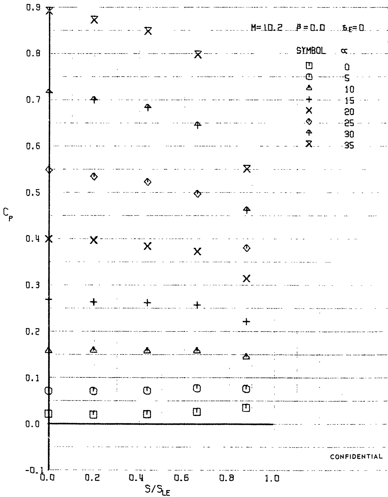
FIGURE 392 (U) LOWER SURFACE SPANWISE PRESSURES AT X/L = 0.30
