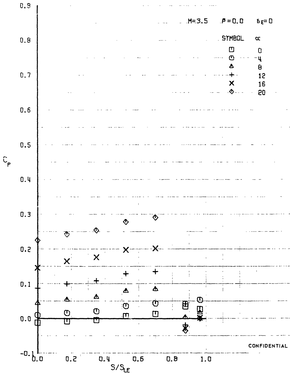
FIGURE 368 (U) LOWER SURFACE SPANWISE PRESSURES AT X/L = 0.76
