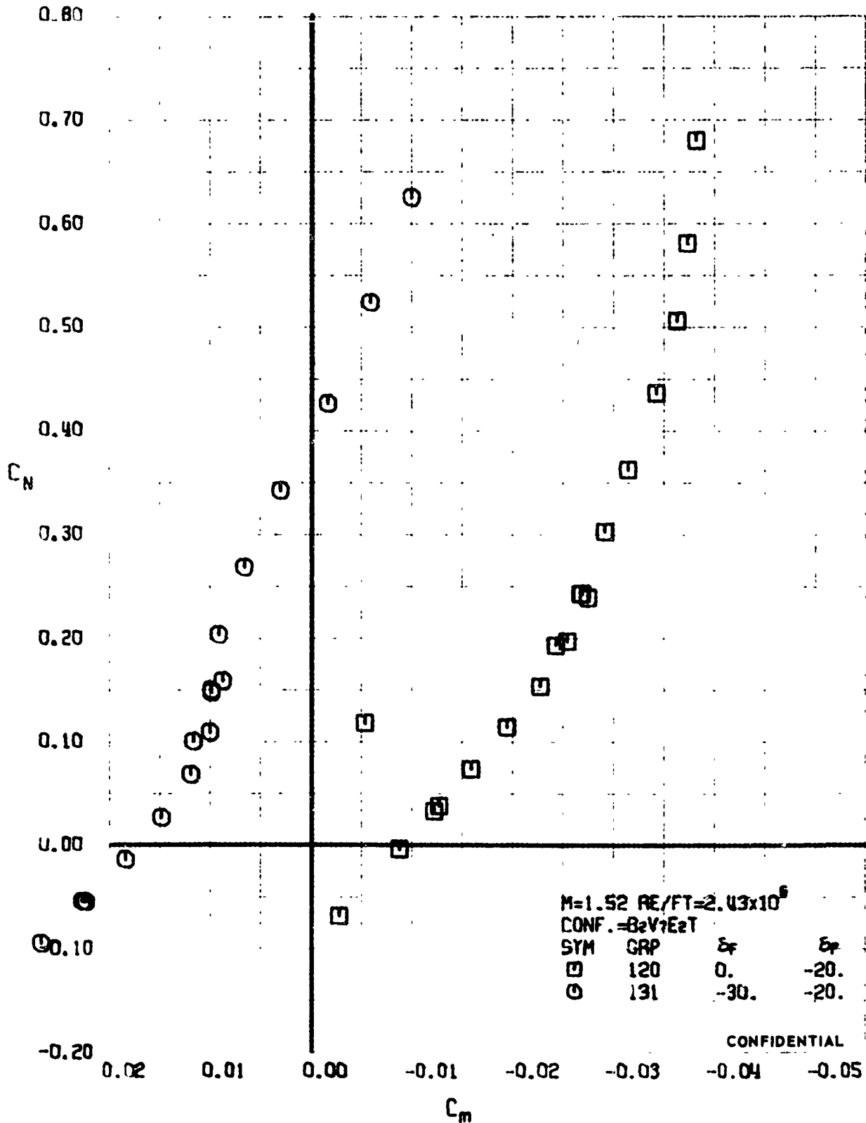
FIGURE 45 (U) FLAP EFFECTS - LONGITUDINAL STABILITY VARIATION (M=1.52)
