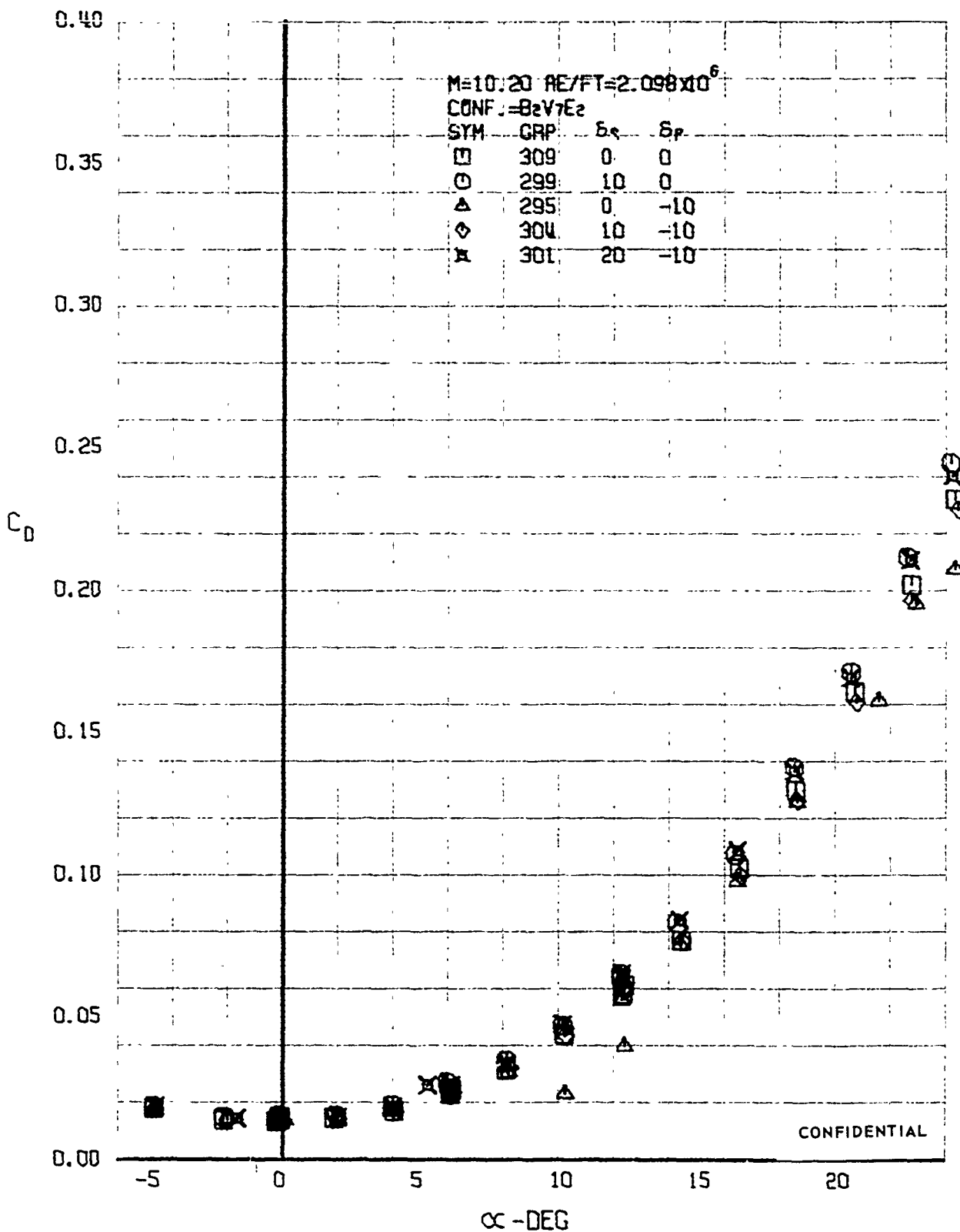
FIGURE 276 (U) AILERON EFFECTS - DRAG COEFFICIENT VARIATION WITH ANGLE OF ATTACK ( M=10.20 )
