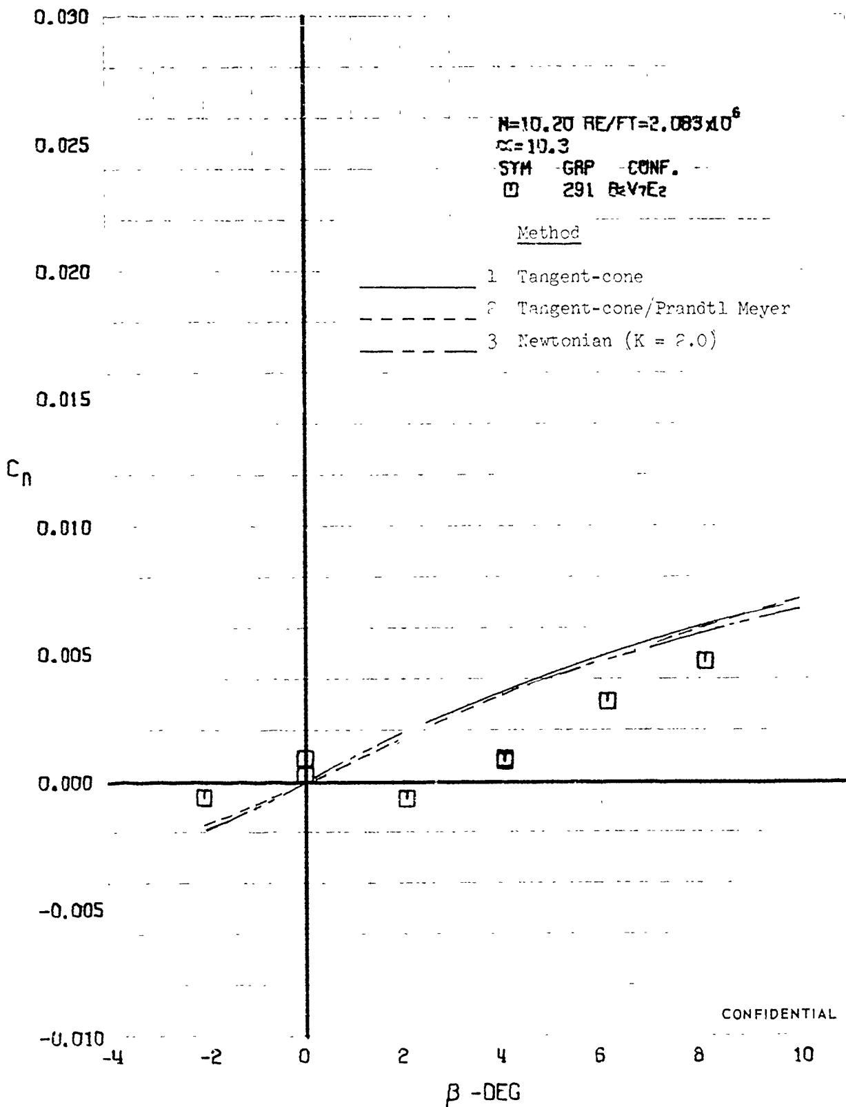
FIGURE 444 (U) COMPARISON OF ESTIMATED AND EXPERIMENTAL COEFFICIENTS - YAWING MOMENT COEFFICIENT VARIATION WITH ANGLE OF YAW ( N=10.20 )
