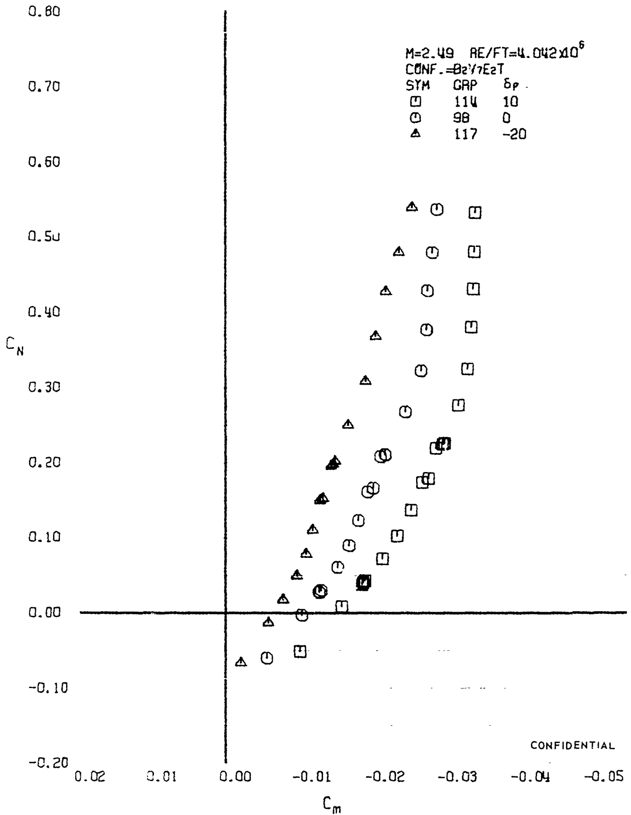
FIGURE 10- (U) ELEVON EFFECTS - LONGITUDINAL STABILITY VARIATION (M=2.49)
