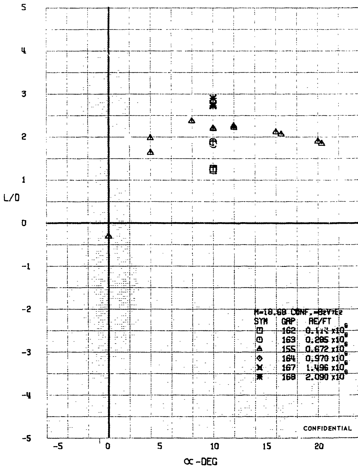
FIGURE 320 (U) REYNOLDS NUMBER EFFECTS - LIFT-DRAG RATIO VARIATION WITH ANGLE OF ATTACK (M=18.68)
