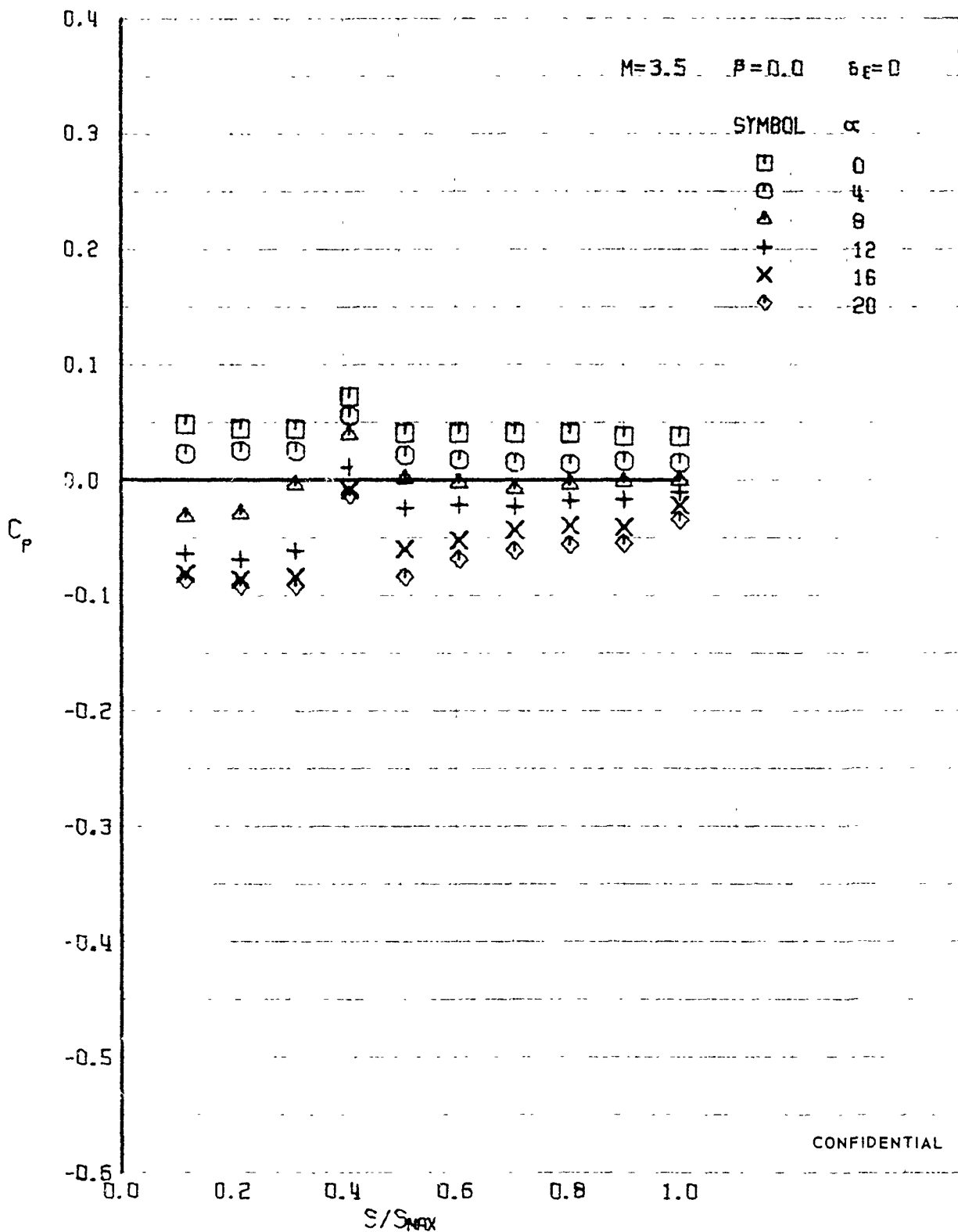
FIGURE 373 (U) UPPER SURFACE SPANWISE PRESSURES AT X/L = 0.50
