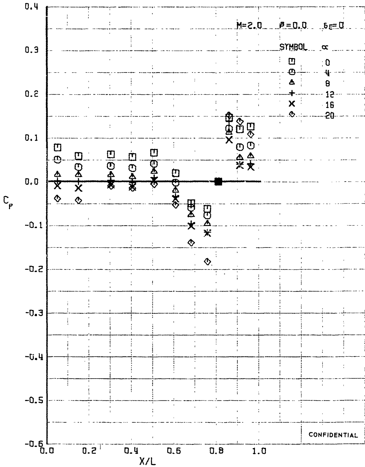
FIGURE 344 (U) UPPER SURFACE CENTERLINE PRESSURES
