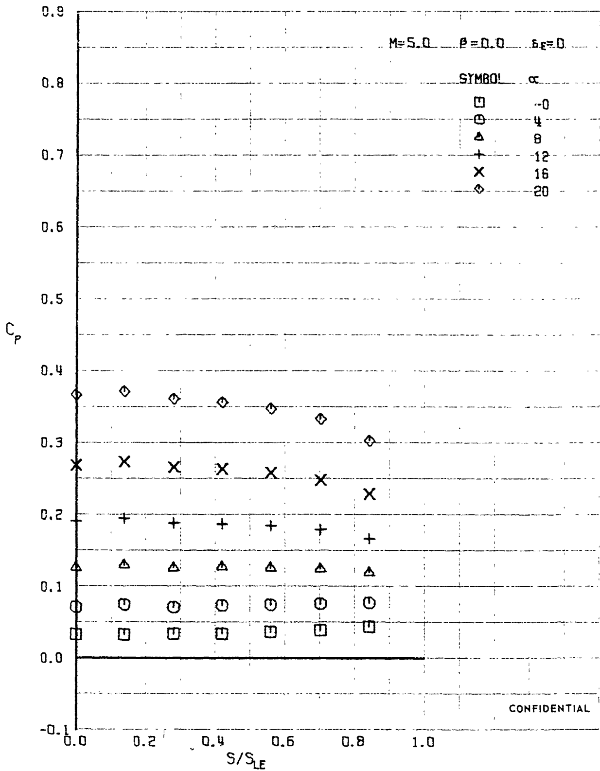
FIGURE 380 (U) LOWER SURFACE SPANWISE PRESSURES AT X/L = 0.50
