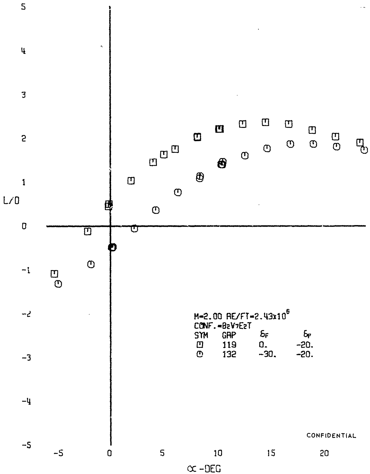
FIGURE 8, (U) FLAP EFFECTS - LIFT-DRAG RATIO VARIATION WITH ANGLE OF ATTACK (M=2.00)
