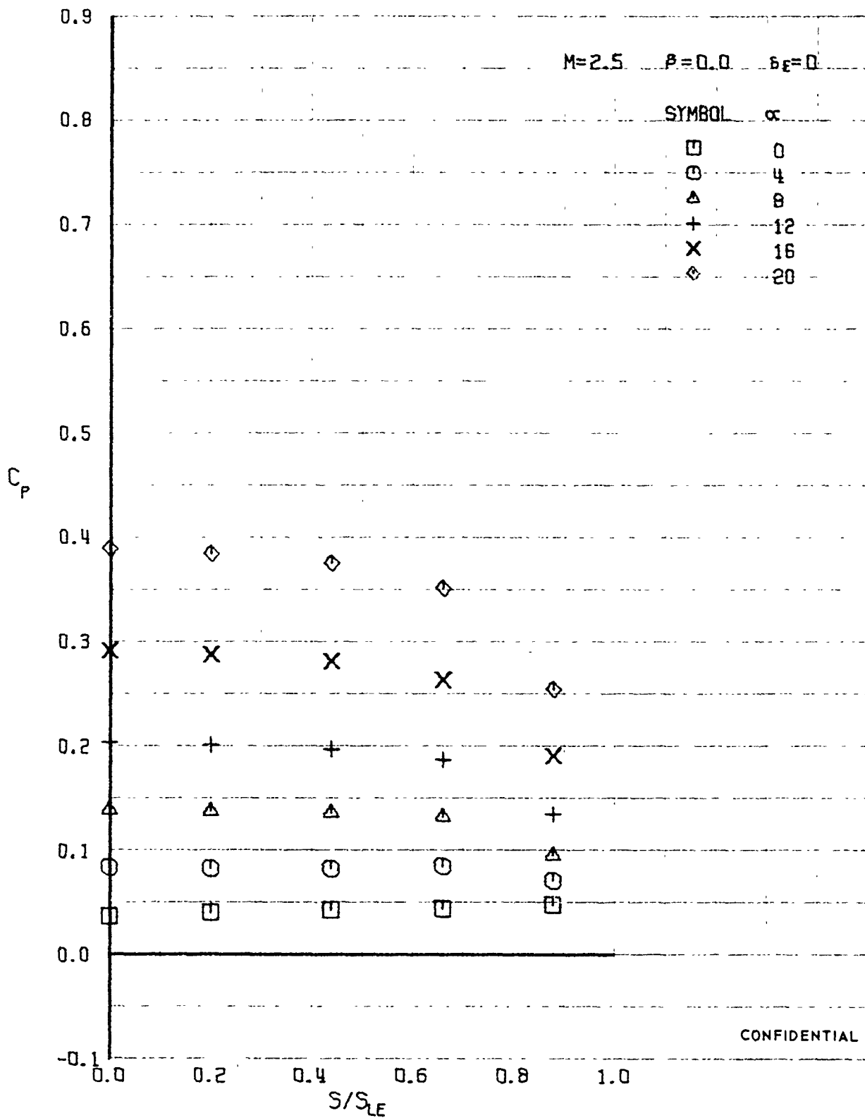
FIGURE 353 (U) LOWER SURFACE SPANWISE PRESSURES AT X/L = 0.30
