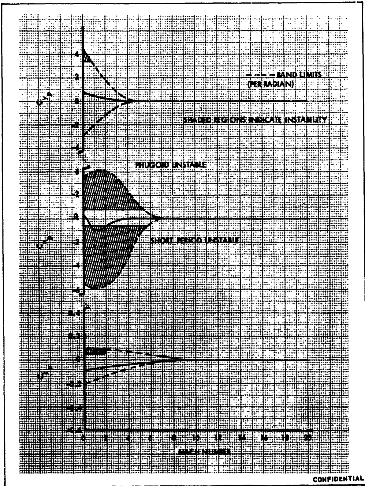
FIGURE 493 (U) VARIATION OF \rho DERIVATIVES WITH MACH NUMBER
