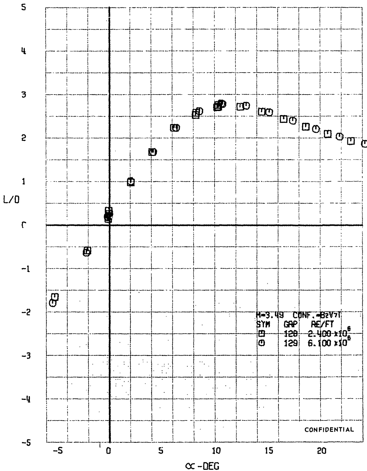
FIGURE 182 (U) REYNOLDS NUMBER EFFECTS - LIFT-DRAG RATIO VARIATION WITH ANGLE OF ATTACK (M=3.49)
