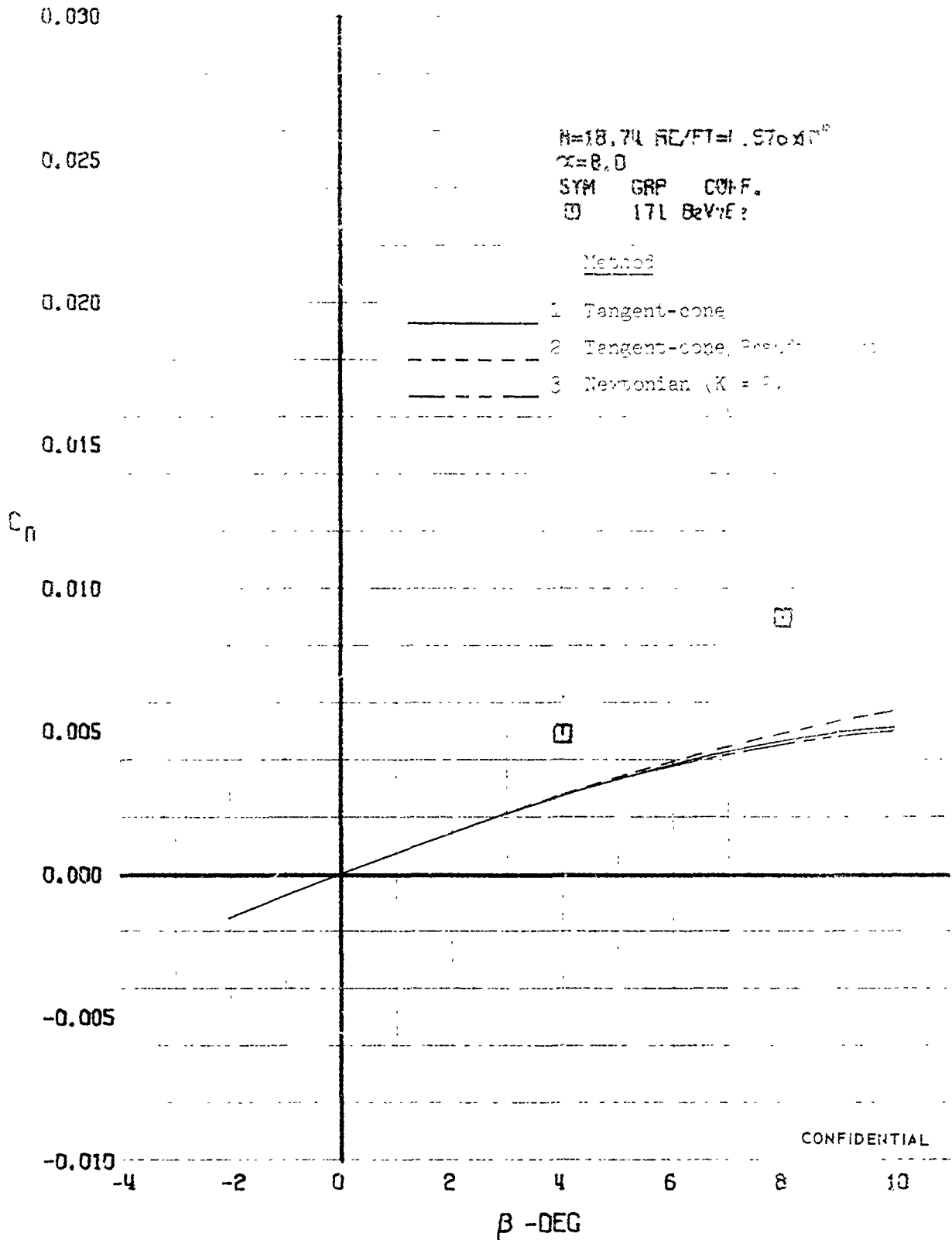
FIGURE 447 (U) COMPARISON OF ESTIMATED AND EXPERIMENTAL COEFFICIENTS - TAKING MOMENT COEFFICIENT VARIATION WITH ANGLE OF TAW ( M=18.74 )
