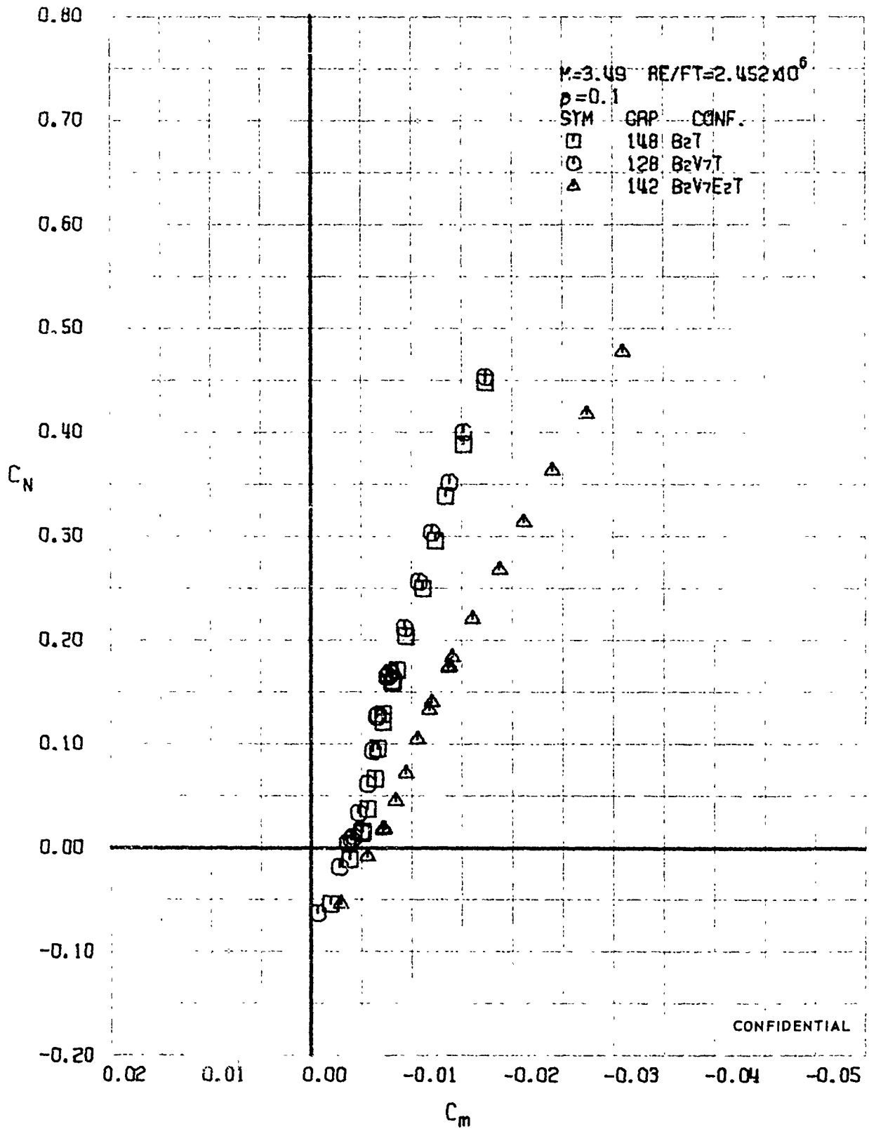
FIGURE 153 (U) CONFIGURATION BUILDUP - LONGITUDINAL STABILITY VARIATION (M=3.49)
