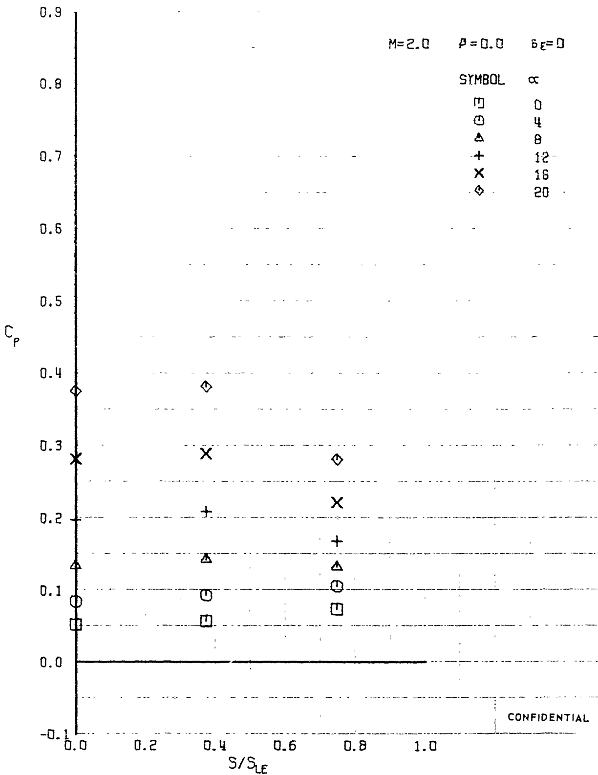
FIGURE 339 (U) LOWER SURFACE SPANWISE PRESSURES AT X/L = 0.15
