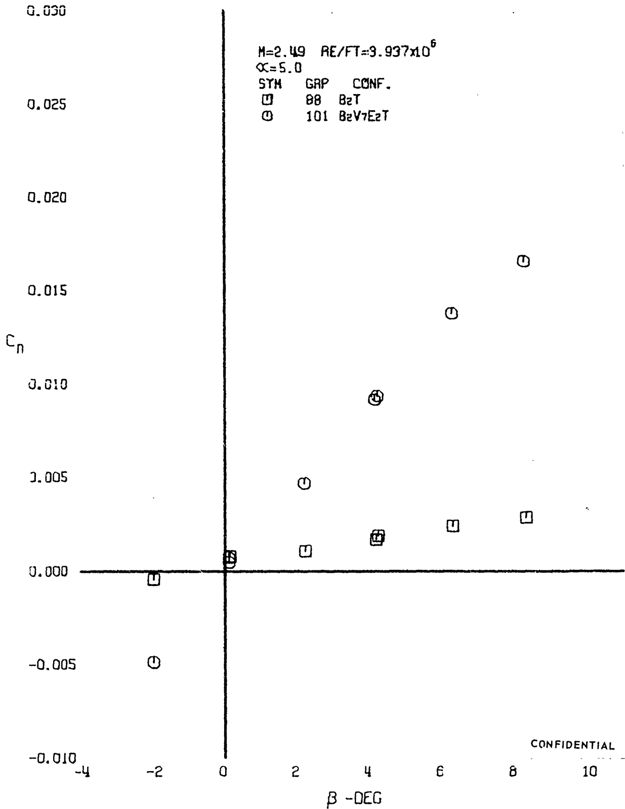
FIGURE 114 (U) CONFIGURATION BUILDUP - YAWING MOMENT COEFFICIENT VARIATION WITH ANGLE OF YAW (M=2.49)
