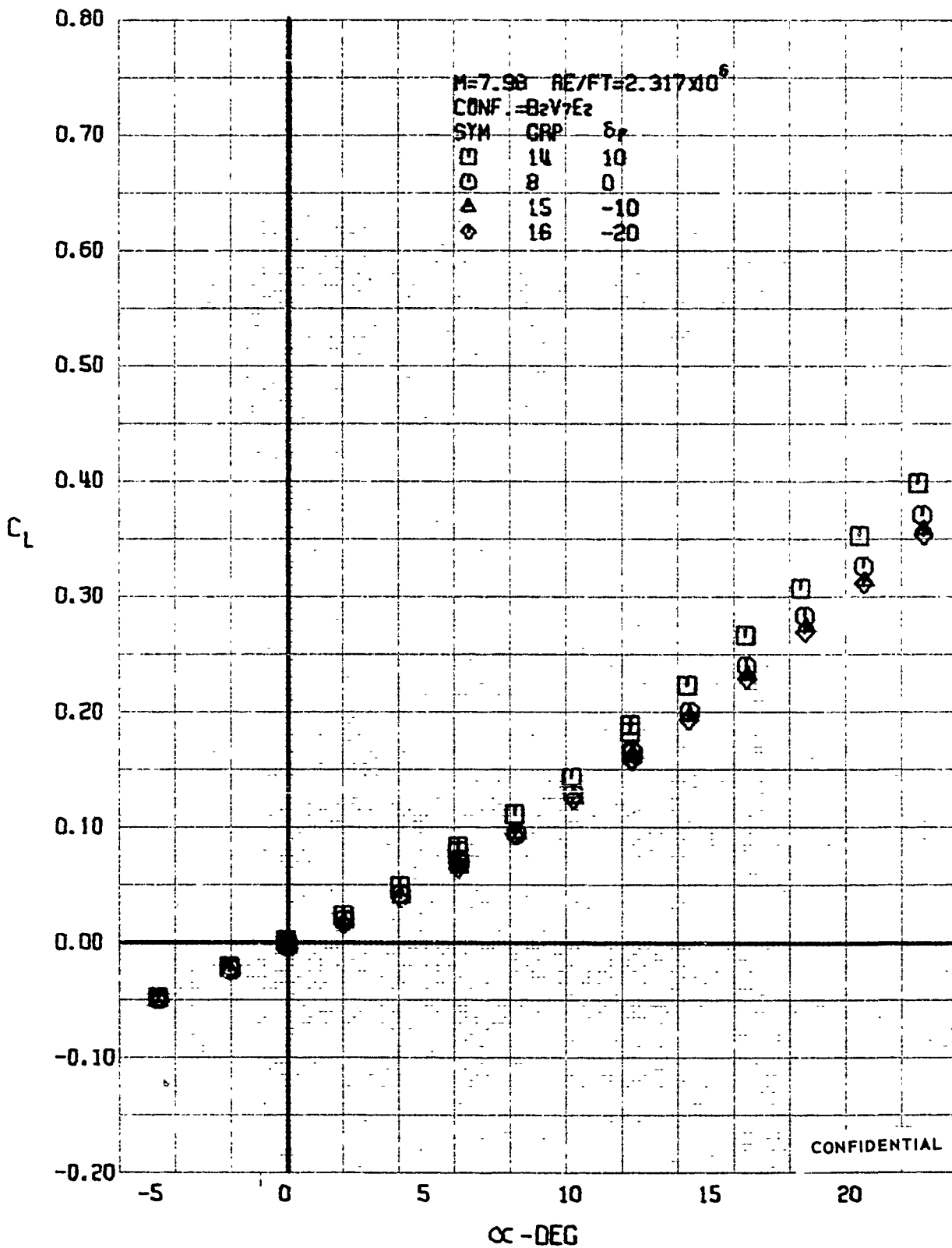
FIGURE 234 (U) ELEVON EFFECTS - LIFT COEFFICIENT VARIATION WITH ANGLE OF ATTACK (M=7.98)
