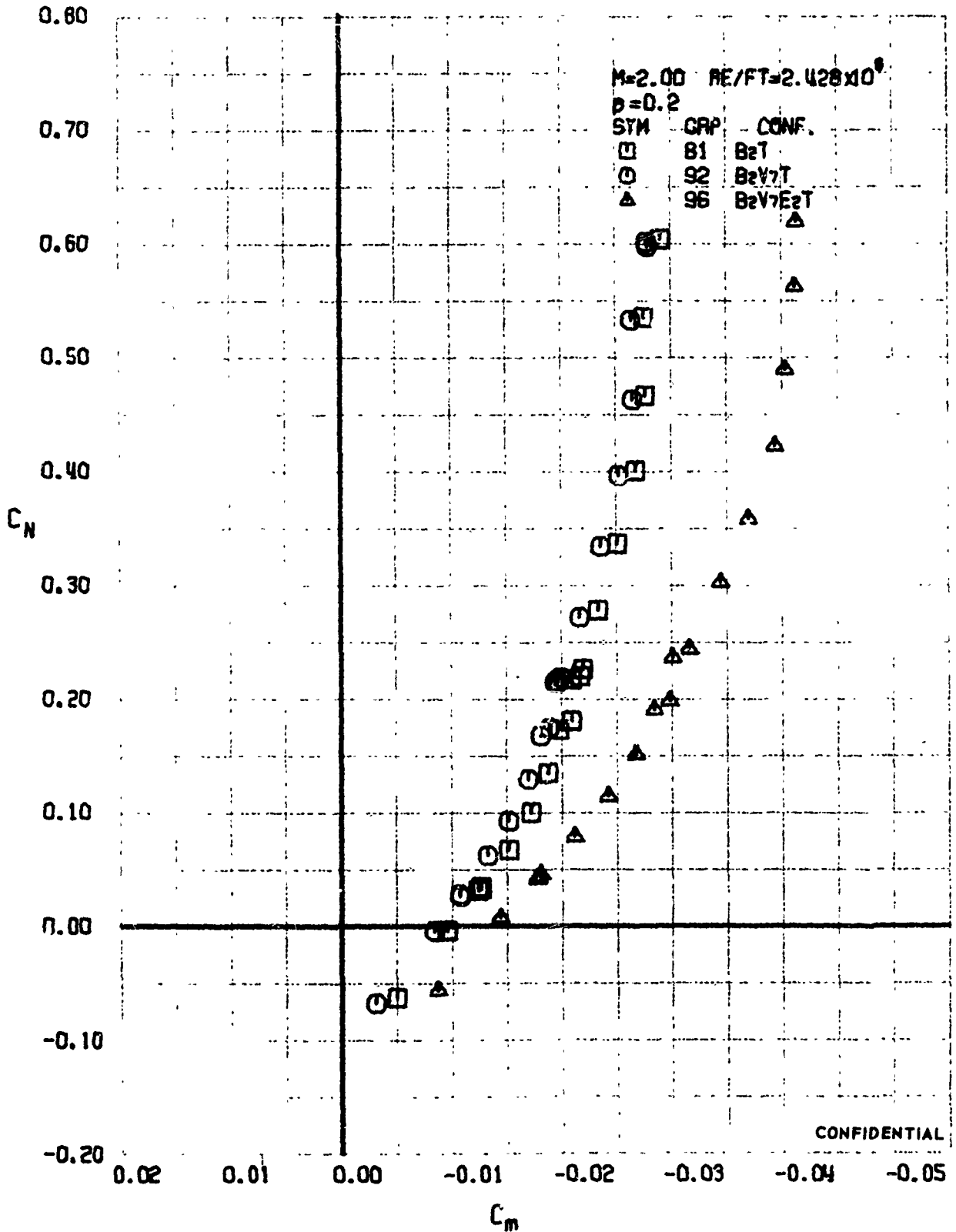
FIGURE 60 (U) CONFIGURATION BUILDUP - LONGITUDINAL STABILITY VARIATION (M=2.00)
