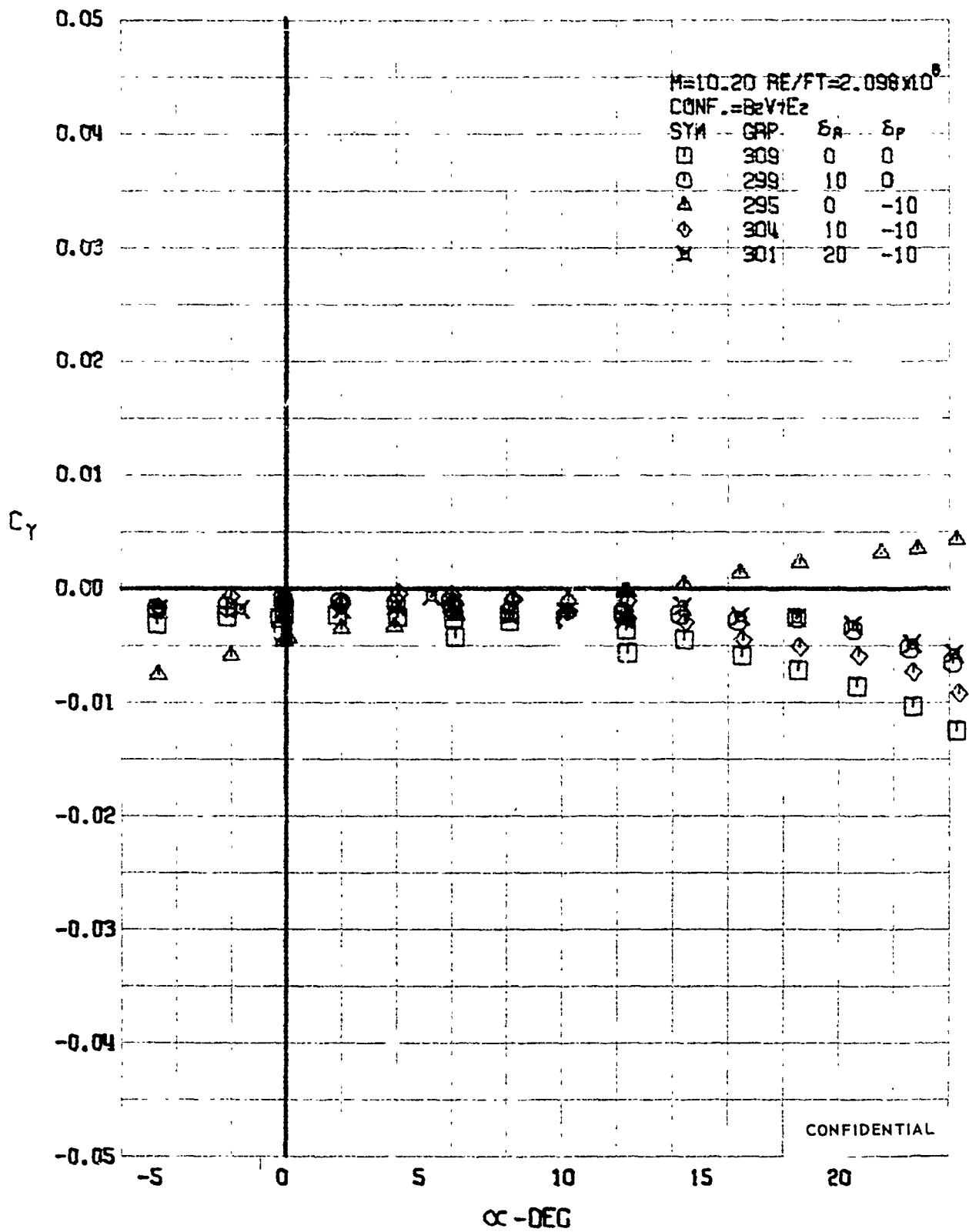
FIGURE 278 (U) AILERON EFFECTS - SIDE FORCE COEFFICIENT VARIATION WITH ANGLE OF ATTACK ( M=10.20 )
