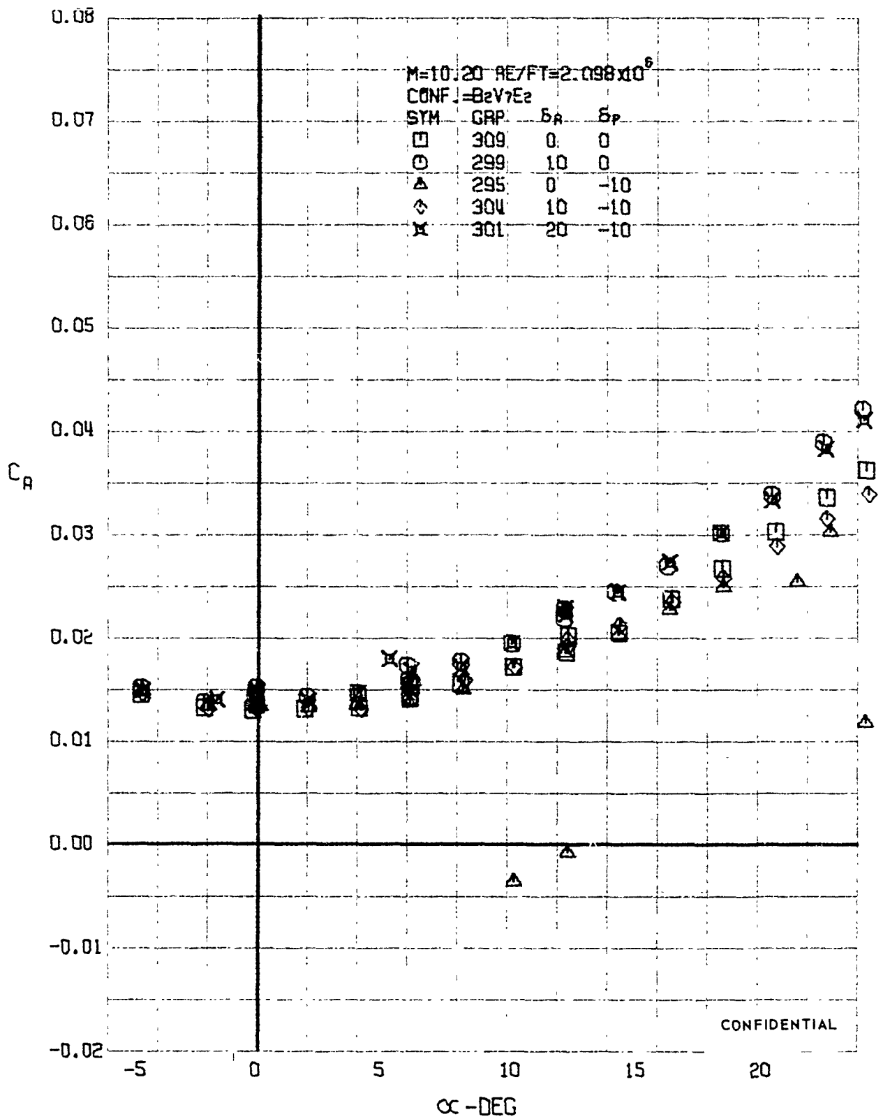
FIGURE 271 (U) AILERON EFFECTS - AXIAL FORCE COEFFICIENT VARIATION WITH ANGLE OF ATTACK ( M=10.20 )
