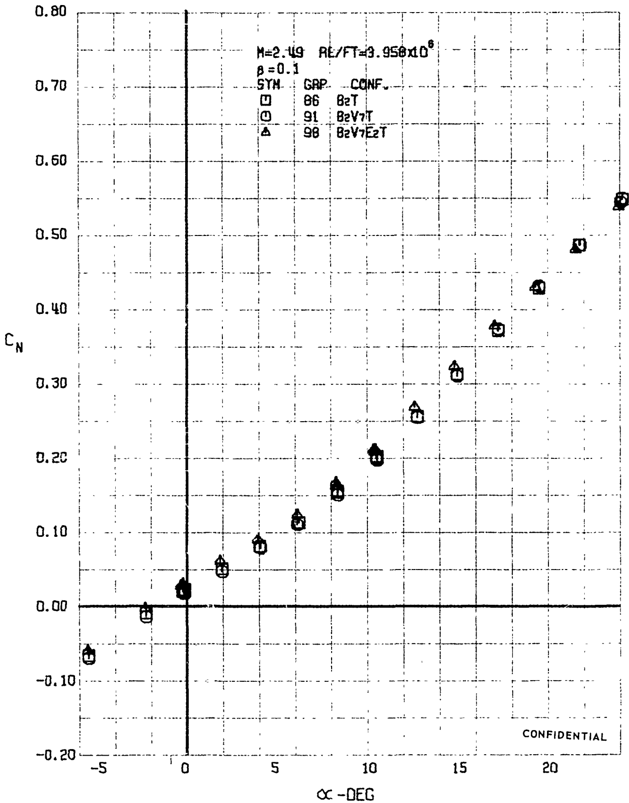
FIGURE 103 (U) CONFIGURATION BUILDUP - NORMAL FORCE COEFFICIENT VARIATION WITH ANGLE OF ATTACK (M=2.49)
