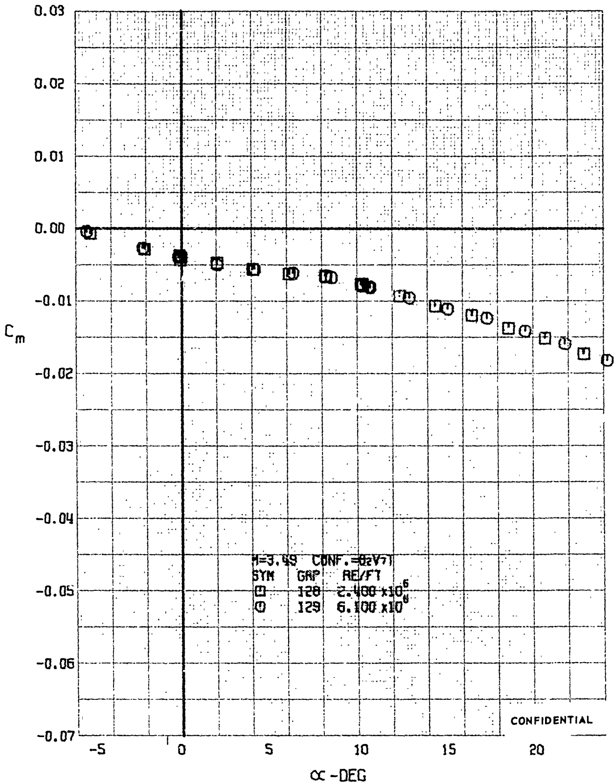
FIGURE 178 (U) REYNOLDS NUMBER EFFECTS - PITCHING MOMENT COEFFICIENT VARIATION WITH ANGLE OF ATTACK ( M=3.49 )
