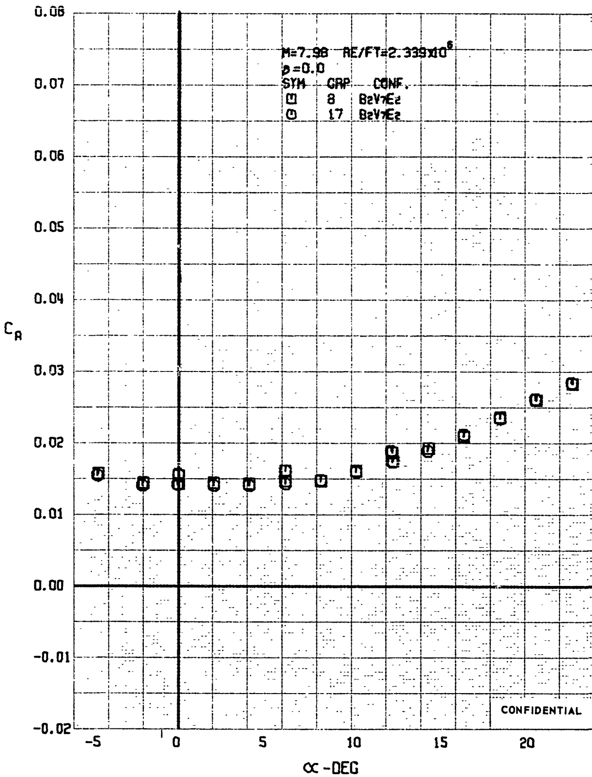
FIGURE 237 (U) REPEATABILITY - AXIAL FORCE COEFFICIENT VARIATION WITH ANGLE OF ATTACK (M=7.98)
