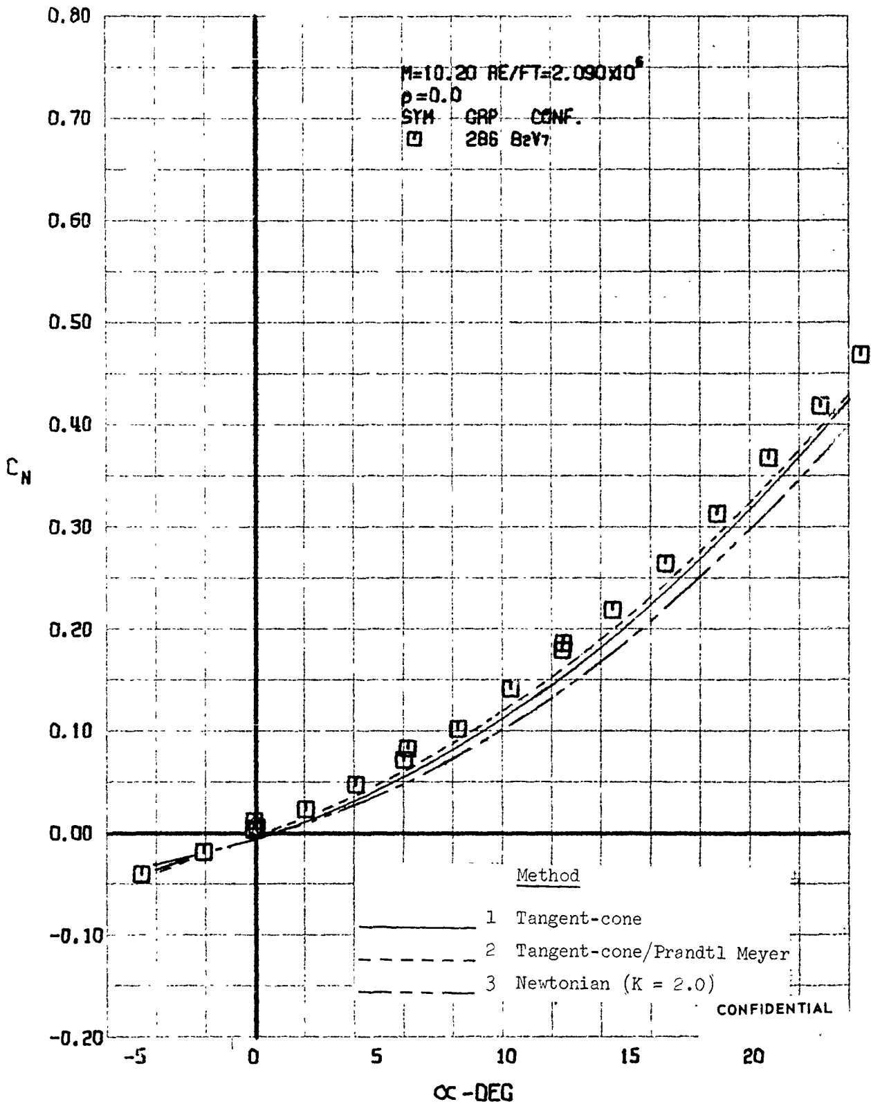
FIGURE 419 (U) COMPARISON OF ESTIMATED AND EXPERIMENTAL COEFFICIENTS - NORMAL FORCE COEFFICIENT VARIATION WITH ANGLE OF ATTACK ( M=10.20 )
