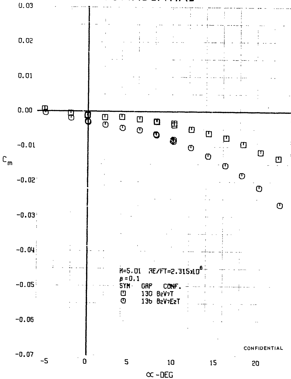
FIGURE 18 o (U) CONFIGURATION BUILDUP - PITCHING MOMENT COEFFICIENT VARIATION WITH ANGLE OF ATTACK (M=5.01)
