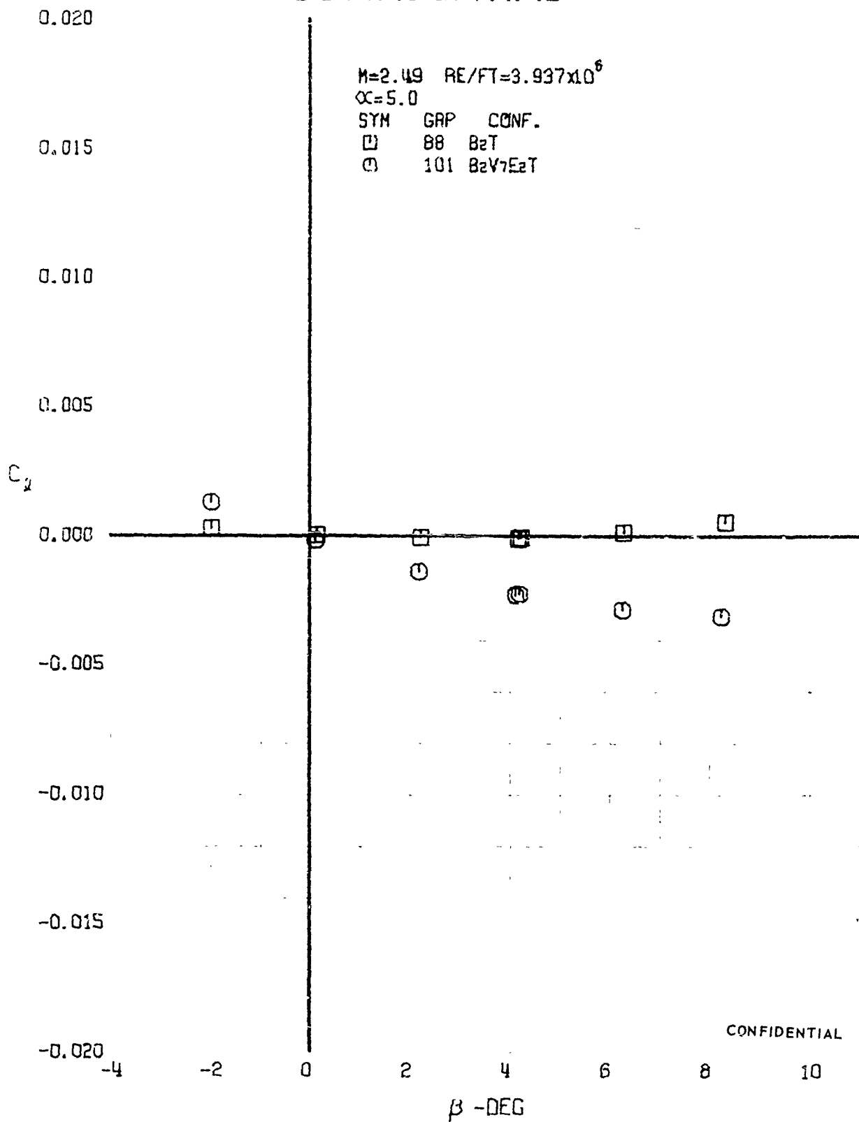
FIGURE 113 (U) CONFIGURATION BUILDUP - ROLLING MOMENT COEFFICIENT VARIATION WITH ANGLE OF YAW ( M=2.49 )
