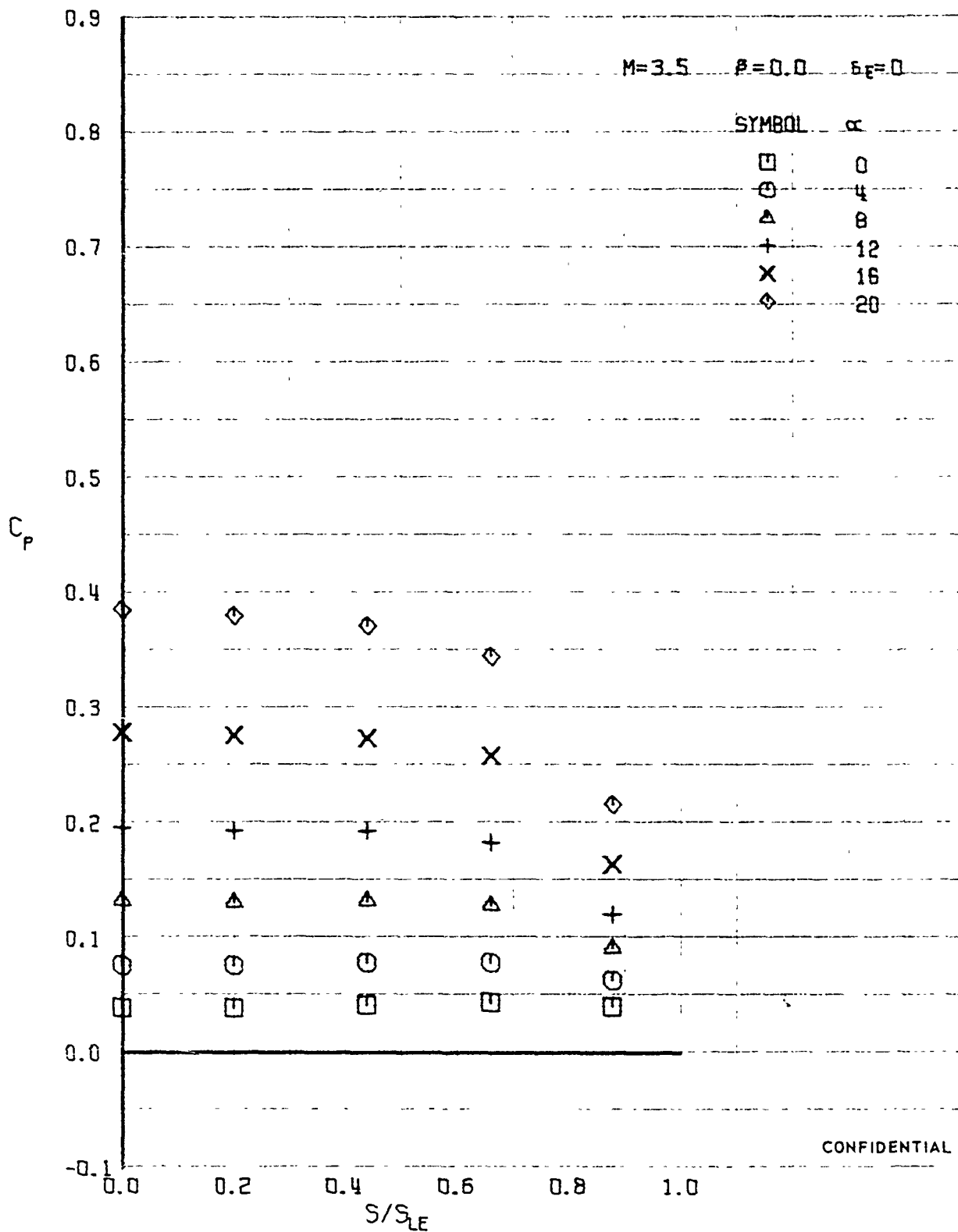
FIGURE 366 (U) LOWER SURFACE SPANWISE PRESSURES AT X/L = 0.30
