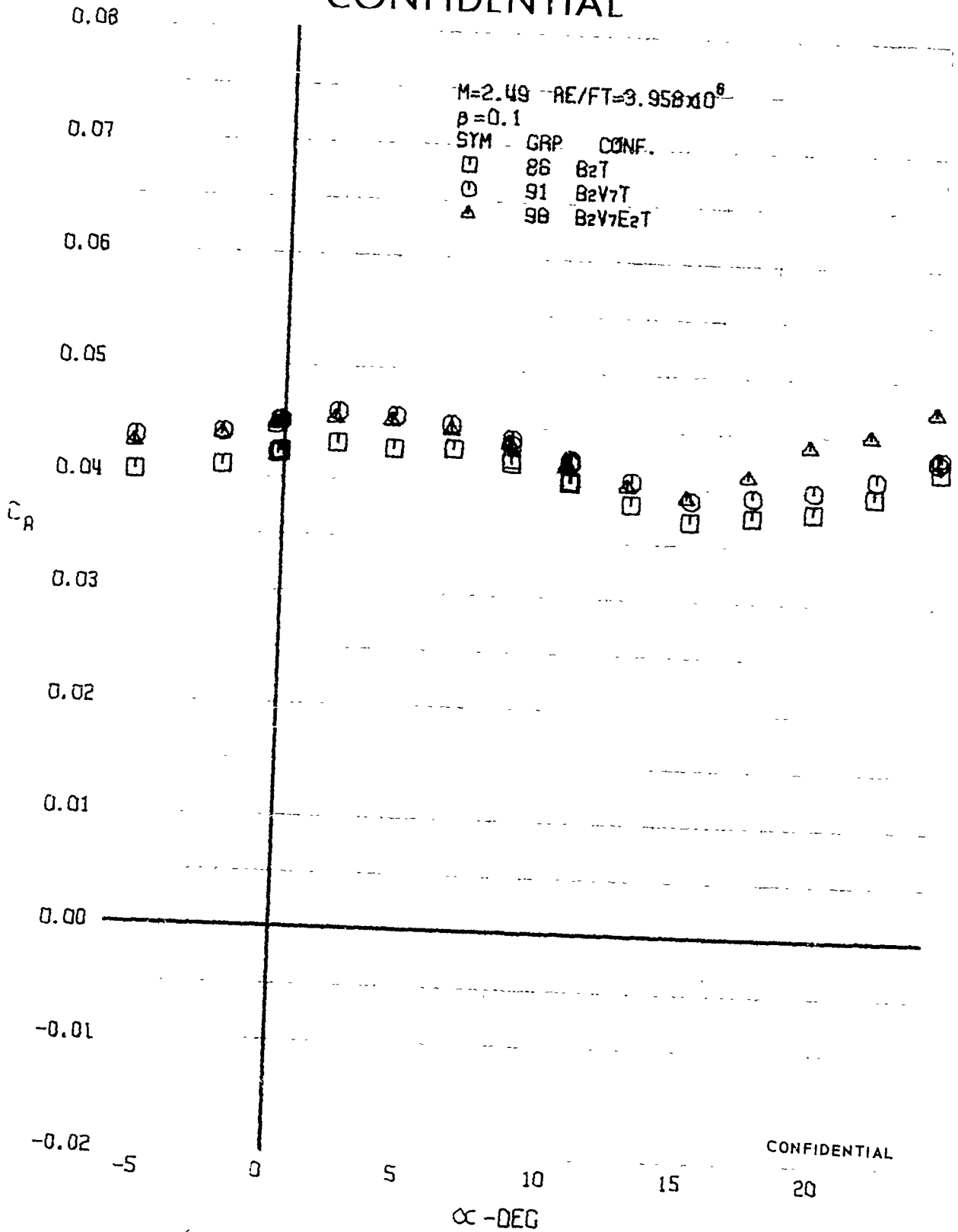
FIGURE 102 (U) CONFIGURATION BUILDUP - AXIAL FORCE COEFFICIENT VARIATION WITH ANGLE OF ATTACK (M=2.49)
