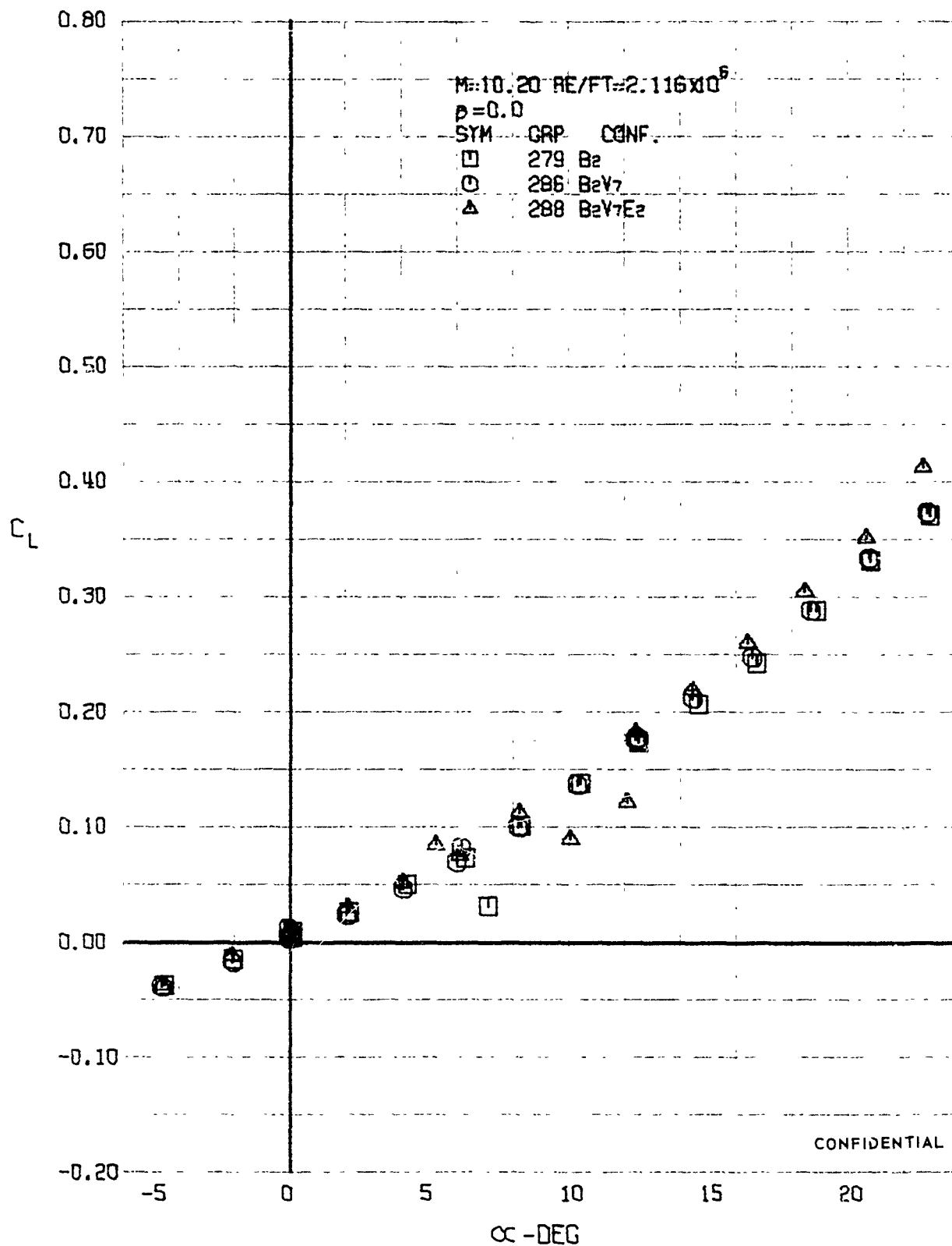
FIGURE 245 (U) CONFIGURATION BUILDUP - LIFT COEFFICIENT VARIATION WITH ANGLE OF ATTACK (M=10.20)
