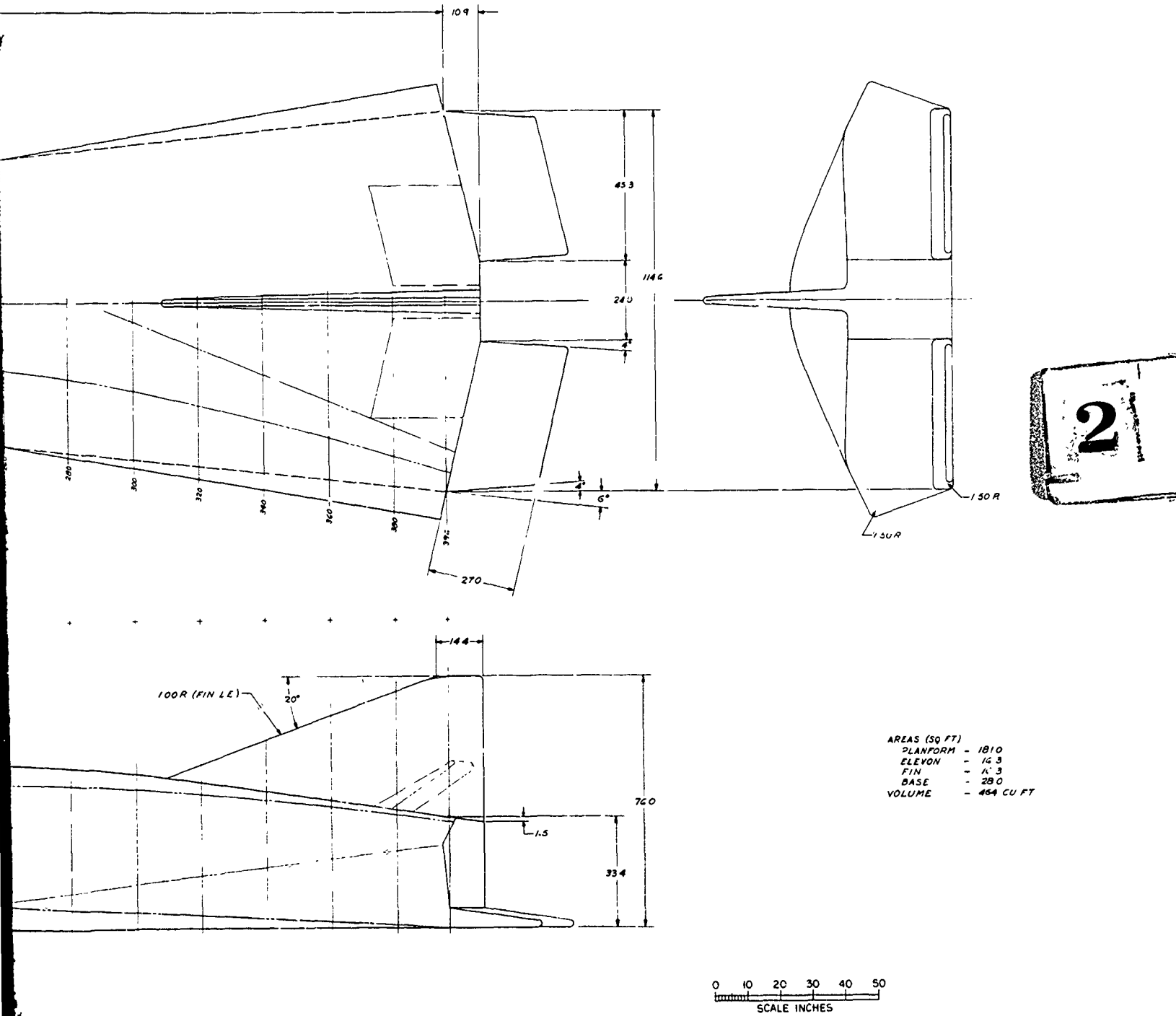
FIGURE 1 (U) FD7-5 TEST CONFIGURATION
