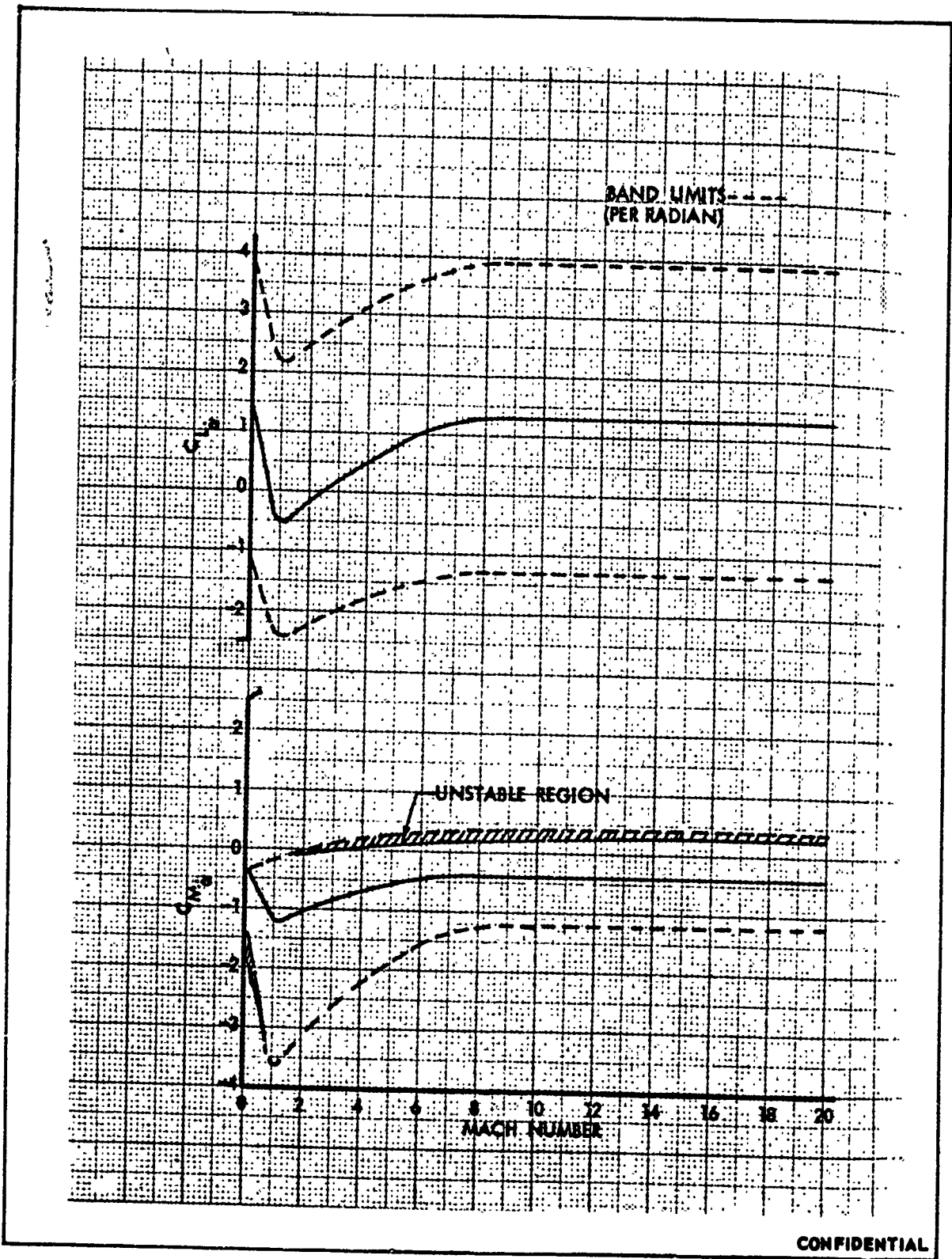
FIGURE 491 (U) VARIATION OF \infty DERIVATIVES WITH MACH NUMBER
