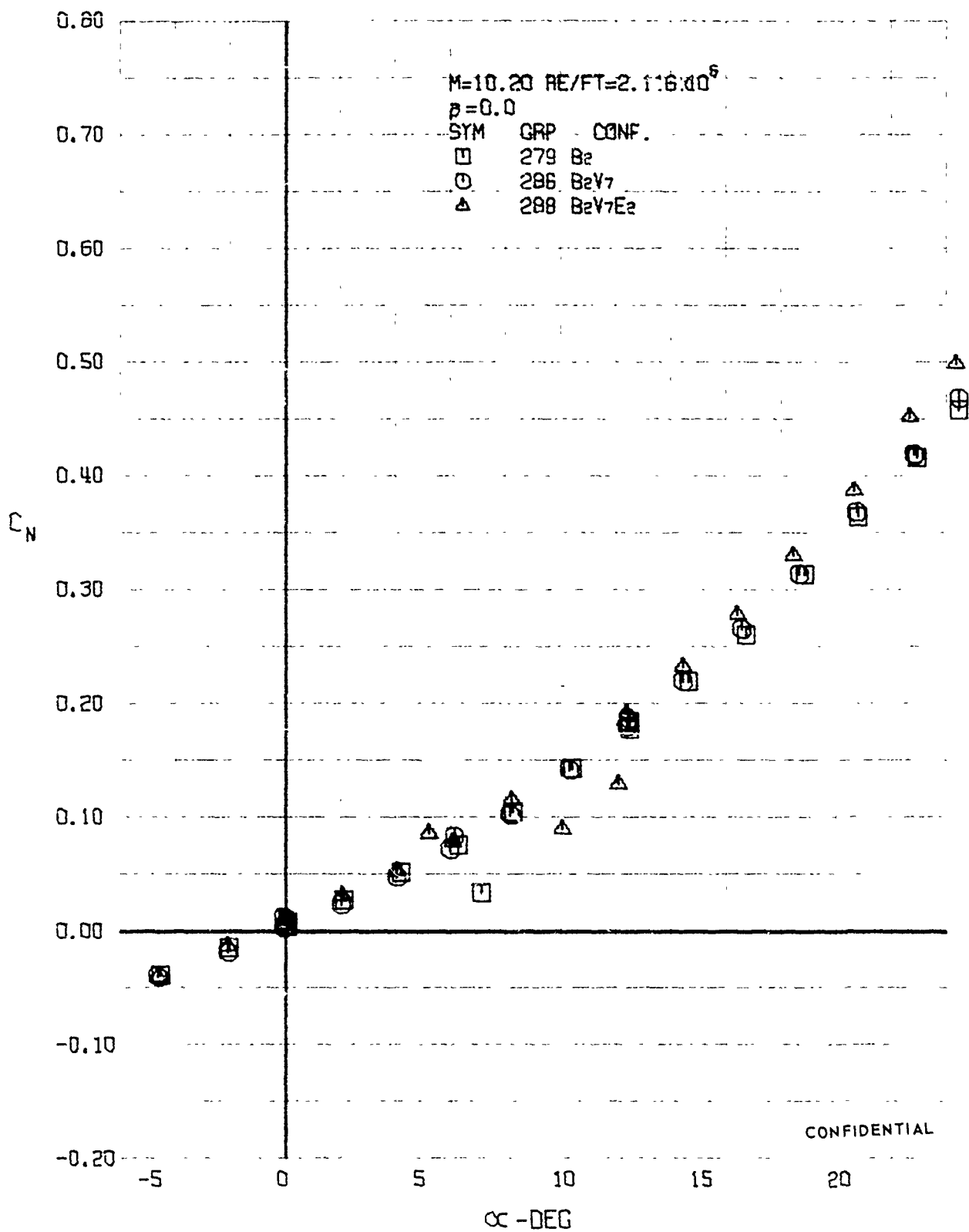
FIGURE 242 (U) CONFIGURATION BUILDUP - NORMAL FORCE COEFFICIENT VARIATION WITH ANGLE OF ATTACK ( M=10.20 )
