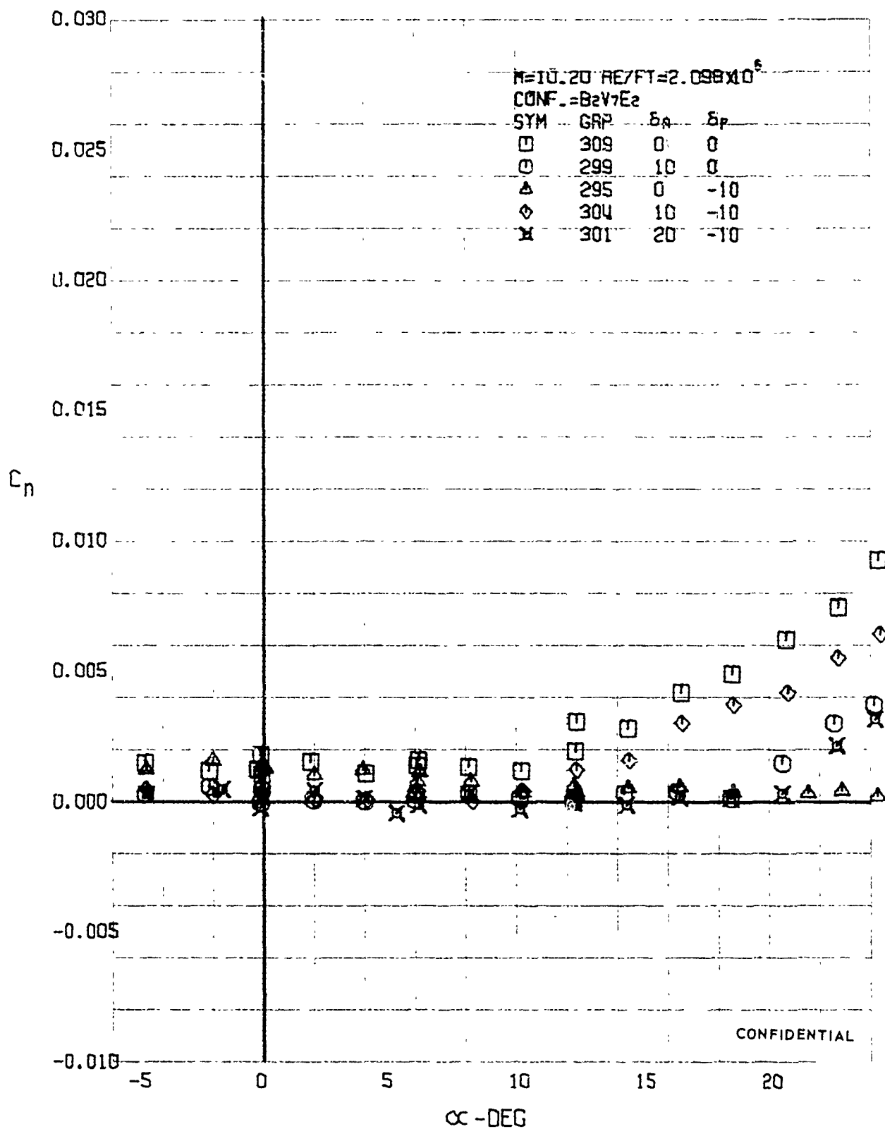
FIGURE 279 (U) AILERON EFFECTS - YAWING MOMENT COEFFICIENT VARIATION WITH ANGLE OF ATTACK M=10.20
