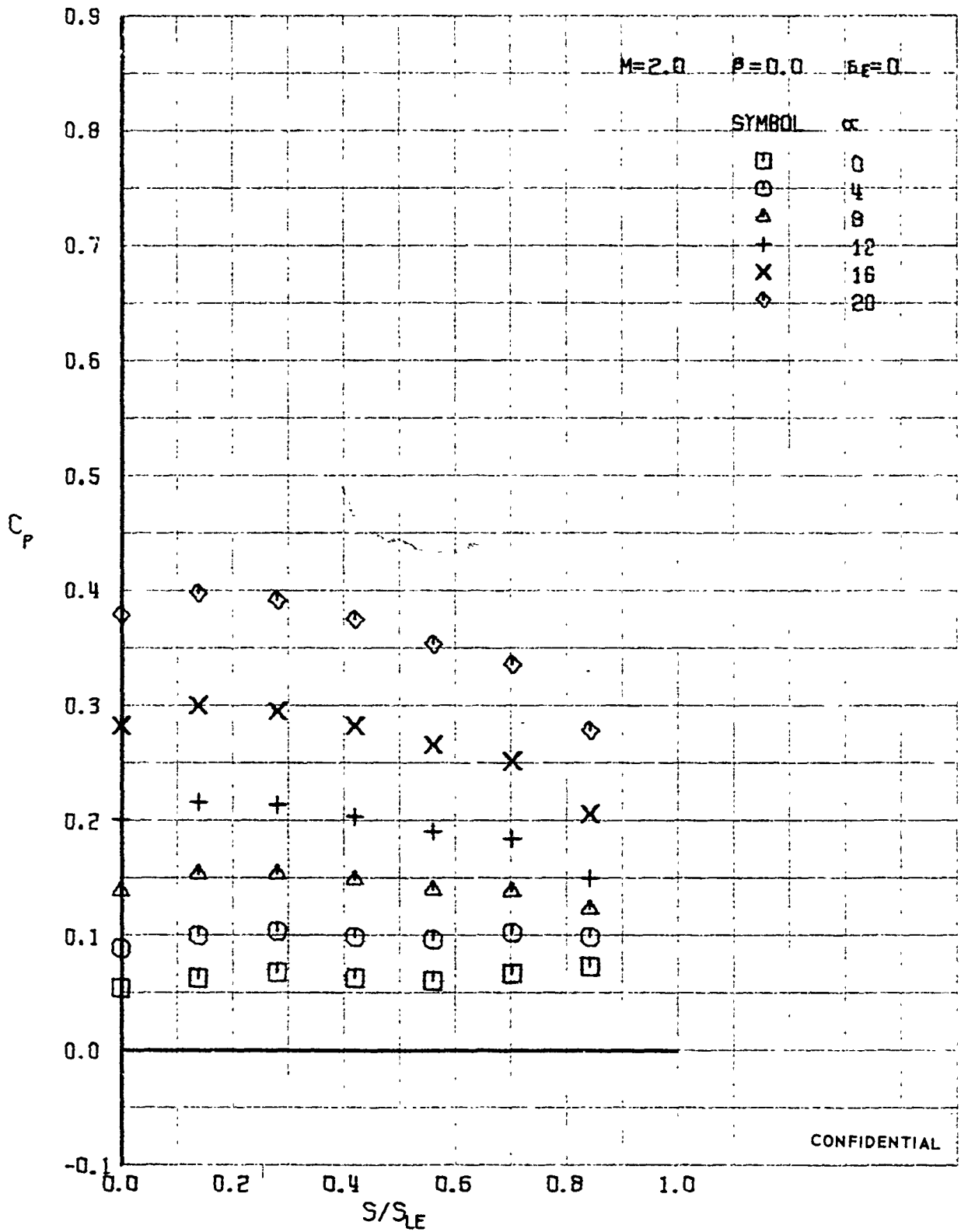
FIGURE 341 (U) LOWER SURFACE SPANWISE PRESSURES AT X/L = 0.5^*
