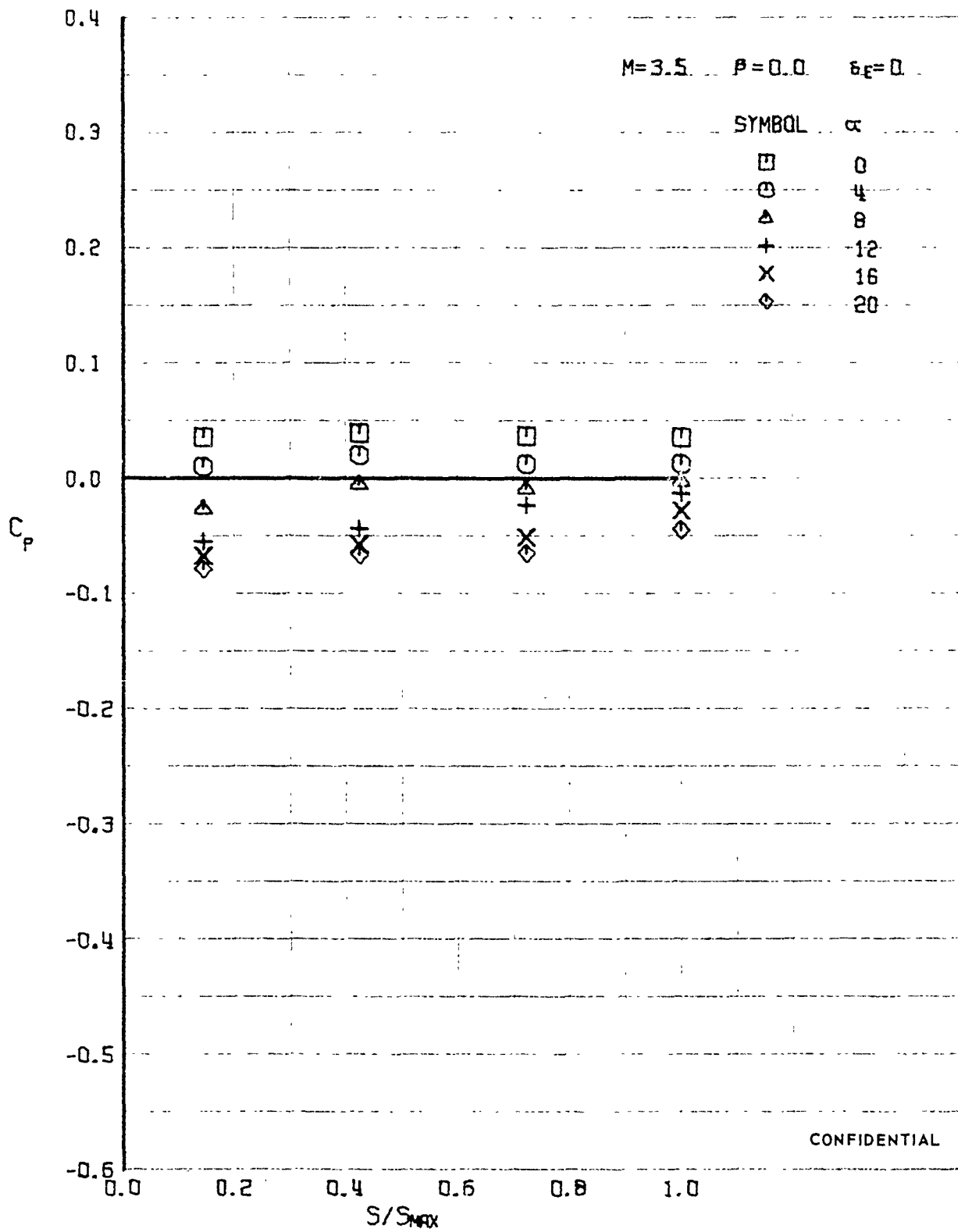
FIGURE 371 (U) UPPER SURFACE SPANWISE PRESSURES AT X/L = 0.15
