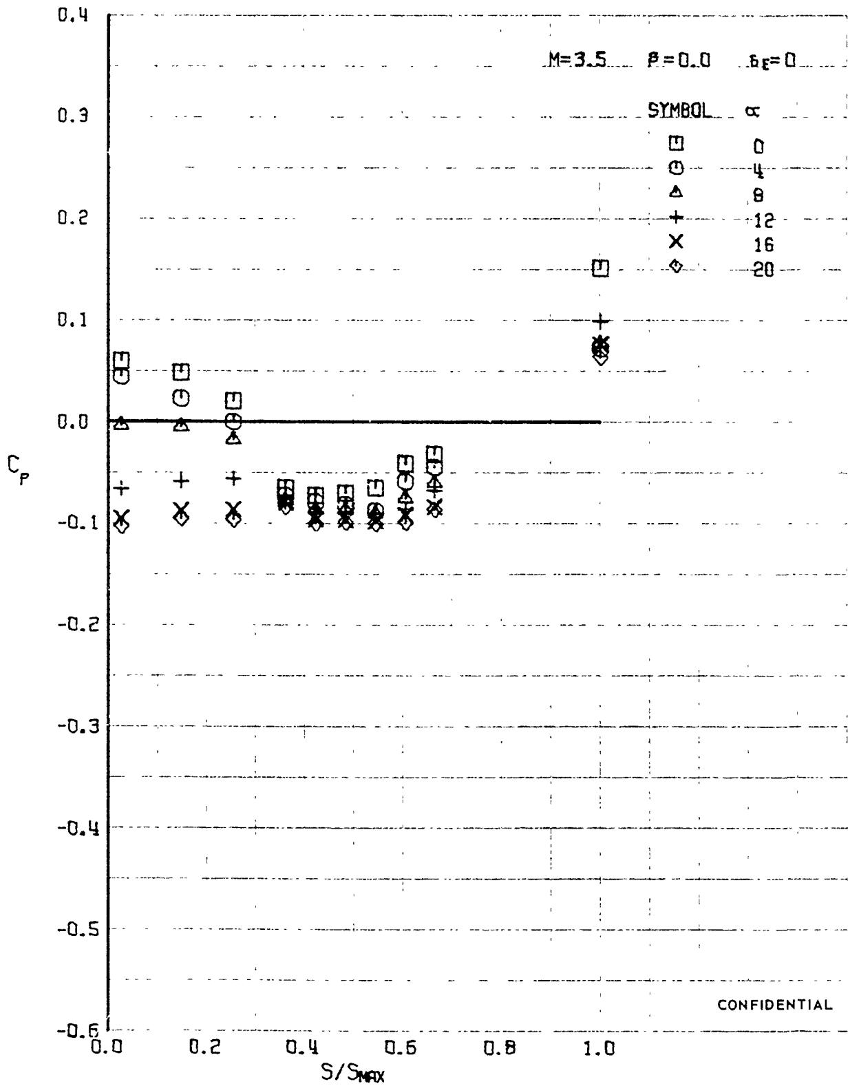
FIGURE 375 (U) UPPER SURFACE SPANWISE PRESSURES AT X/L = 0.86
