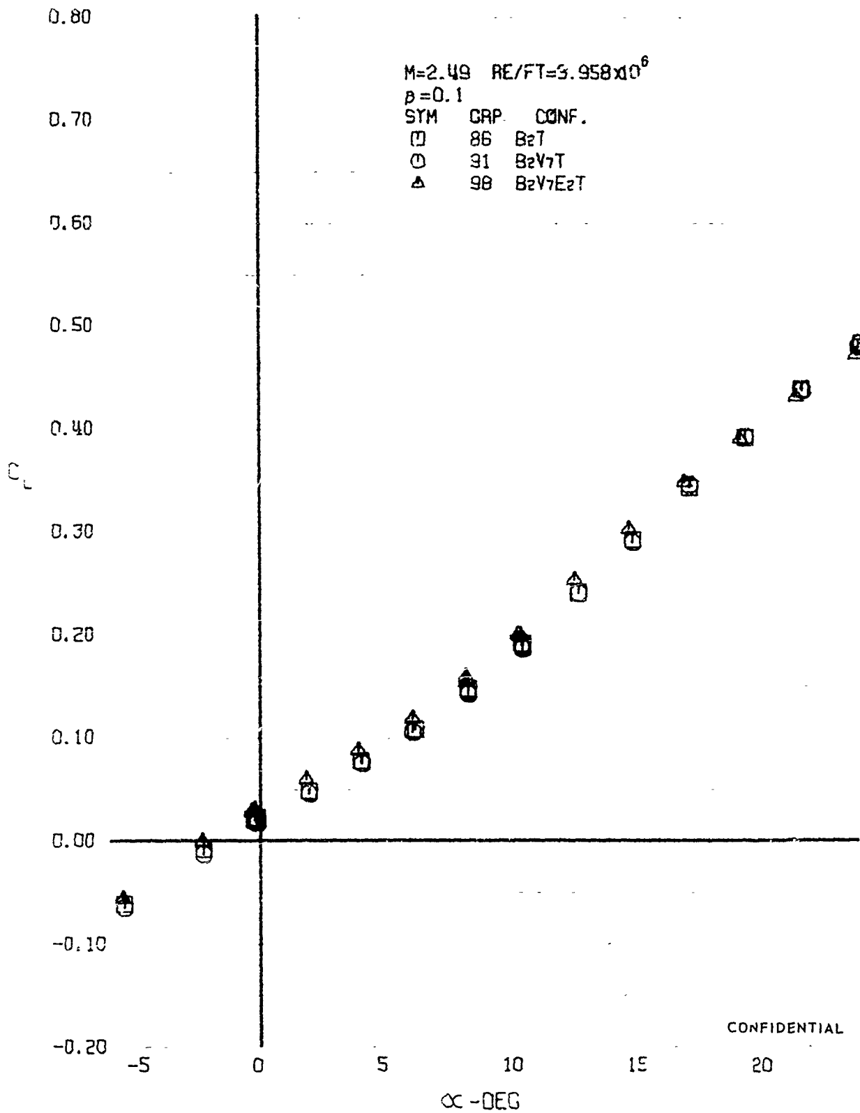
FIGURE 106 (U) CONFIGURATION BUILDUP - LIFT COEFFICIENT VARIATION WITH ANGLE OF ATTACK (M=2.49)
