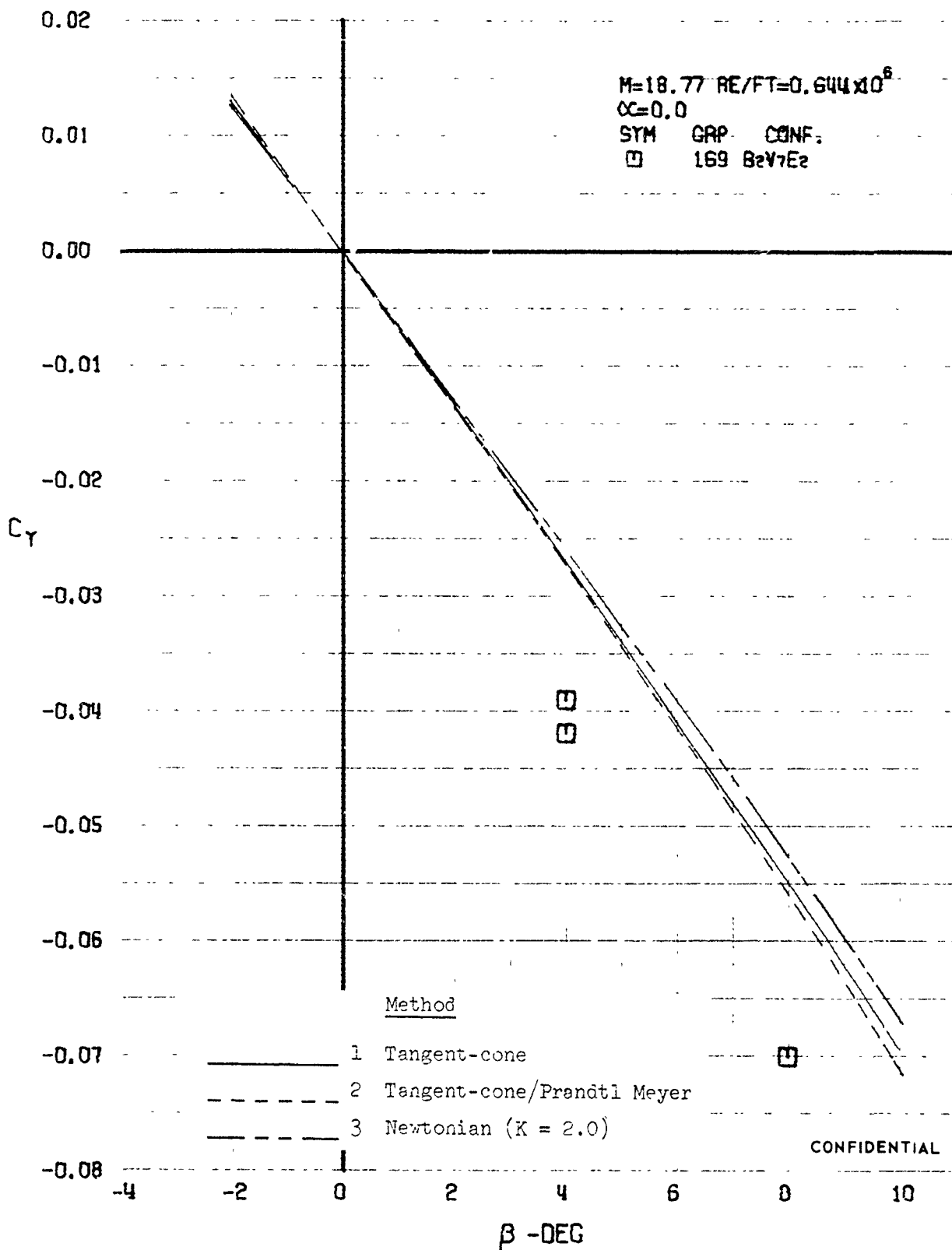
FIGURE 434 (U) COMPARISON OF ESTIMATED AND EXPERIMENTAL COEFFICIENTS - SIDE FORCE COEFFICIENT VARIATION WITH ANGLE OF YAW ( M = 18.7 )
