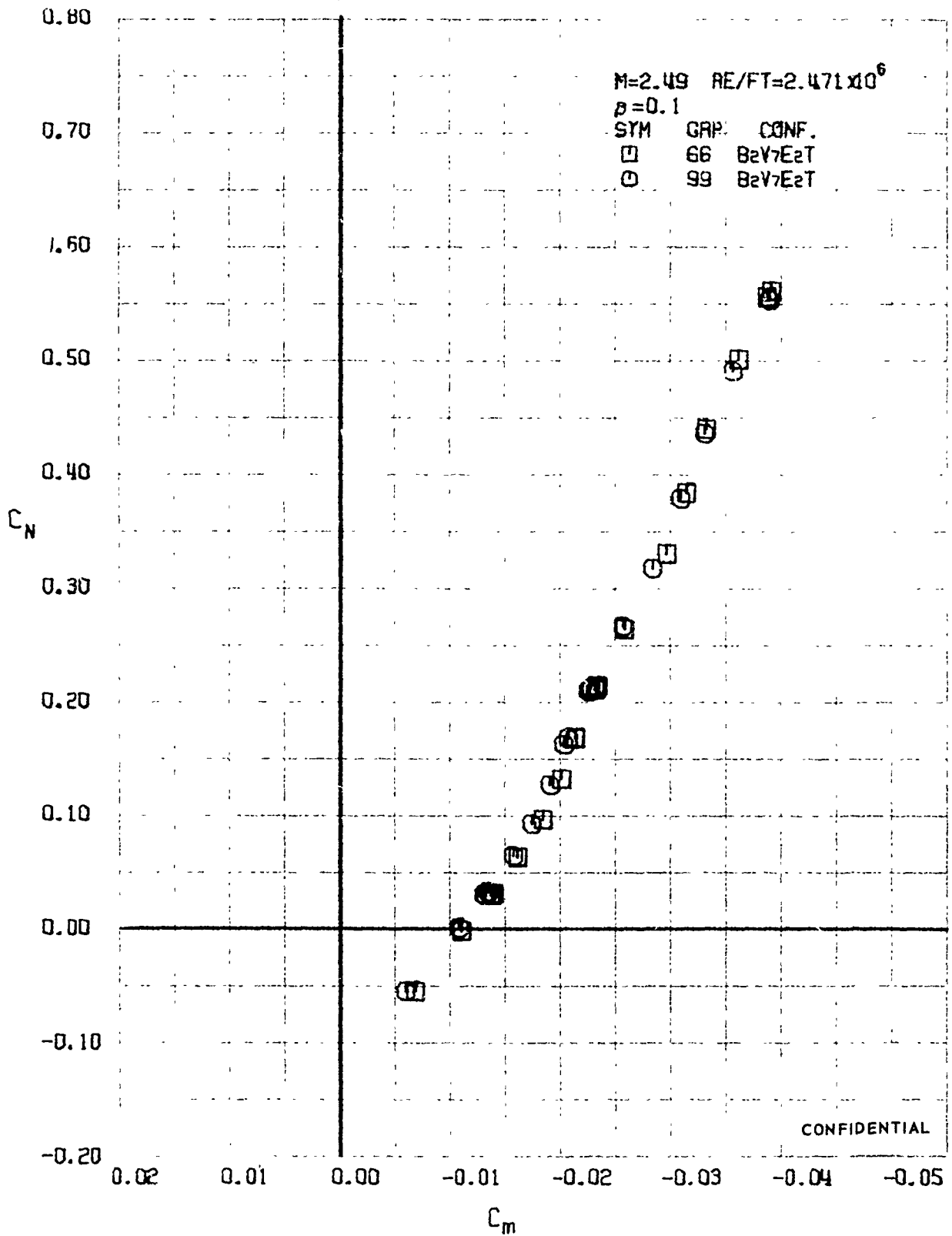
FIGURE 148 (U) REPEATABILITY - LONGITUDINAL STABILITY VARIATION (M=2.49)
