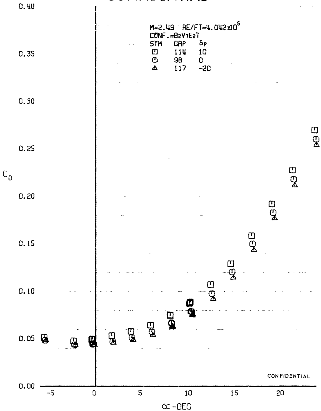
FIGURE 12 (U) ELEVON EFFECTS - DRAG COEFFICIENT VARIATION WITH ANGLE OF ATTACK (M=2.49)
