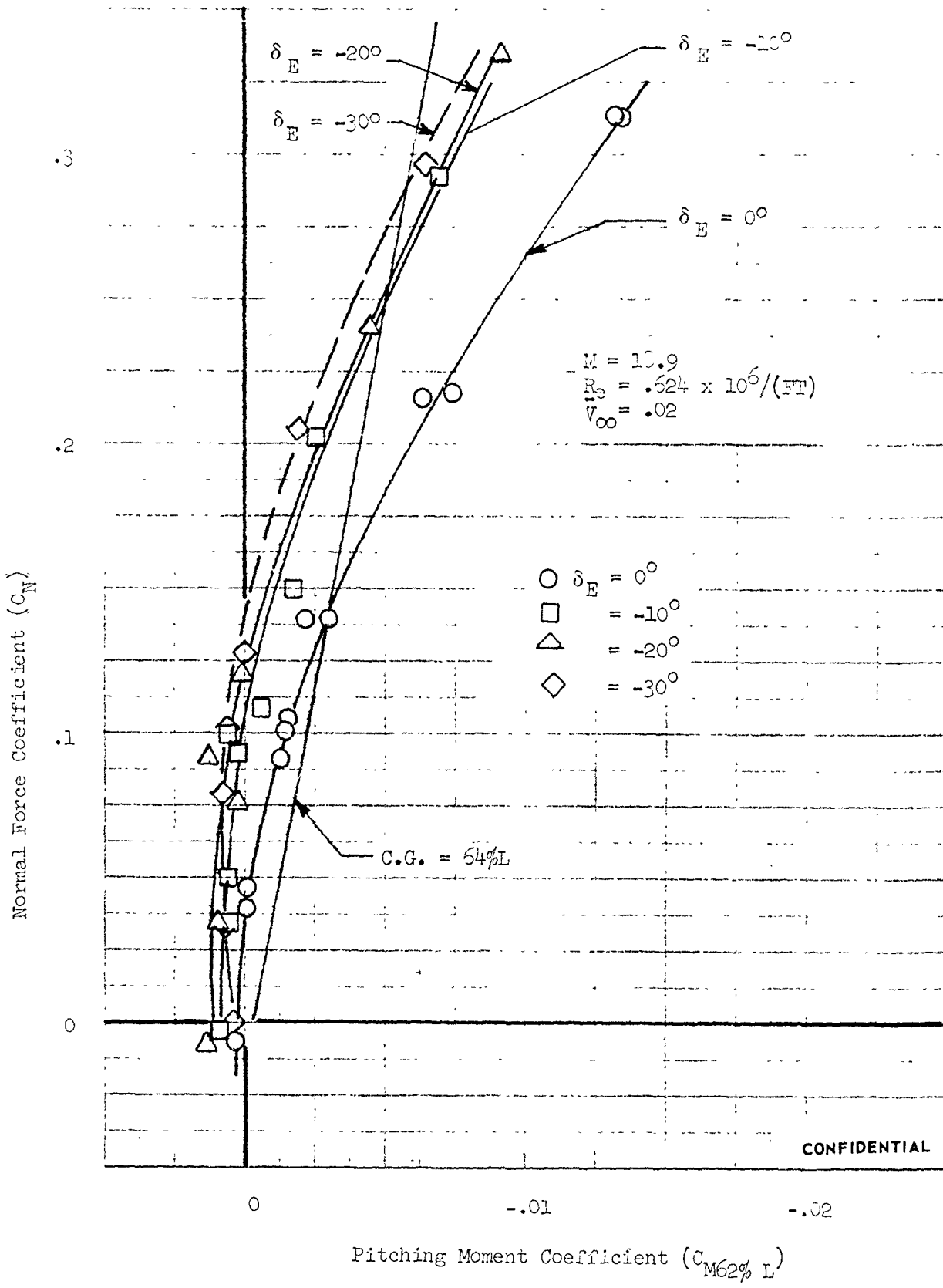
FIGURE 310 (U) FDL-5 LONGITUDINAL STABILITY ( M = 18.9 )
