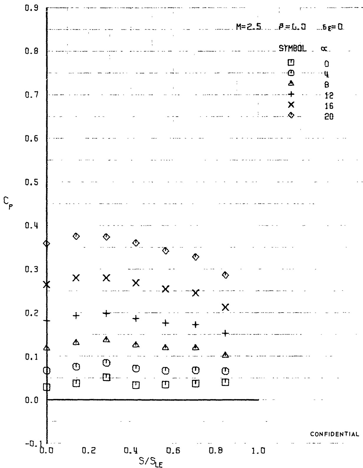
FIGURE 354 (U) LOWER SURFACE SPANWISE PRESSURES AT X/L = 0.50
