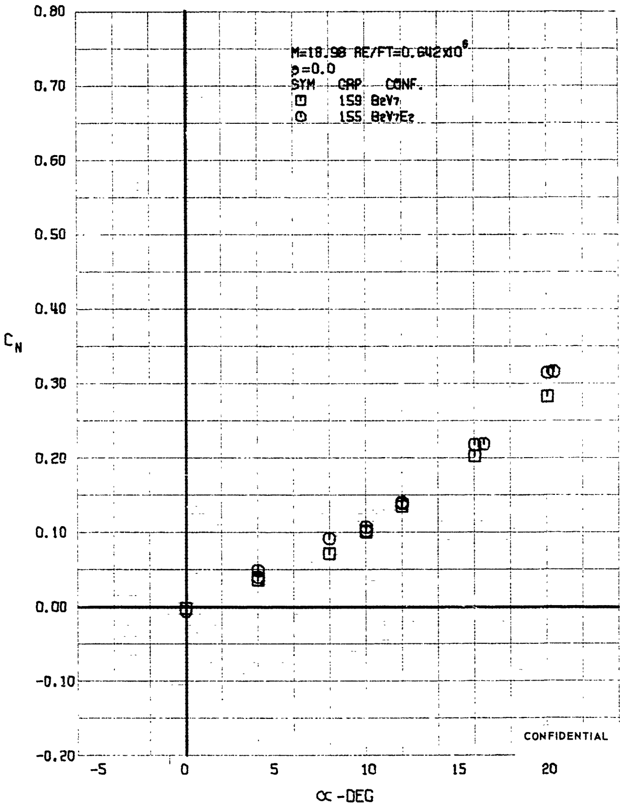
FIGURE 297 (U) CONFIGURATION BUILDUP - NORMAL FORCE COEFFICIENT VARIATION WITH ANGLE OF ATTACK ( M=18.98 )
