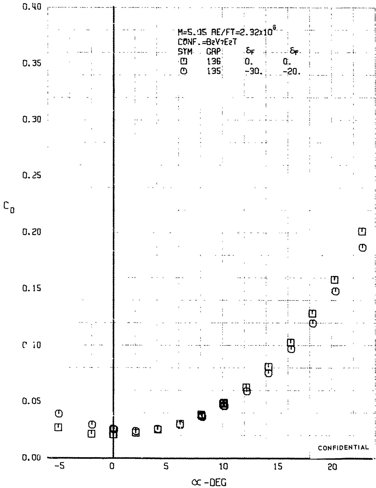
FIGURE 2.2 (U) COMBINED ELEVON AND FLAP EFFECTS - DRAG COEFFICIENT VARIATION WITH ANGLE OF ATTACK (M=5.05)
