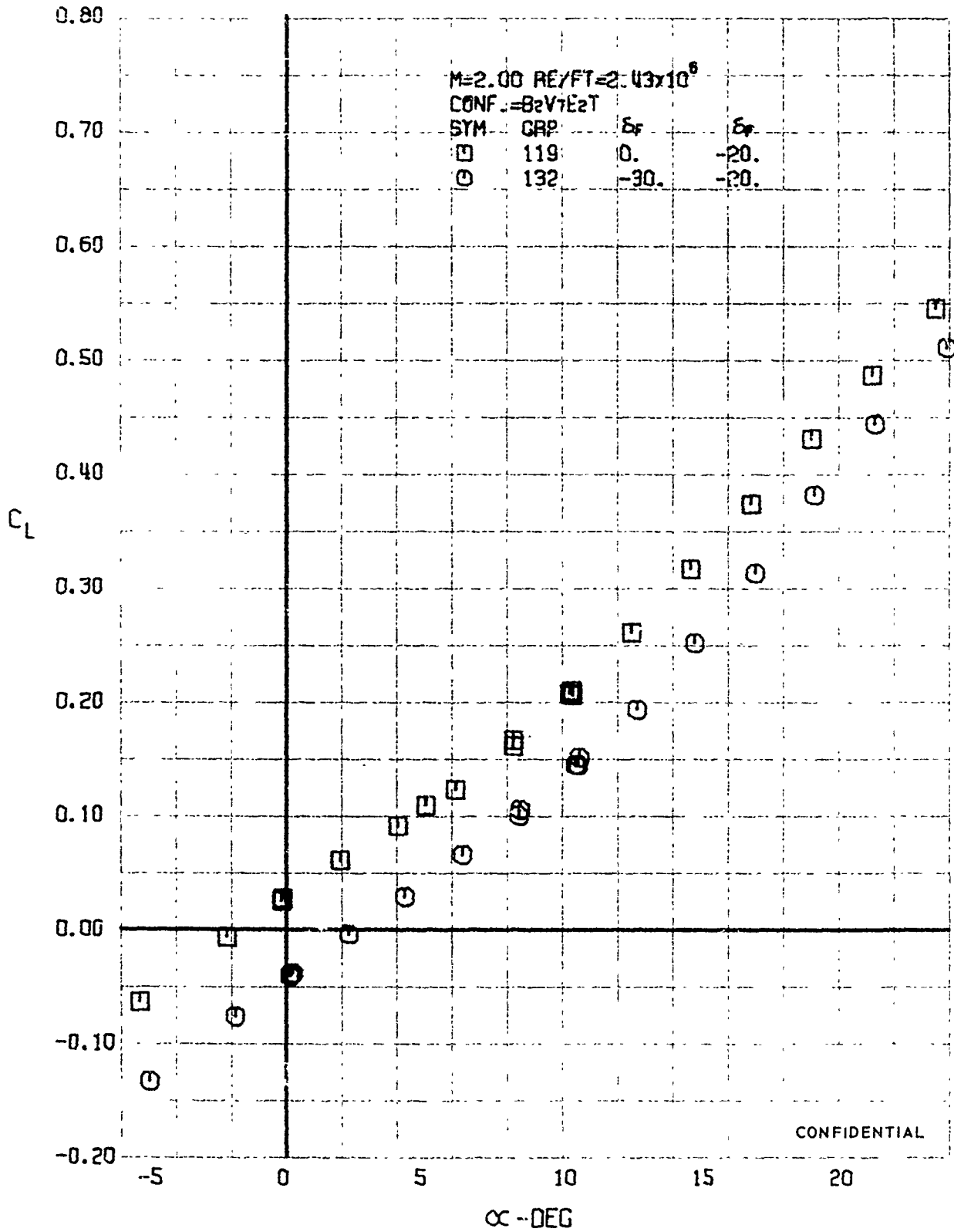
FIGURE 78 (1) FLAP EFFECTS - LIFT COEFFICIENT VARIATION WITH ANGLE OF ATTACK (M=2.00)
