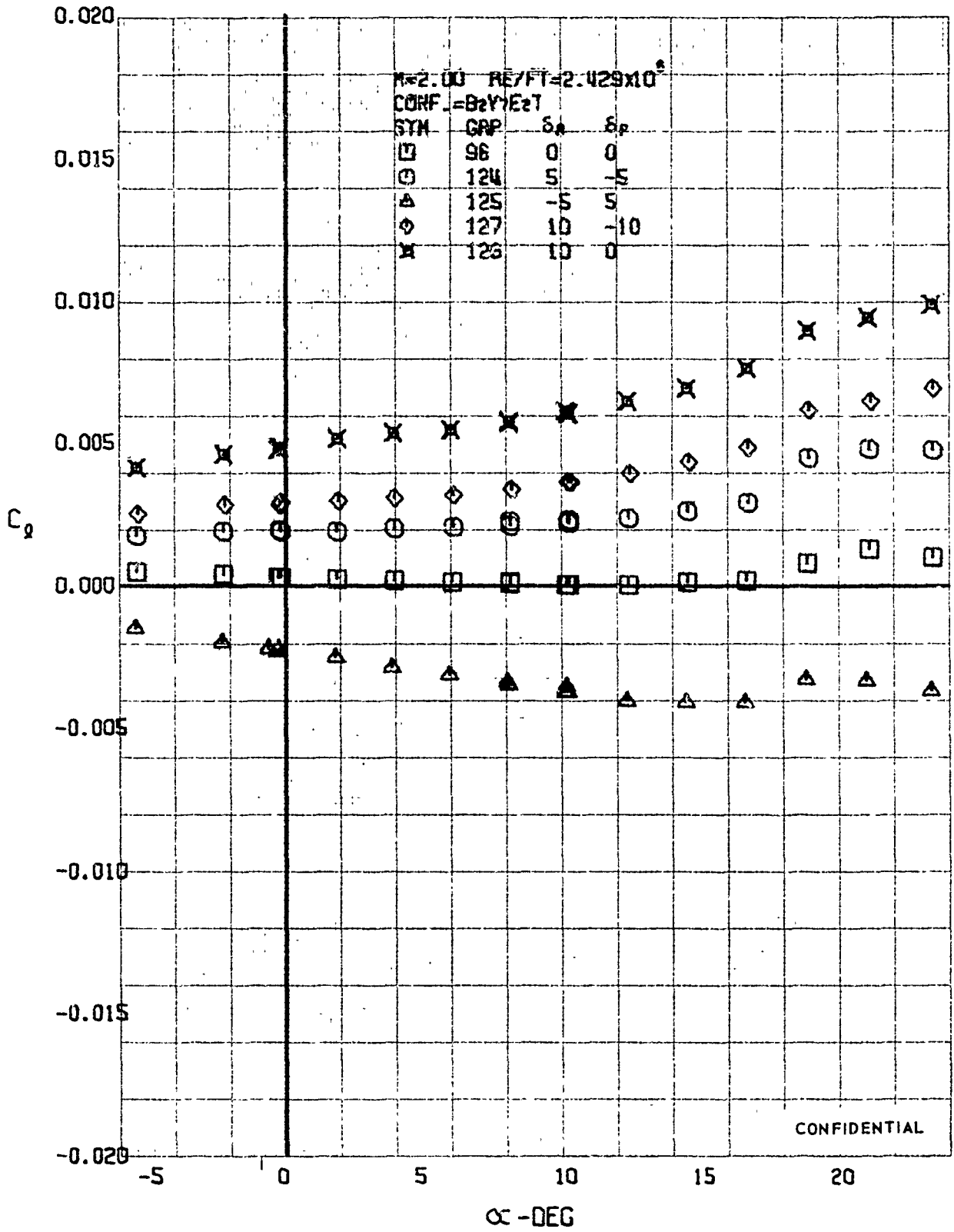
FIGURE 90 (U) AILERON EFFECTS - ROLLING MOMENT COEFFICIENT VARIATION WITH ANGLE OF ATTACK ( M=2.00 )
