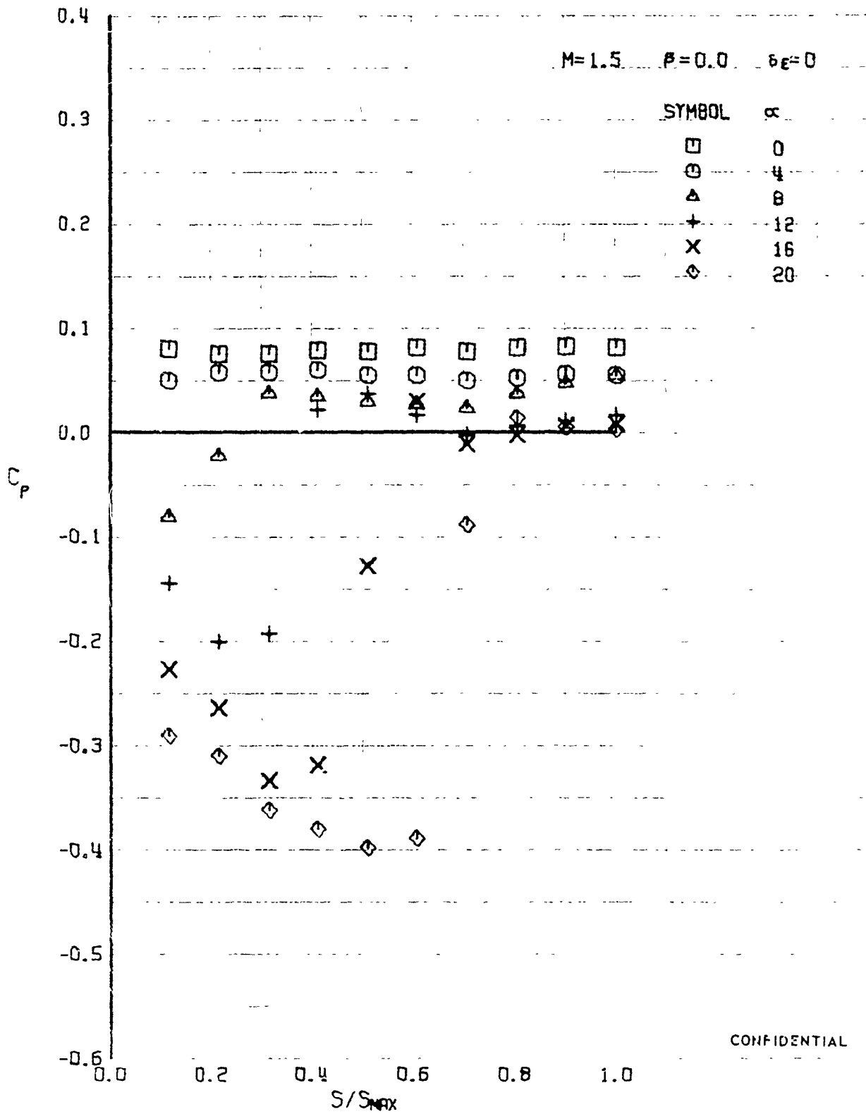
FIGURE 33 1 (U) UPPER SURFACE SPANWISE PRESSURES AT X/L = 0.50
