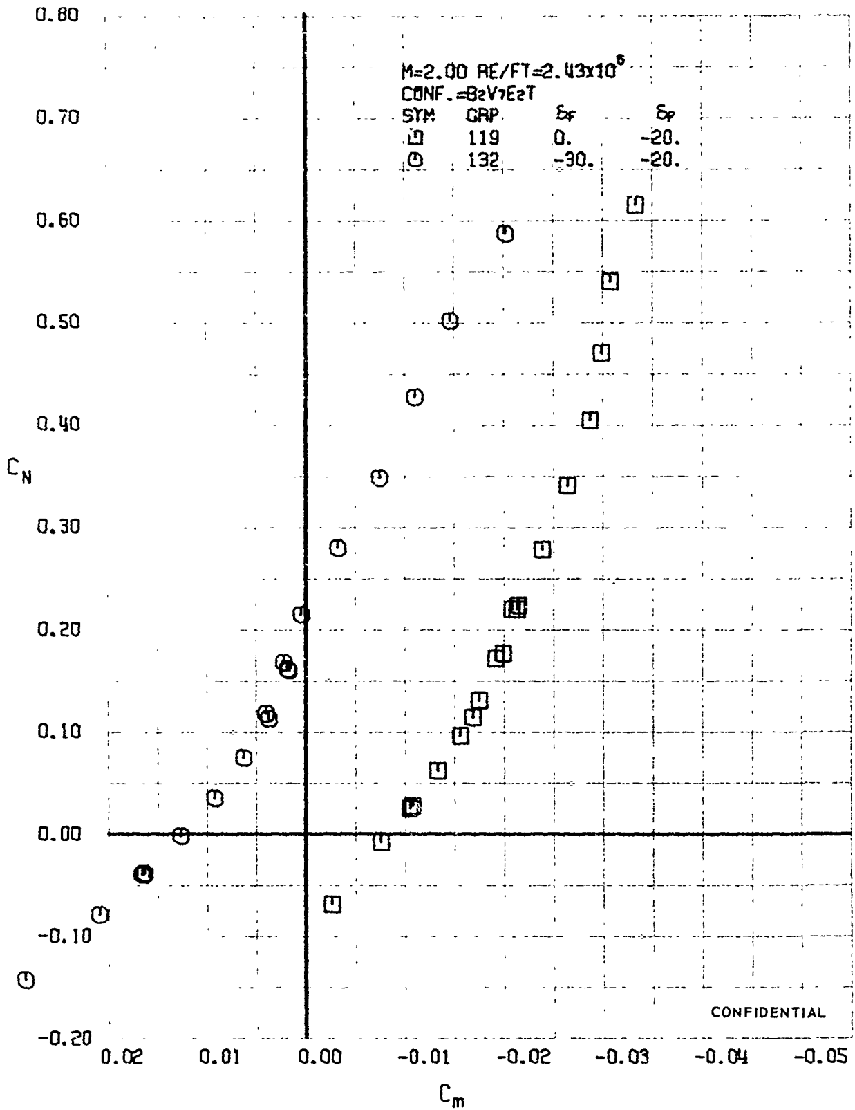
FIGURE 77 (U) FLAP EFFECTS - LONGITUDINAL STABILITY VARIATION (M=2.00)
