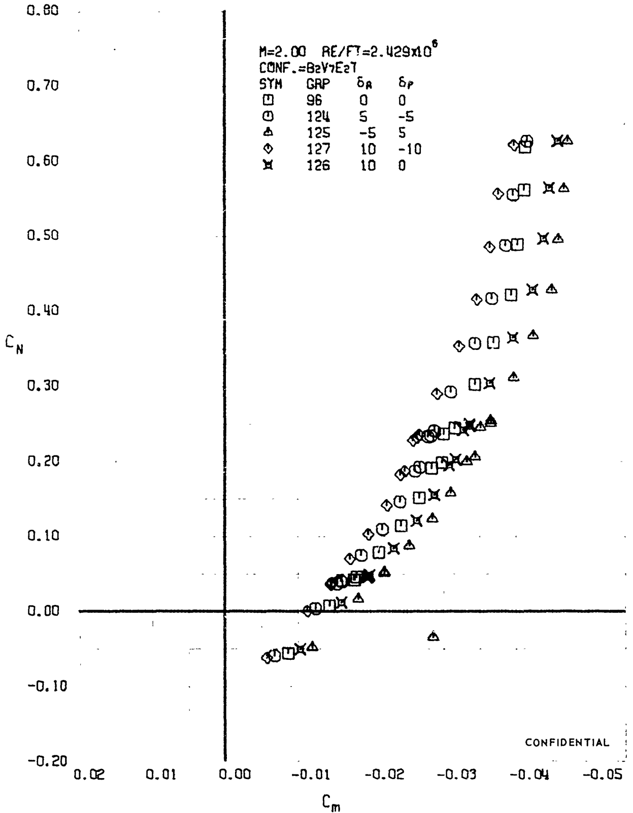
FIGURE 8L (U) AILERON EFFECTS - LONGITUDINAL STABILITY VARIATION (M=2.00)
