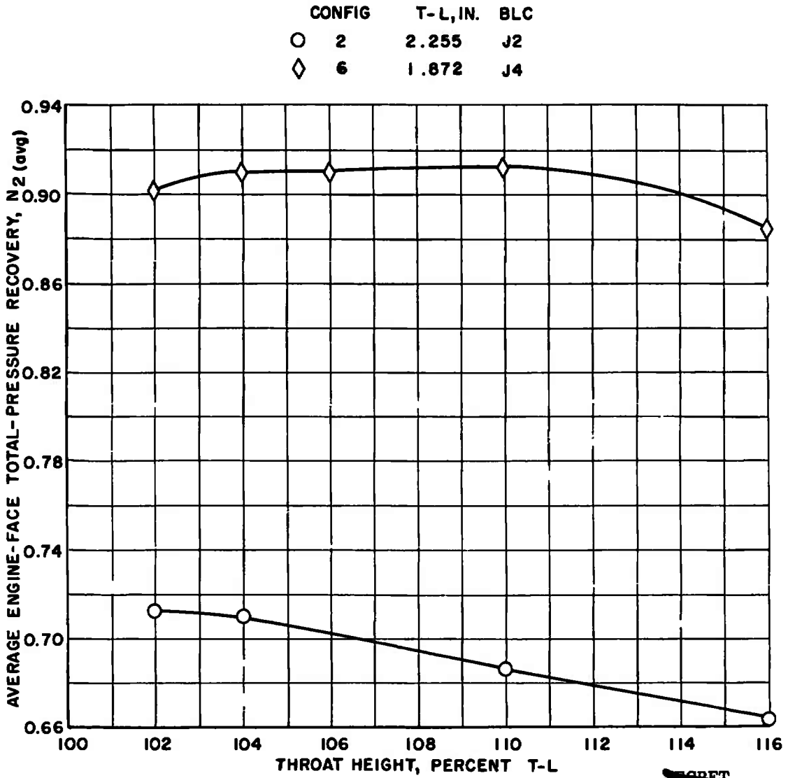
Fig. 12 (b)(7)(C) Variation in Total-Pressure Recovery as a Function of Throat Height for BLC Configurations J2 and J4, M_\infty = 2.20 , \alpha = 4.0 deg, \psi = 0 deg
