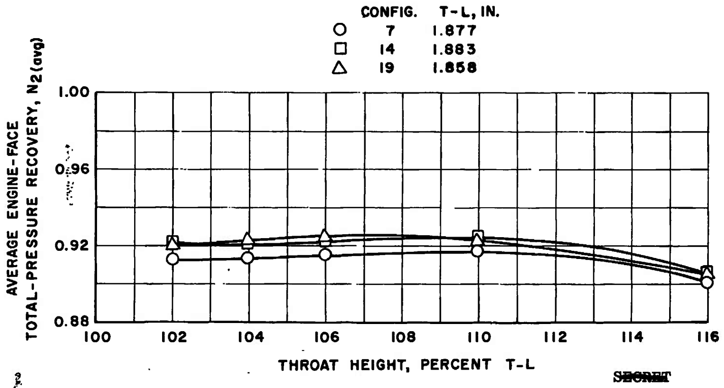
Fig. 19 (Secret) Variation in Total-Pressure Recovery as a Function of Throat Height for Model Configurations 7, 14, and 19, M_{\infty} = 2.20 , \alpha = 4.0 deg, \psi = 0 deg
