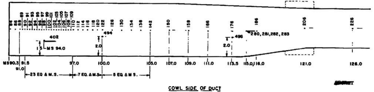
Fig. 9 (Unclassified) Duct Pressure Instrumentation
