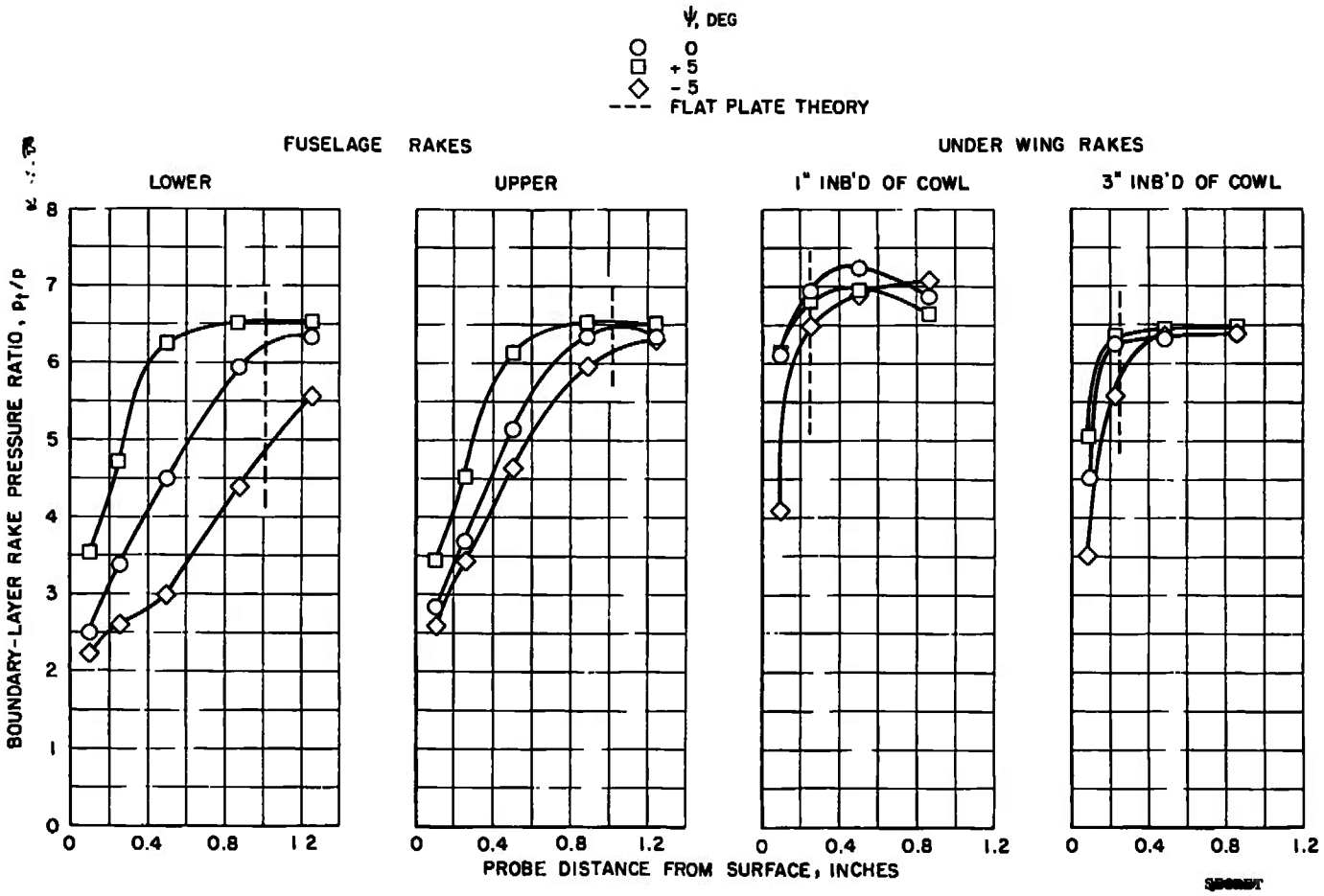
Fig. 11 Fuselage and Wing Boundary-Layer Total-Pressure Profiles at M_\infty = 2.20
