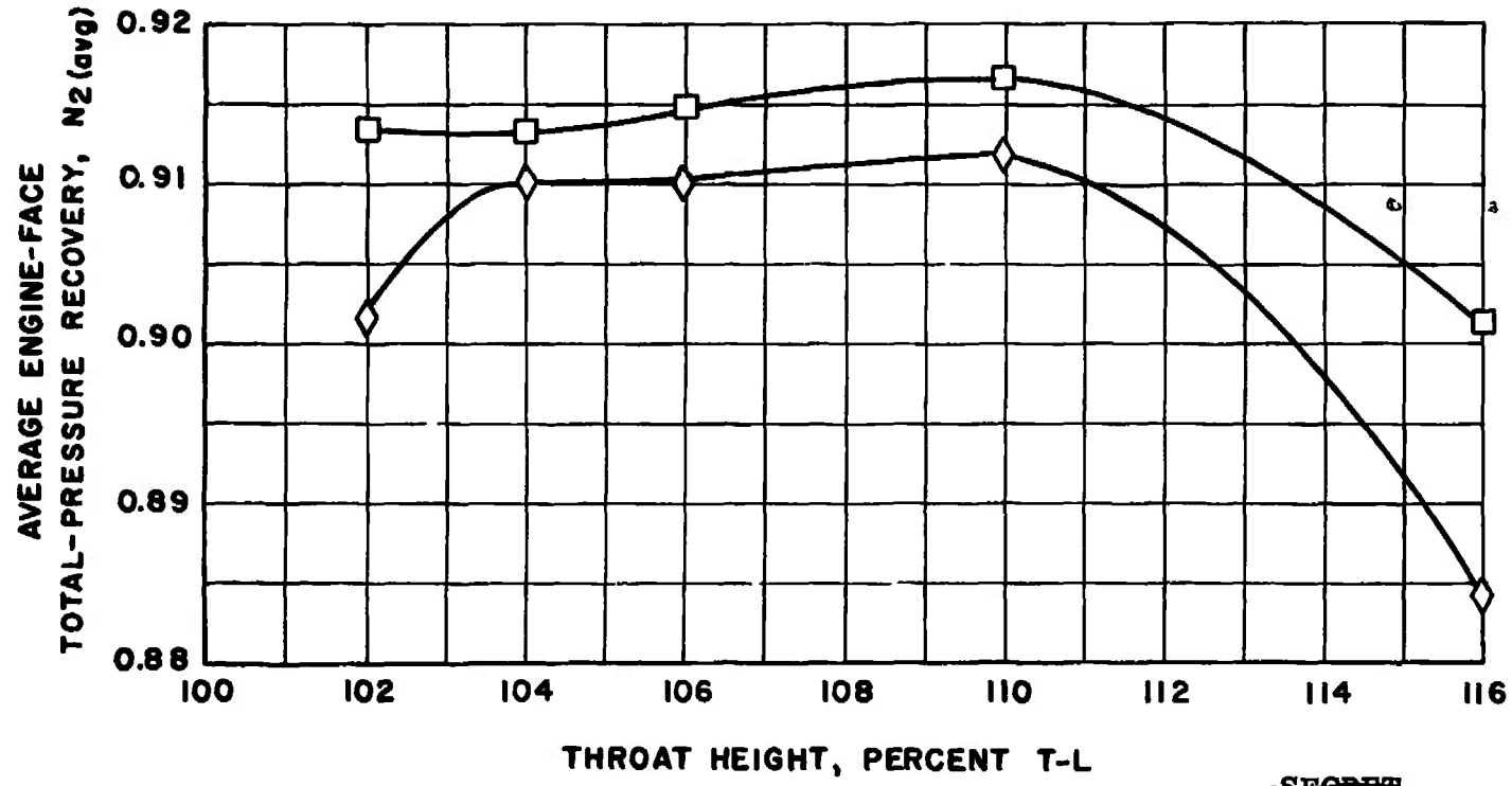
Fig. 15 Variation in Total-Pressure Recovery as a Function of Throat Height for Subsonic Diffusers A and D, M_{\infty} = 2.20 , \alpha = 4.0 deg, \psi = 0 deg
