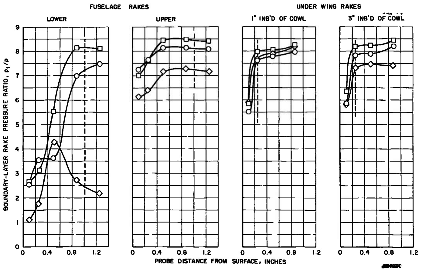
c. \alpha = 11.0 deg Fig. 11 Concluded
