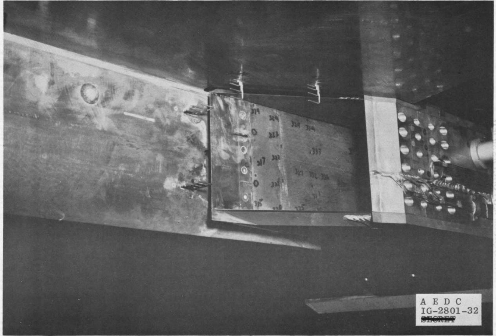
Fig. 6 (Unclassified) Photograph of Inlet Boundary-Layer Rakes
