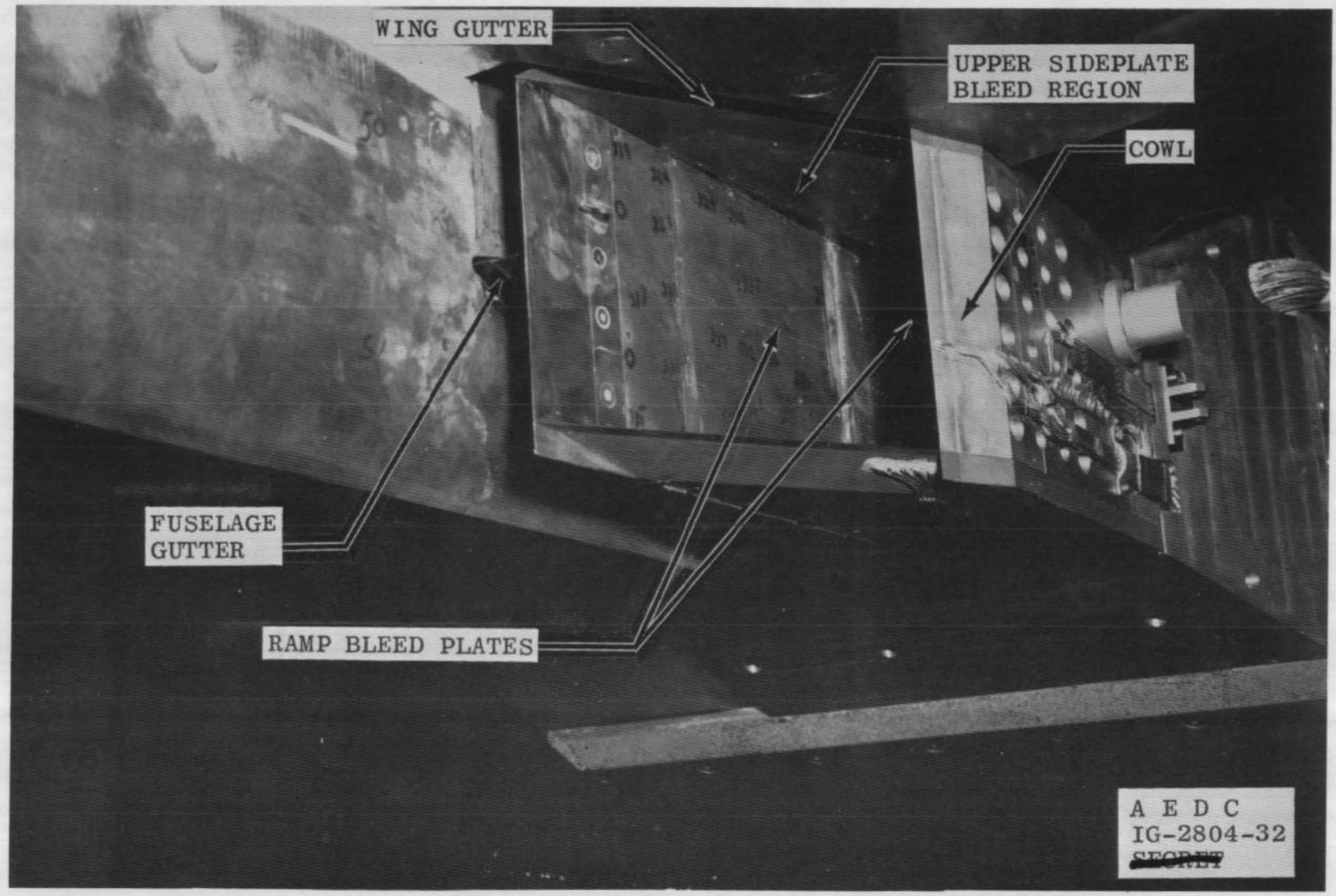
b. Boundary-Layer Gutters and Porous Plate Installation on Ramp and Upper Sideplate Fig. 3 Concluded
