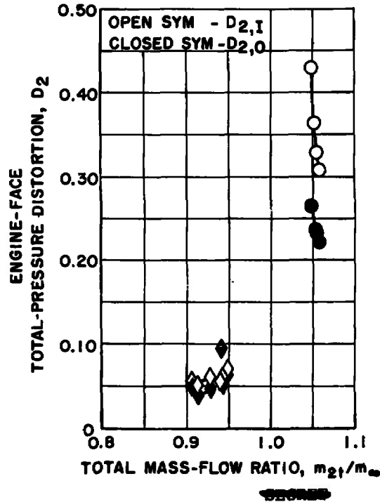
Fig. 13 ( SECRET ) Inlet Performance BLC Configurations J2 and J4 as a Function of Mass-Flow Ratio, M_\infty = 2.20 , \alpha = 4.0 deg, \psi = 0 deg
