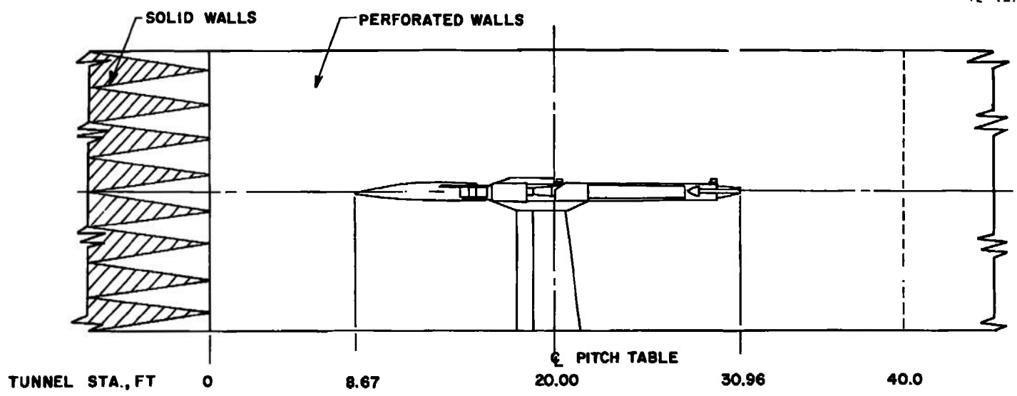
MODEL LAYOUT IN THE 16T TEST SECTION
