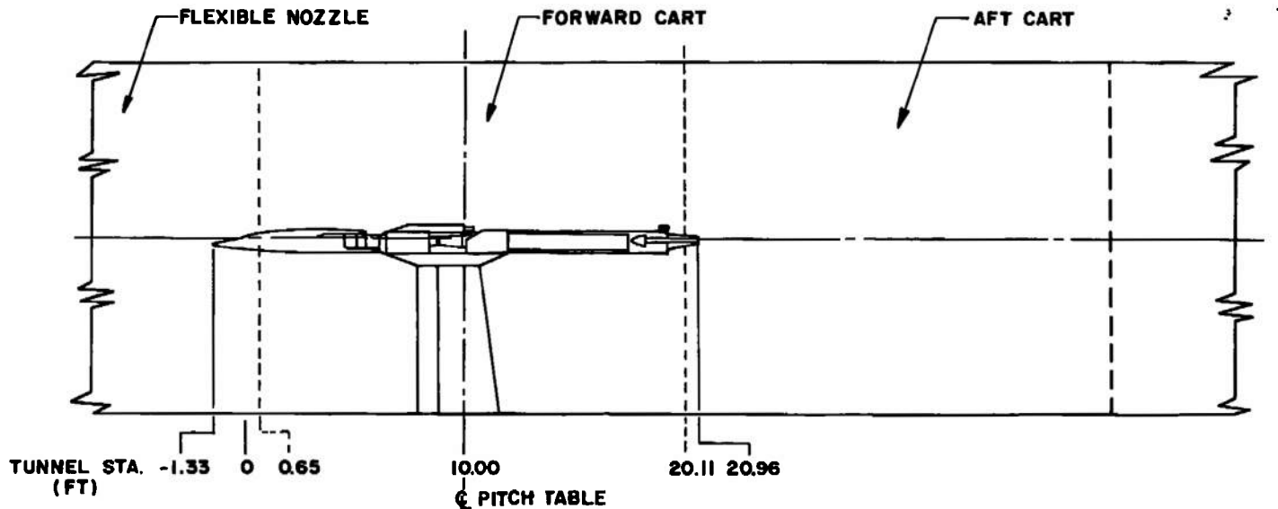
MODEL LAYOUT IN THE 16S TEST SECTION
