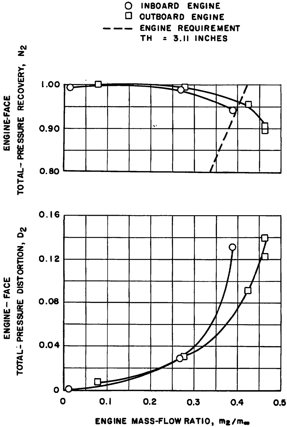
b. M_\infty = 0.85 , Configuration 22
