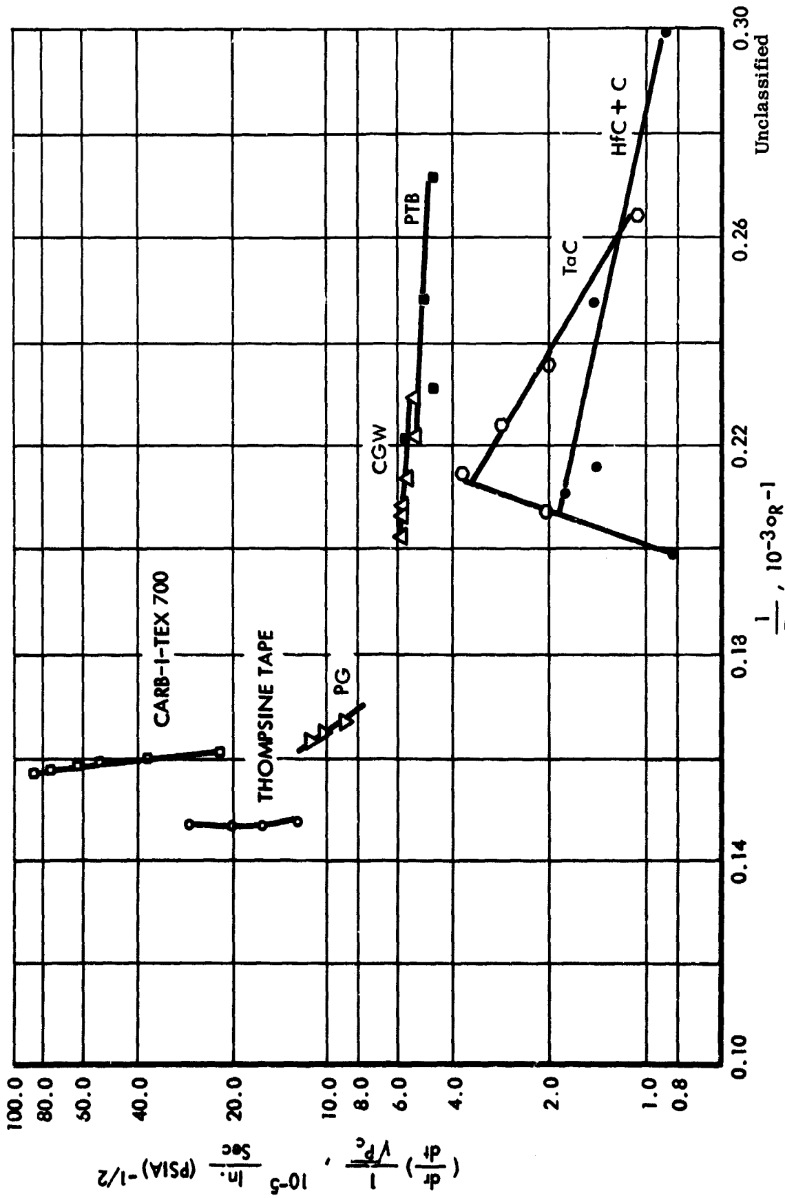
FIGURE 120 (U) CORRELATED EROSION DATA
