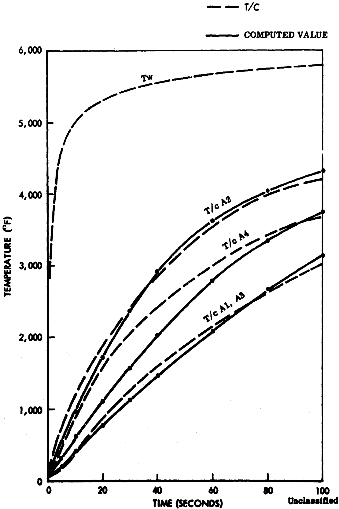
FIGURE 95 (U) THEORETICAL ACTUAL TEMPERATURE COMPARISON FOR UNIT S/N 1: RUN 281
