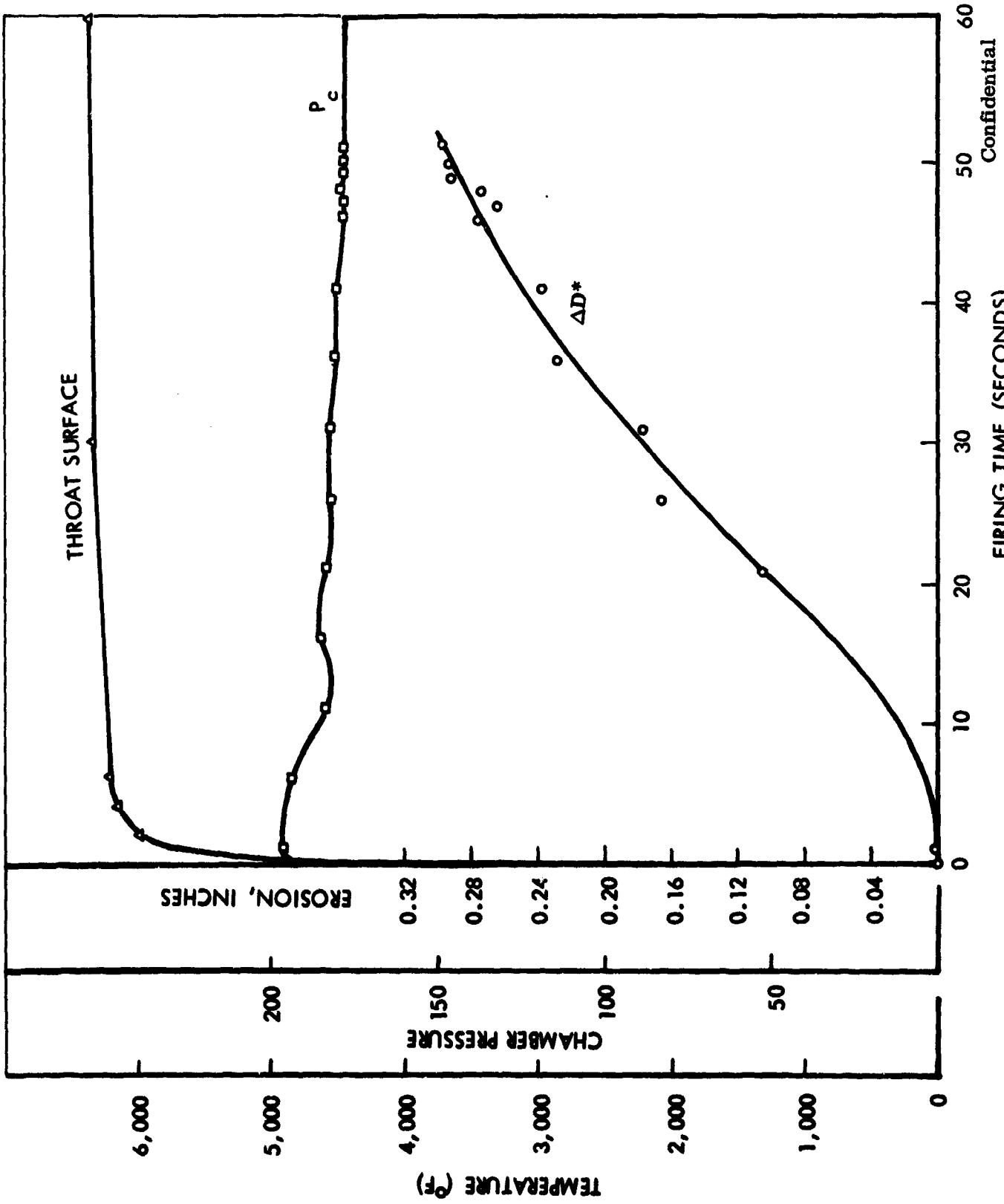
FIGURE 94 (U) UNIT S/N 3 DATA: RUN 348
