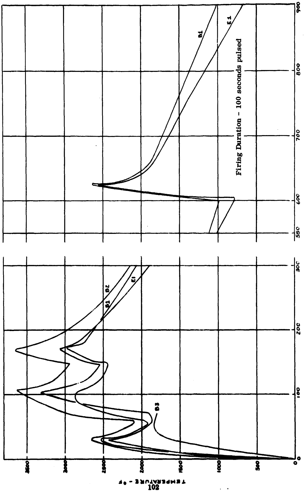
FIGURE 63 (U) Thermocouple Data, Run 057
