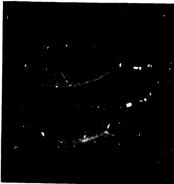
FIGURE 30 (U) Unit S/N 2 Assembly Unclassified
