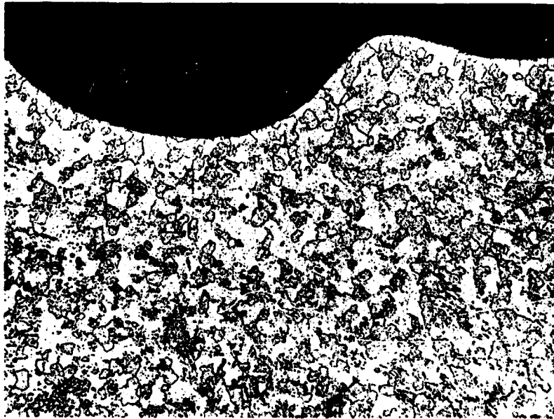
a) Surface Microstructure of W-2% ThO 2 Nozzle Throat Insert - High Erosion Area of Test Fired Insert.
