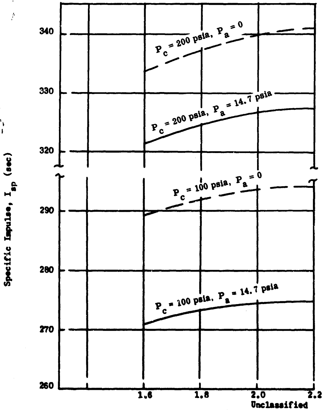
Mixture Ratio ( ^{\circ}/F ) LF/ N_2H_4 Blend Propellants FIGURE 4 (6) Theoretical Specific Impulse
