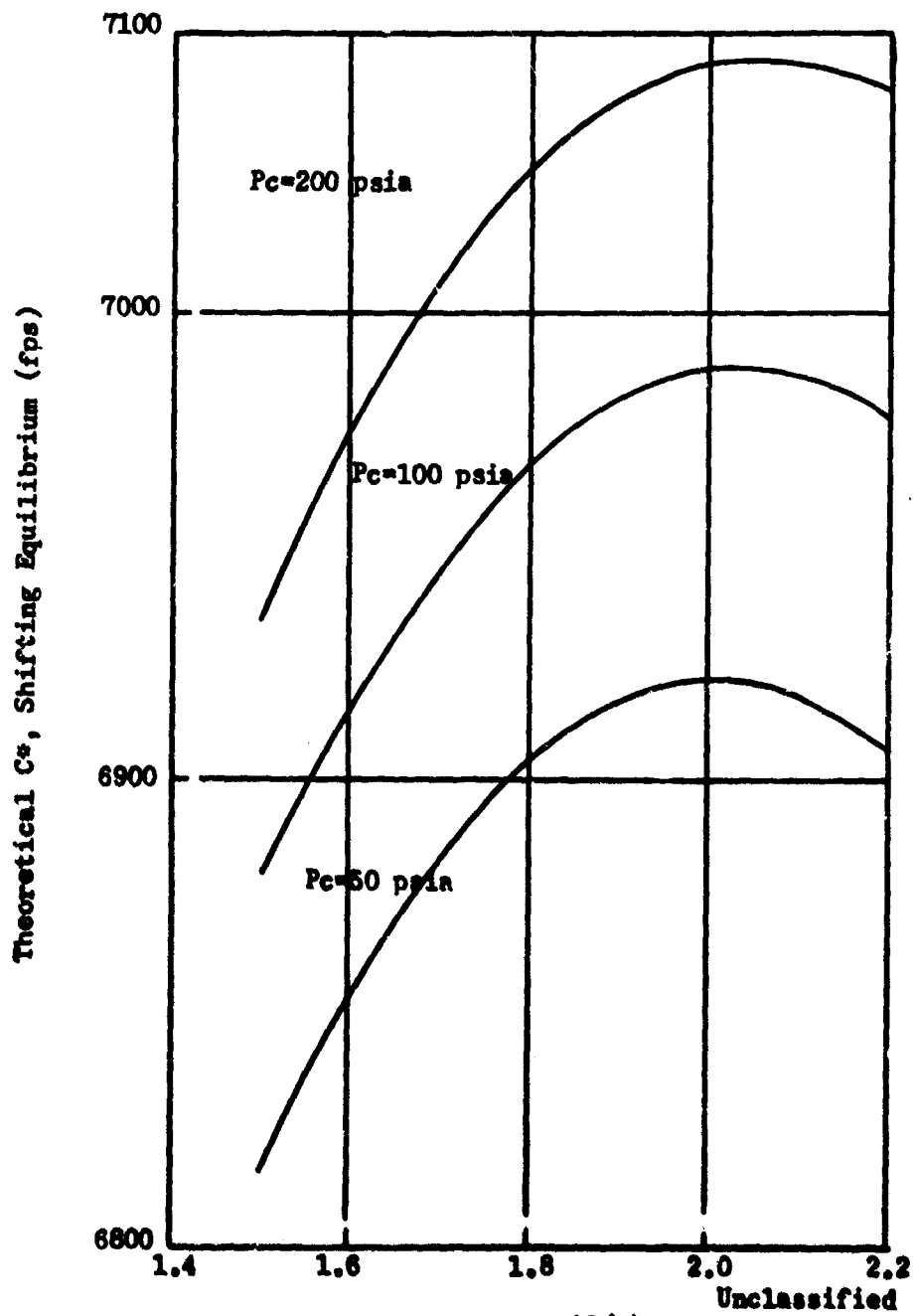
Mixture Ratio (°/F) LF_2/N_2H_4 Blend Propellants FIGURE 3 (U) Theoretical C* vs. Mixture Ratio
