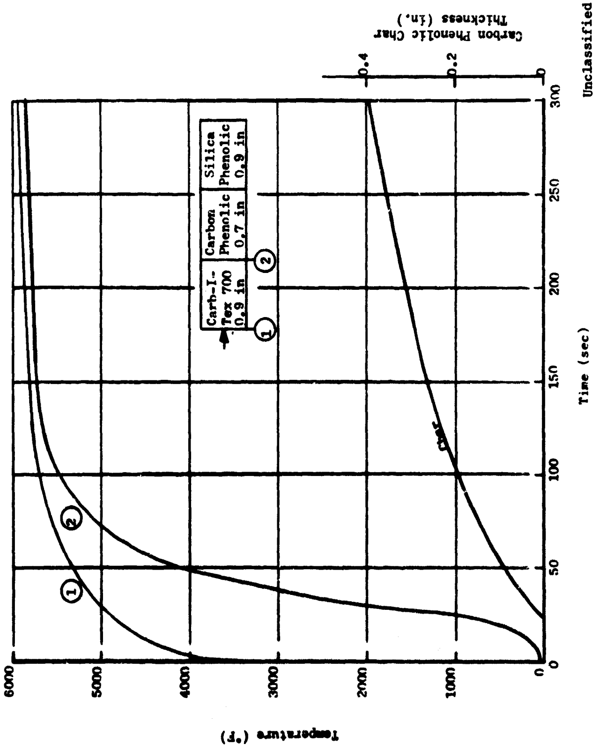
FIGURE 20 (L) Temperature Distribution at Throat for Unit S/N 3
