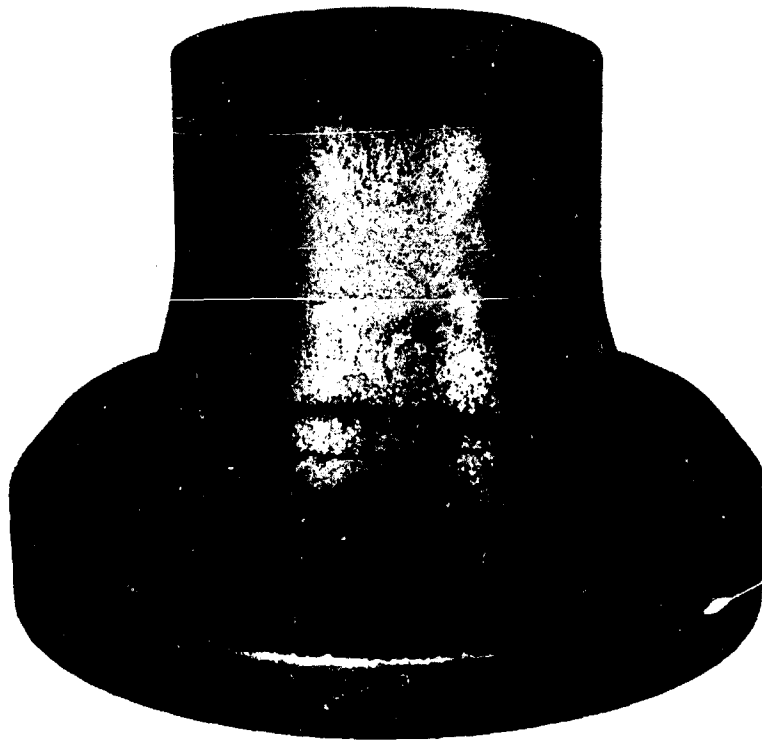
FIGURE 43 (U) Back Side of Prestressed Throat Insert Assembly
