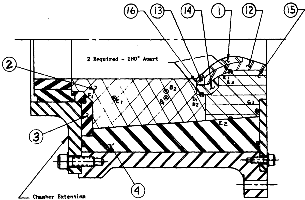
FIGURE 7 (U) Subscale Thrust Chamber S/N 1
