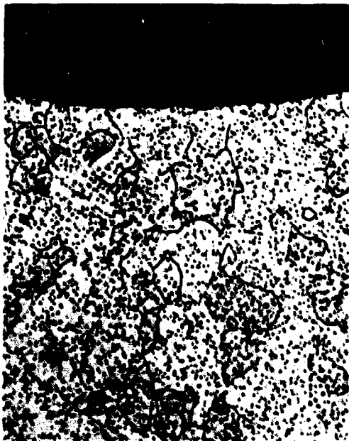
a) Surface Microstructure of W-2% ThO 2 Nozzle Throat Insert - High Erosion Area of Test Fired Insert.
