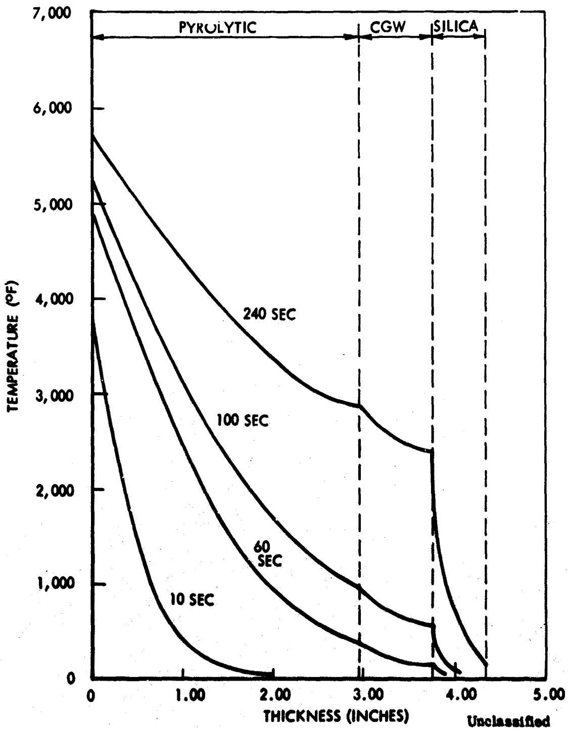
FIGURE 78 (U) PREDICTED TEMPERATURE PROFILE AT STATION 2: FULL SCALE UNIT 8/N 2
