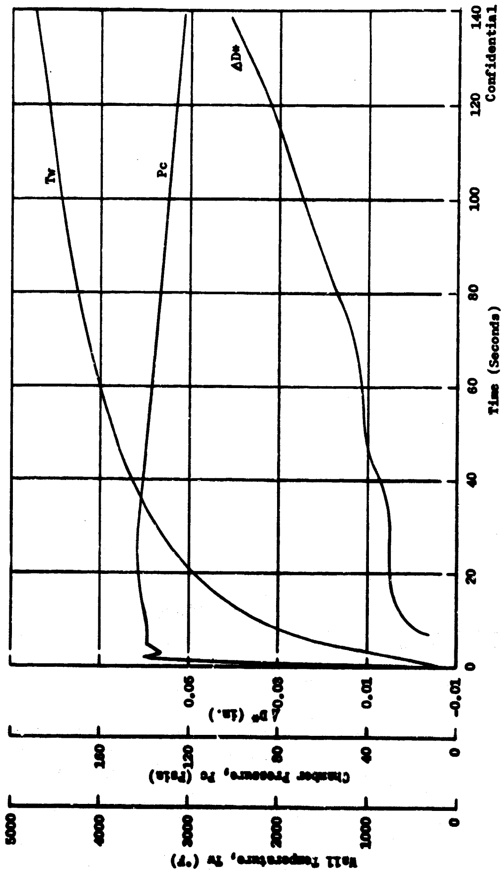
FIGURE 65 (U) Unit S/N 2 Data: Run 049
