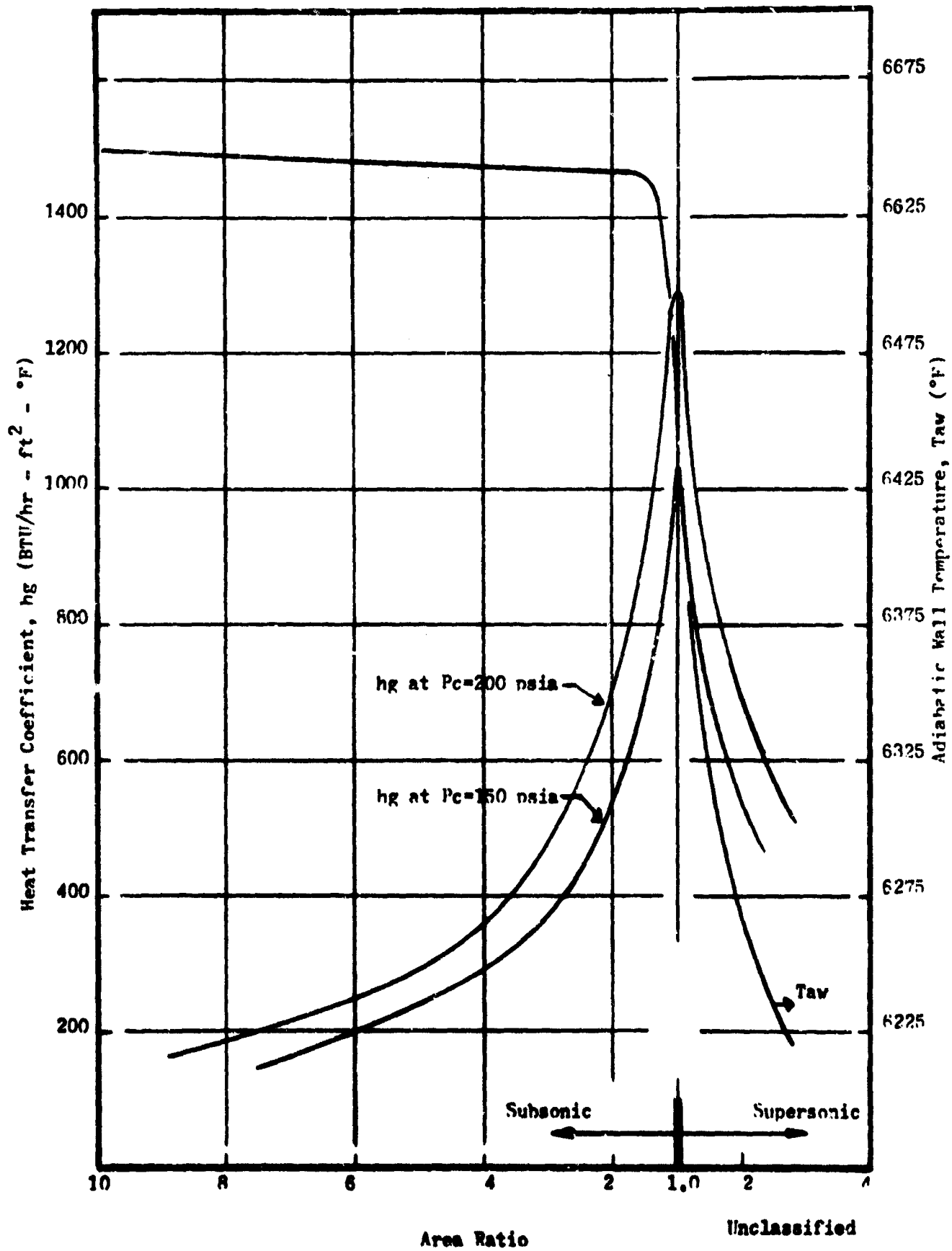
FIGURE 5 (U) Heat Transfer Coefficient and Adiabatic Wall Temperature; Subacale Thrust Chambers
