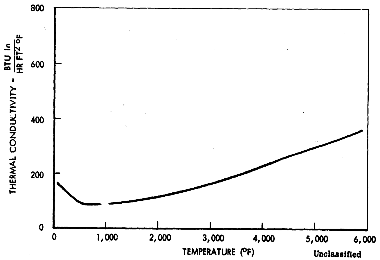
FIGURE 96 (U) THERMAL CONDUCTIVITY VERSUS TEMPERATURE FOR CARB-I-TEX 700
