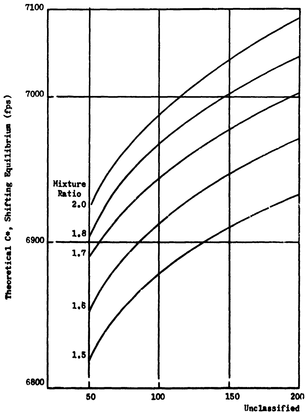
Chamber Pressure LF 2 /N 2 H 4 Blend Propellants FIGURE 2 (U) Theoretical C* vs. Chamber Pressure
