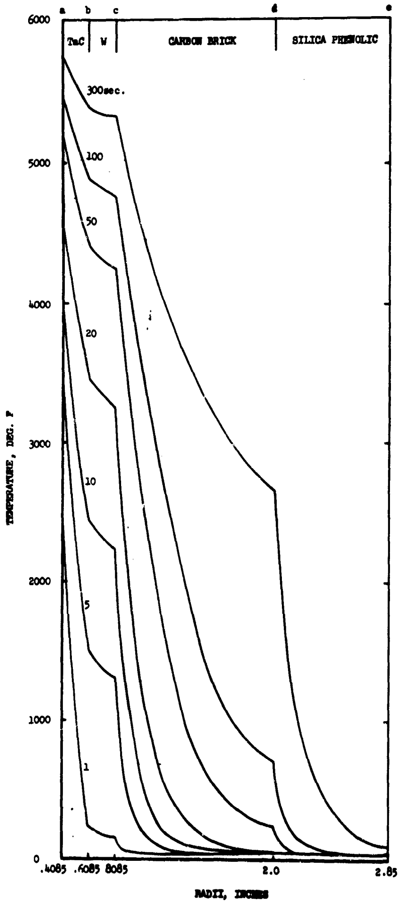
FIGURE 15 (U) Temperature Profile for Unit S/N 1
