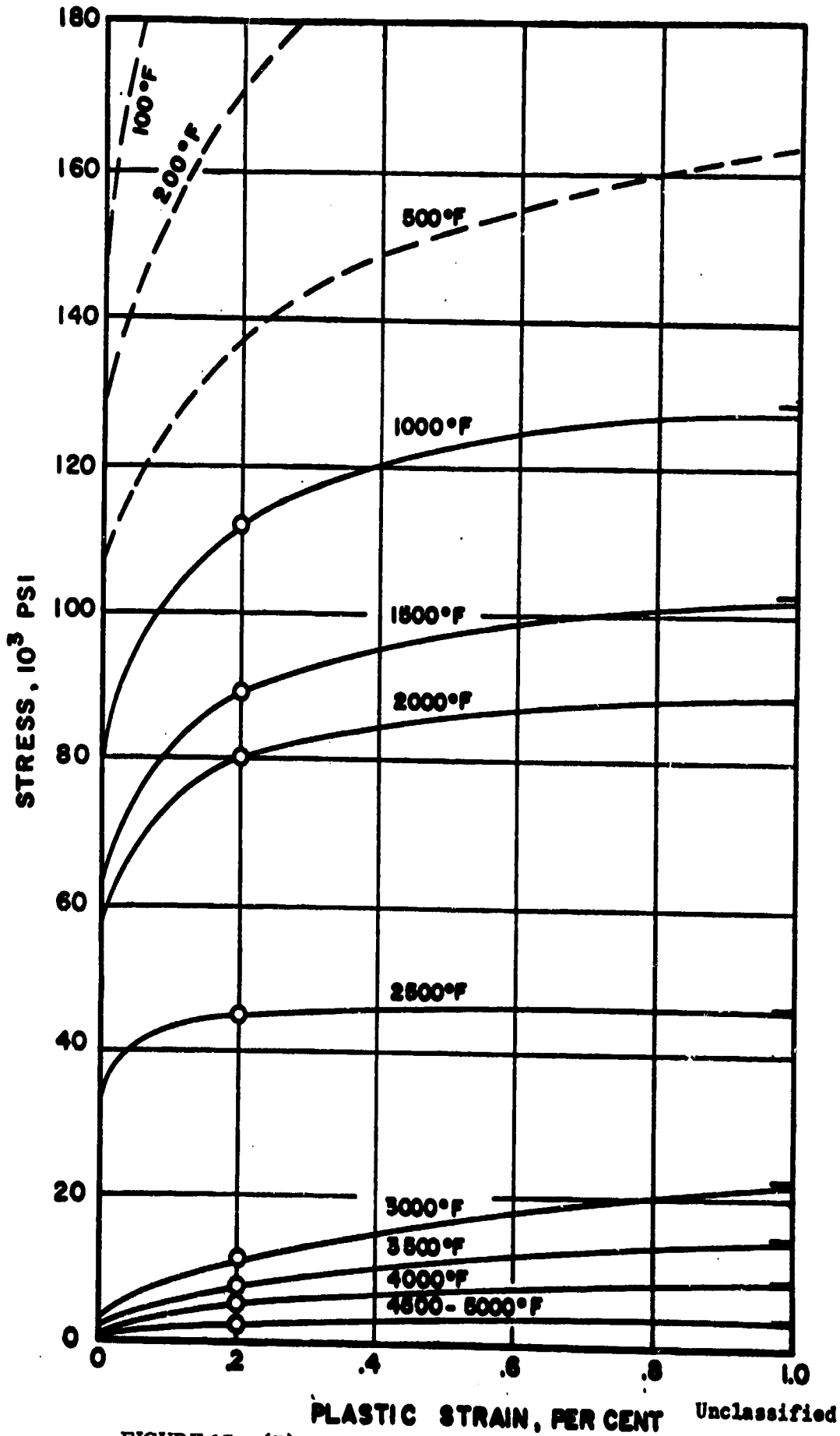
FIGURE 17 (U) Stress-Strain Behavior of Tungsten
