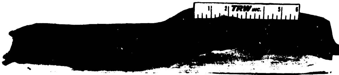
FIGURE 115 (U) Unit S/N 3 Axial Segment, Repaired Area
