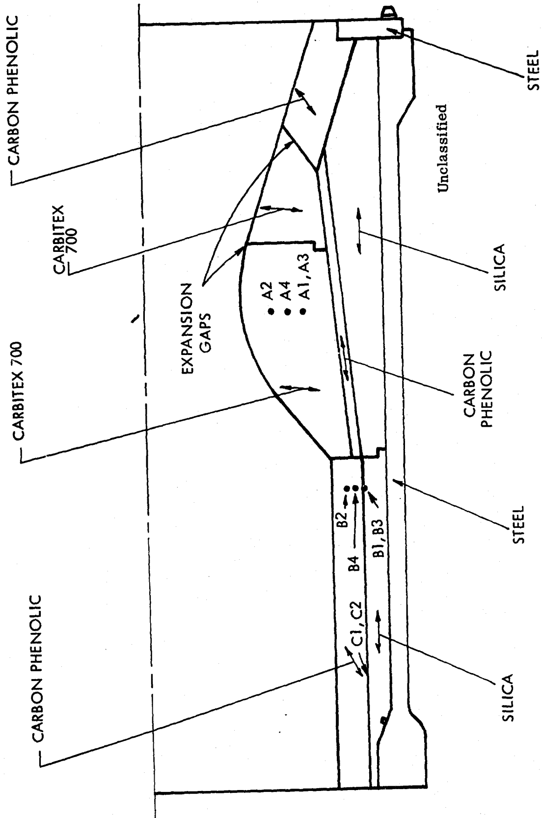
FIGURE 70 (U) FULL SCALE THRUST CHAMBER S/N 1
