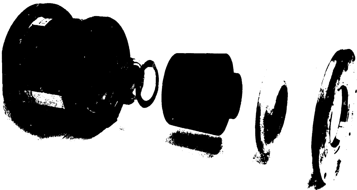
Unclassified FIGURE 28 (U) Unit S/N 1 Assembly
