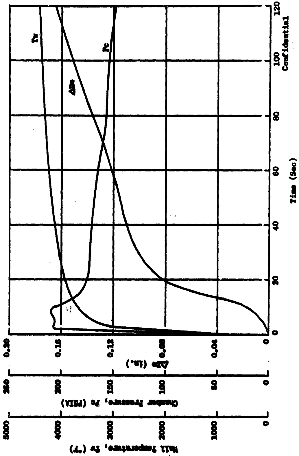
FIGURE 67 (U) Unit S/N 8 Data: Run 062
