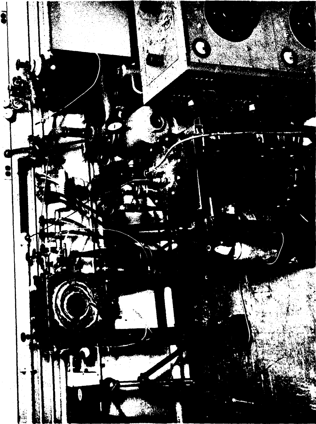
Figure 2 (U) Reactivity Test Apparatus
