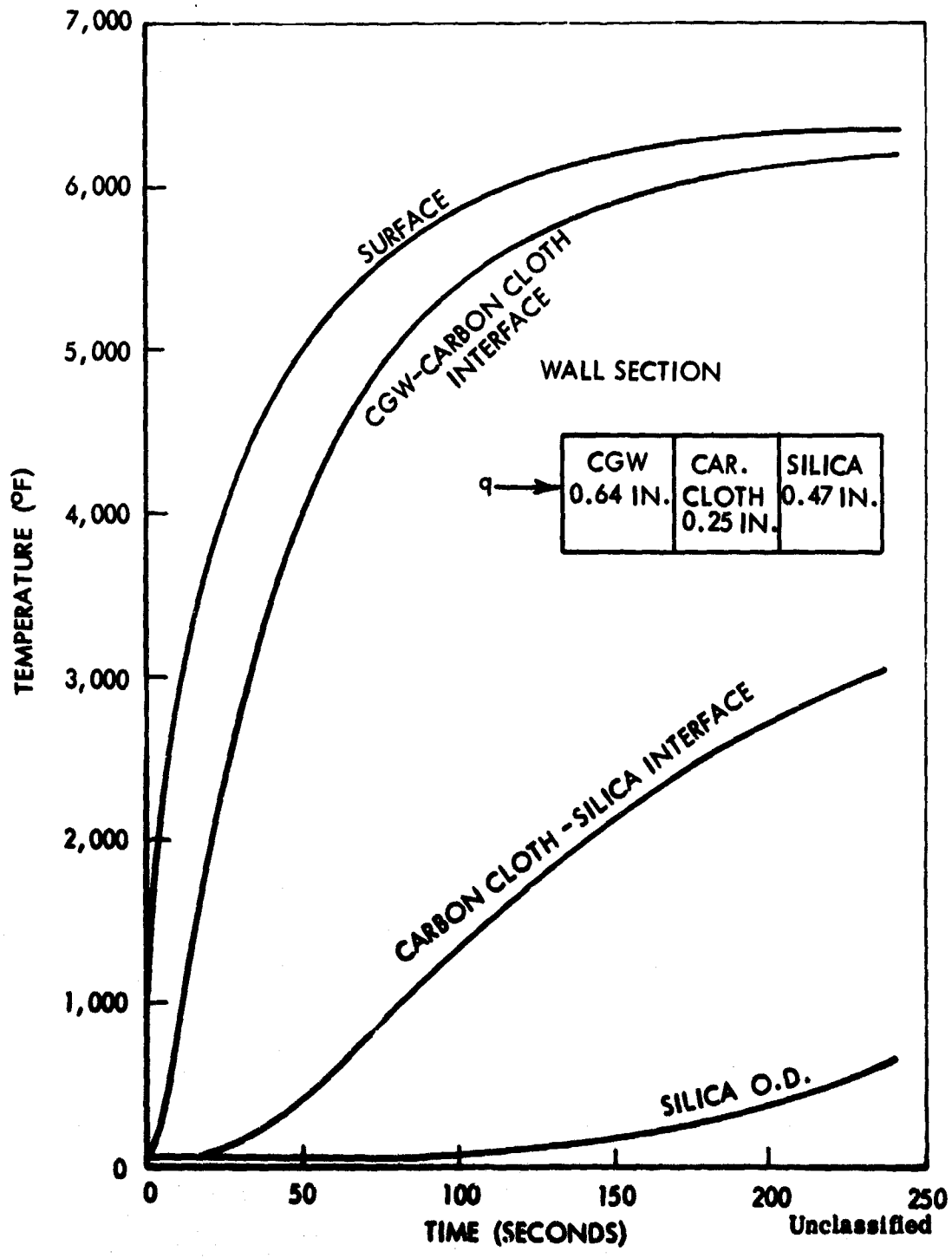
FIGURE 75 (U) PREDICTED TEMPERATURE DISTRIBUTION AT STATION 1 FOR UNIT 8/N 2
