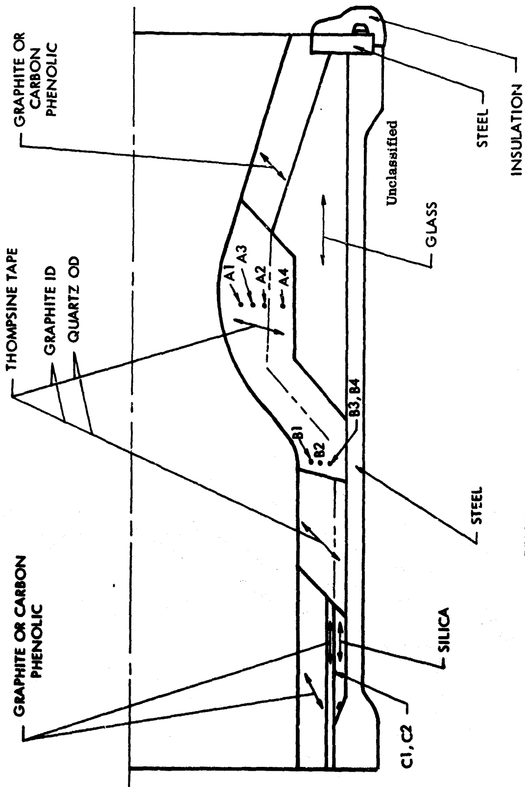
FIGURE 72 (U) FULL SCALE THRUST CHAMBER S/N 3
