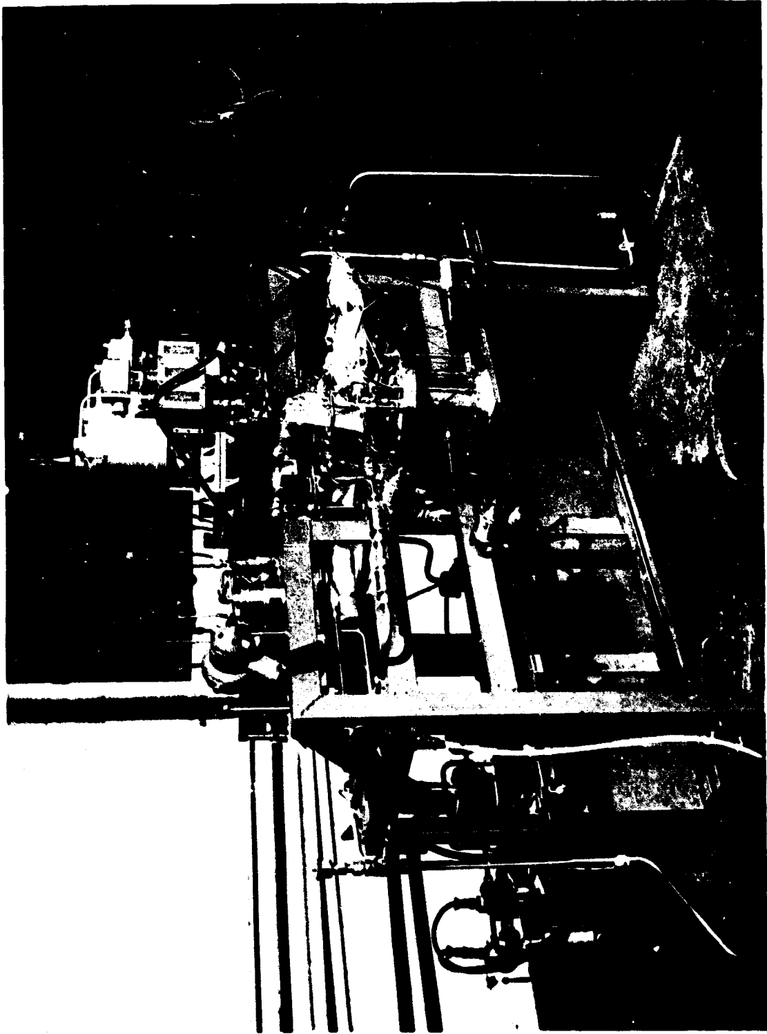
FIGURE 38 (U) Engine Assembly Installed on Test Stand
