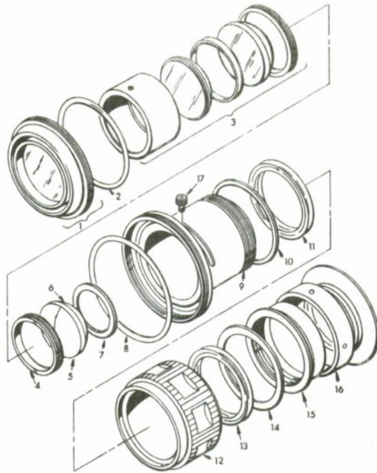
(U) FIGURE A-8. Small Starlight Scope, eyepiece assembly.
